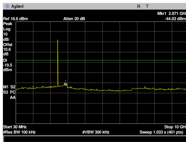
Plot 21: Conducted Spurious Emissions 30MHz-10GHz 2445MHz Mid Channel
