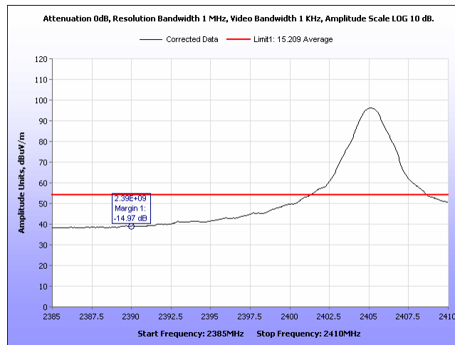
Plot 16: Radiated Band Edge, Low Channel 2405MHz, Average.
