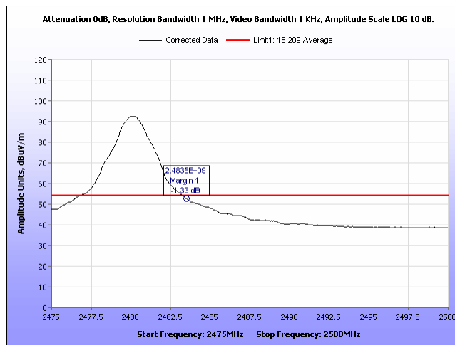
Plot 18: Radiated Band Edge, High Channel 2480MHz, Average.
