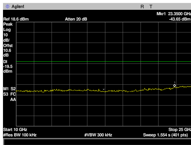
Plot 24: Conducted Spurious Emissions 10GHz-25GHz 2445MHz Mid Channel
