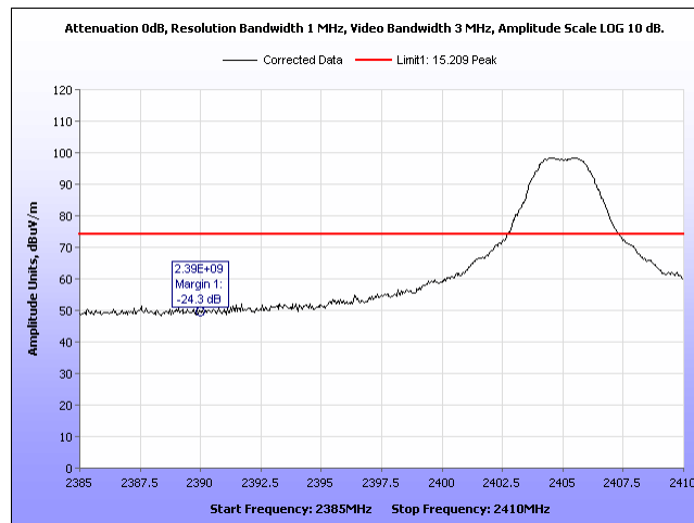
Plot 17: Radiated Band Edge, Low Channel 2405MHz, Peak.
