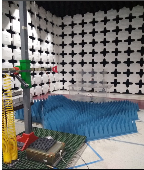
Photograph 1: Radiated Spurious Emissions Requirements, 1GHz-18GHz
