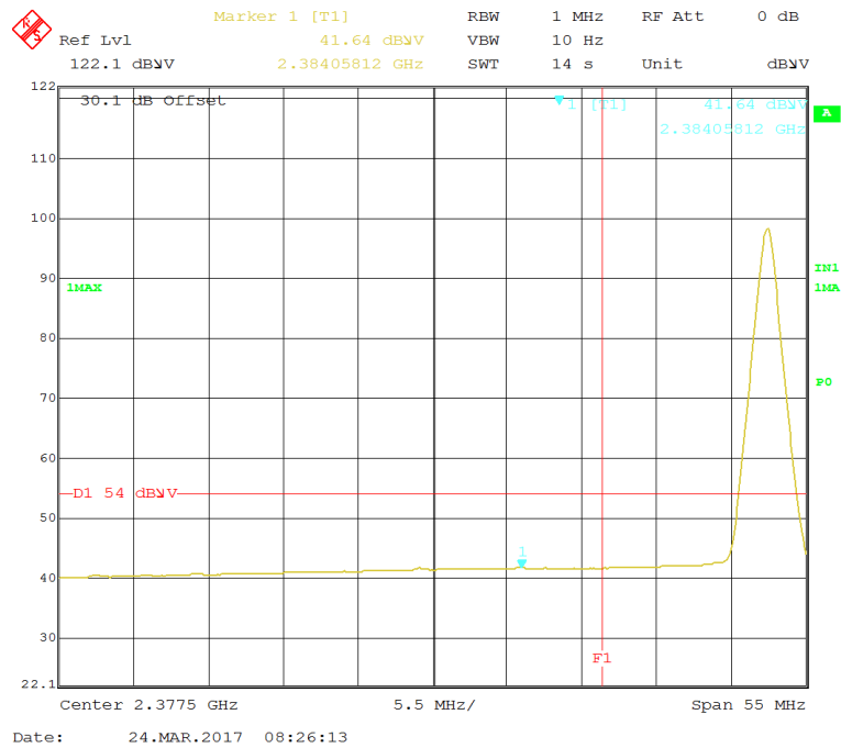
Figure 29: Radiated Bandedge at 2390MHz – BLE – Horz. (Ave)
