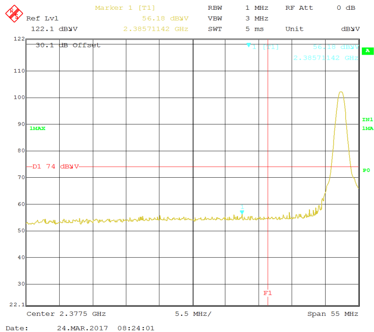
Figure 30: Radiated Bandedge at 2390MHz – BLE – Horz. (Peak)
