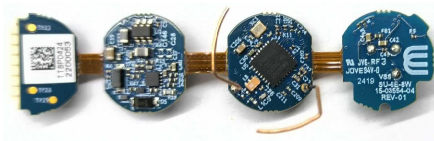
SU-6E-8W and SU-6E-8W-LR Internal Image – Bot
