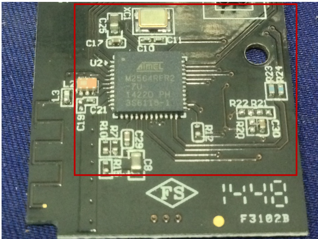
Wireless Module
