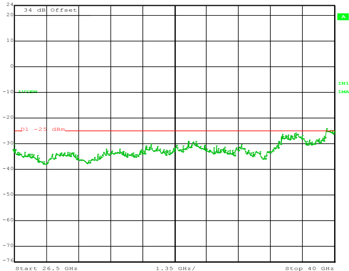
Figure 47 - Spurs 4967.5 MHz – 5 MHz Channel, 26.5 - 40 GHz
