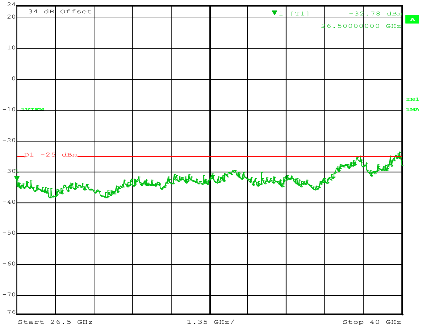
Figure 59 - Spurs 4950 MHz – 20 MHz Channel, 26.5 - 40 GHz
