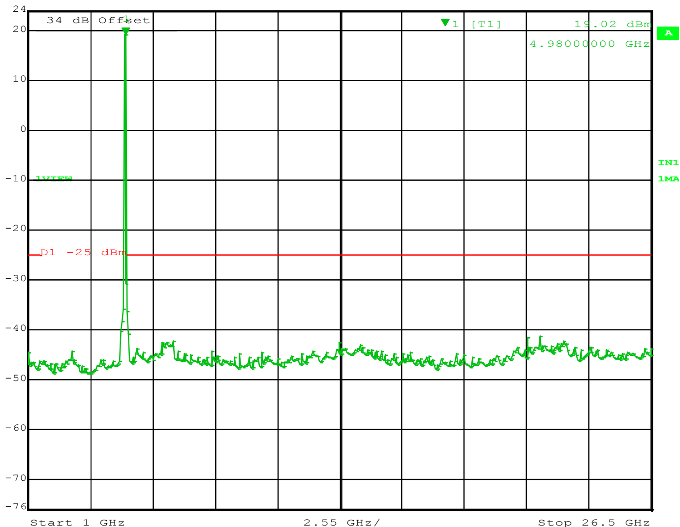
Figure 62 - Spurs 4980 MHz – 20 MHz Channel, 1 - 26.5 GHz
