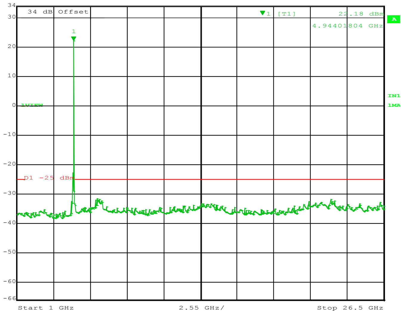
Figure 51 - Spurs 4945 MHz – 10 MHz Channel, 1 - 26.5 GHz
