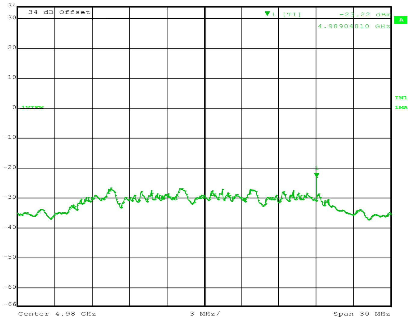
Figure 33: 4980 MHz at 20 MHz BW
