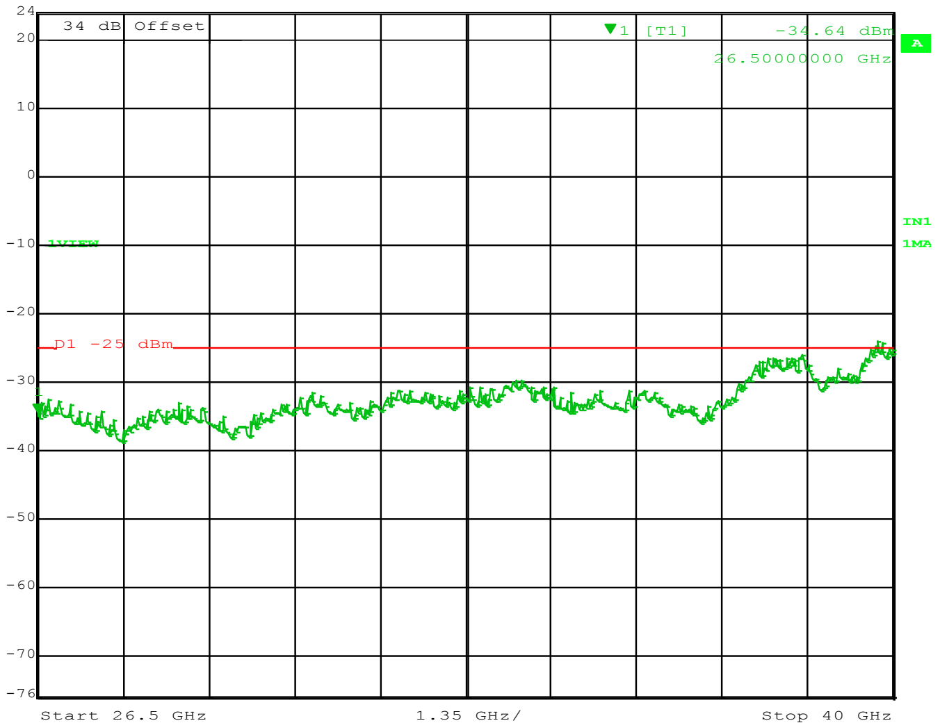
Figure 54 - Spurs 4965 MHz – 10 MHz Channel, 26.5 - 40 GHz
