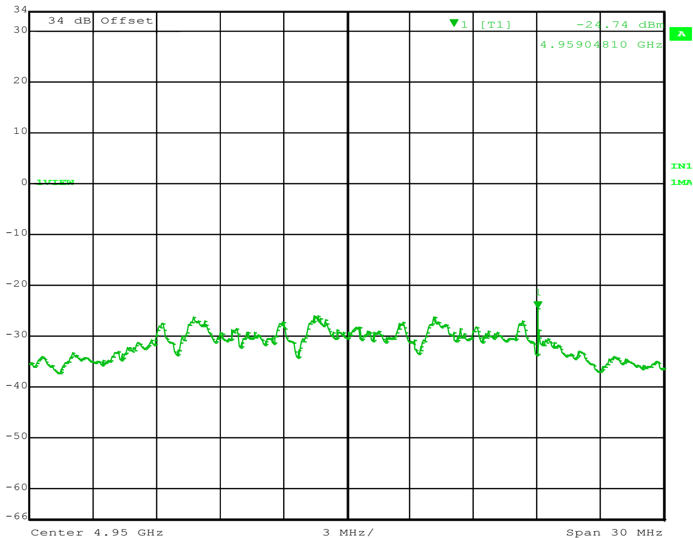
Figure 31: 4950 MHz at 20 MHz BW
