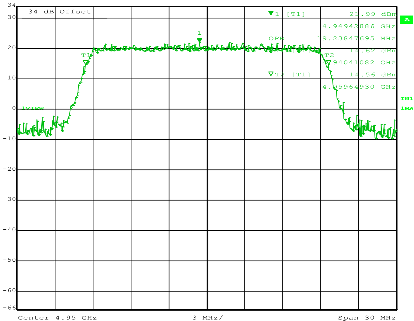
Figure 40: 99% Occupied Bandwidth 4950 MHz - 20 MHz Channel
