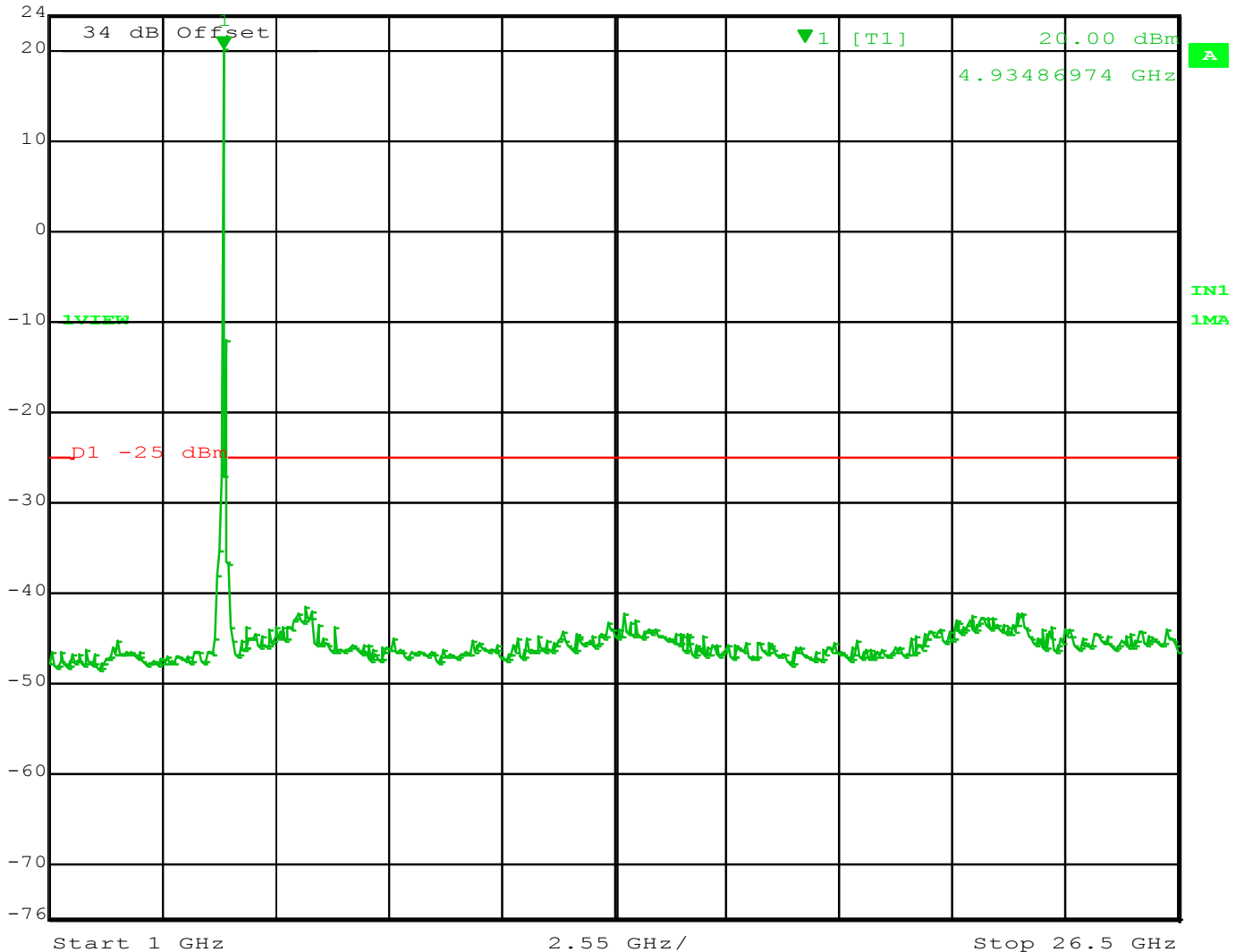
Figure 60 - Spurs 4960 MHz -20 MHz Channel, 1 - 26.5 GHz
