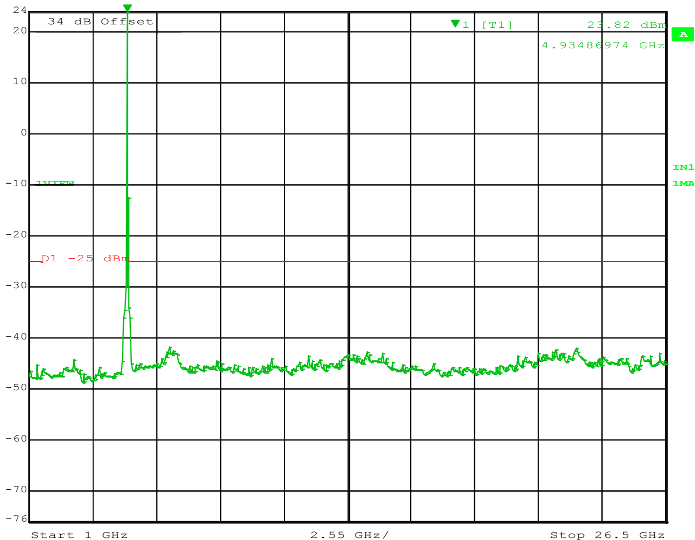
Figure 53 - Spurs 4965 MHz – 10 MHz Channel, 1 - 26.5 GHz
