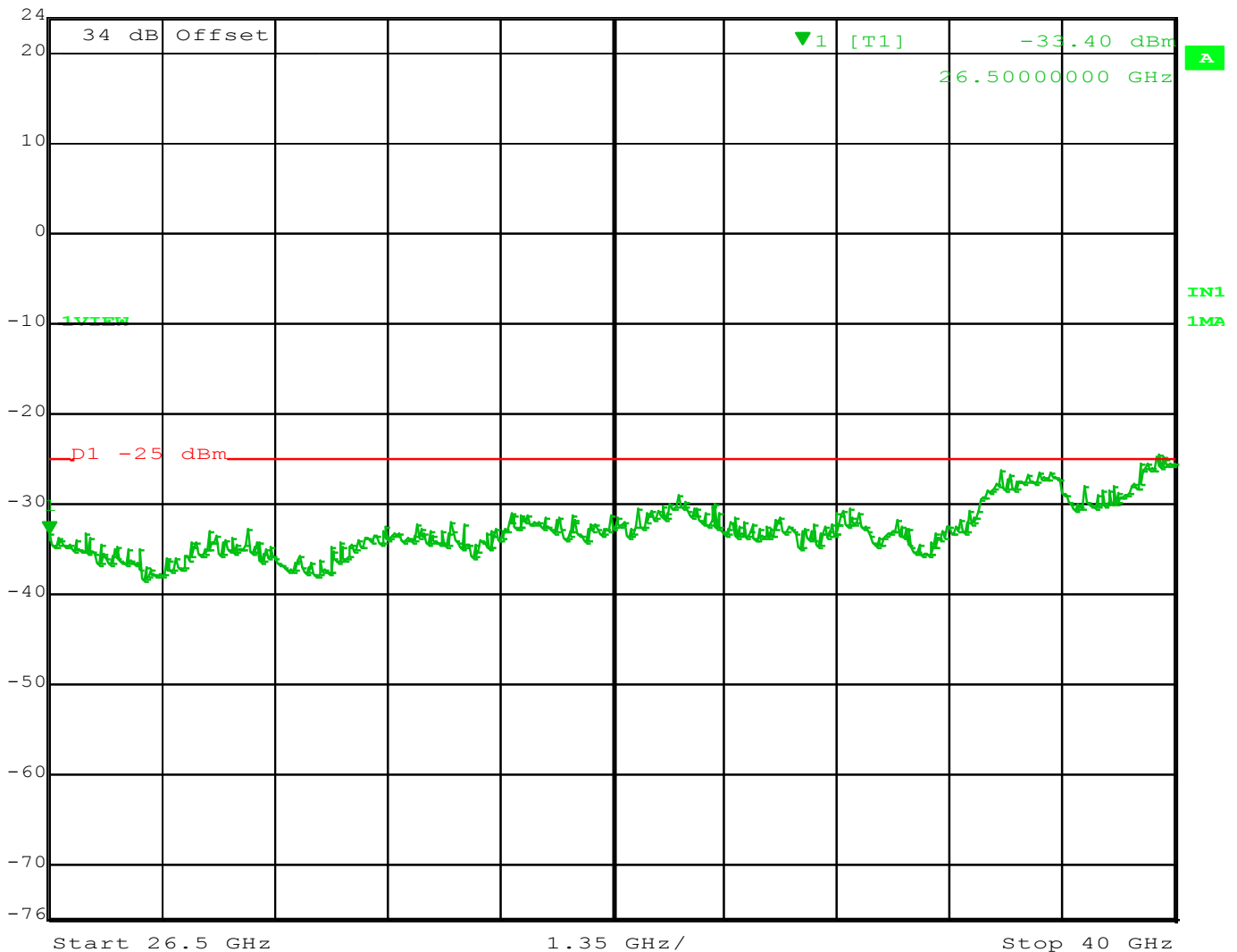
Figure 52 - Spurs 4945 MHz – 10 MHz Channel, 26.5 - 40 GHz
