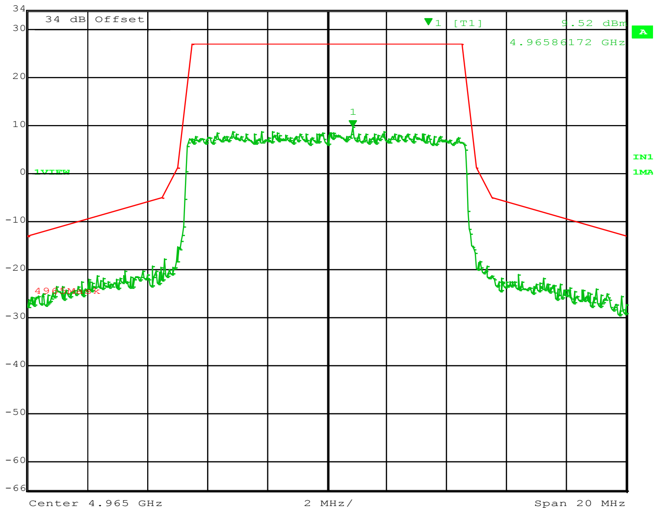
Figure 5 – Center Frequency 4965 MHz - 10 MHz Channel Spacing
