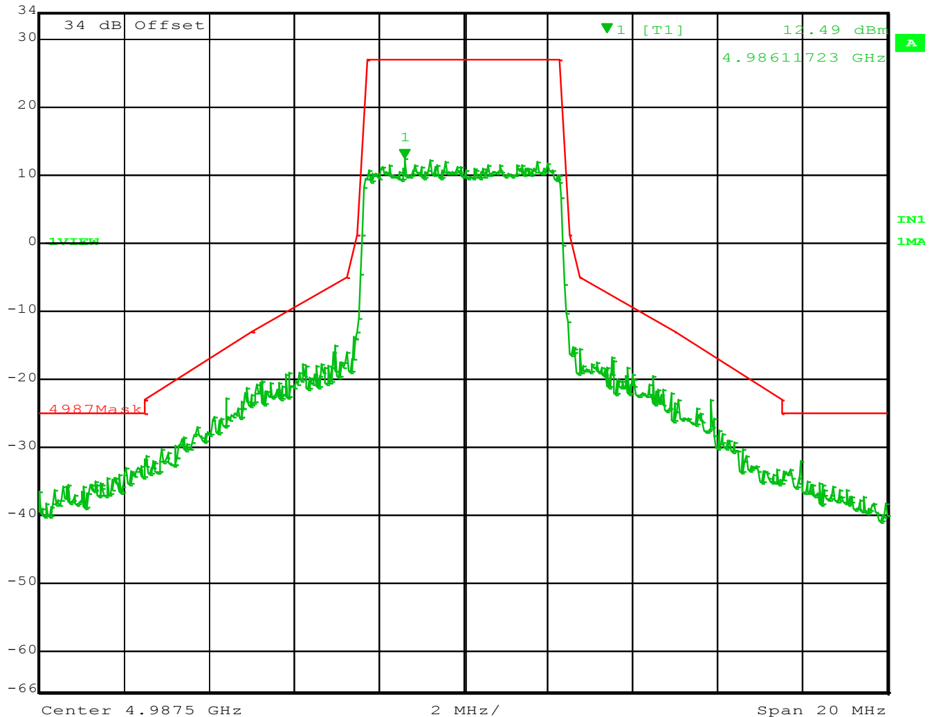
Figure 3 – Center Frequency 4987.5 MHz - 5 MHz Channel Spacing
