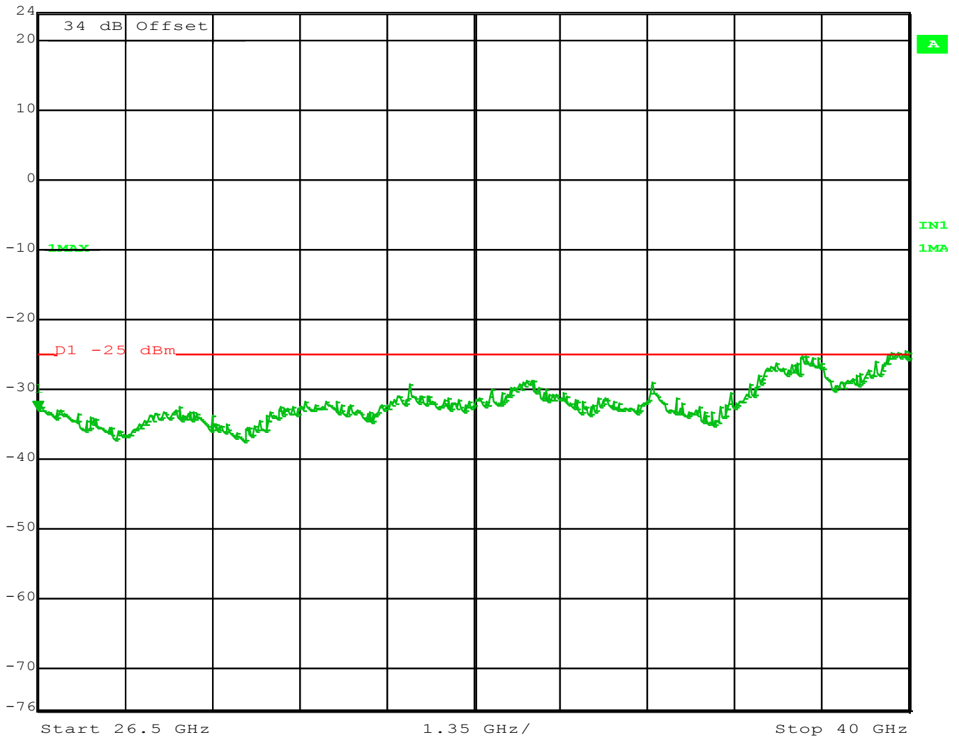
Figure 49 - Spurs 4987.5 MHz – 5 MHz Channel, 26.5 - 40 GHz
