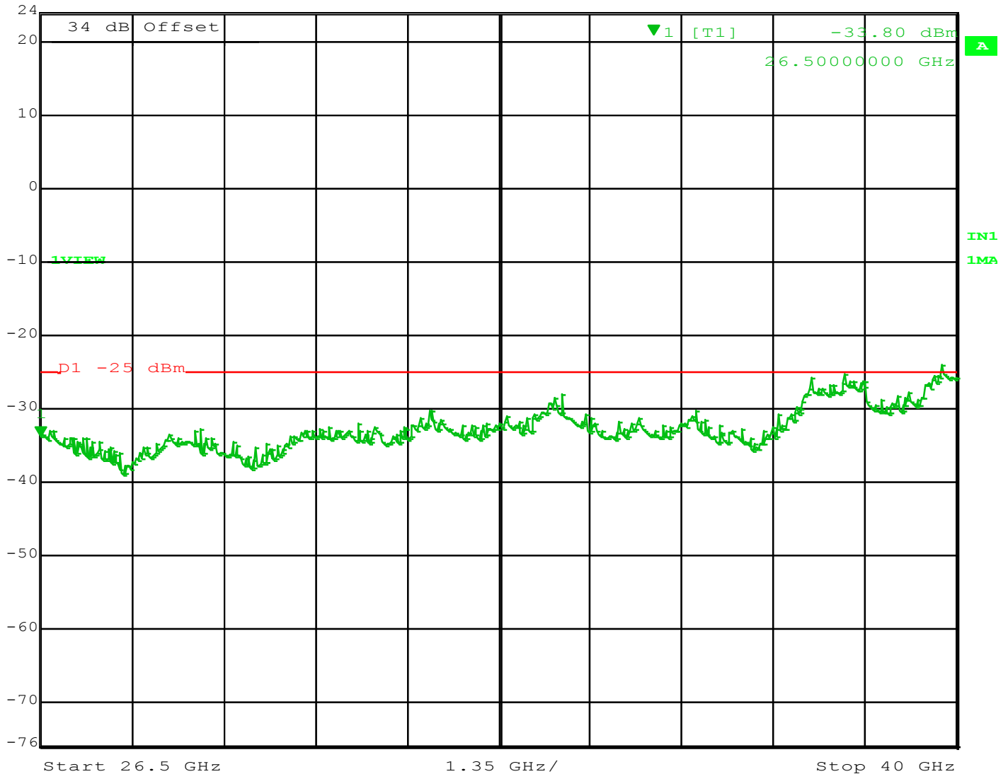
Figure 63 - Spurs 4980 MHz – 20 MHz Channel, 26.5 - 40 GHz
