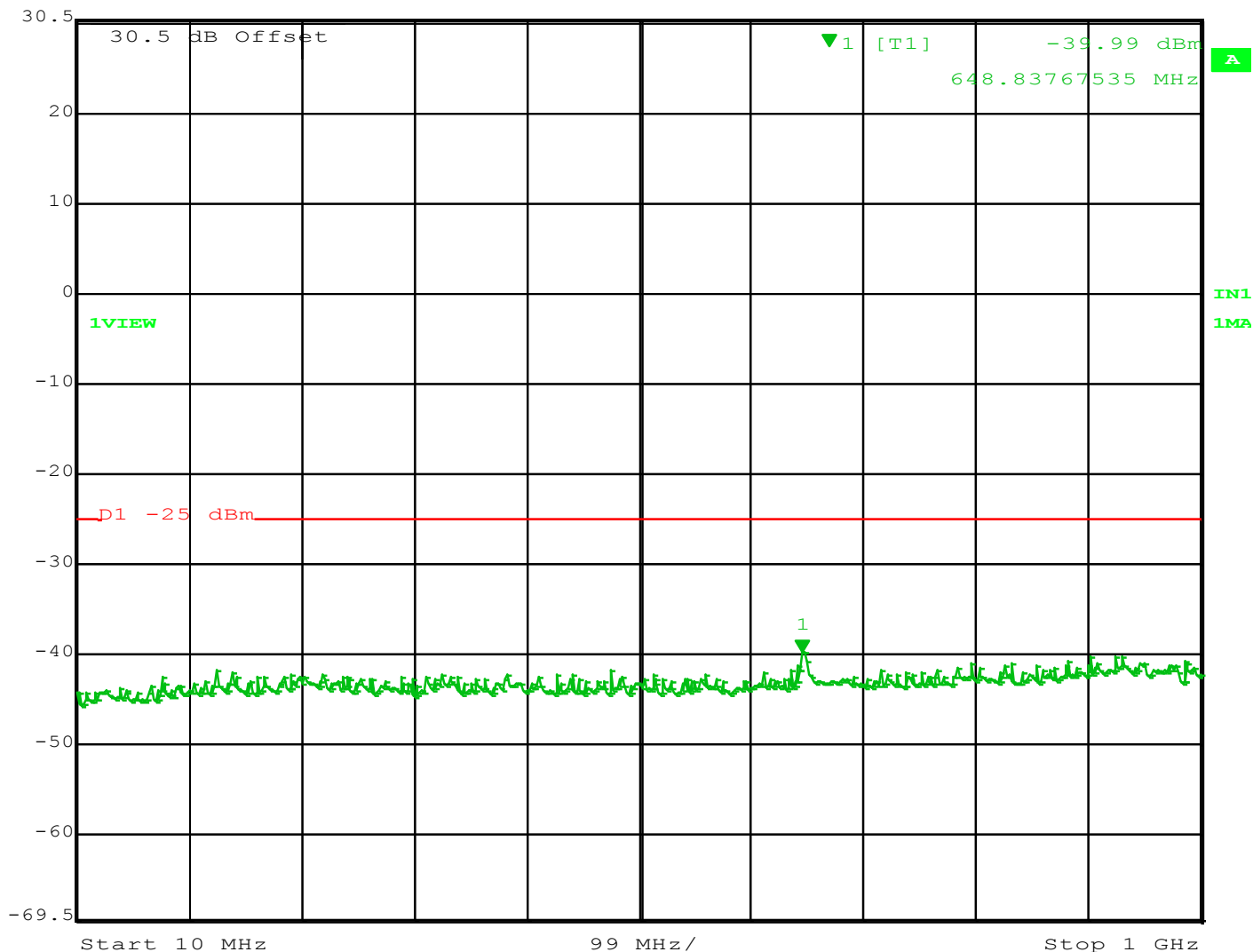
Figure 57 - Spurs 4950 MHz – 20 MHz Channel, 10 MHz - 1 GHz
