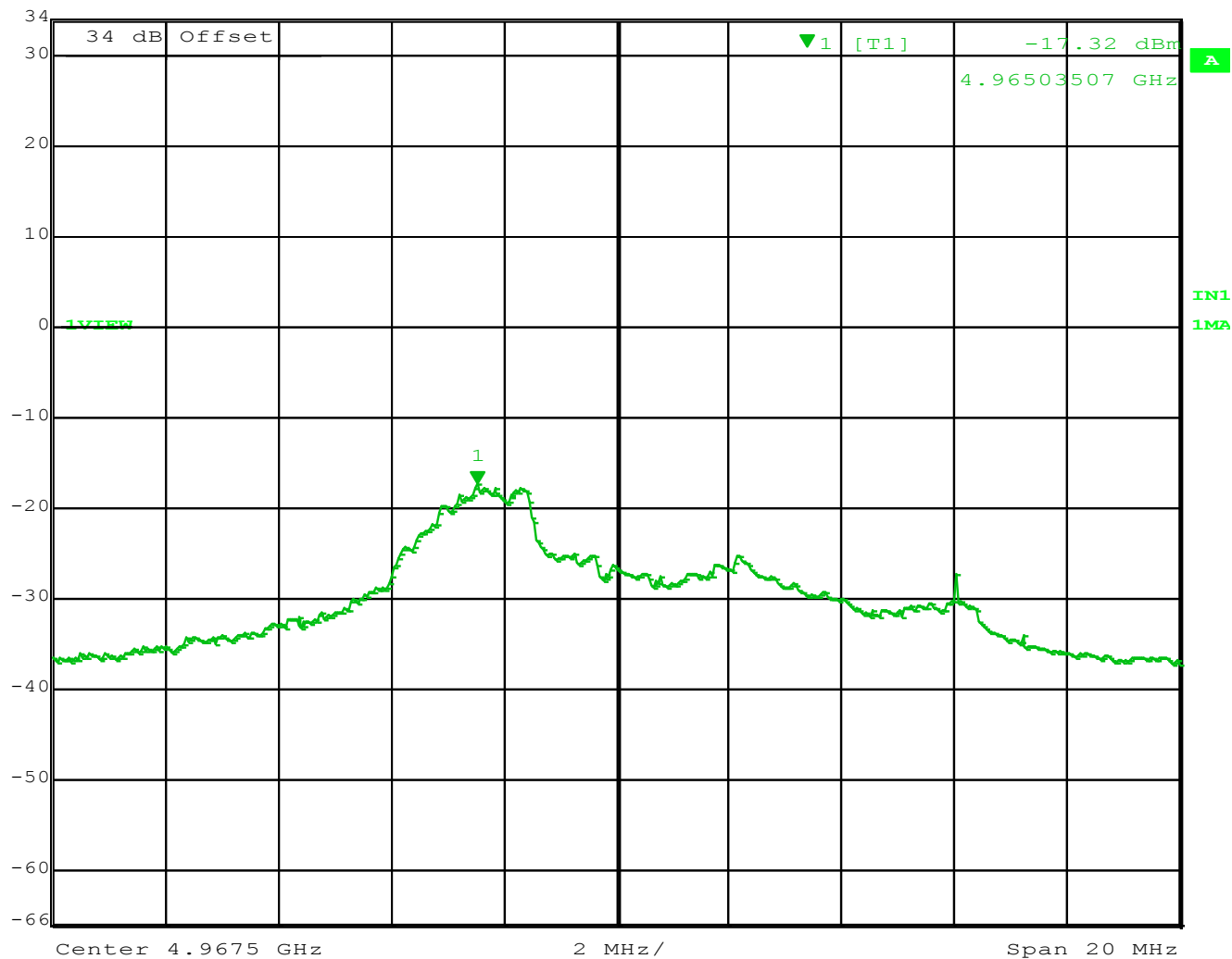
Figure 26: 4967.5 MHz at 5 MHz BW
