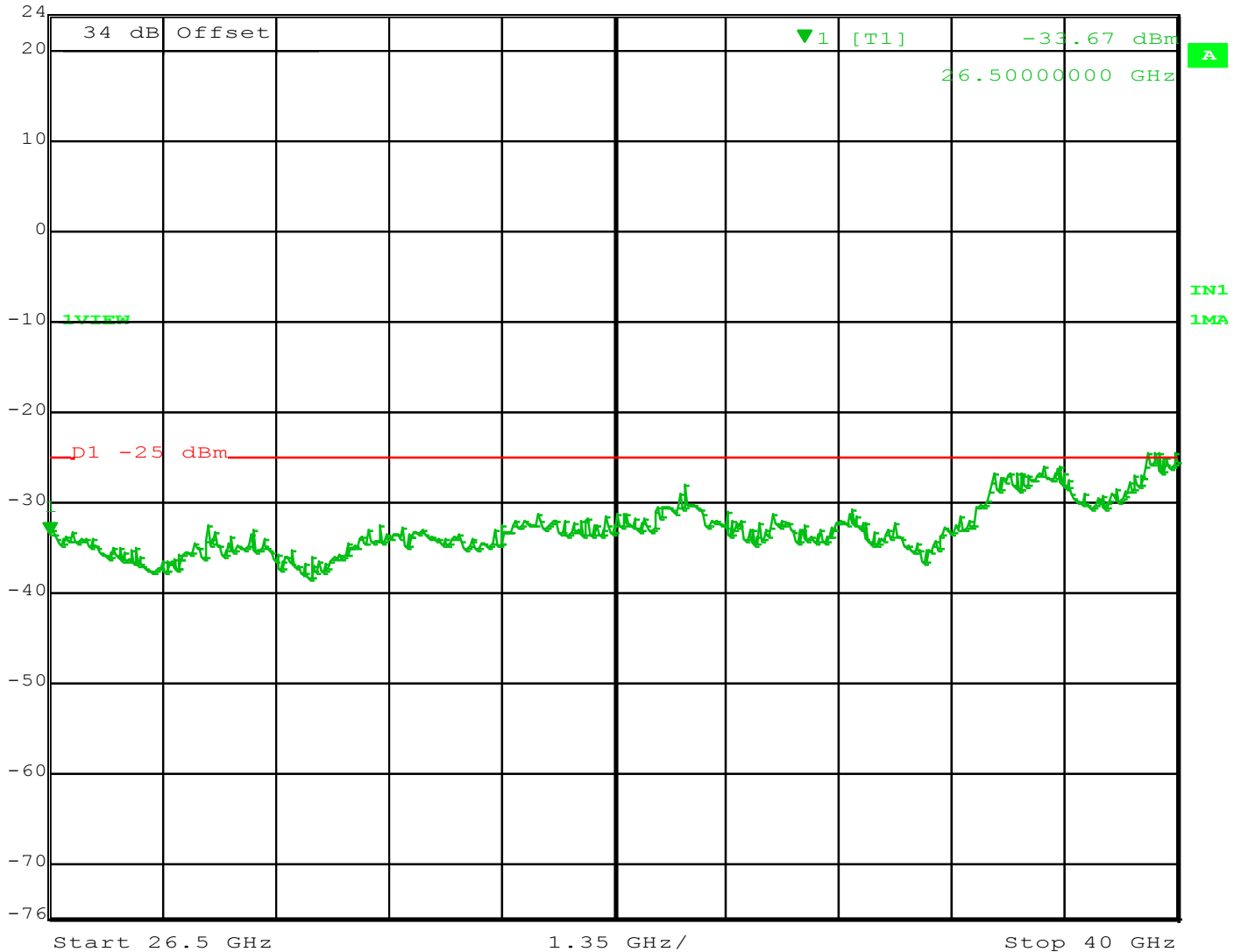
Figure 61 - Spurs 4960 MHz – 20 MHz Channel, 26.5 - 40 GHz
