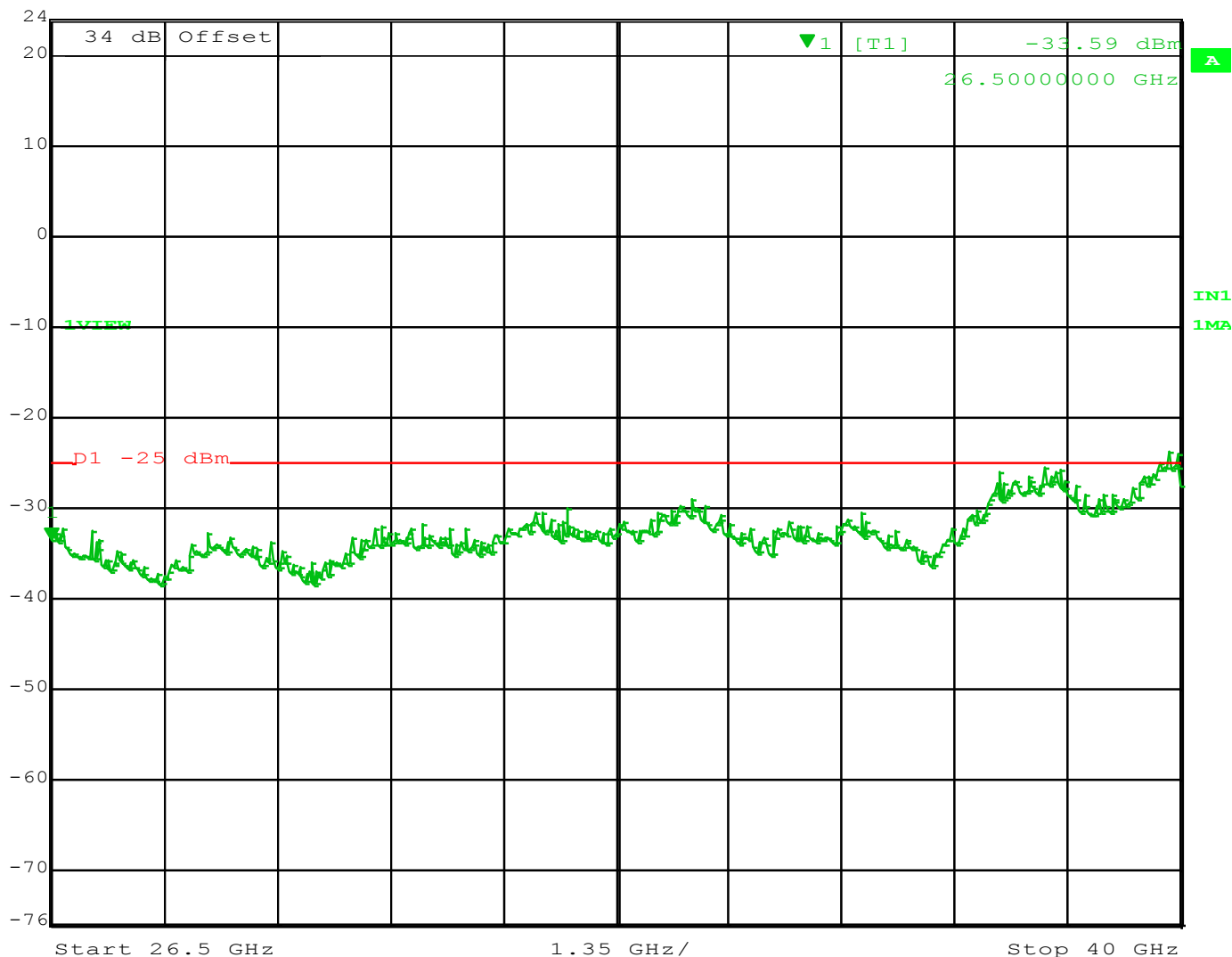
Figure 56 - Spurs 4985 MHz – 10 MHz Channel, 26.5 - 40 GHz
