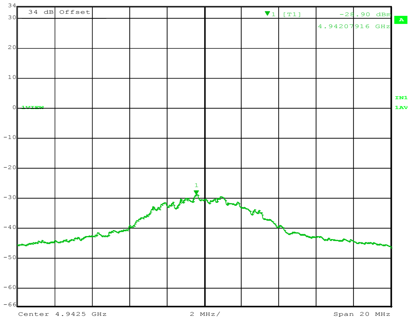
Figure 25: 4942.5 MHz at 5MHz BW
