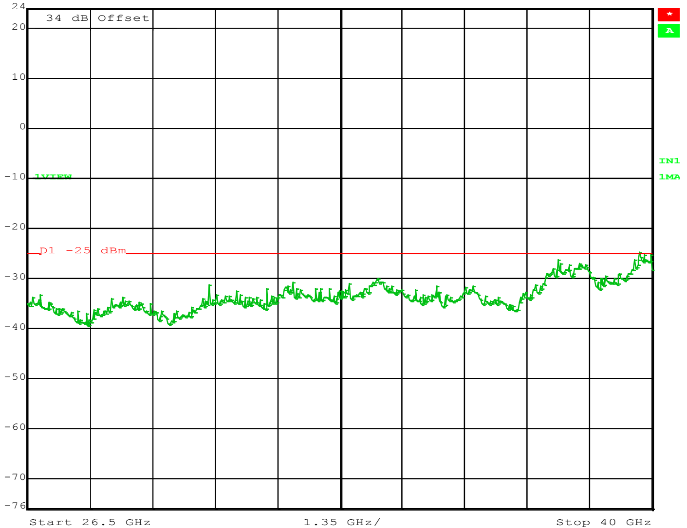
Figure 45 - Spurs 4942.5 MHz – 5 MHz Channel, 26.5 - 40 GHz
