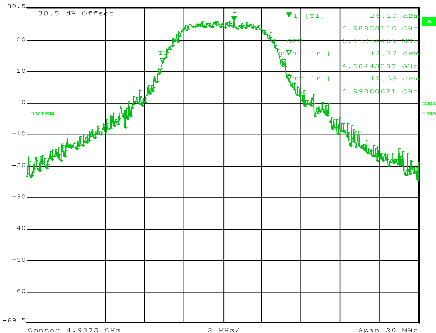
Figure 36: 99% Occupied Bandwidth 4987.5 MHz - 5 MHz Channel
