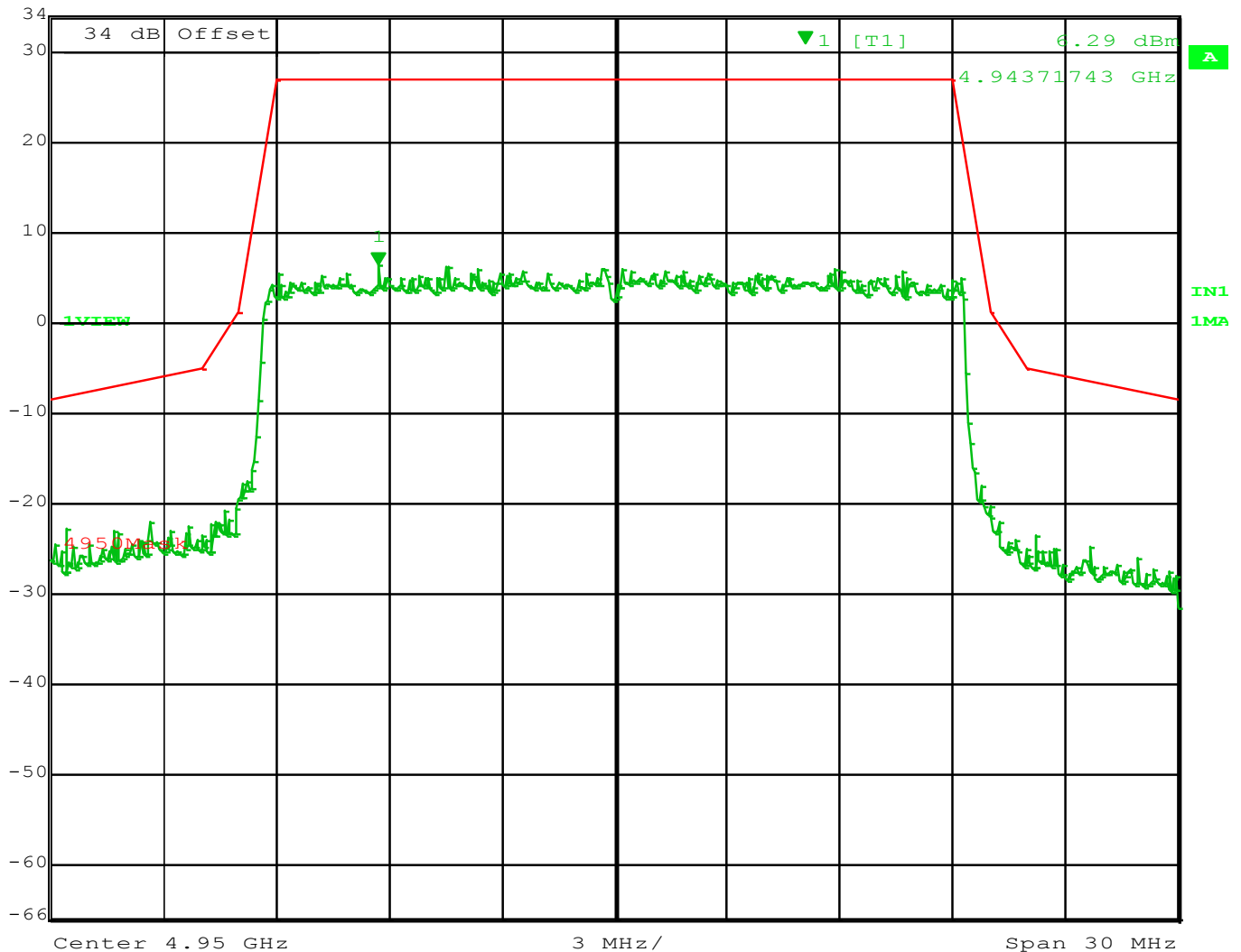
Figure 7 – Center Frequency 4950 MHz - 20 MHz Channel Spacing
