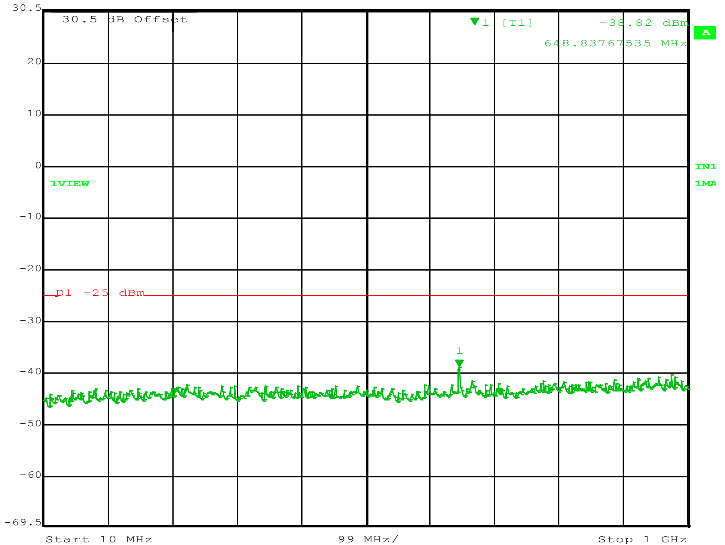
Figure 43 – Spurs 4942.5 MHz – 5 MHz Channel, 10 MHz - 1 GHz
