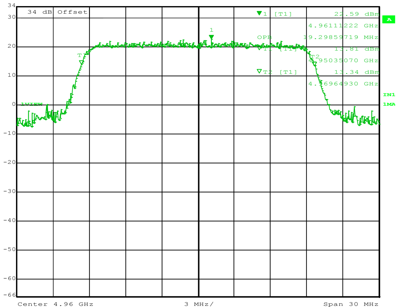
Figure 41: 99% Occupied Bandwidth 4960 MHz - 20 MHz Channel
