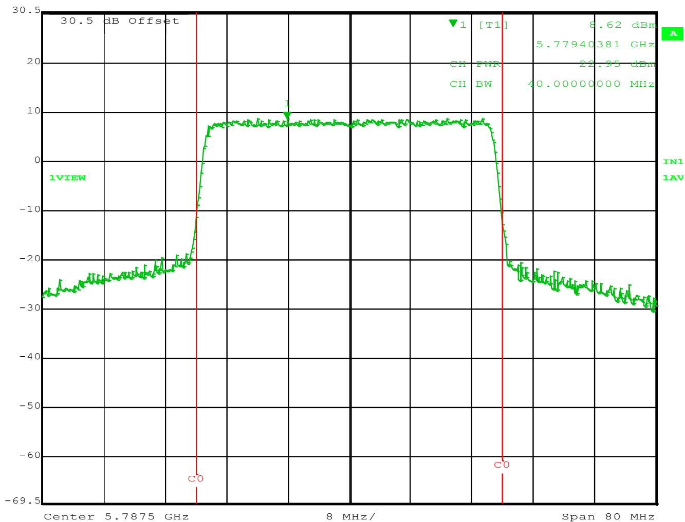
Figure 2 – Highest Peak Conducted Power Output for Mid Channel at 5787.5 MHz using a 40 MHz Bandwidth.
