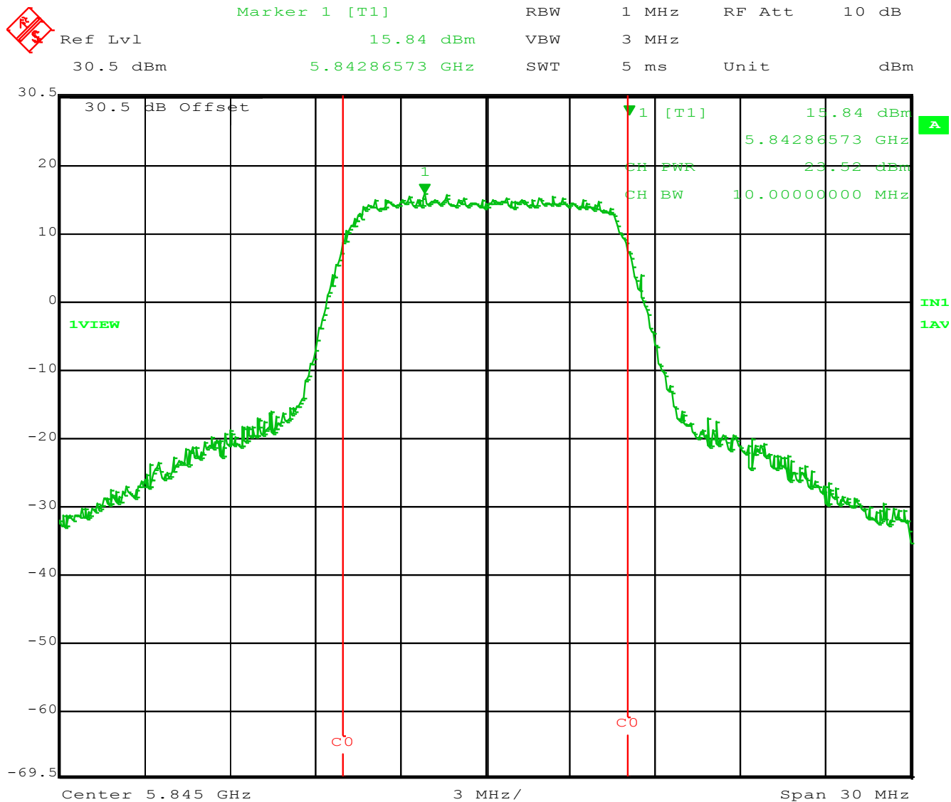
Figure 7 – Highest Peak Conducted Power Output for Highest Channel at 5845 MHz using a 10 MHz Bandwidth.
