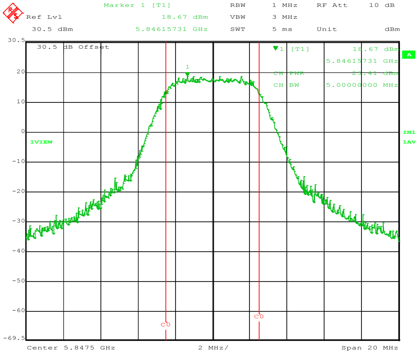
Figure 10 – Highest Peak Conducted Power Output for Highest Channel at 5847.5 MHz using a 5 MHz Bandwidth.
