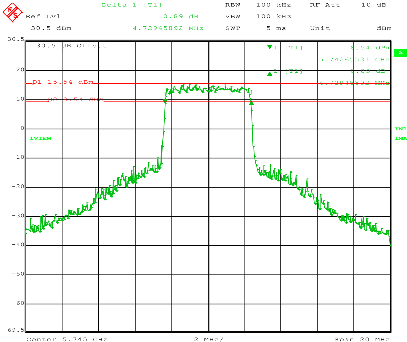
Figure 17: 6dB Occupied Bandwidth 5 MHz Channel at 5745 MHz
