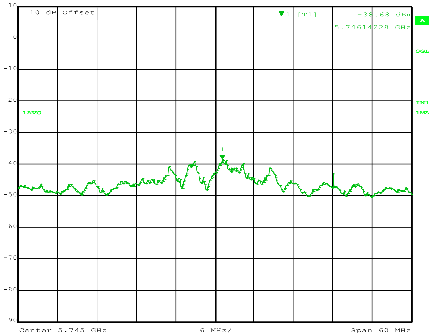
Figure 16: 5745 MHz at 40 MHz BW
