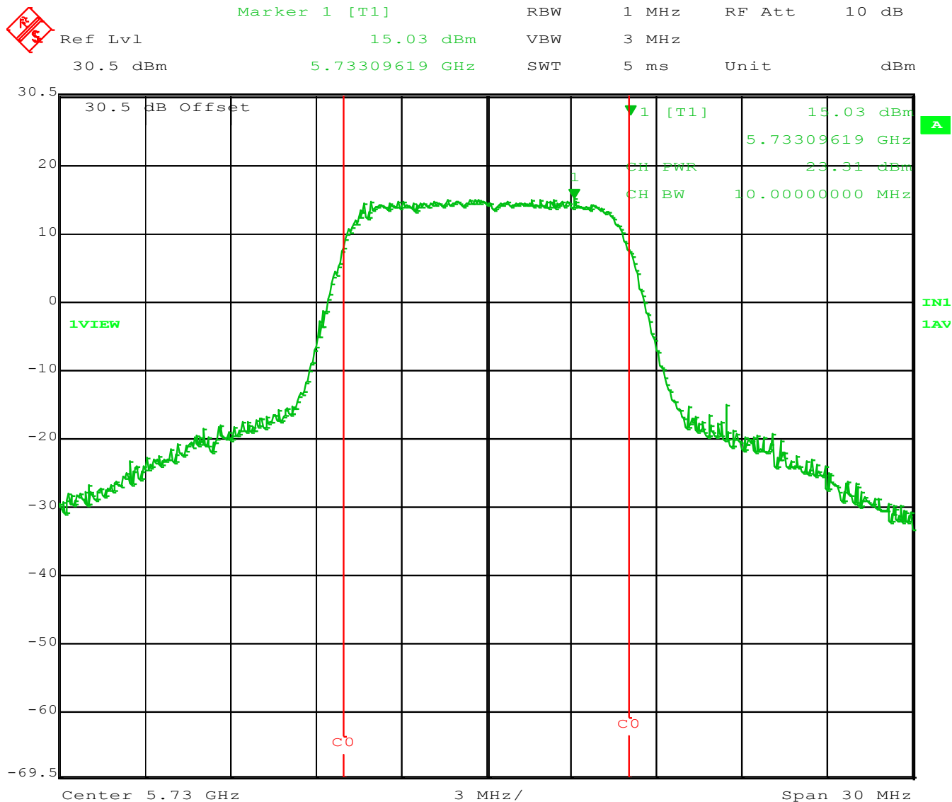
Figure 9 – Highest Peak Conducted Power Output for Lowest Channel at 5730 MHz using a 10 MHz Bandwidth.
