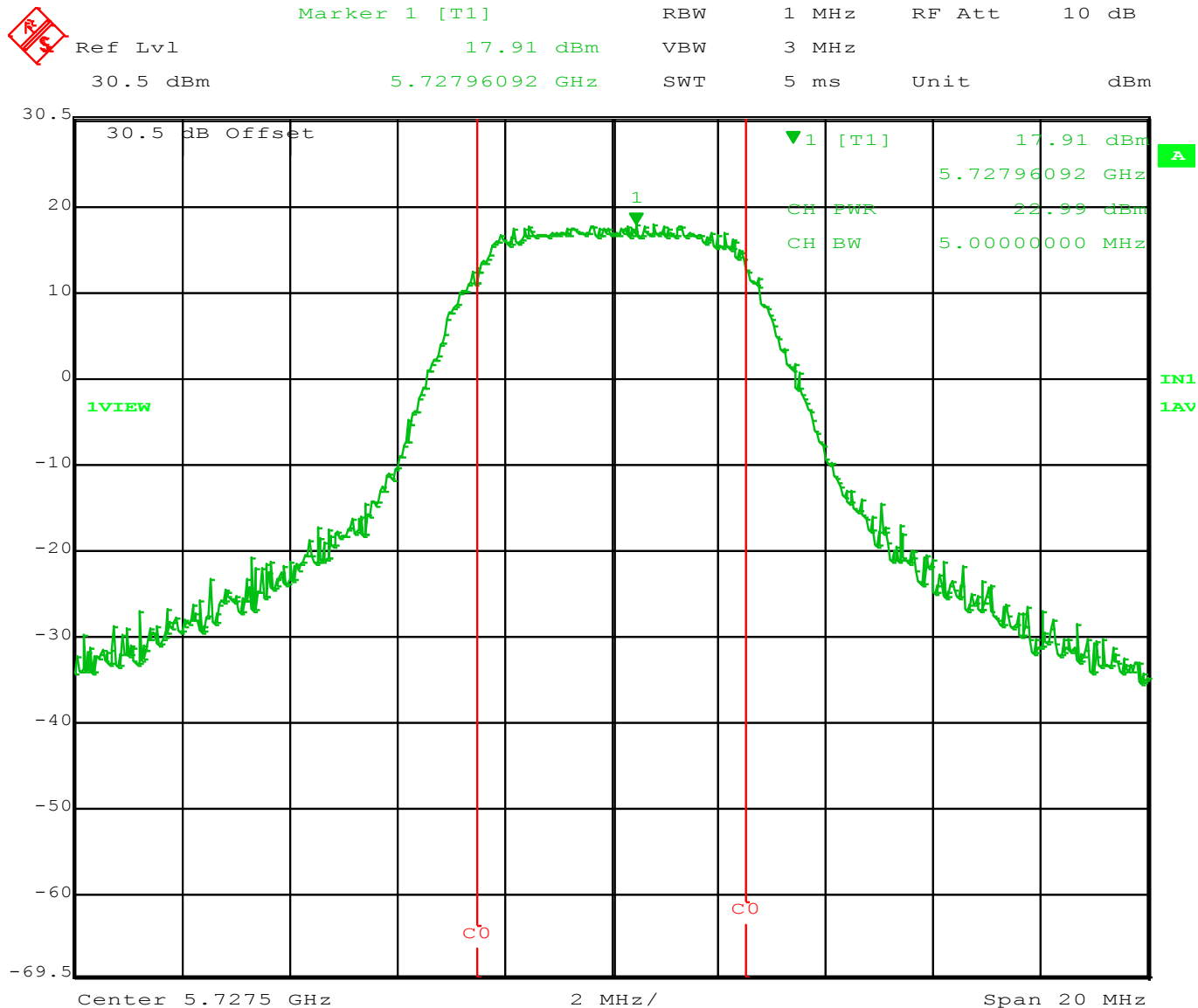
Figure 12 – Highest Peak Conducted Power Output for Lowest Channel at 5727.5 MHz using a 5 MHz Bandwidth.
