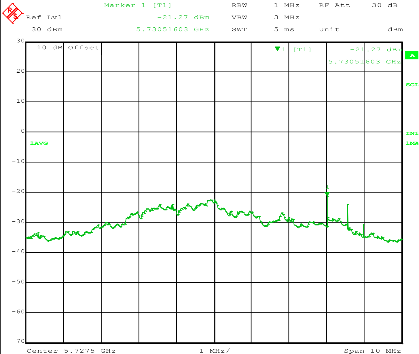
Figure 13: 5727.5 MHz at 5MHz BW
