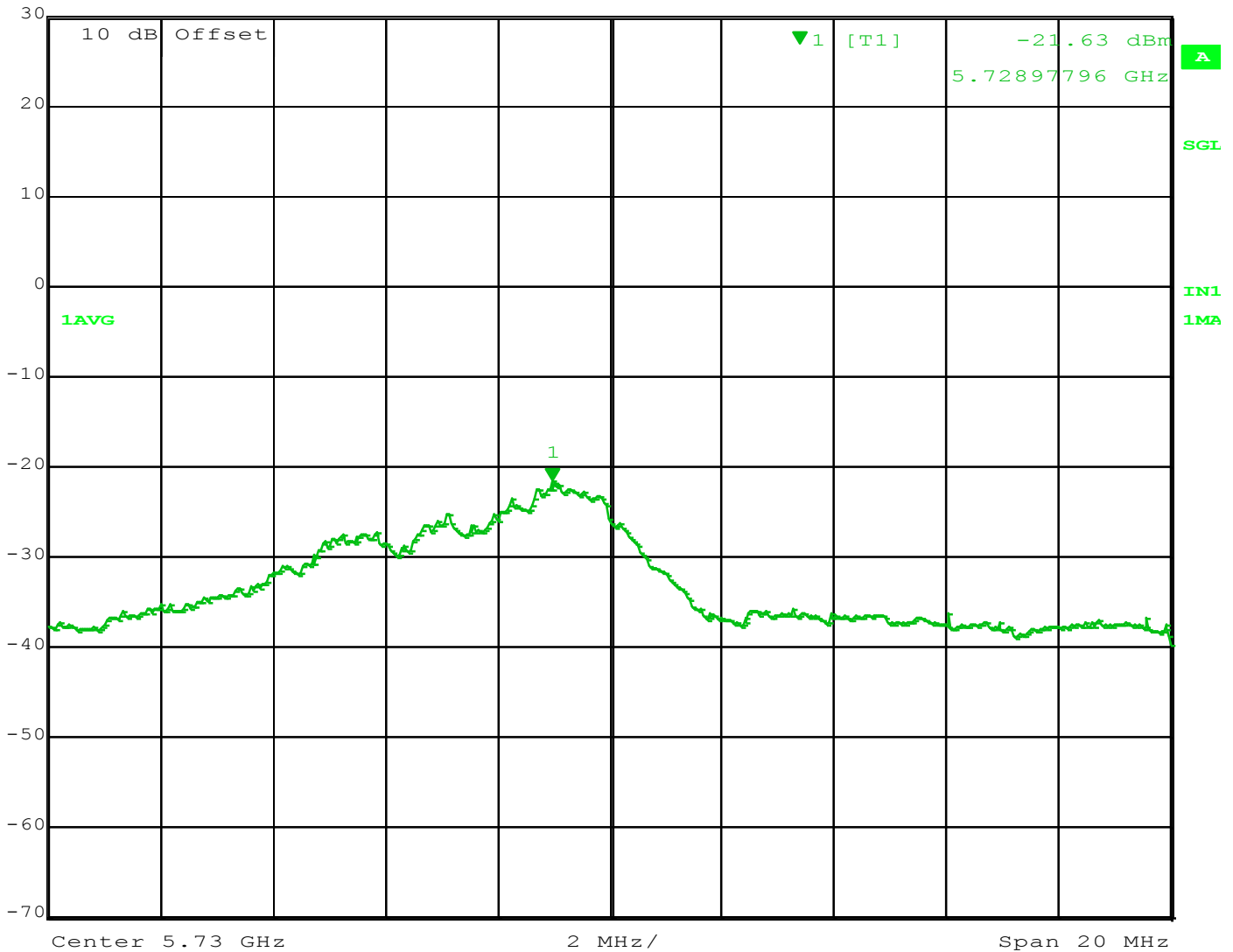
Figure 14: 5730 MHz at 10 MHz BW
