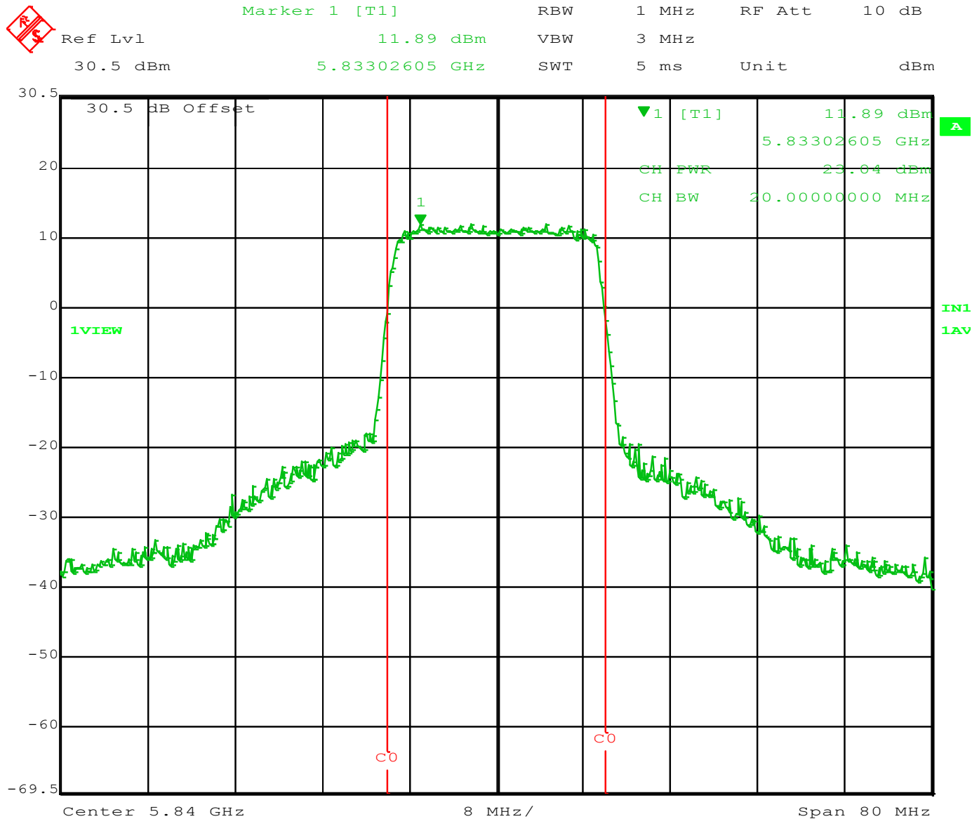
Figure 4 – Highest Peak Conducted Power Output for Highest Channel at 5840 MHz using a 20 MHz Bandwidth.
