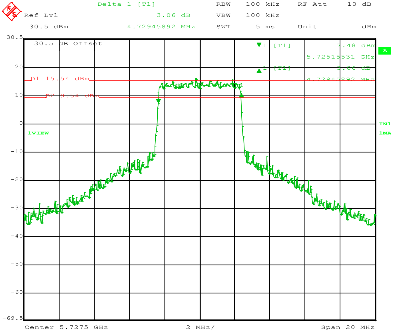
Figure 18: 6dB Occupied Bandwidth 5 MHz Channel at 5727.5 MHz
