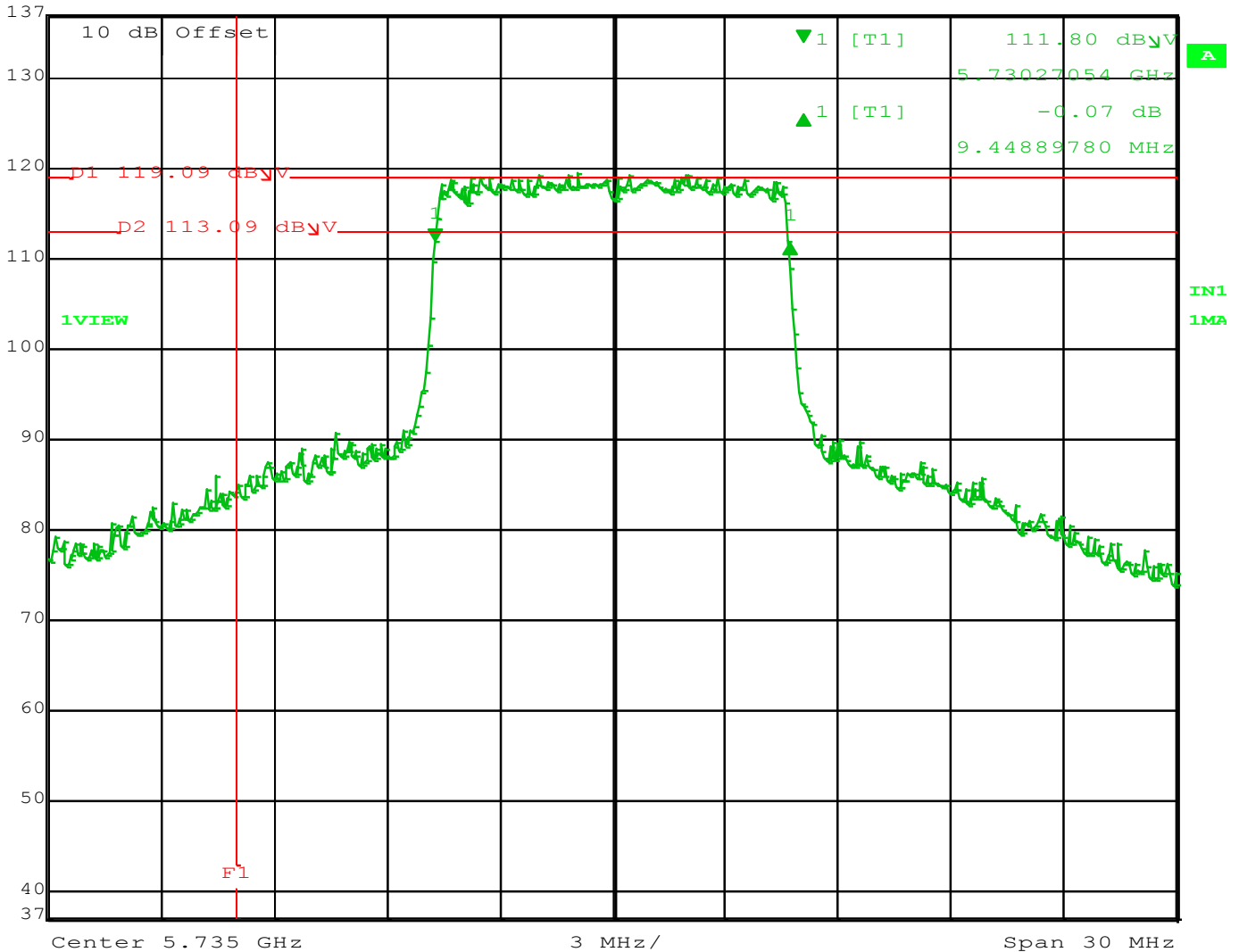
Figure 21: 6dB Occupied Bandwidth 10 MHz Channel at 5735 MHz
