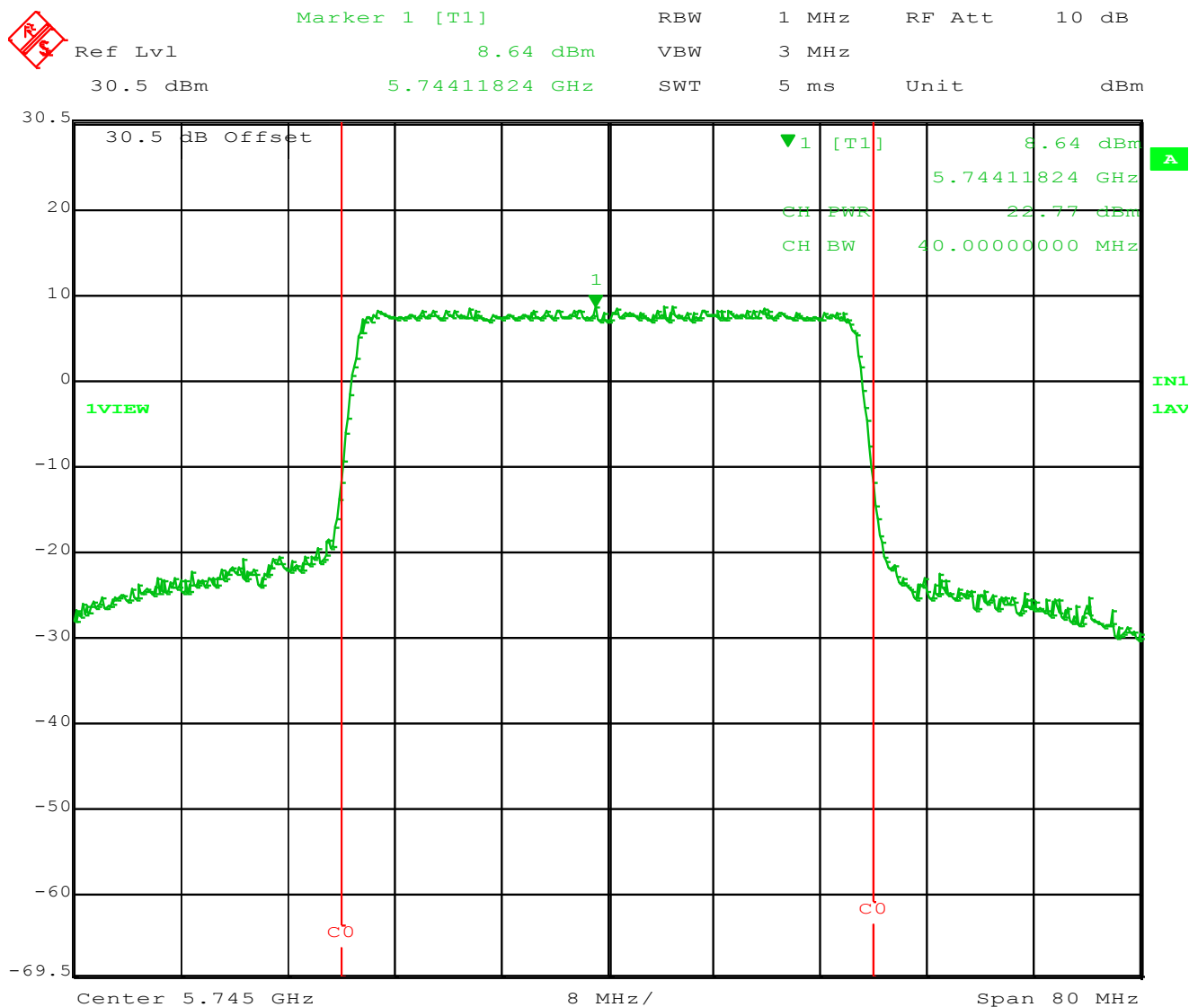
Figure 1 – Highest Peak Conducted Power Output for Lowest Channel at 5745 MHz using a 40 MHz Bandwidth.
