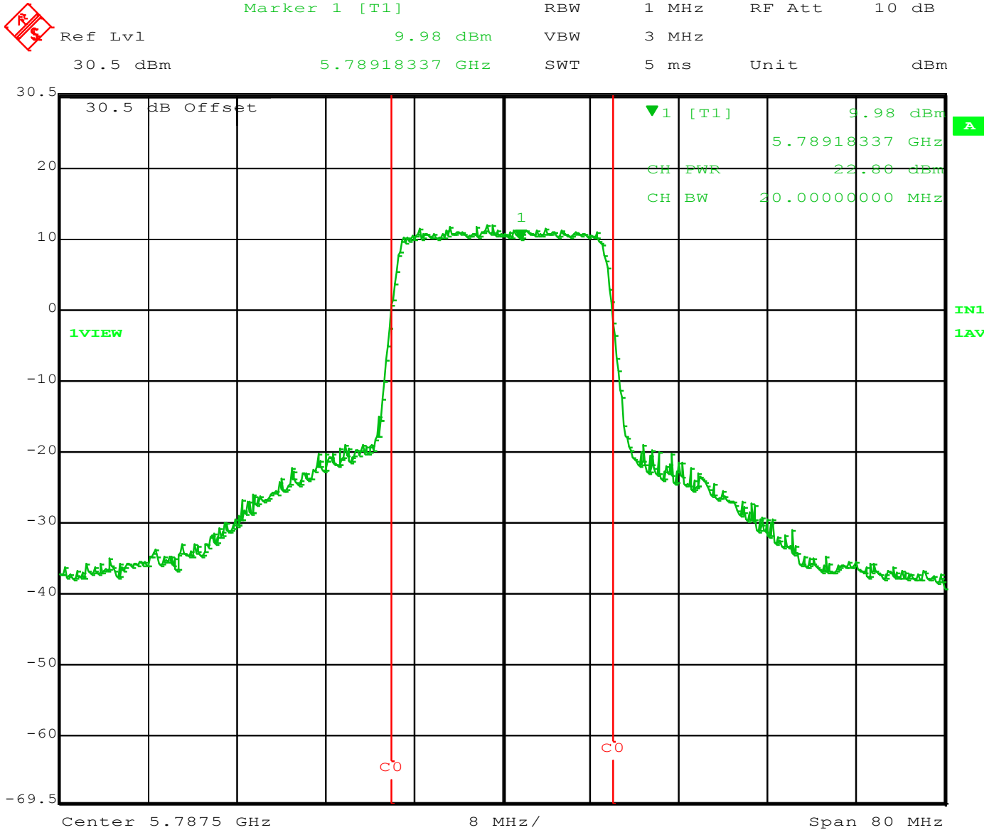
Figure 5 – Highest Peak Conducted Power Output for Mid Channel at 5787.5 MHz using a 20 MHz Bandwidth.
