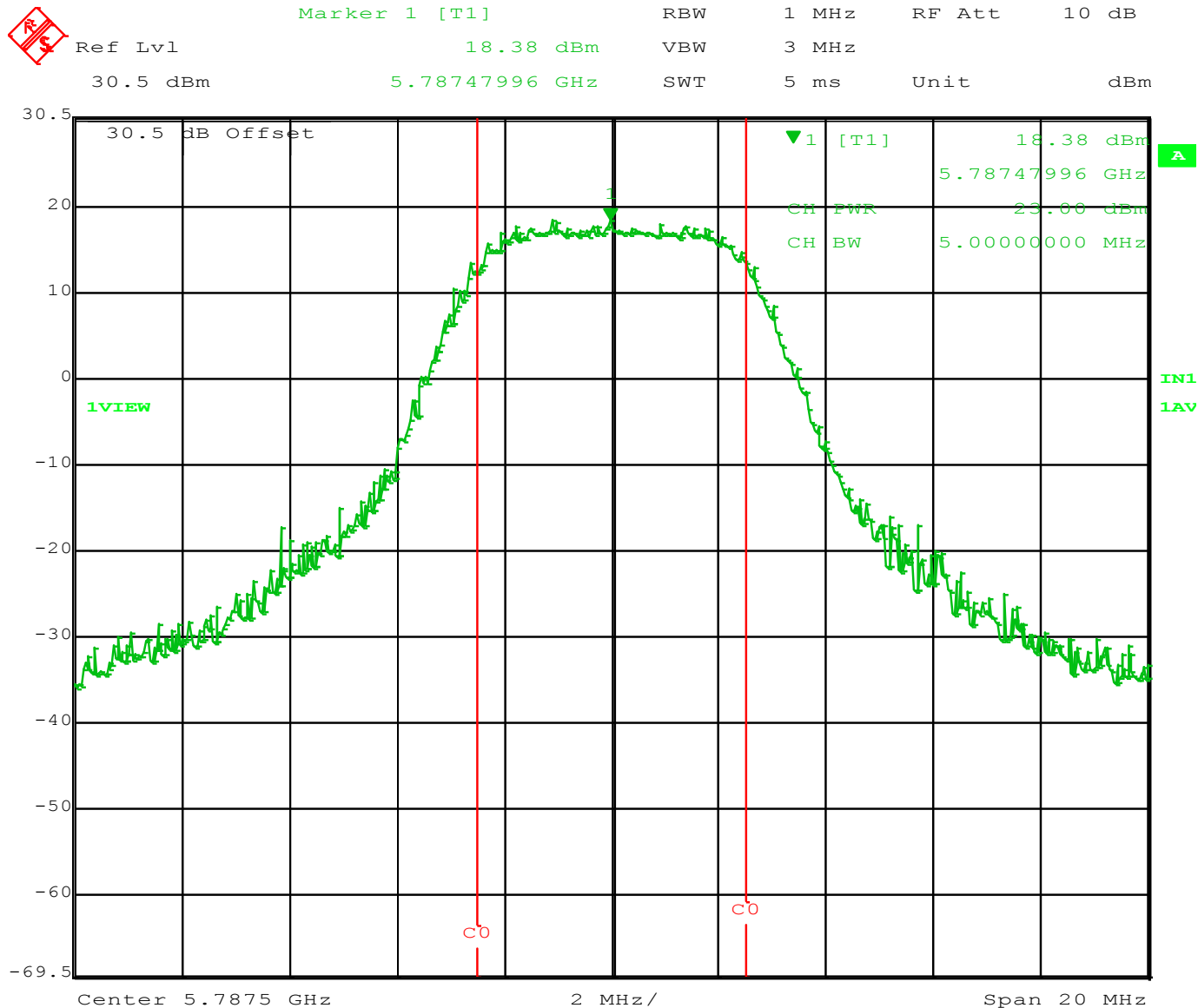
Figure 11 – Highest Peak Conducted Power Output for Highest Channel at 5787.5 MHz using a 5 MHz Bandwidth.
