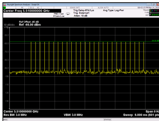
Plot 24. Radar Waveform Calibration, 5510 MHz, 40 MHz, Channel Radar Type 2
