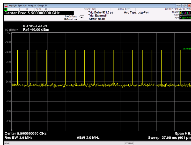
Plot 15. Radar Waveform Calibration, 5500 MHz, 20 MHz, Channel Radar Type 0
