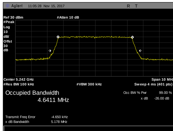
Plot 27. 26 dB Occupied Bandwidth, 5M, 5242.5, 3'Para, rf2
