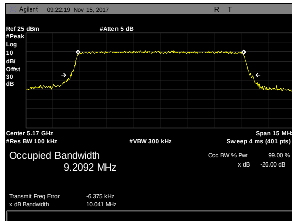
Plot 52. 26 dB Occupied Bandwidth, 10M, 5170, Omni8, rf2
