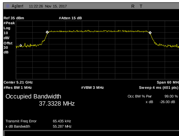
Plot 11. 26 dB Occupied Bandwidth, 40M, 5210, 1'Panel, rf2
