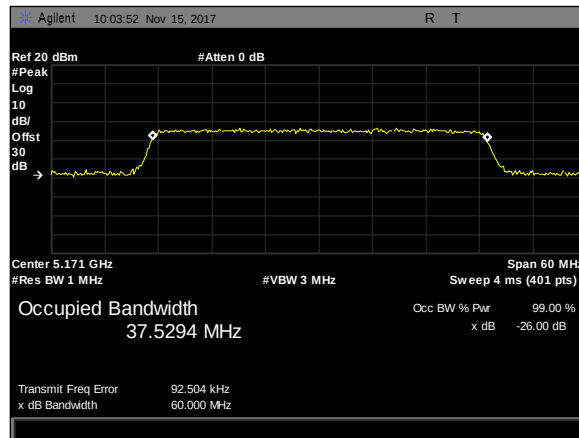
Plot 34. 26 dB Occupied Bandwidth, 40M, 5170, 3'Para, rf2
