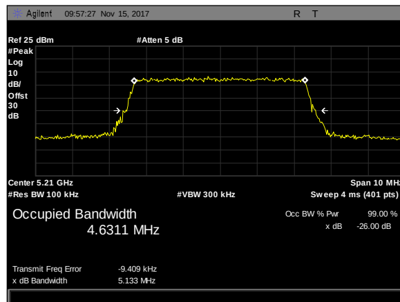
Plot 26. 26 dB Occupied Bandwidth, 5M, 5210, 3'Para, rf2
