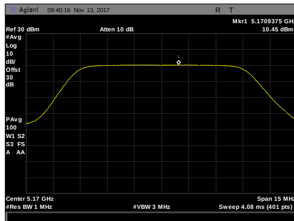
Plot 298. Maximum Power Spectral Density, 10M, 5170, 50Omni, rf2
