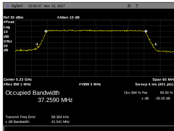
Plot 36. 26 dB Occupied Bandwidth, 40M, 5230, 3'Para, rf2
