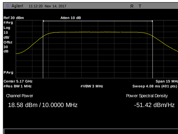
Plot 153. Maximum Conducted Output Power, 10M, 5170, 50mni, rf2
