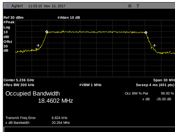
Plot 21. 26 dB Occupied Bandwidth, 20M, 5235.5, 2'Panel, rf2
