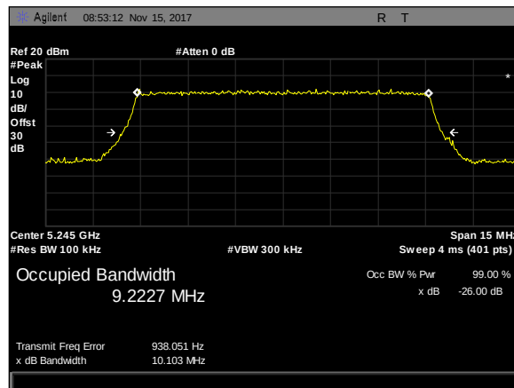
Plot 42. 26 dB Occupied Bandwidth, 10M, 5245, 90Sector, rf2
