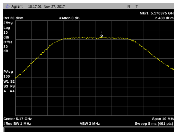
Plot 220. Maximum Power Spectral Density, 5M, 5170, 1Panel, rf2
