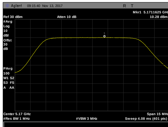
Plot 297. Maximum Power Spectral Density, 10M, 5170, 50Omni, rf1
