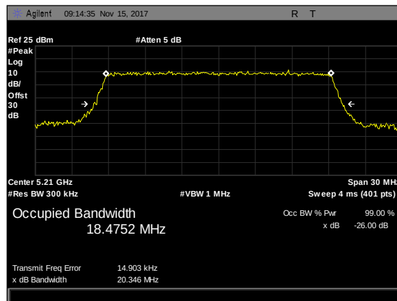
Plot 44. 26 dB Occupied Bandwidth, 20M, 5210, 90Sector, rf2
