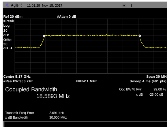
Plot 19. 26 dB Occupied Bandwidth, 20M, 5170, 2'Panel, rf2
