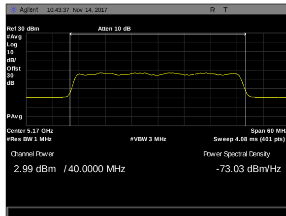
Plot 164. Maximum Conducted Output Power, 40M, 5170, 50mni, rf1
