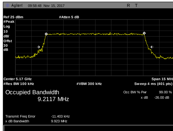
Plot 28. 26 dB Occupied Bandwidth, 10M, 5170, 3'Para, rf2
