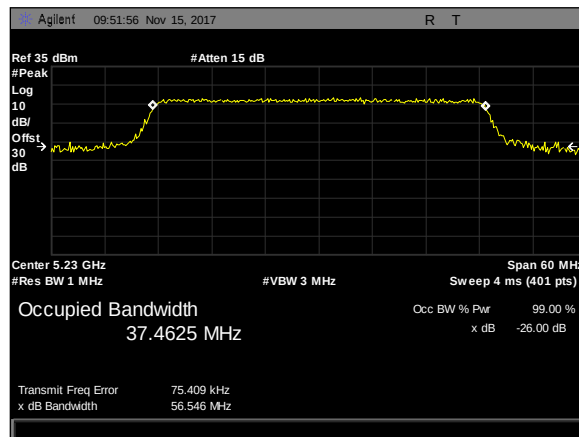
Plot 72. 26 dB Occupied Bandwidth, 40M, 5230, 50Omni, rf2
