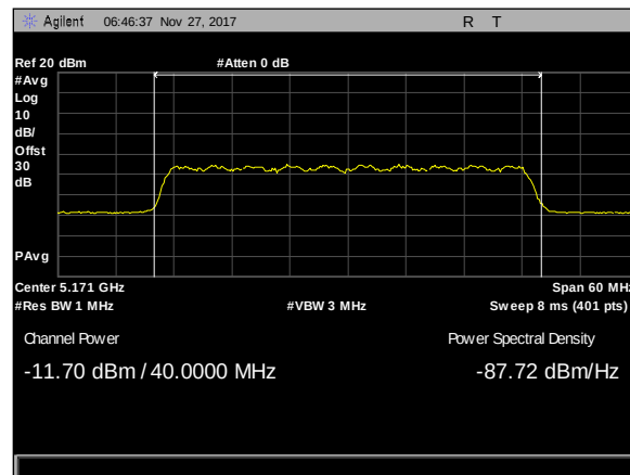
Plot 92. Maximum Conducted Output Power, 40M, 5171, 1Panel, rf1
