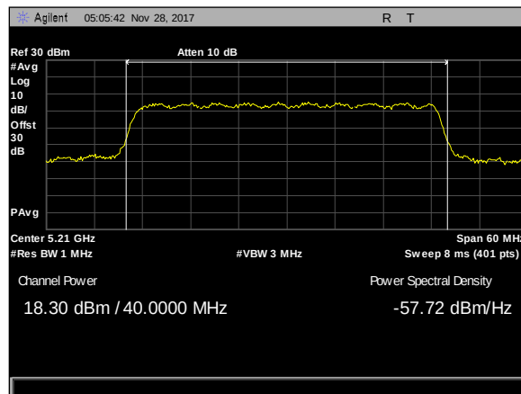
Plot 167. Maximum Conducted Output Power, 40M, 5210, 50mni, rf2
