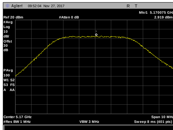
Plot 219. Maximum Power Spectral Density, 5M, 5170, 1Panel, rf1
