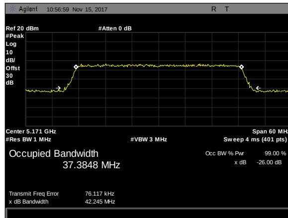
Plot 22. 26 dB Occupied Bandwidth, 40M, 5171, 2'Panel, rf2
