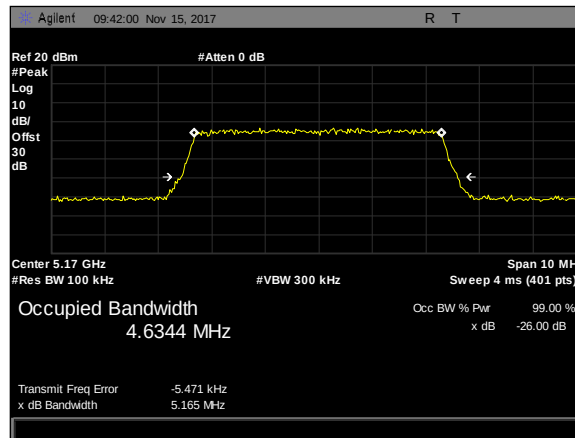
Plot 61. 26 dB Occupied Bandwidth, 5M, 5170, 50mni, rf2
