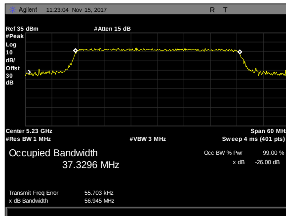
Plot 12. 26 dB Occupied Bandwidth, 40M, 5230, 1'Panel, rf2
