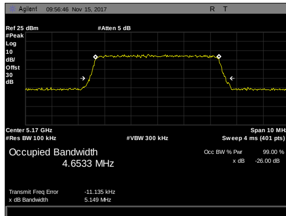
Plot 25. 26 dB Occupied Bandwidth, 5M, 5170, 3'Para, rf2
