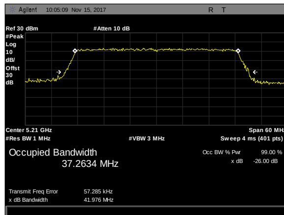
Plot 35. 26 dB Occupied Bandwidth, 40M, 5210, 3'Para, rf2
