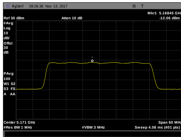
Plot 309. Maximum Power Spectral Density, 40M, 5170, 50mni, rf1
