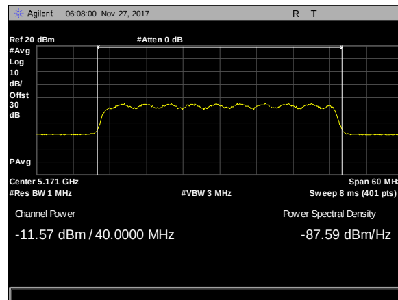
Plot 116. Maximum Conducted Output Power, 40M, 5171, 2Panel, rf1
