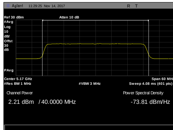
Plot 165. Maximum Conducted Output Power, 40M, 5170, 50mni, rf2
