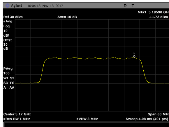
Plot 310. Maximum Power Spectral Density, 40M, 5170, 50mni, rf2
