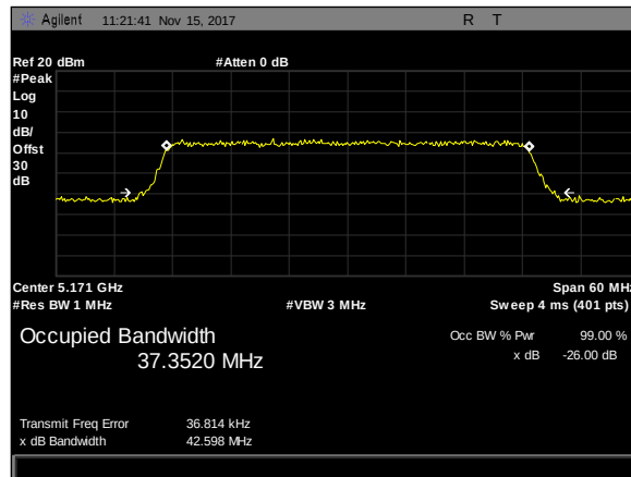
Plot 10. 26 dB Occupied Bandwidth, 40M, 5171, 1'Panel, rf2
