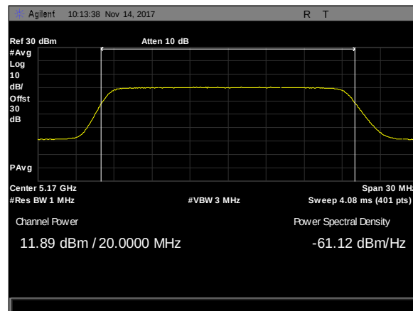
Plot 158. Maximum Conducted Output Power, 20M, 5170, 50mni, rf1
