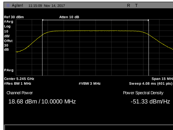
Plot 157. Maximum Conducted Output Power, 10M, 5245, 50mni, rf2
