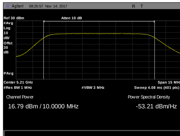
Plot 179. Maximum Conducted Output Power, 10M, 5210, Omni8, rf2, 15
