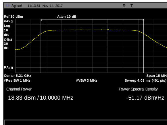
Plot 155. Maximum Conducted Output Power, 10M, 5210, 50mni, rf2
