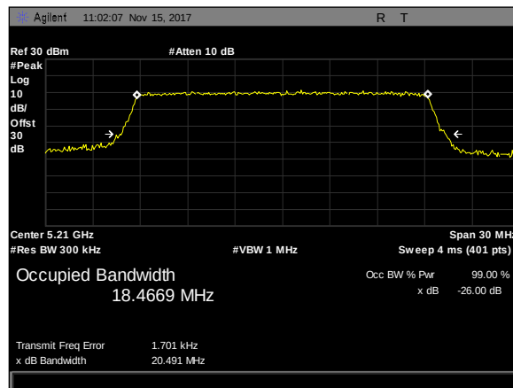
Plot 20. 26 dB Occupied Bandwidth, 20M, 5210, 2'Panel, rf2
