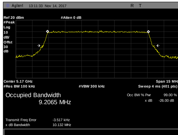
Plot 40. 26 dB Occupied Bandwidth, 10M, 5170, 90Sector, rf2
