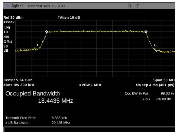
Plot 57. 26 dB Occupied Bandwidth, 20M, 5240, Omni8, rf2
