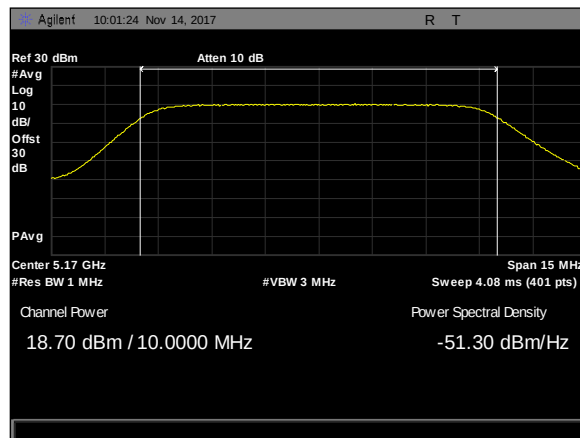
Plot 152. Maximum Conducted Output Power, 10M, 5170, 50mni, rf1
