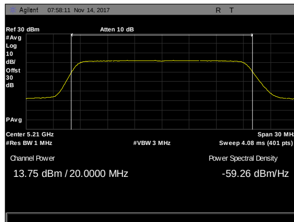
Plot 209. Maximum Conducted Output Power, 20M, 5210, 90Sector, rf2
