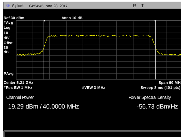
Plot 166. Maximum Conducted Output Power, 40M, 5210, 50mni, rf1
