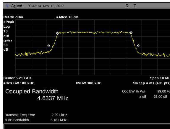
Plot 62. 26 dB Occupied Bandwidth, 5M, 5210, 50mni, rf2
