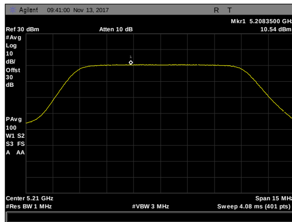
Plot 300. Maximum Power Spectral Density, 10M, 5210, 50mni, rf2
