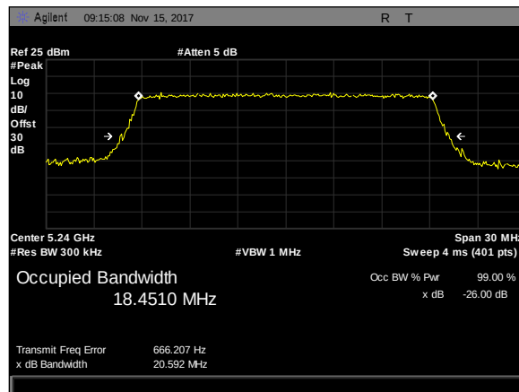
Plot 45. 26 dB Occupied Bandwidth, 20M, 5240, 90Sector, rf2
