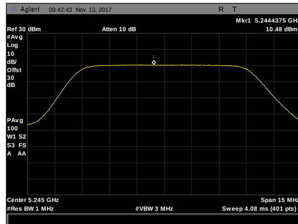
Plot 302. Maximum Power Spectral Density, 10M, 5245, 5Omni, rf2
