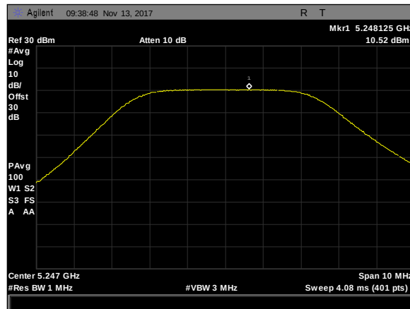
Plot 296. Maximum Power Spectral Density, 5M, 5247.5, 50Omni, rf2
