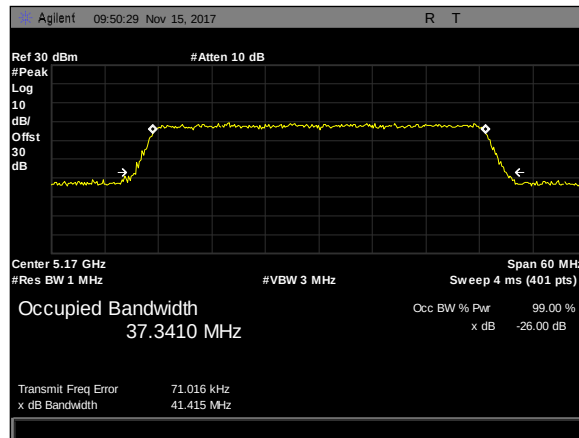
Plot 70. 26 dB Occupied Bandwidth, 40M, 5170, 50Omni, rf2
