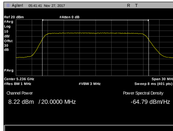
Plot 115. Maximum Conducted Output Power, 20M, 5235.5, 2Panel, rf2
