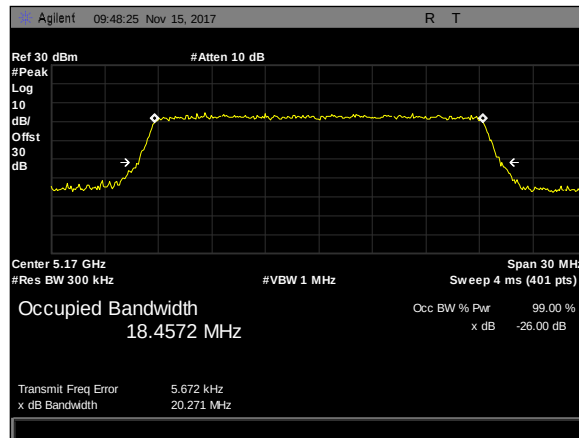
Plot 67. 26 dB Occupied Bandwidth, 20M, 5170, 50Omni, rf2
