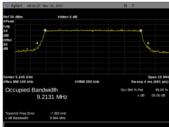
Plot 54. 26 dB Occupied Bandwidth, 10M, 5245, Omni8, rf2
