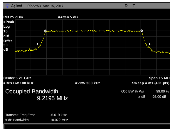
Plot 53. 26 dB Occupied Bandwidth, 10M, 5210, Omni8, rf2
