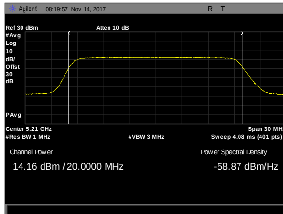
Plot 208. Maximum Conducted Output Power, 20M, 5210, 90Sector, rf1
