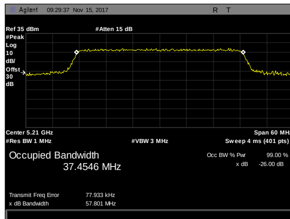
Plot 59. 26 dB Occupied Bandwidth, 40M, 5210, Omni8, rf2
