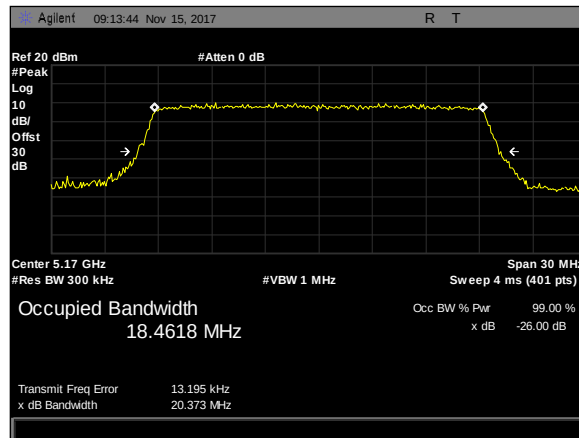
Plot 43. 26 dB Occupied Bandwidth, 20M, 5170, 90Sector, rf2
