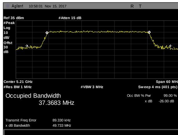
Plot 23. 26 dB Occupied Bandwidth, 40M, 5210, 2'Panel, rf2
