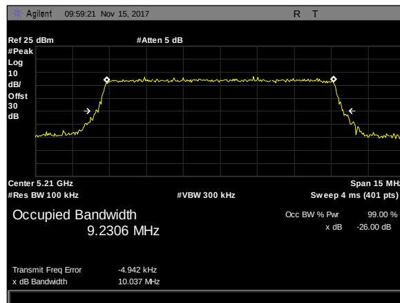
Plot 29. 26 dB Occupied Bandwidth, 10M, 5210, 3'Para, rf2
