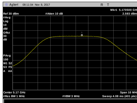
Plot 348. Maximum Power Spectral Density, 5M, 5170, 90Sector, rf1
