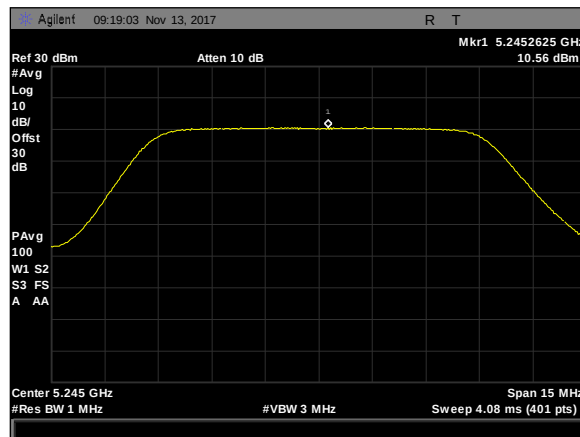
Plot 301. Maximum Power Spectral Density, 10M, 5245, 50mni, rf1
