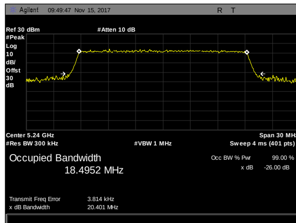
Plot 69. 26 dB Occupied Bandwidth, 20M, 5240, 50Omni, rf2
