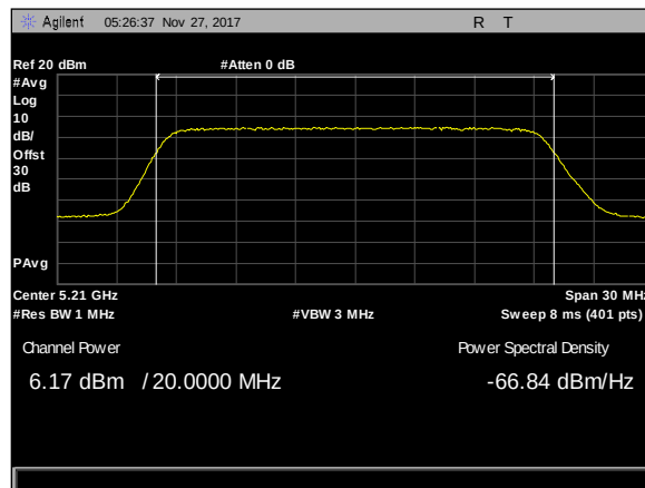
Plot 137. Maximum Conducted Output Power, 20M, 5210, 3Para, rf2
