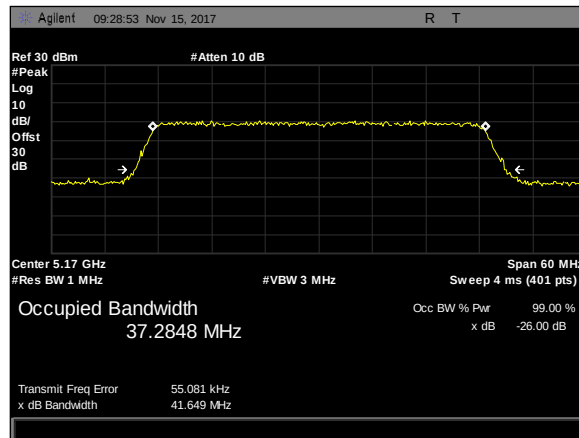
Plot 58. 26 dB Occupied Bandwidth, 40M, 5170, Omni8, rf2
