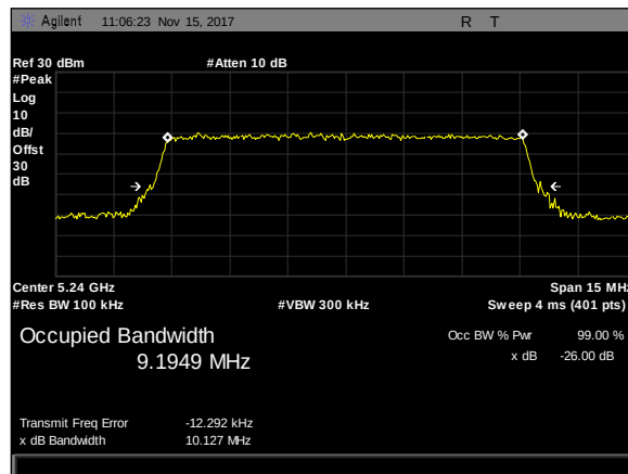
Plot 30. 26 dB Occupied Bandwidth, 10M, 5240.5, 3'Para, rf2
