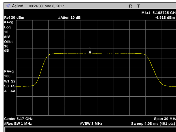
Plot 340. Maximum Power Spectral Density, 20M, 5170, 90Sector, rf1
