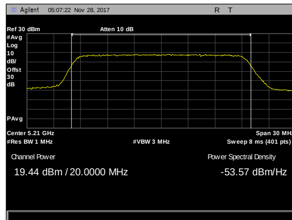
Plot 161. Maximum Conducted Output Power, 20M, 5210, 50mni, rf2
