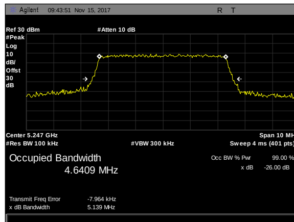
Plot 63. 26 dB Occupied Bandwidth, 5M, 5247.5, 50mni, rf2
