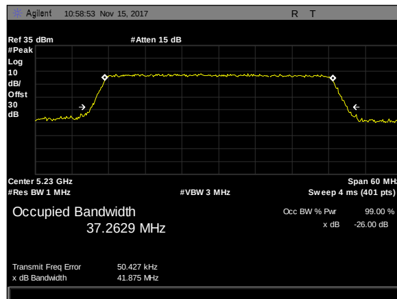
Plot 24. 26 dB Occupied Bandwidth, 40M, 5230, 2'Panel, rf2
