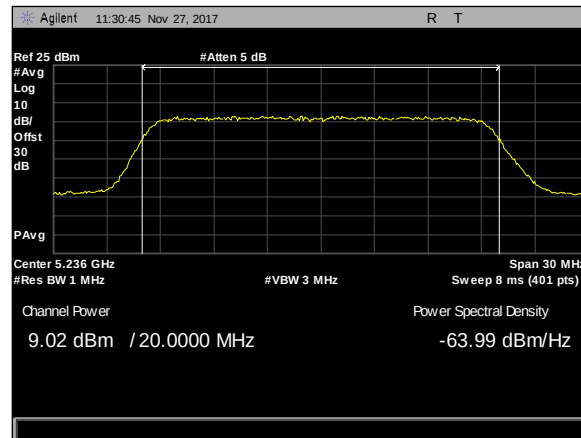
Plot 91. Maximum Conducted Output Power, 20M, 5235.5, 1Panel, rf2
