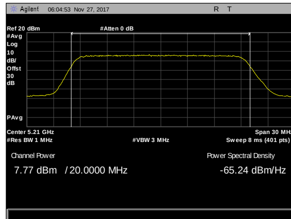
Plot 112. Maximum Conducted Output Power, 20M, 5210, 2Panel, rf1
