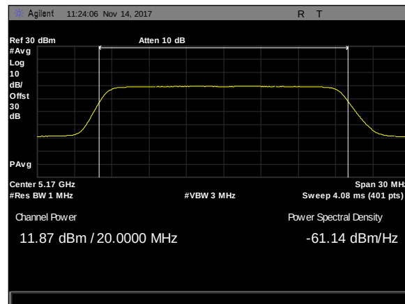
Plot 159. Maximum Conducted Output Power, 20M, 5170, 50mni, rf2
