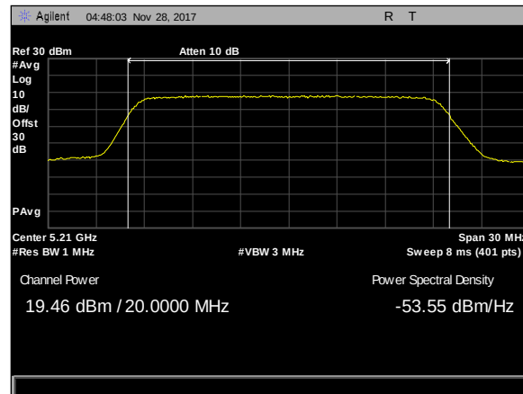
Plot 160. Maximum Conducted Output Power, 20M, 5210, 50mni, rf1
