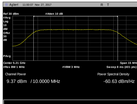
Plot 83. Maximum Conducted Output Power, 10M, 5210, 1Panel, rf1
