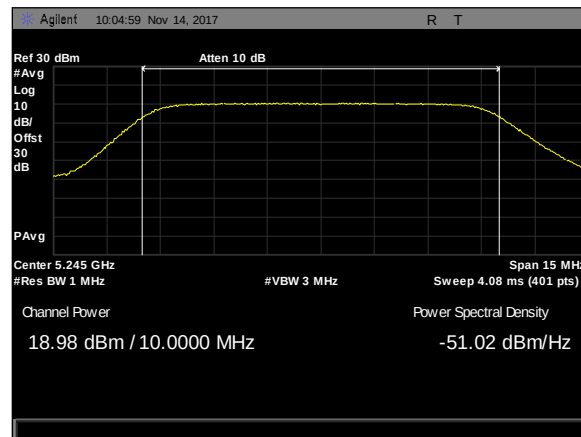
Plot 156. Maximum Conducted Output Power, 10M, 5245, 50mni, rf1
