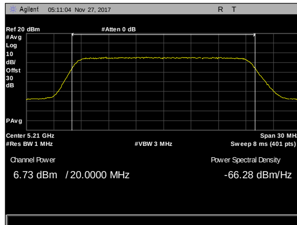
Plot 136. Maximum Conducted Output Power, 20M, 5210, 3Para, rf1
