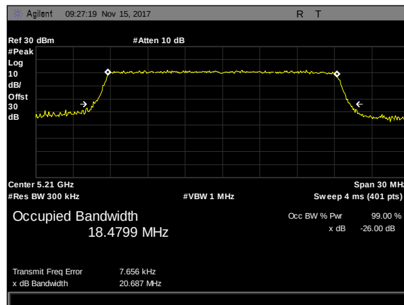
Plot 56. 26 dB Occupied Bandwidth, 20M, 5210, Omni8, rf2
