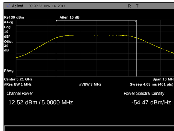
Plot 173. Maximum Conducted Output Power, 5M, 5210, Omni8, rf2
