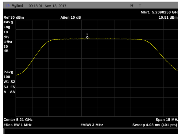
Plot 299. Maximum Power Spectral Density, 10M, 5210, 50mni, rf1
