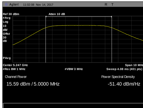
Plot 151. Maximum Conducted Output Power, 5M, 5247.5, 50mni, rf2
