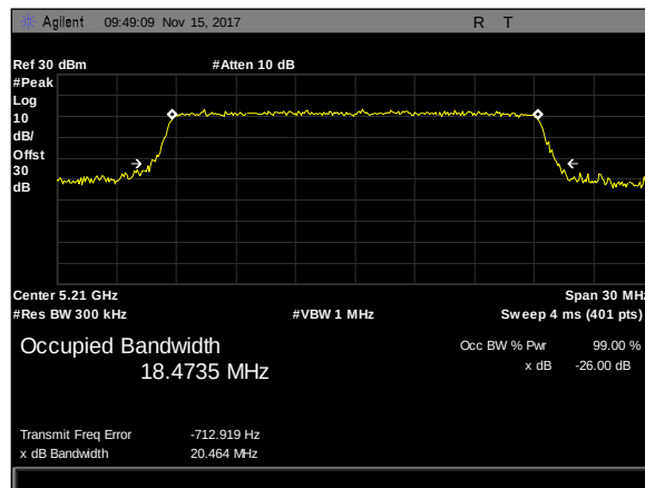
Plot 68. 26 dB Occupied Bandwidth, 20M, 5210, 50Omni, rf2
