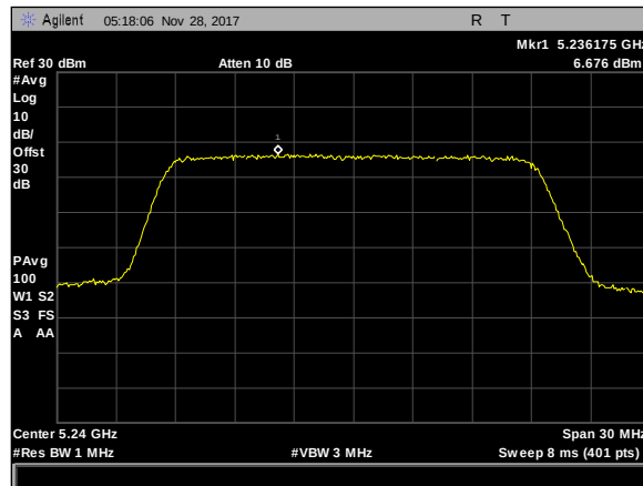
Plot 308. Maximum Power Spectral Density, 20M, 5240, 50mni, rf2
