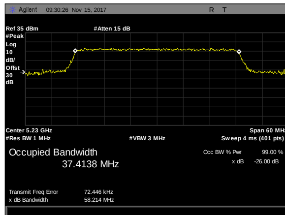
Plot 60. 26 dB Occupied Bandwidth, 40M, 5230, Omni8, rf2
