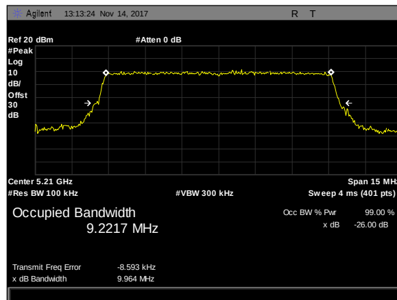
Plot 41. 26 dB Occupied Bandwidth, 10M, 5210, 90Sector, rf2
