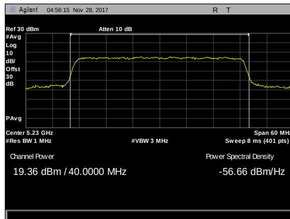
Plot 168. Maximum Conducted Output Power, 40M, 5230, 50mni, rf1
