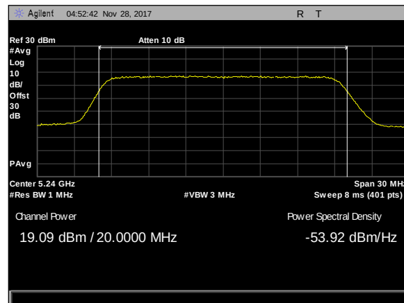
Plot 162. Maximum Conducted Output Power, 20M, 5240, 50mni, rf1
