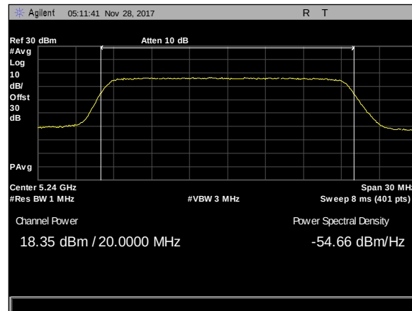
Plot 163. Maximum Conducted Output Power, 20M, 5240, 50mni, rf2
