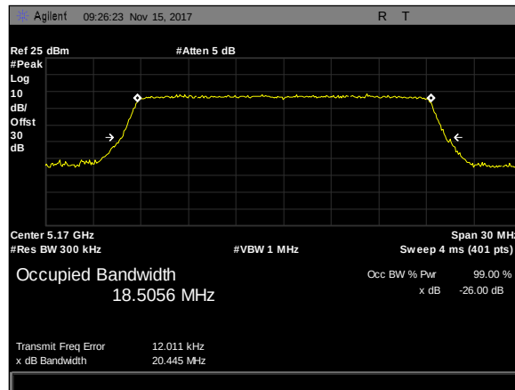
Plot 55. 26 dB Occupied Bandwidth, 20M, 5170, Omni8, rf2
