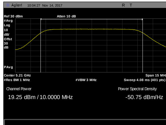
Plot 154. Maximum Conducted Output Power, 10M, 5210, 50mni, rf1
