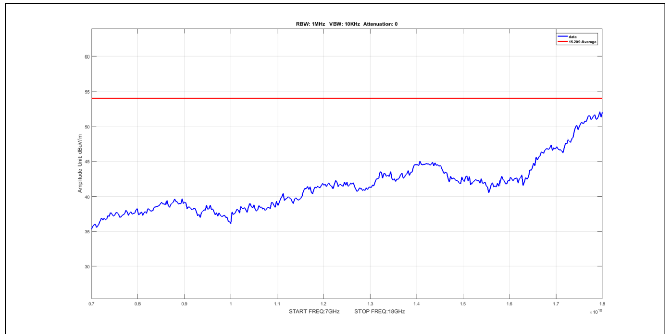
Plot 483. Undesirable Emissions, 3Para Avg 7-18GHz 40M 5210 pow5
