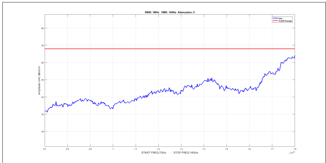
Plot 484. Undesirable Emissions, 3Para Avg 7-18GHz 40M 5230 pow5
