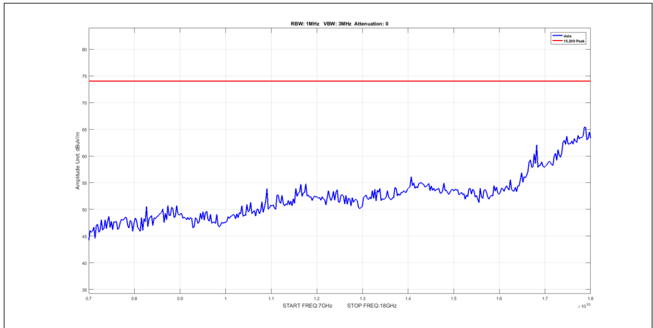
Plot 555. Undesirable Emissions, 50mni Peak 7-18GHz 20M 5230 pow20
