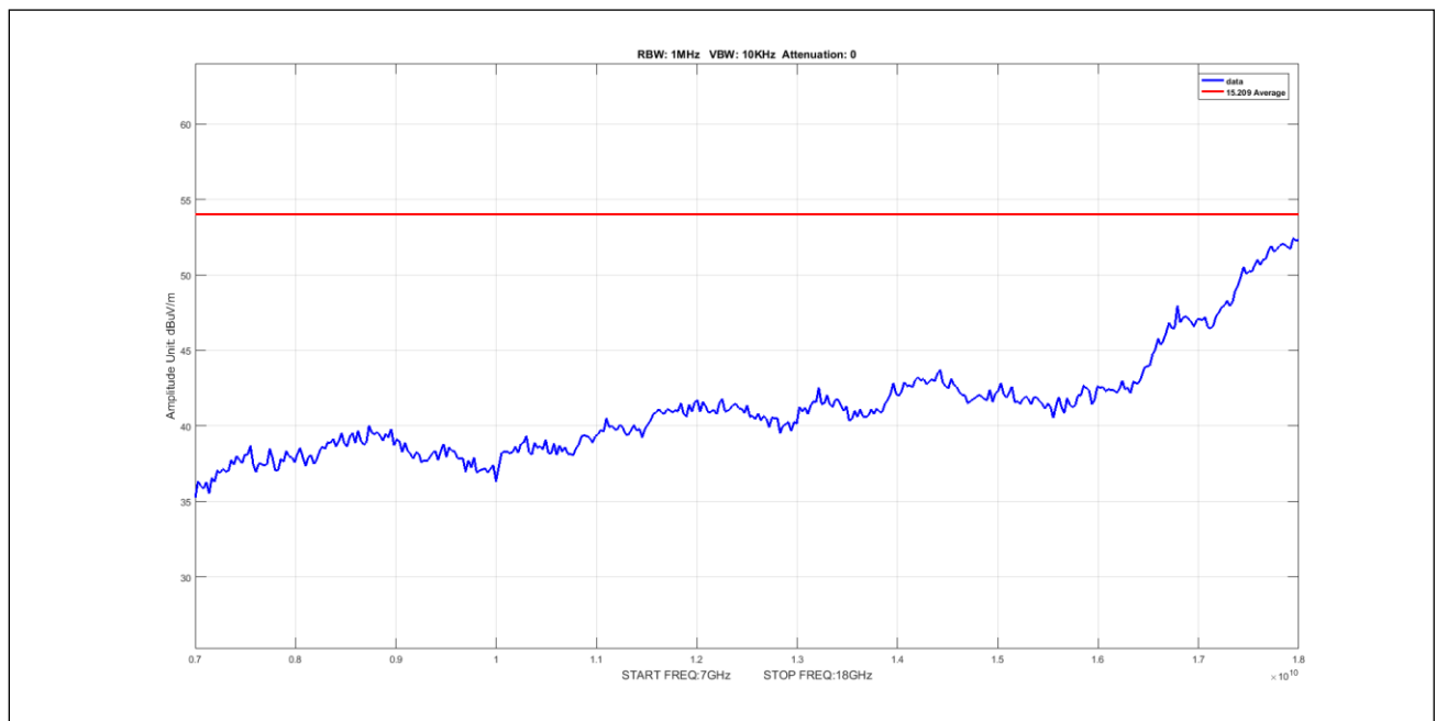
Plot 524. Undesirable Emissions, 50mni Avg 7-18GHz 5M 5210 pow14
