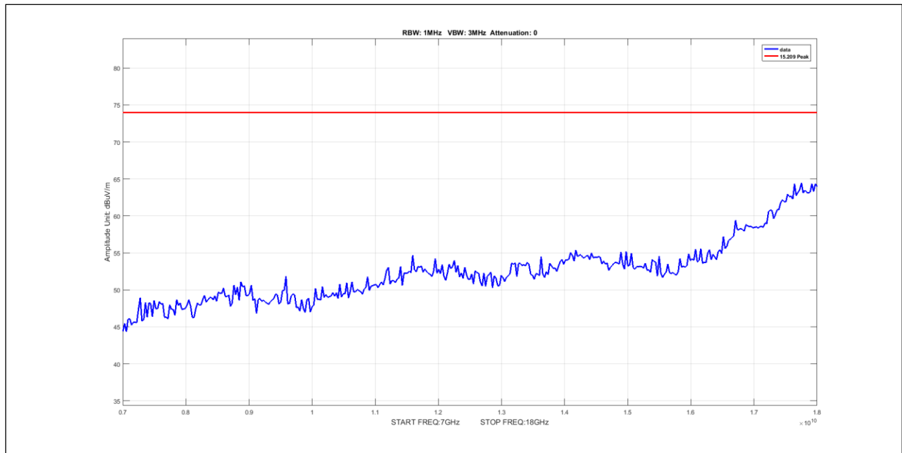
Plot 551. Undesirable Emissions, 5Omni Peak 7-18GHz 10M 5210 pow17
