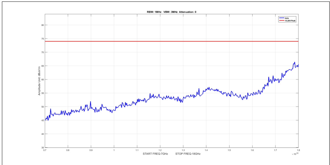
Plot 507. Undesirable Emissions, 3Para Peak 7-18GHz 40M 5210 pow5
