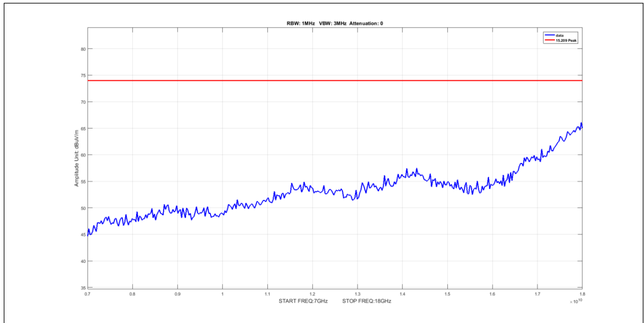
Plot 499. Undesirable Emissions, 3Para Peak 7-18GHz 5M 5242.5 pow0
