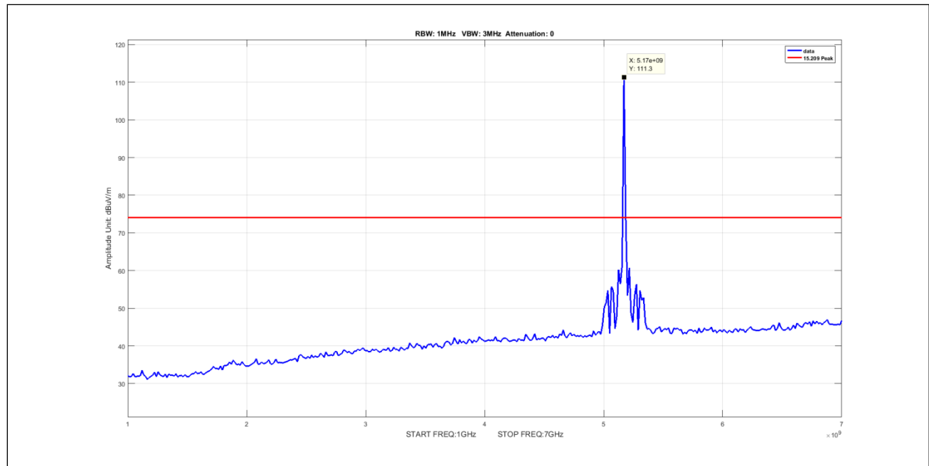
Plot 535. Undesirable Emissions, 5Omni Peak 1-7GHz 5M 5170 pow14
