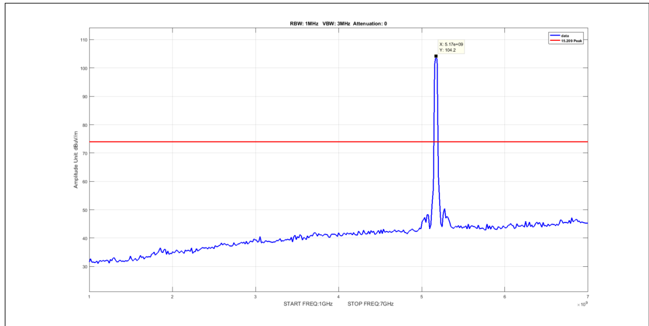
Plot 541. Undesirable Emissions, 50mni Peak 1-7GHz 20M 5170 pow10
