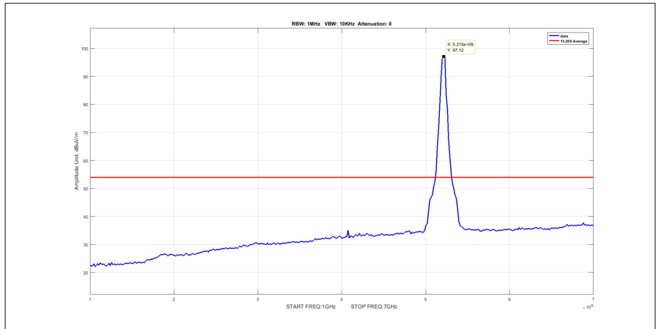
Plot 519. Undesirable Emissions, 50mni Avg 1-7GHz 40M 5210 pow21
