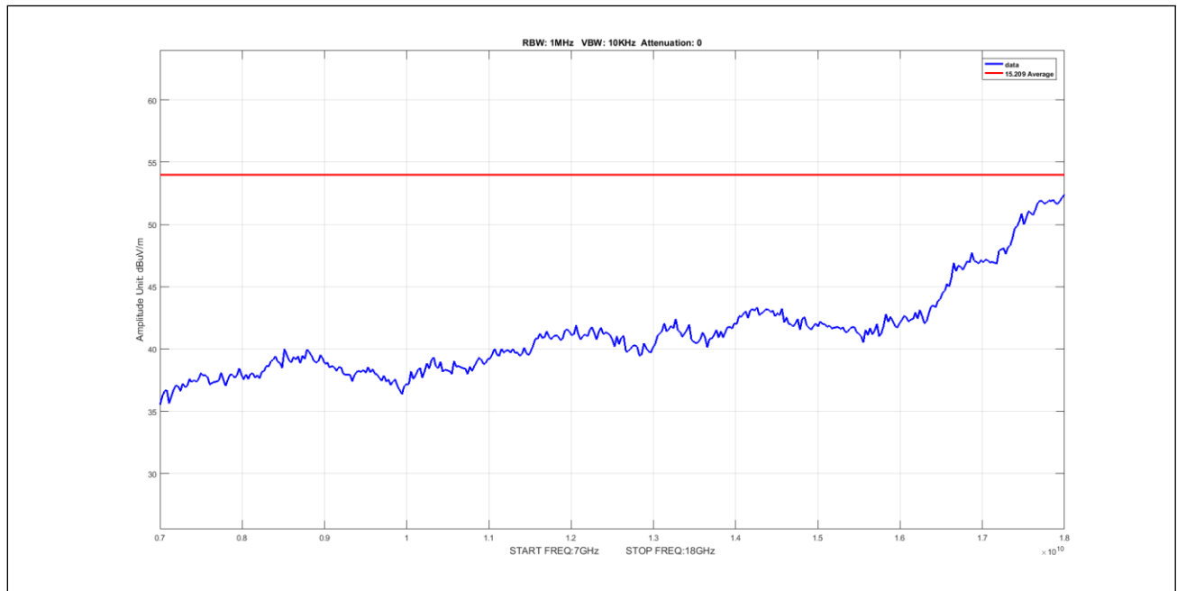
Plot 527. Undesirable Emissions, 50mni Avg 7-18GHz 10M 5210 pow17
