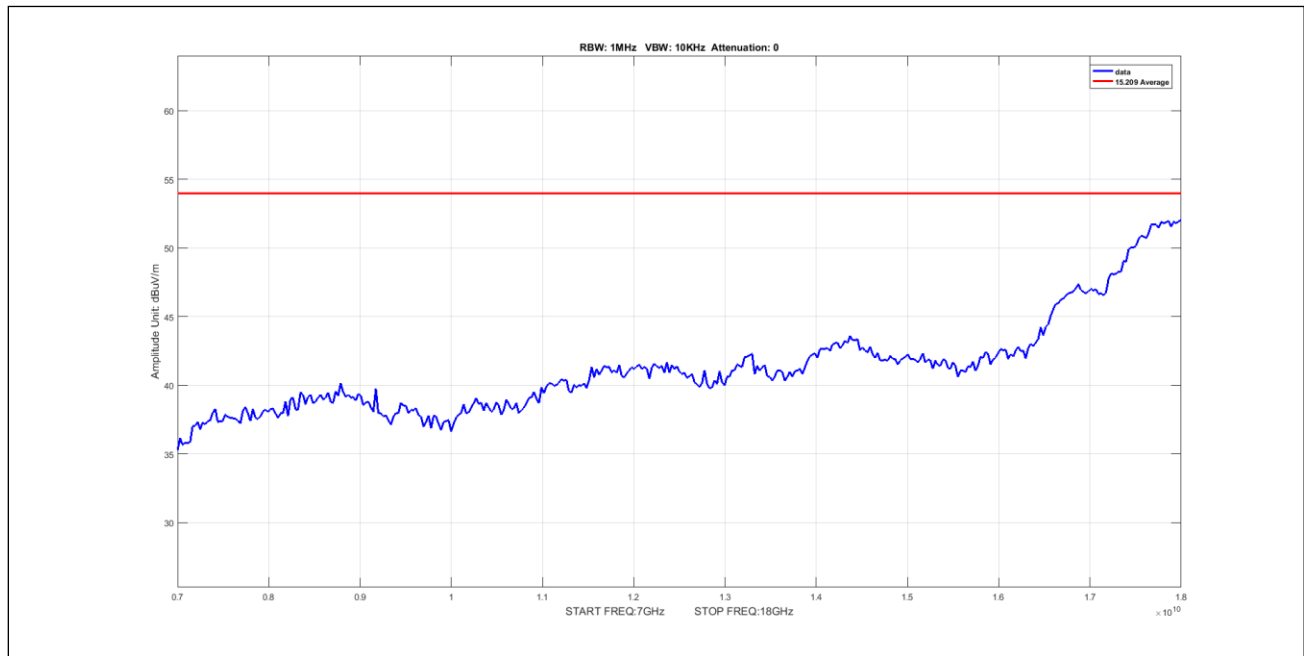
Plot 529. Undesirable Emissions, 50mni Avg 7-18GHz 20M 5170 pow10
