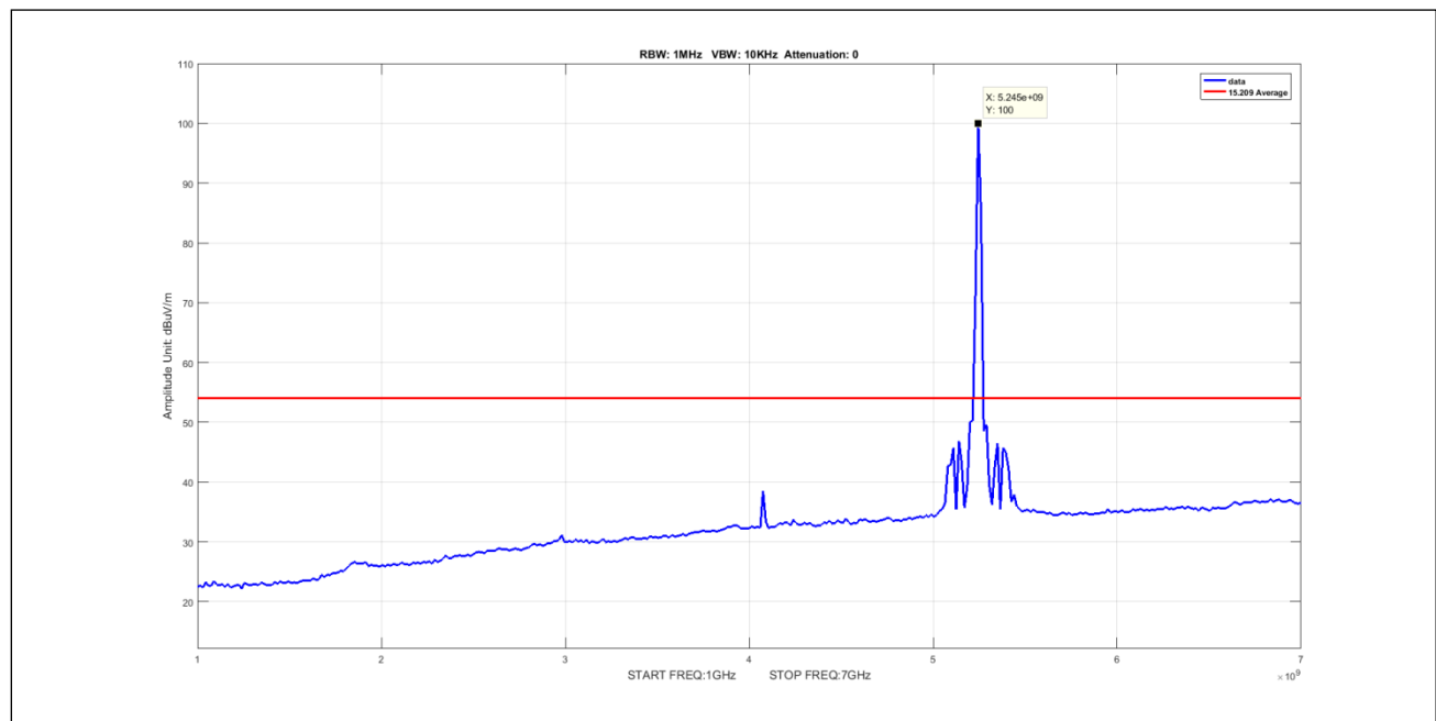
Plot 564. Undesirable Emissions, 8Omni Avg 1-7GHz 10M 5245 pow15
