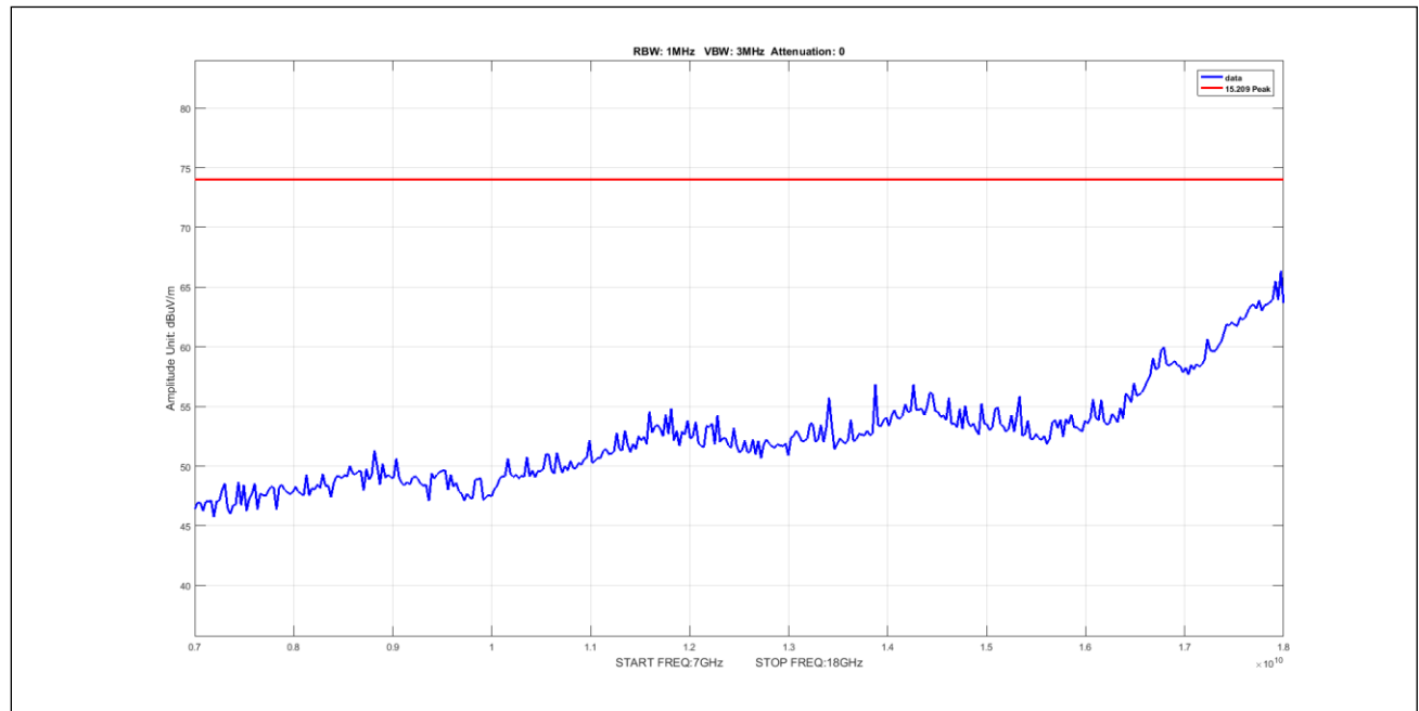
Plot 549. Undesirable Emissions, 50mni Peak 7-18GHz 5M 5247.5 pow14
