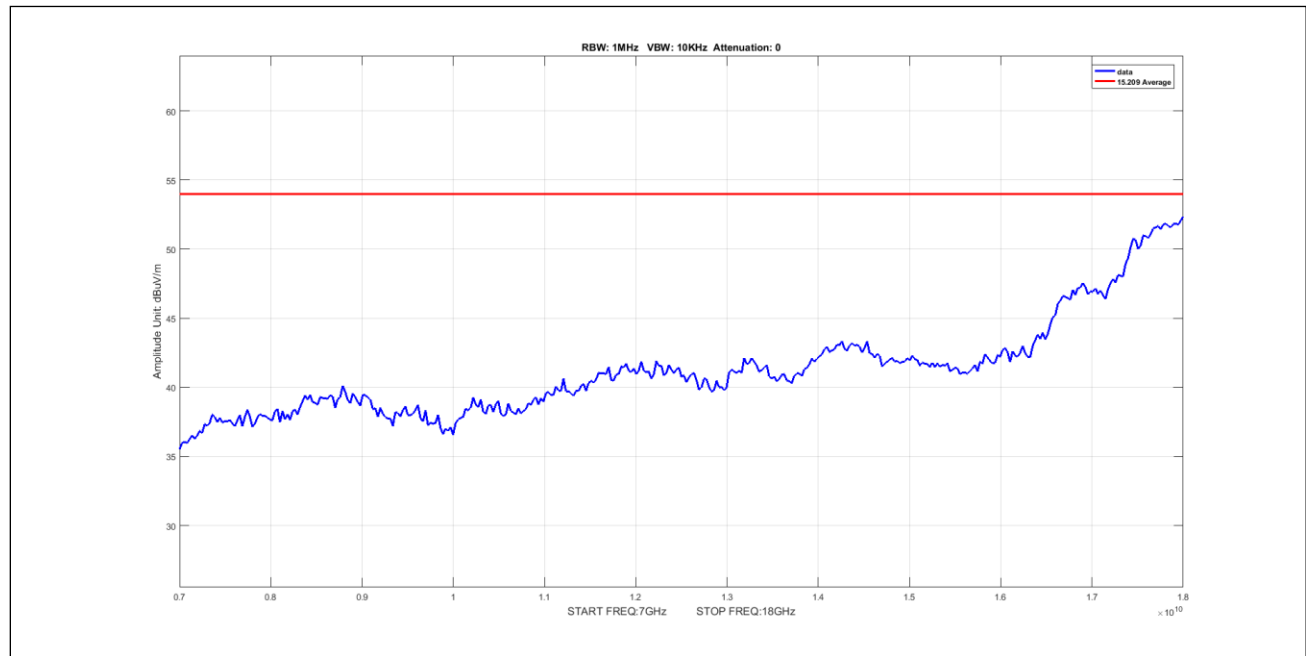
Plot 533. Undesirable Emissions, 50mni Avg 7-18GHz 40M 5210 pow21
