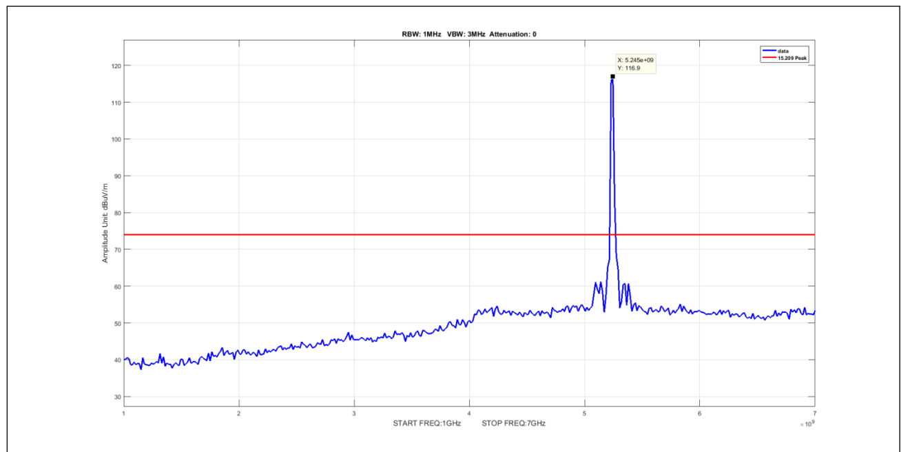
Plot 490. Undesirable Emissions, 3Para Peak 1-7GHz 10M 5240.5 pow3
