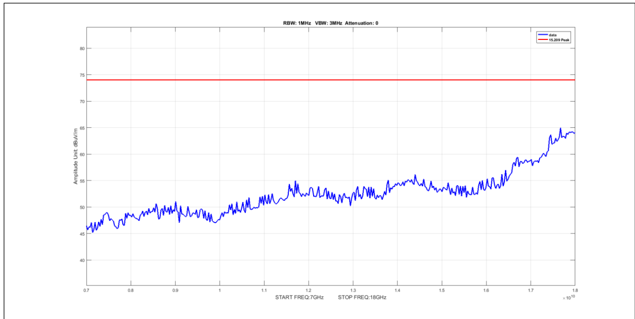
Plot 557. Undesirable Emissions, 5Omni Peak 7-18GHz 40M 5210 pow21
