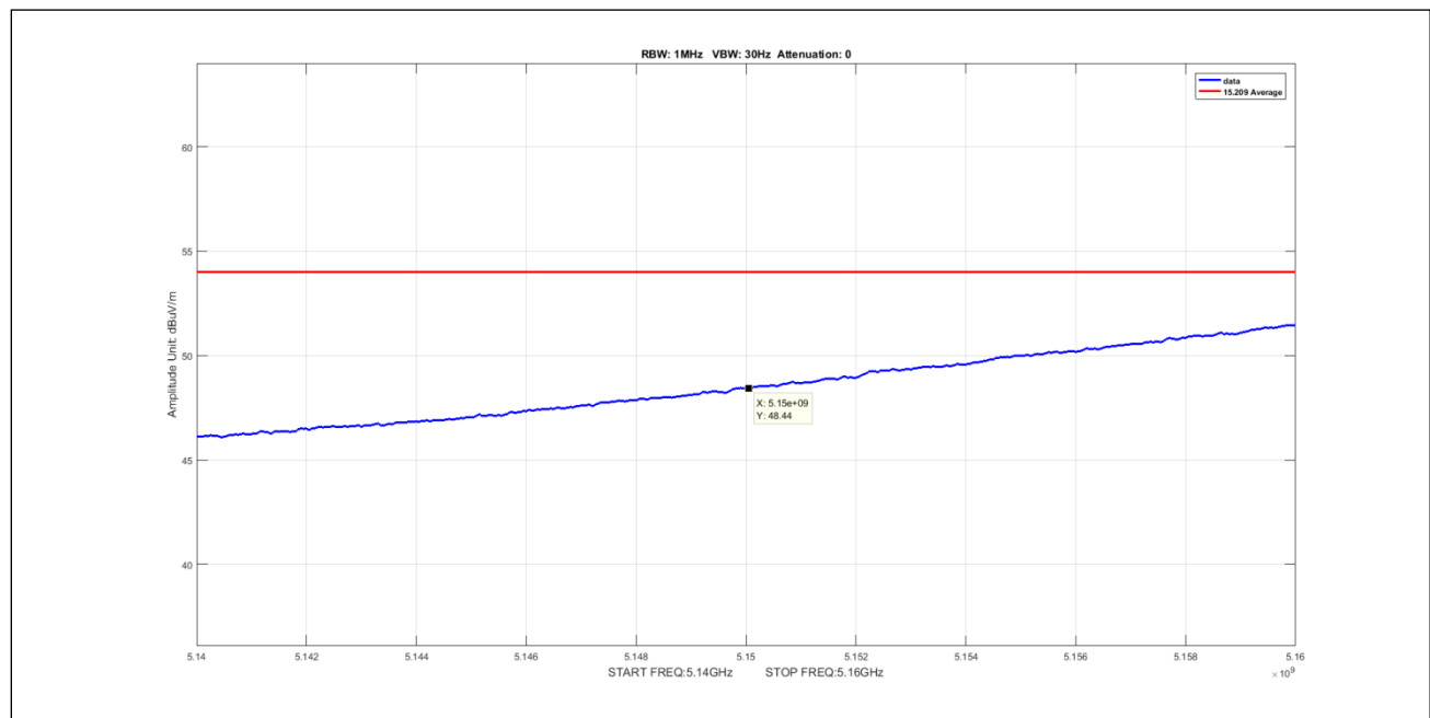
Plot 522. Undesirable Emissions, 50mni Avg 1-7GHz 40M 5230 pow22 zoom
