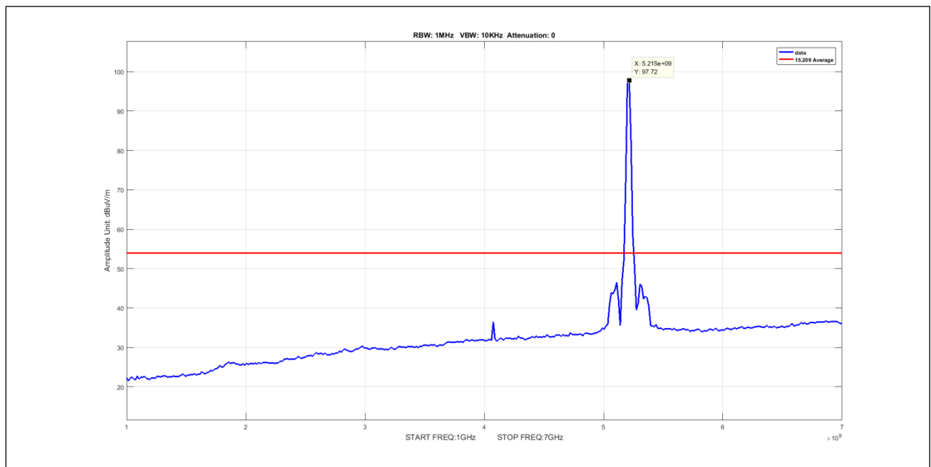
Plot 566. Undesirable Emissions, 8Omni Avg 1-7GHz 20M 5210 pow18
