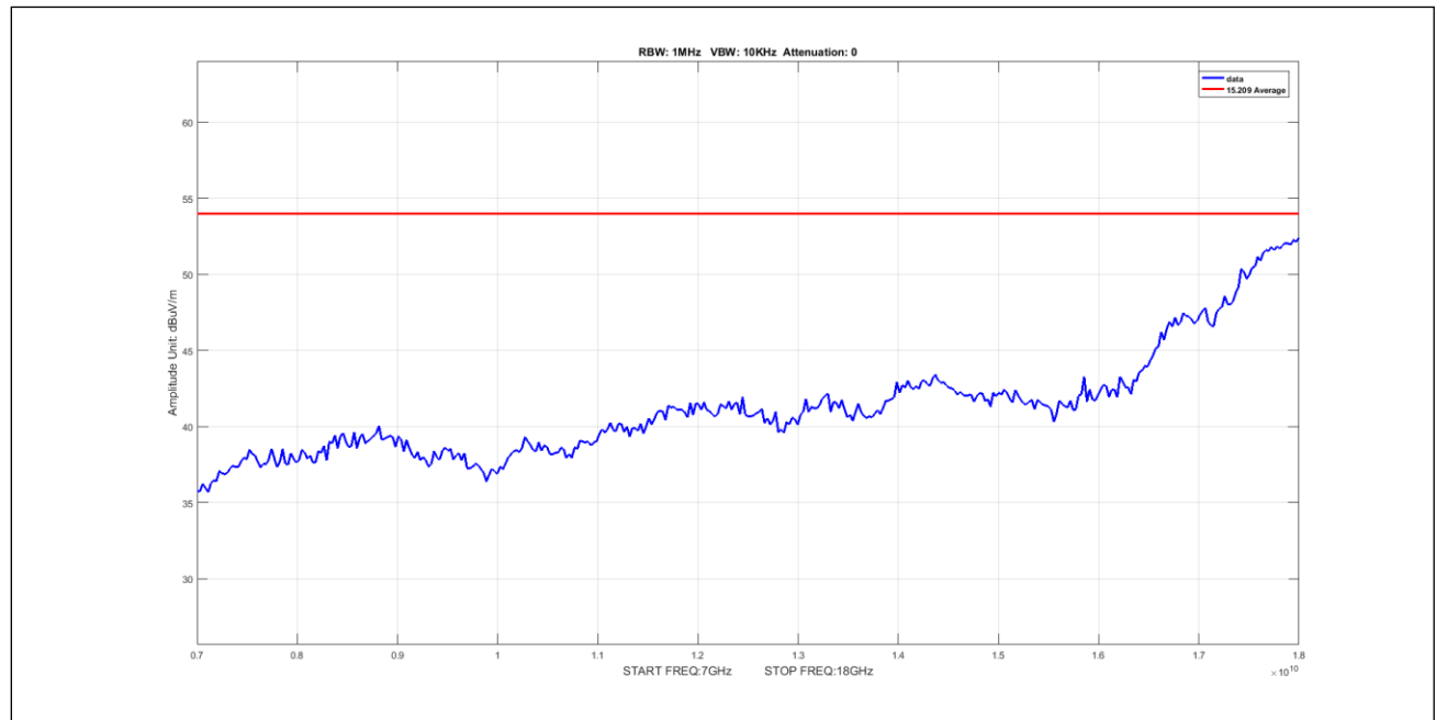
Plot 525. Undesirable Emissions, 50mni Avg 7-18GHz 5M 5247.5 pow14
