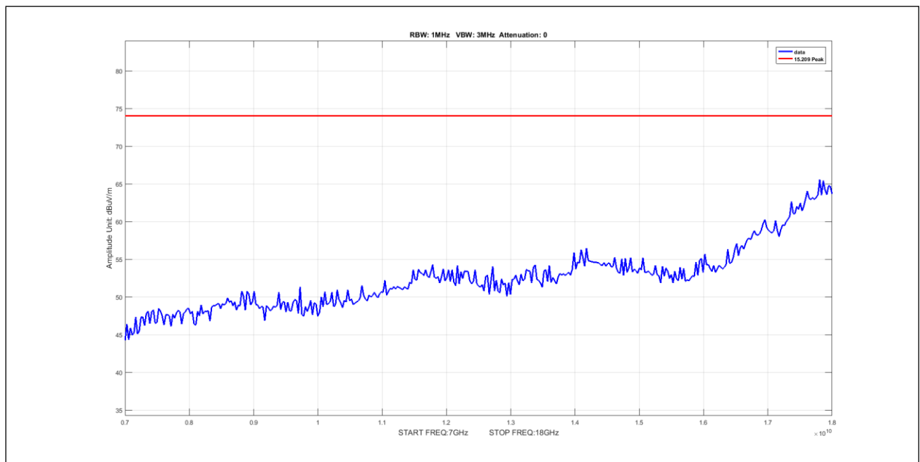
Plot 556. Undesirable Emissions, 50mni Peak 7-18GHz 40M 5170 pow3
