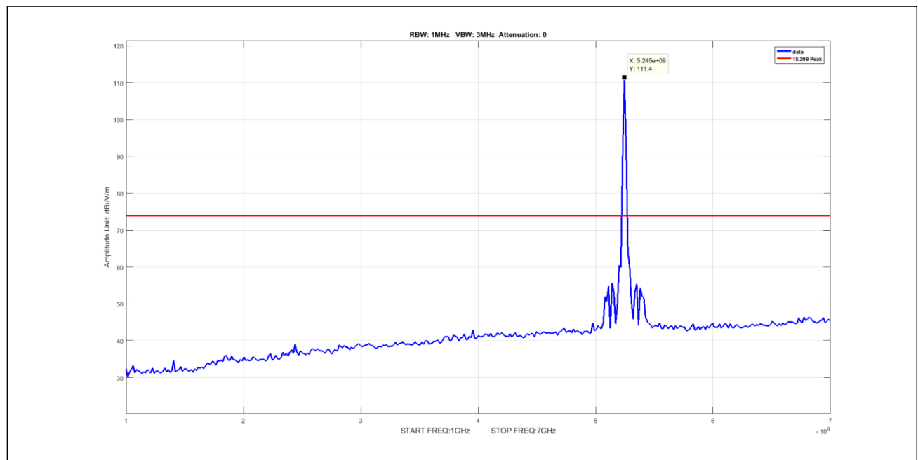
Plot 540. Undesirable Emissions, 5Omni Peak 1-7GHz 10M 5245 pow17
