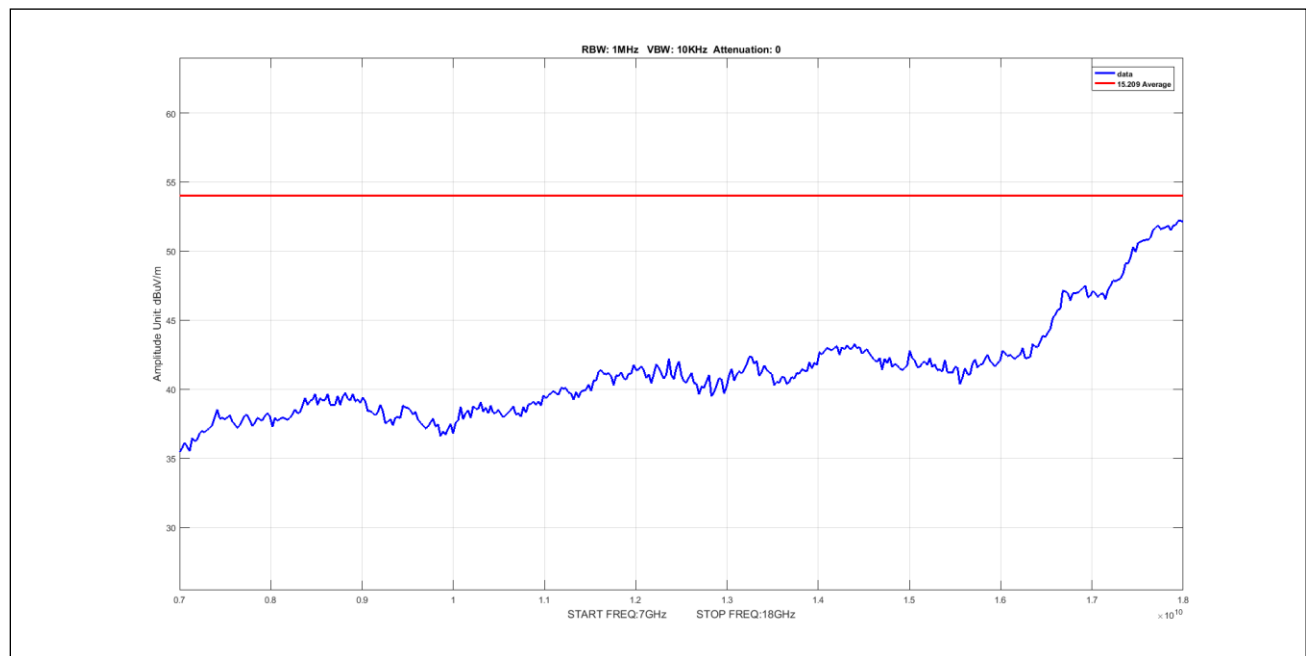
Plot 534. Undesirable Emissions, 50mni Avg 7-18GHz 40M 5230 pow22
