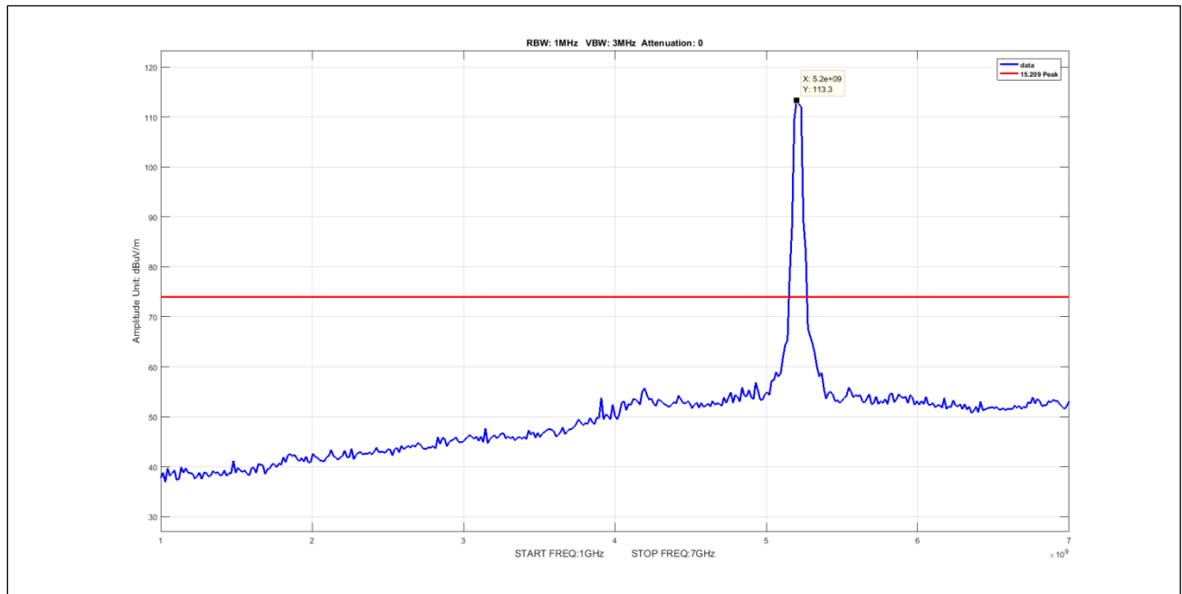
Plot 495. Undesirable Emissions, 3Para Peak 1-7GHz 40M 5210 pow5
