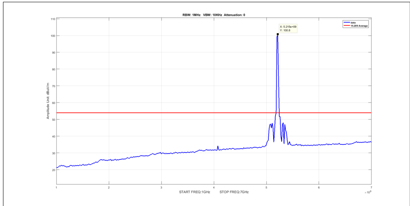
Plot 513. Undesirable Emissions, 5Omni Avg 1-7GHz 10M 5210 pow17
