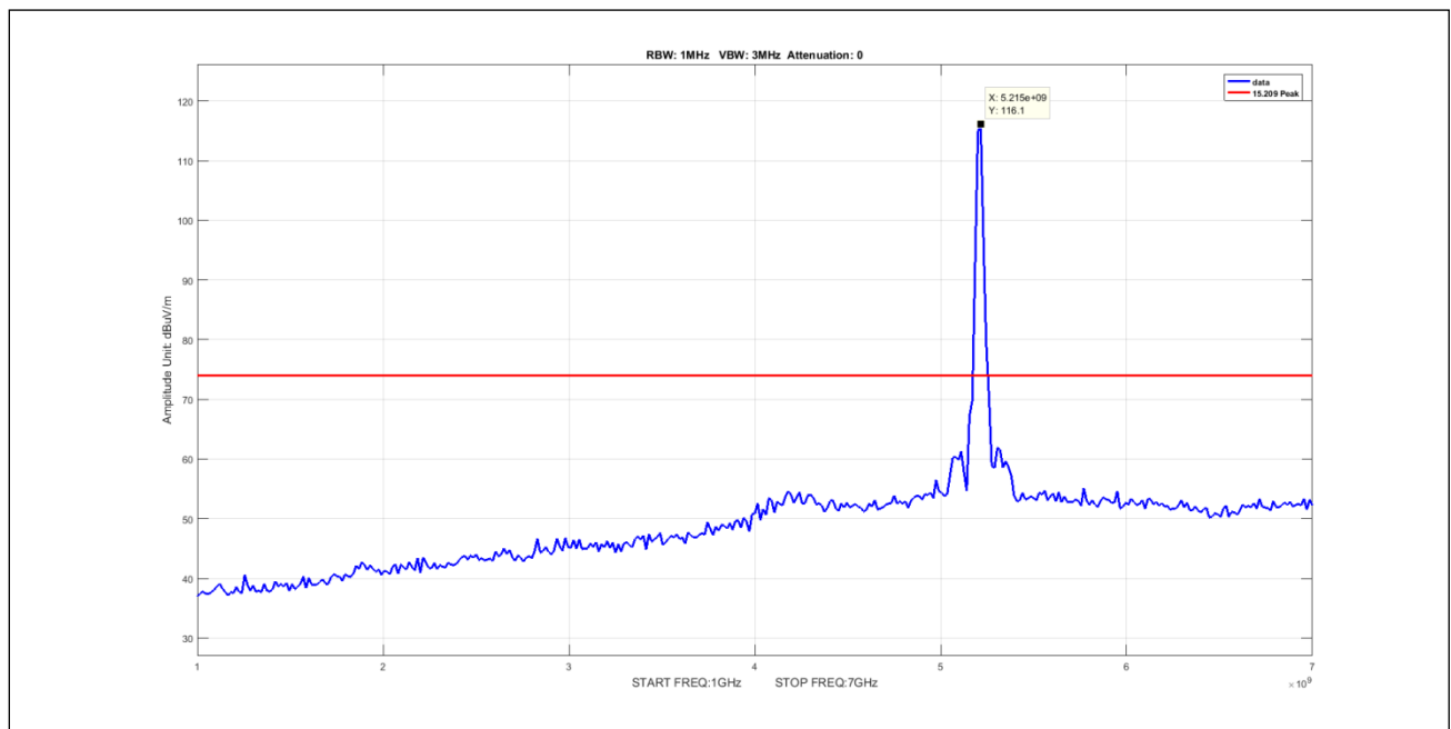
Plot 492. Undesirable Emissions, 3Para Peak 1-7GHz 20M 5210 pow5
