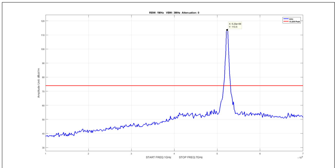
Plot 496. Undesirable Emissions, 3Para Peak 1-7GHz 40M 5230 pow8
