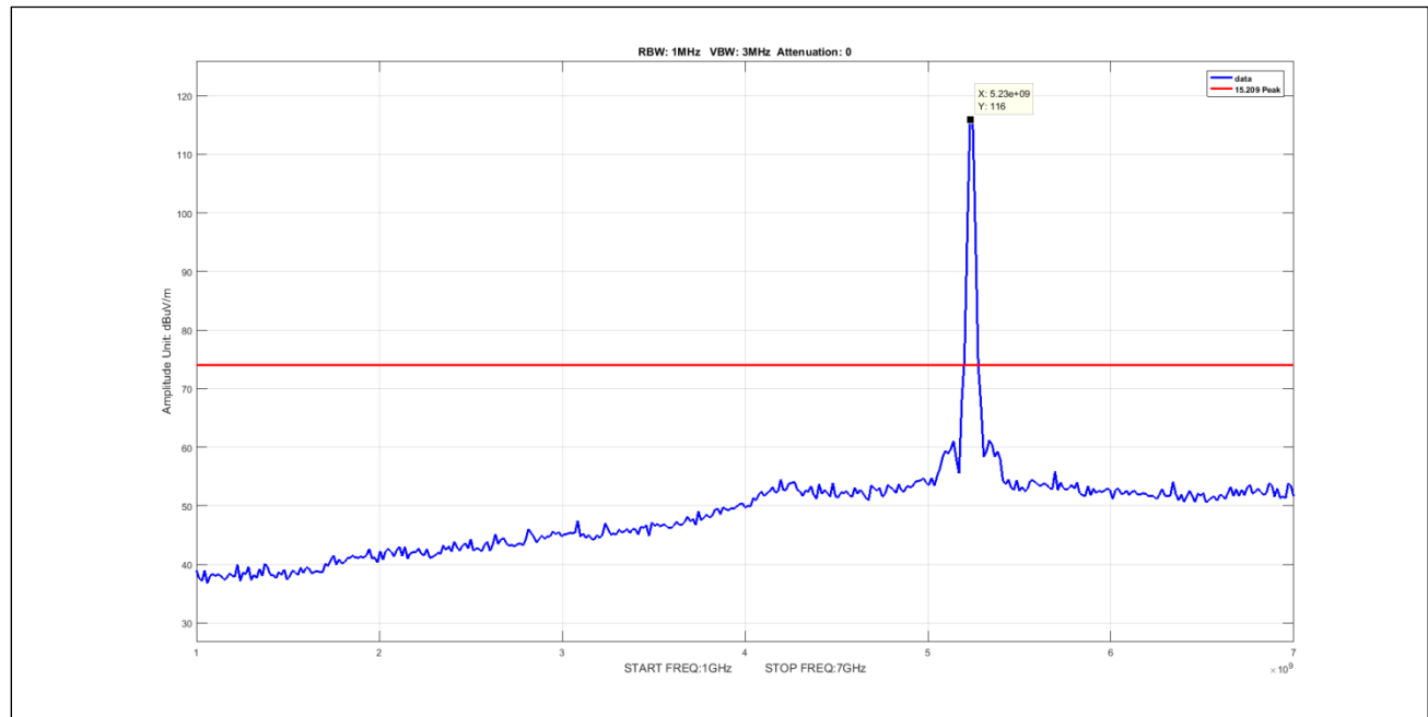
Plot 493. Undesirable Emissions, 3Para Peak 1-7GHz 20M 5235.5 pow5
