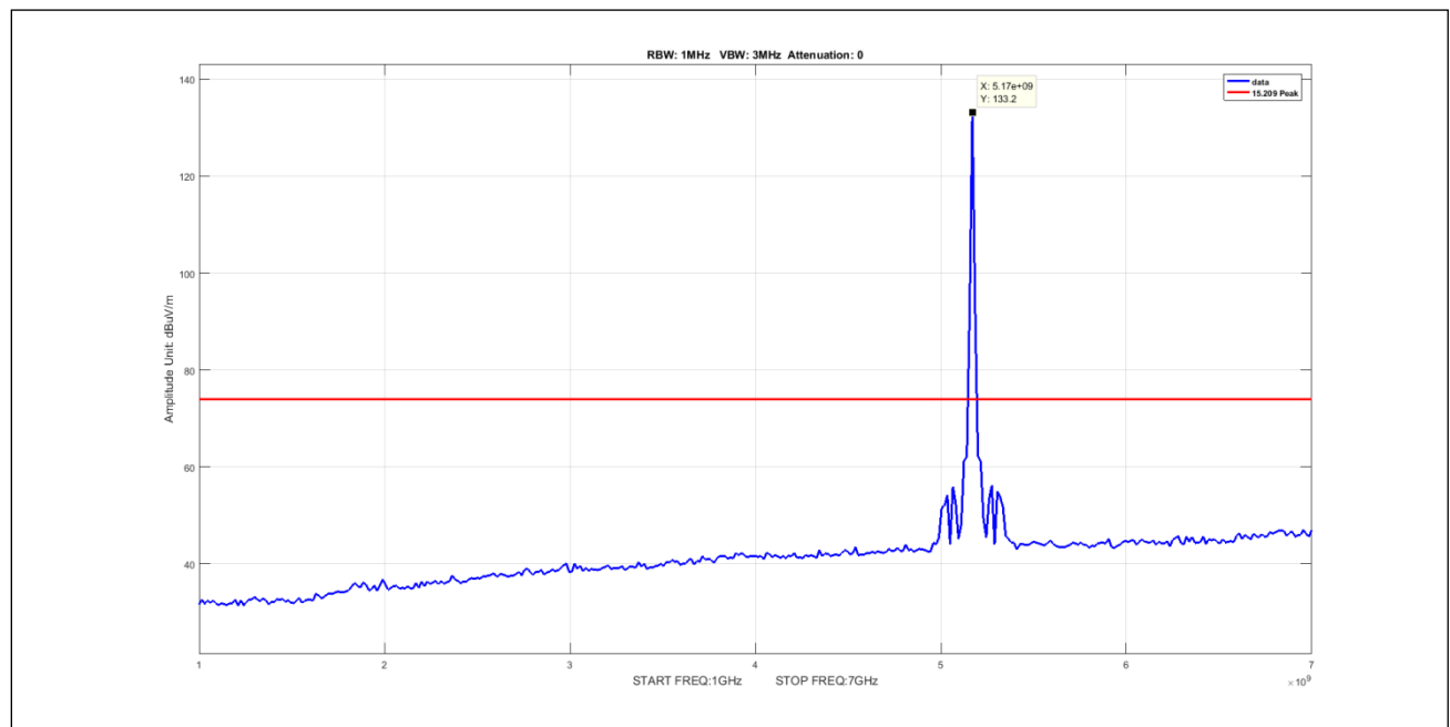
Plot 538. Undesirable Emissions, 5Omni Peak 1-7GHz 10M 5170 pow17
