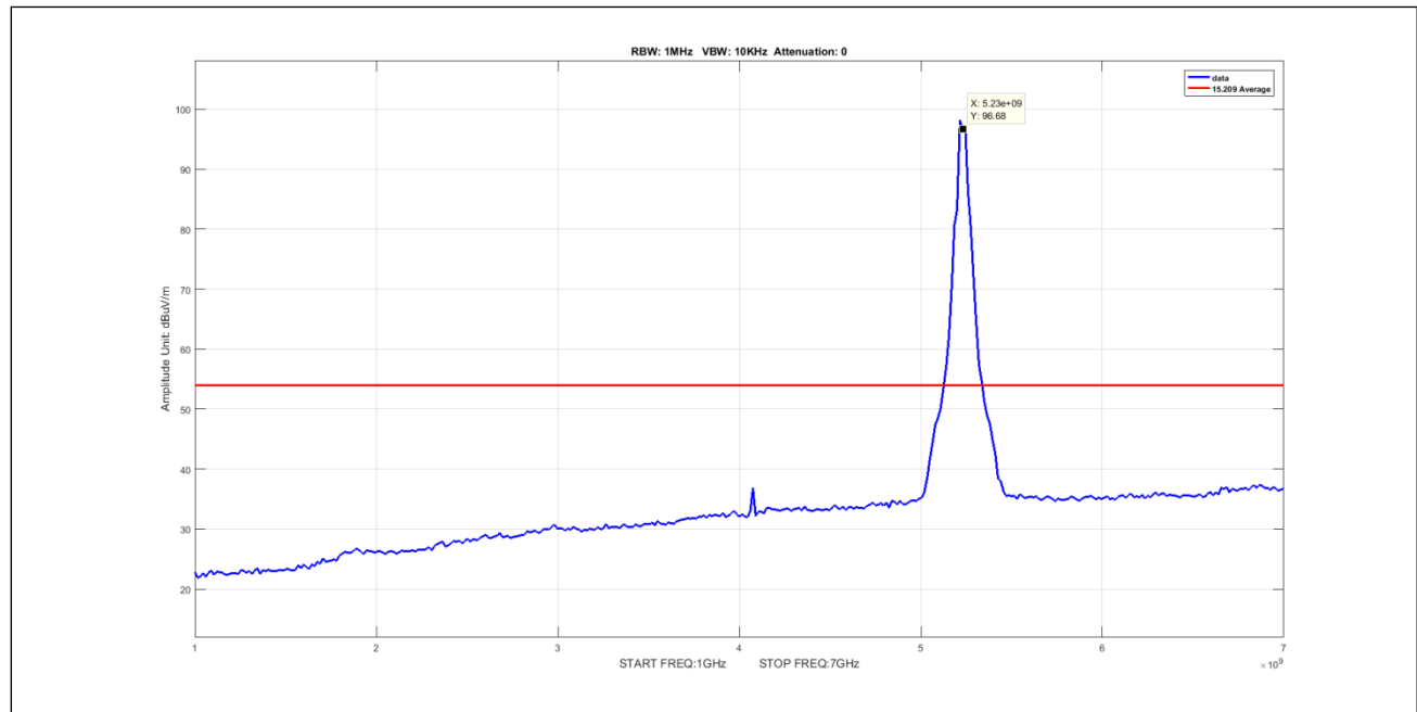
Plot 521. Undesirable Emissions, 50mni Avg 1-7GHz 40M 5230 pow22
