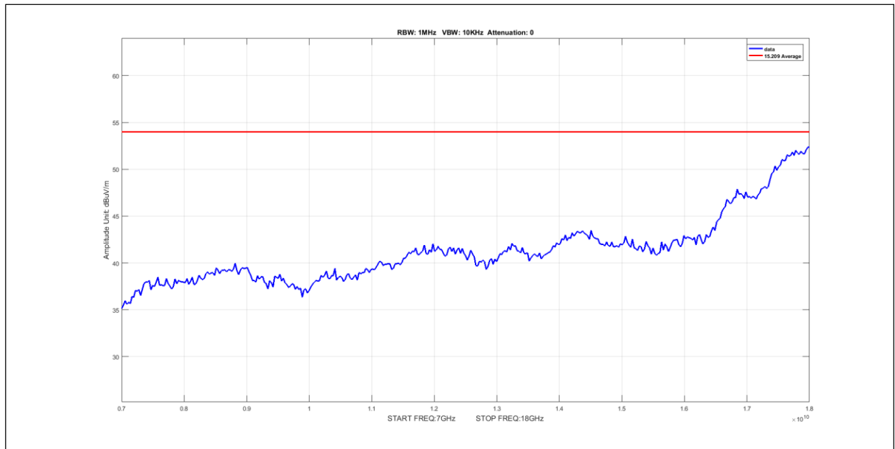
Plot 523. Undesirable Emissions, 50mni Avg 7-18GHz 5M 5170 pow14
