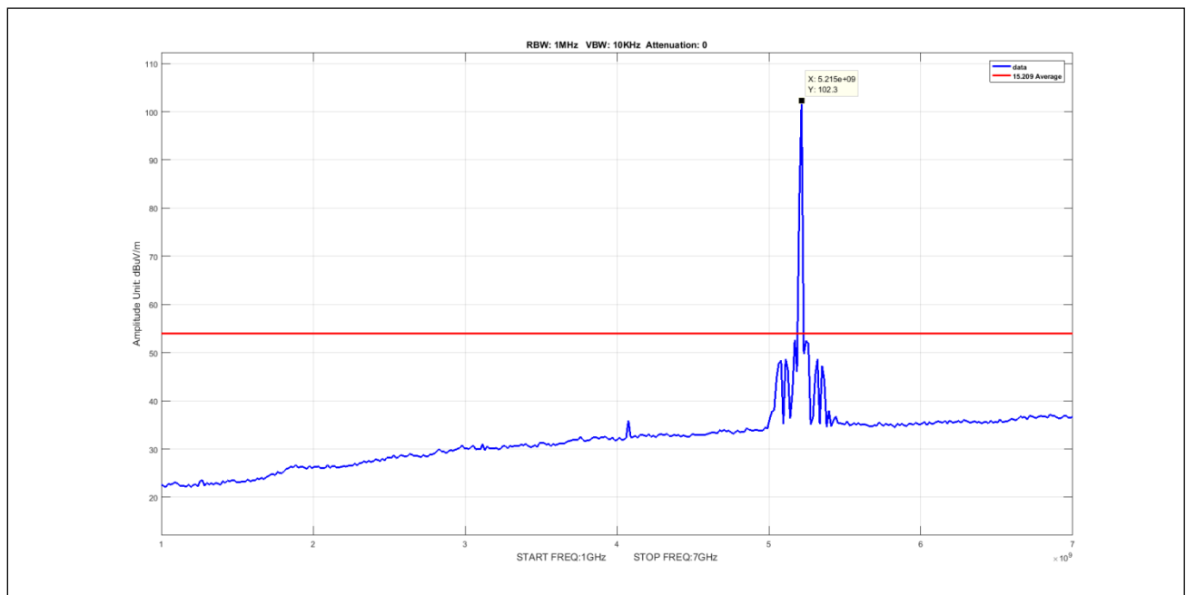
Plot 510. Undesirable Emissions, 50mni Avg 1-7GHz 5M 5210 pow14
