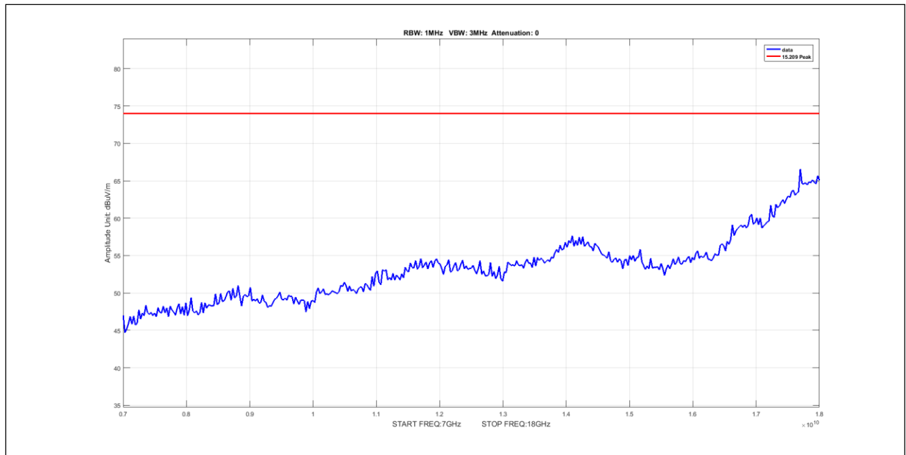
Plot 505. Undesirable Emissions, 3Para Peak 7-18GHz 20M 5235.5 pow5
