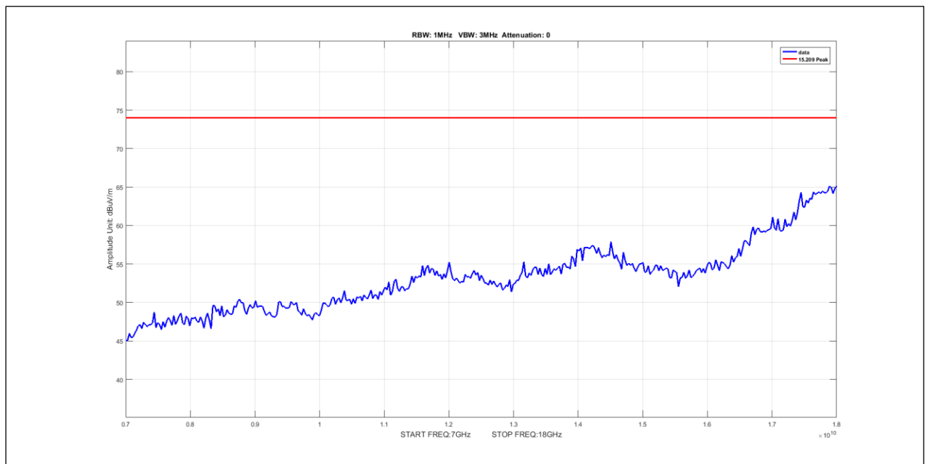
Plot 506. Undesirable Emissions, 3Para Peak 7-18GHz 40M 5171 pow-10
