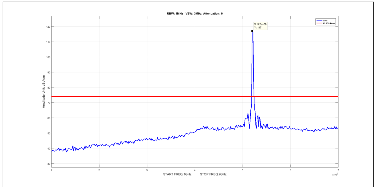
Plot 489. Undesirable Emissions, 3Para Peak 1-7GHz 10M 5210 pow3
