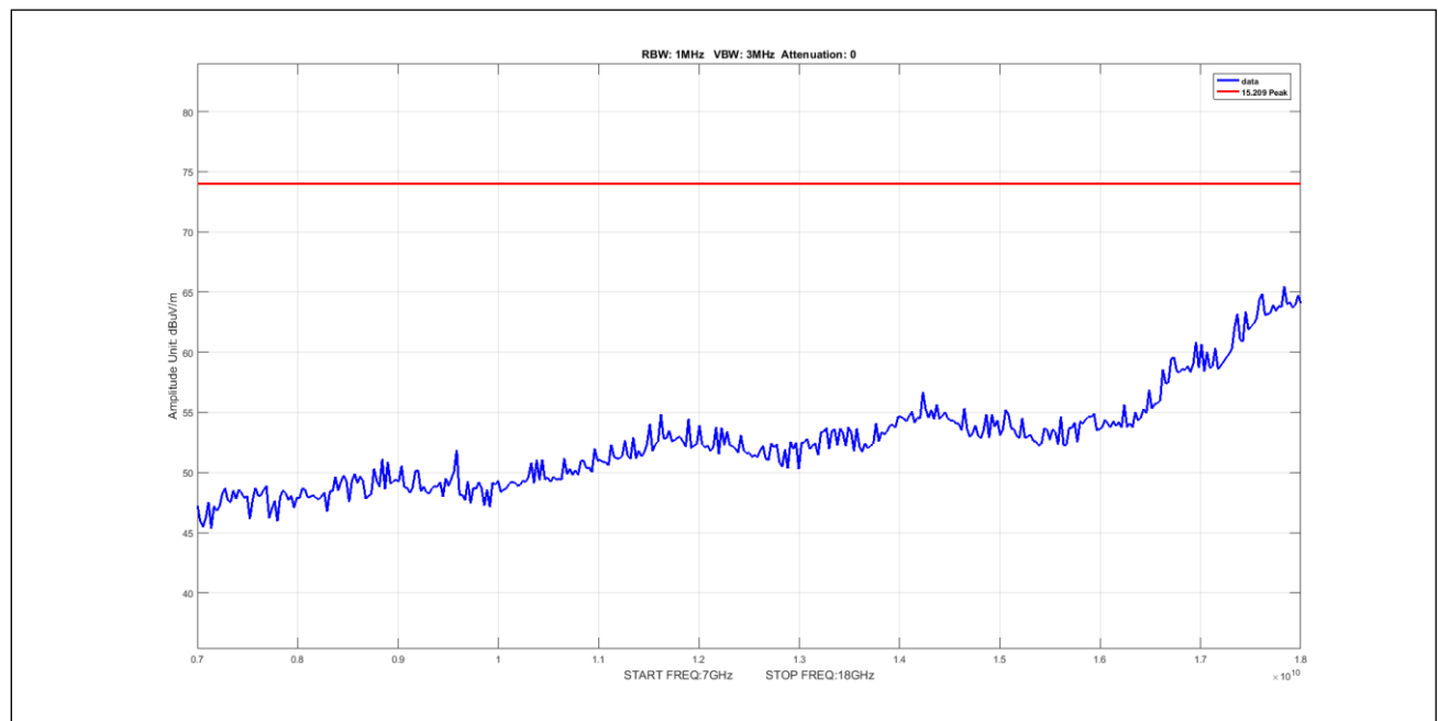
Plot 550. Undesirable Emissions, 50mni Peak 7-18GHz 10M 5170 pow17
