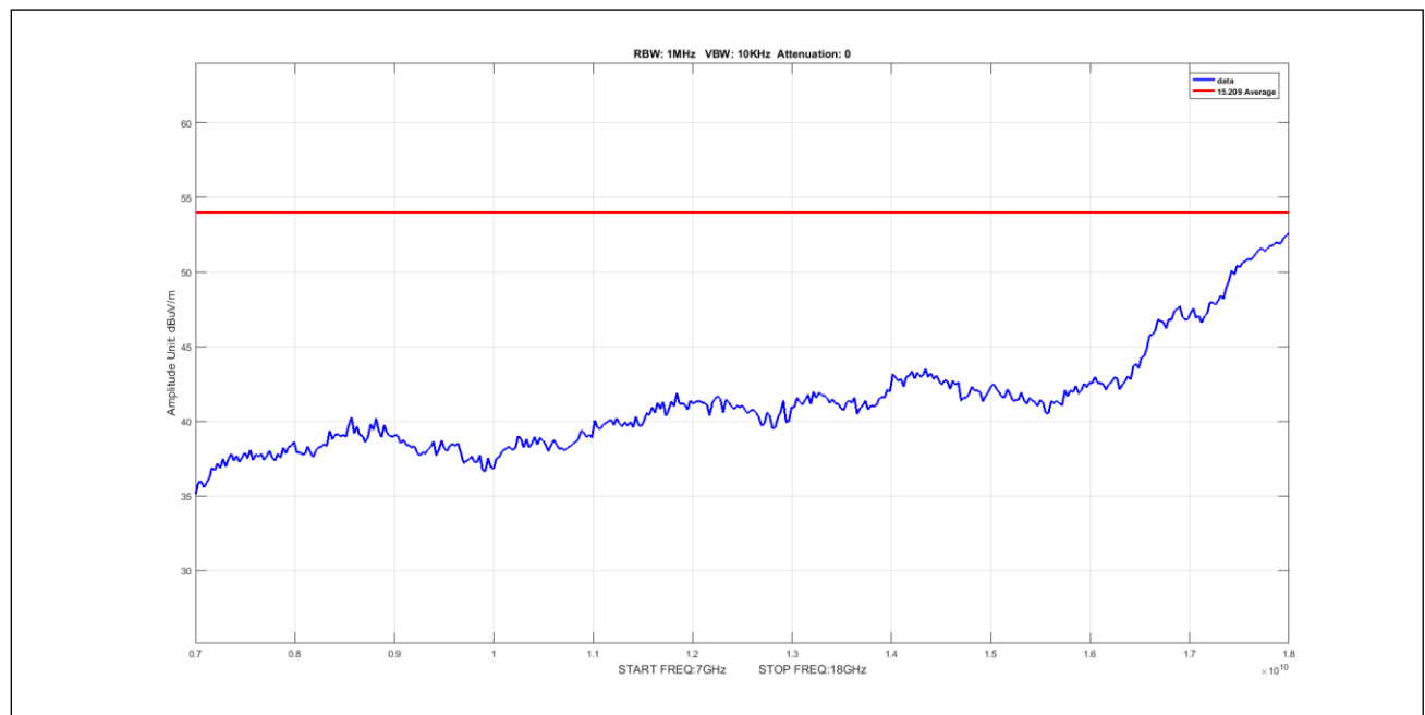
Plot 526. Undesirable Emissions, 50mni Avg 7-18GHz 10M 5170 pow17
