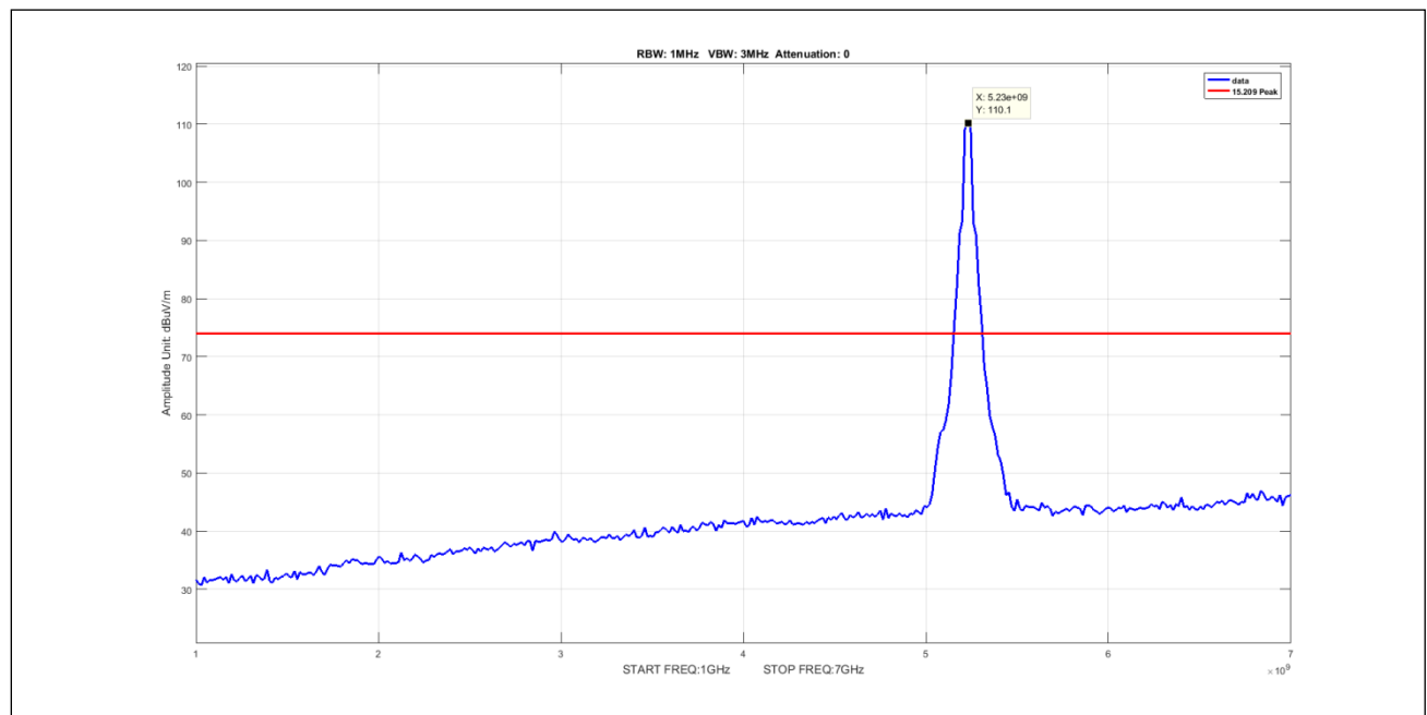
Plot 546. Undesirable Emissions, 5Omni Peak 1-7GHz 40M 5230 pow22
