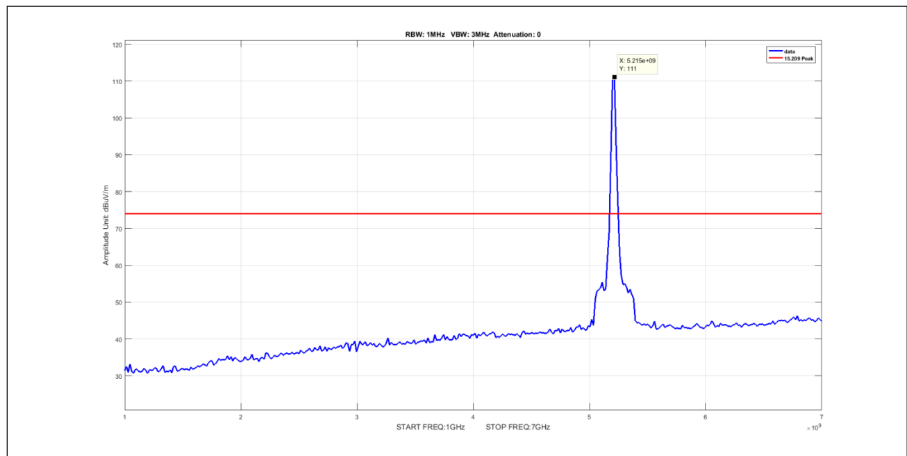
Plot 542. Undesirable Emissions, 50mni Peak 1-7GHz 20M 5210 pow19
