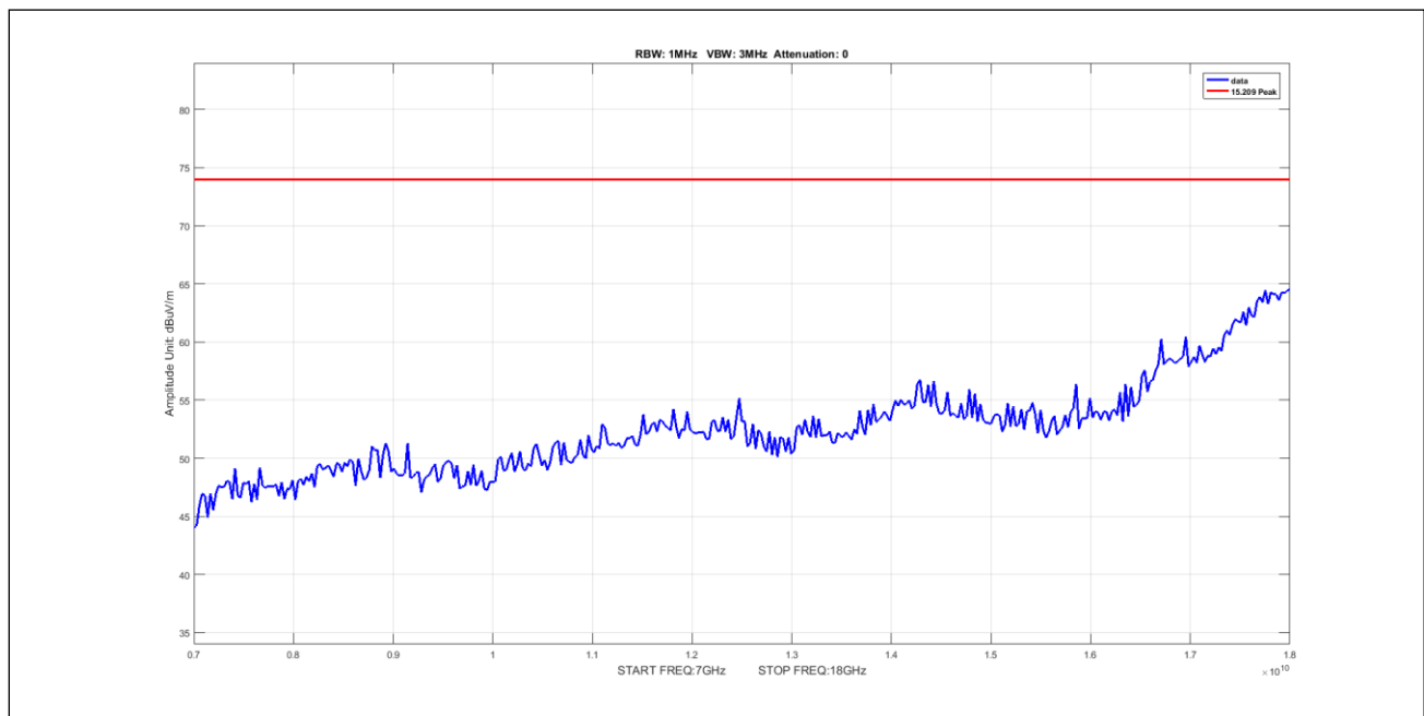
Plot 558. Undesirable Emissions, 5Omni Peak 7-18GHz 40M 5230 pow22
