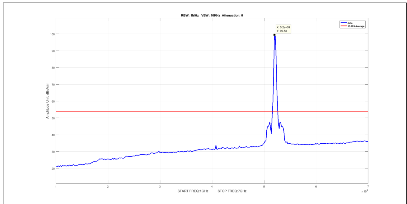
Plot 516. Undesirable Emissions, 50mni Avg 1-7GHz 20M 5210 pow19
