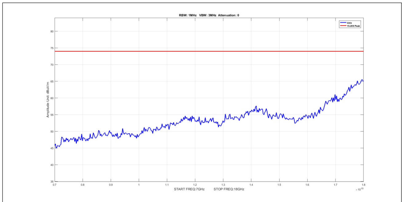
Plot 500. Undesirable Emissions, 3Para Peak 7-18GHz 10M 5170 pow-1
