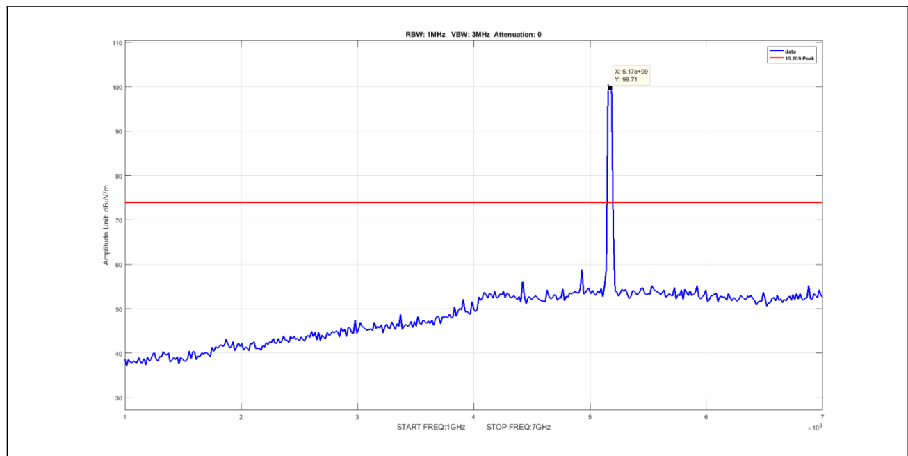
Plot 494. Undesirable Emissions, 3Para Peak 1-7GHz 40M 5171 pow-10
