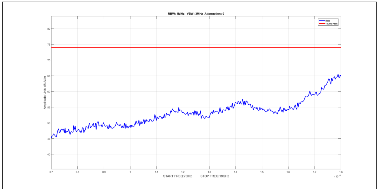
Plot 501. Undesirable Emissions, 3Para Peak 7-18GHz 10M 5210 pow3
