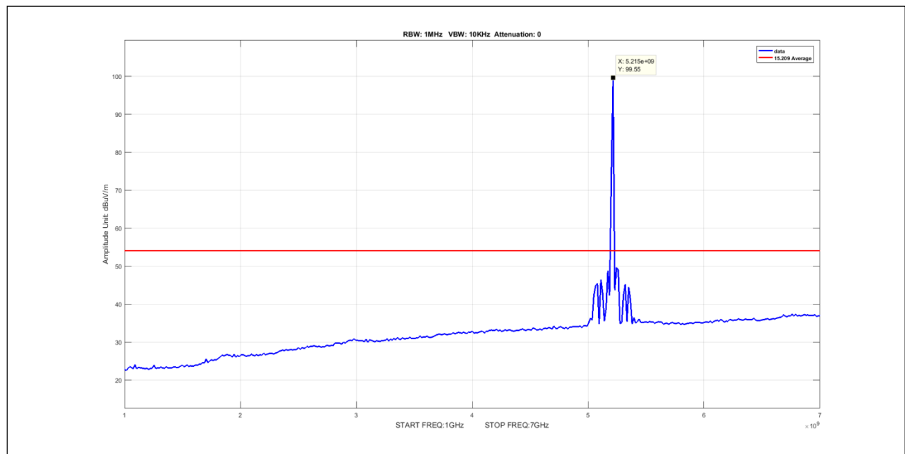
Plot 560. Undesirable Emissions, 8Omni Avg 1-7GHz 5M 5210 pow11
