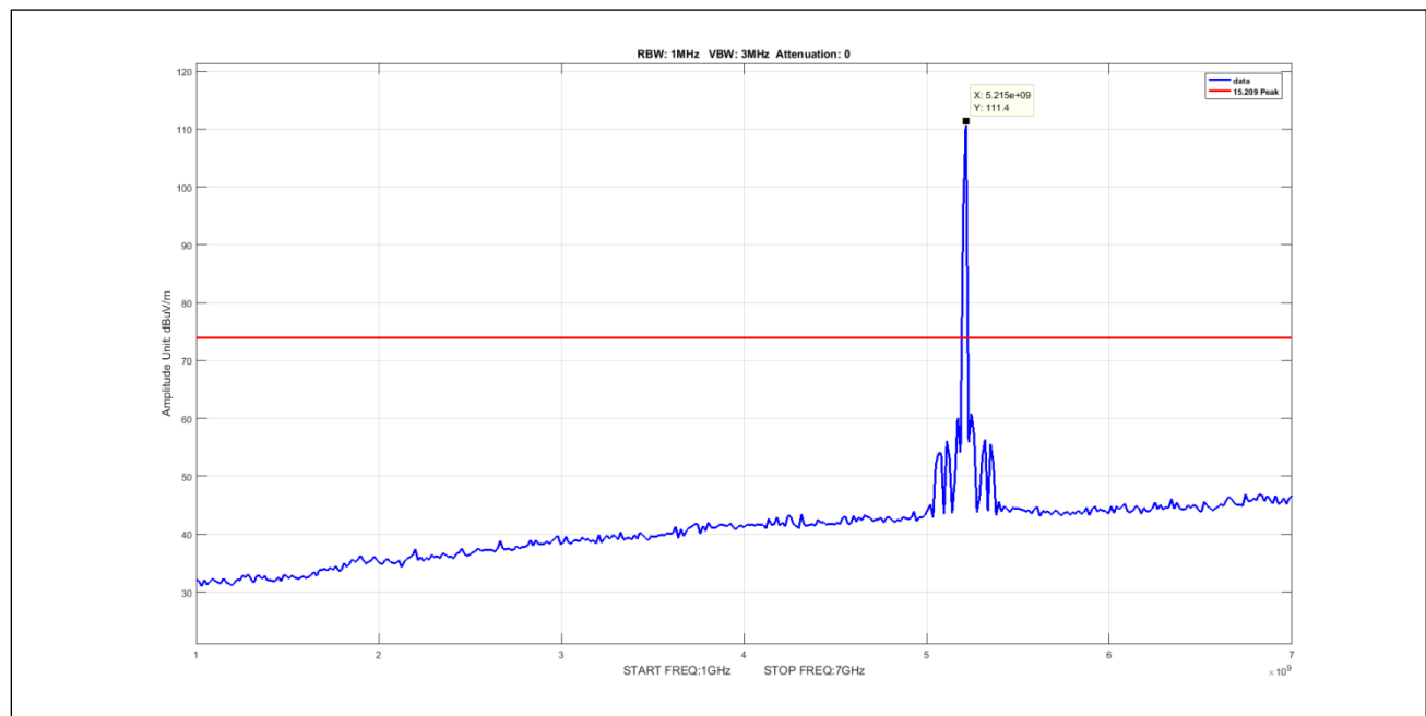
Plot 536. Undesirable Emissions, 5Omni Peak 1-7GHz 5M 5210 pow14
