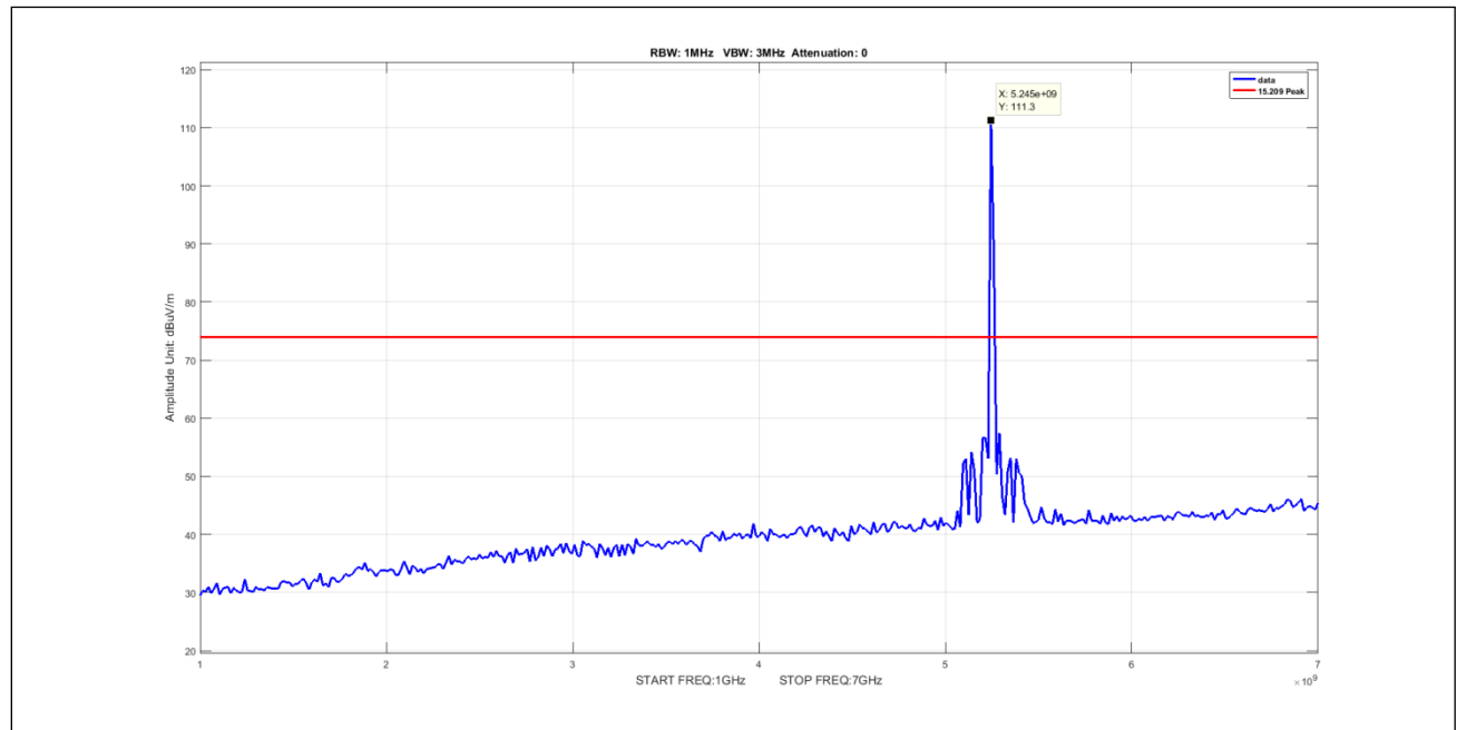
Plot 537. Undesirable Emissions, 5Omni Peak 1-7GHz 5M 5247.5 pow14
