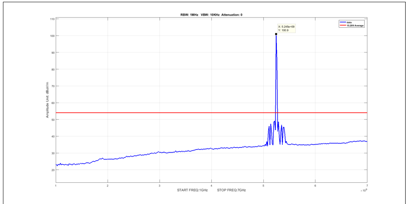
Plot 561. Undesirable Emissions, 8Omni Avg 1-7GHz 5M 5247.5 pow11
