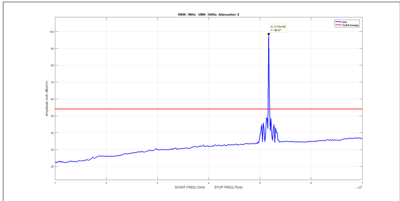
Plot 559. Undesirable Emissions, 8Omni Avg 1-7GHz 5M 5170 pow12
