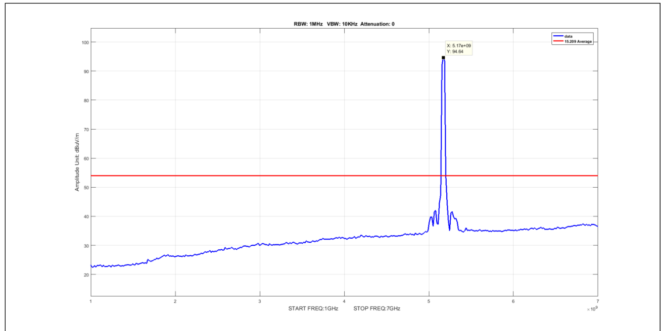
Plot 515. Undesirable Emissions, 50mni Avg 1-7GHz 20M 5170 pow10
