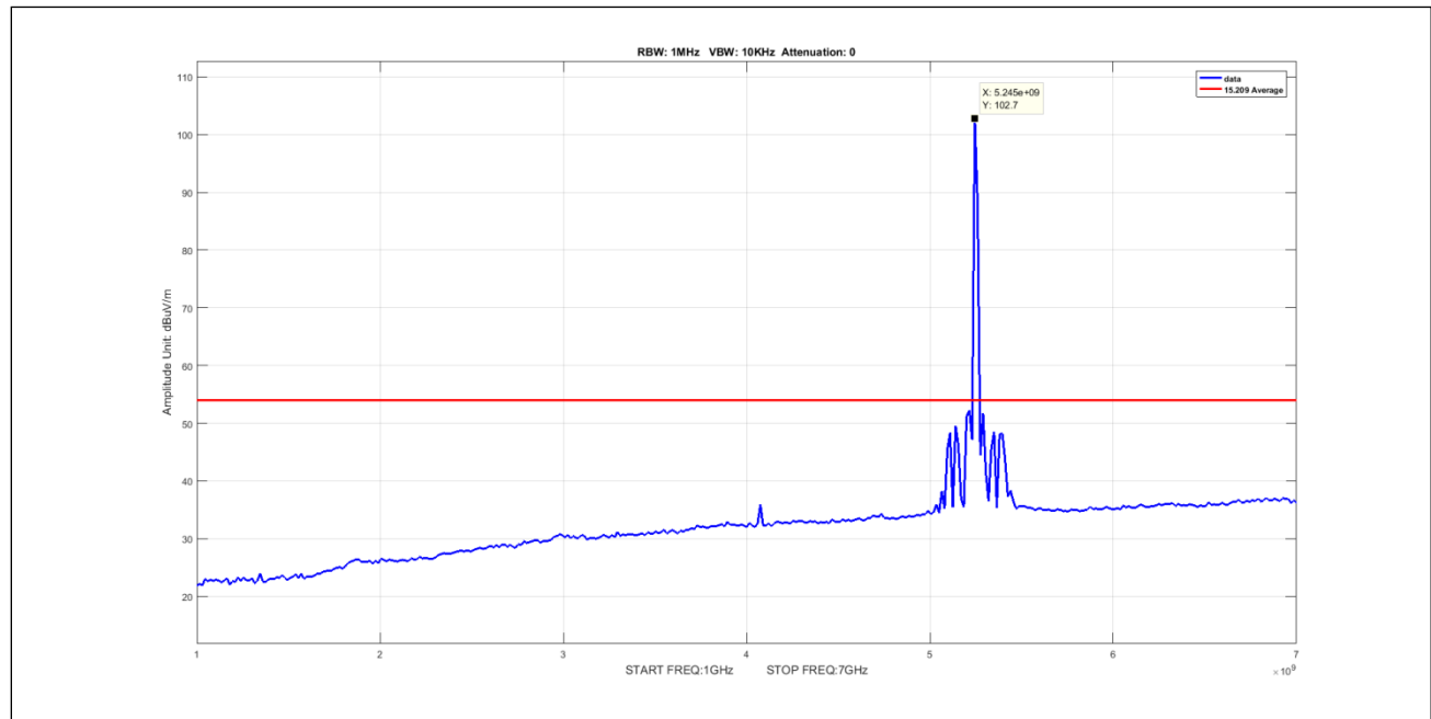
Plot 511. Undesirable Emissions, 50mni Avg 1-7GHz 5M 5247.5 pow14
