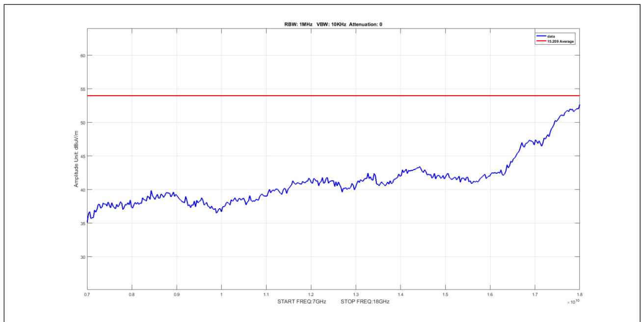
Plot 528. Undesirable Emissions, 50mni Avg 7-18GHz 10M 5245 pow17
