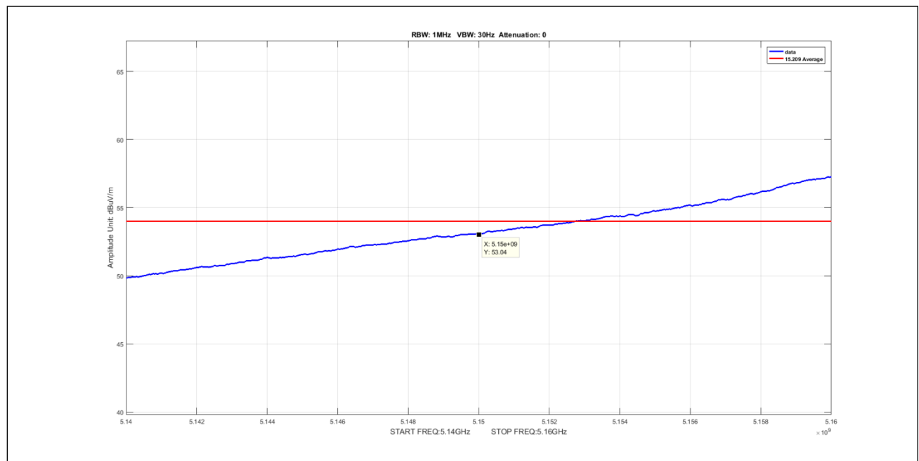
Plot 520. Undesirable Emissions, 50mni Avg 1-7GHz 40M 5210 pow21 zoom
