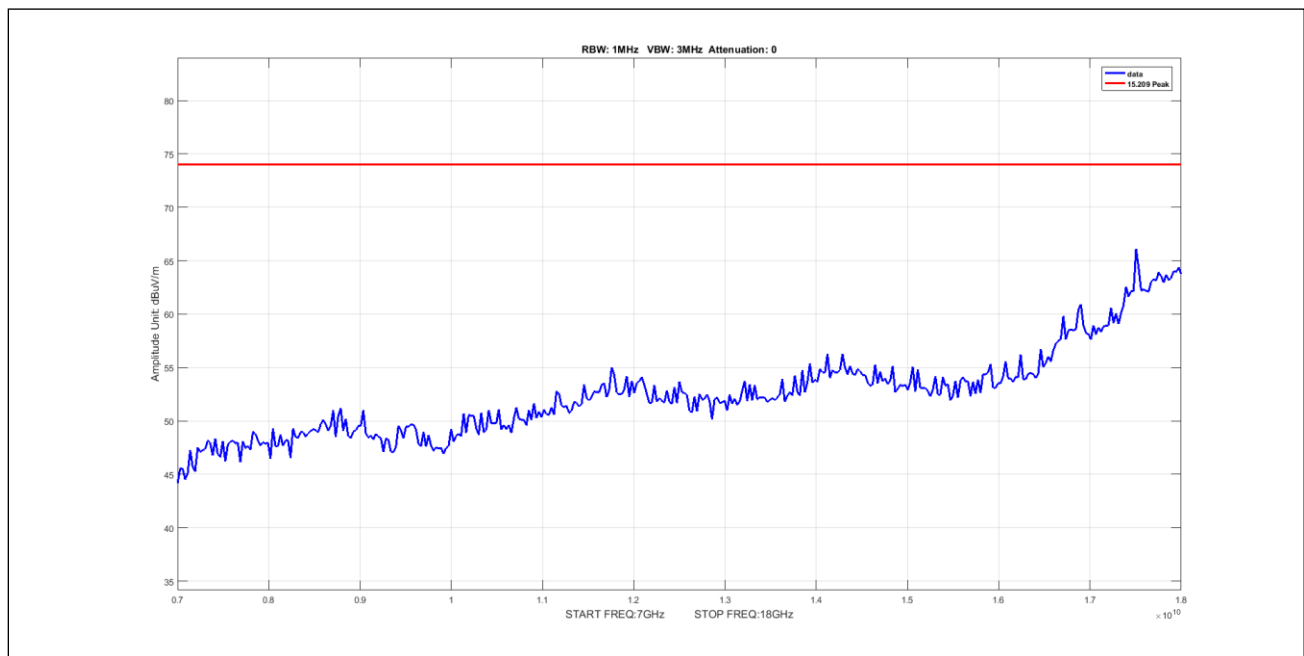
Plot 552. Undesirable Emissions, 5Omni Peak 7-18GHz 10M 5245 pow17
