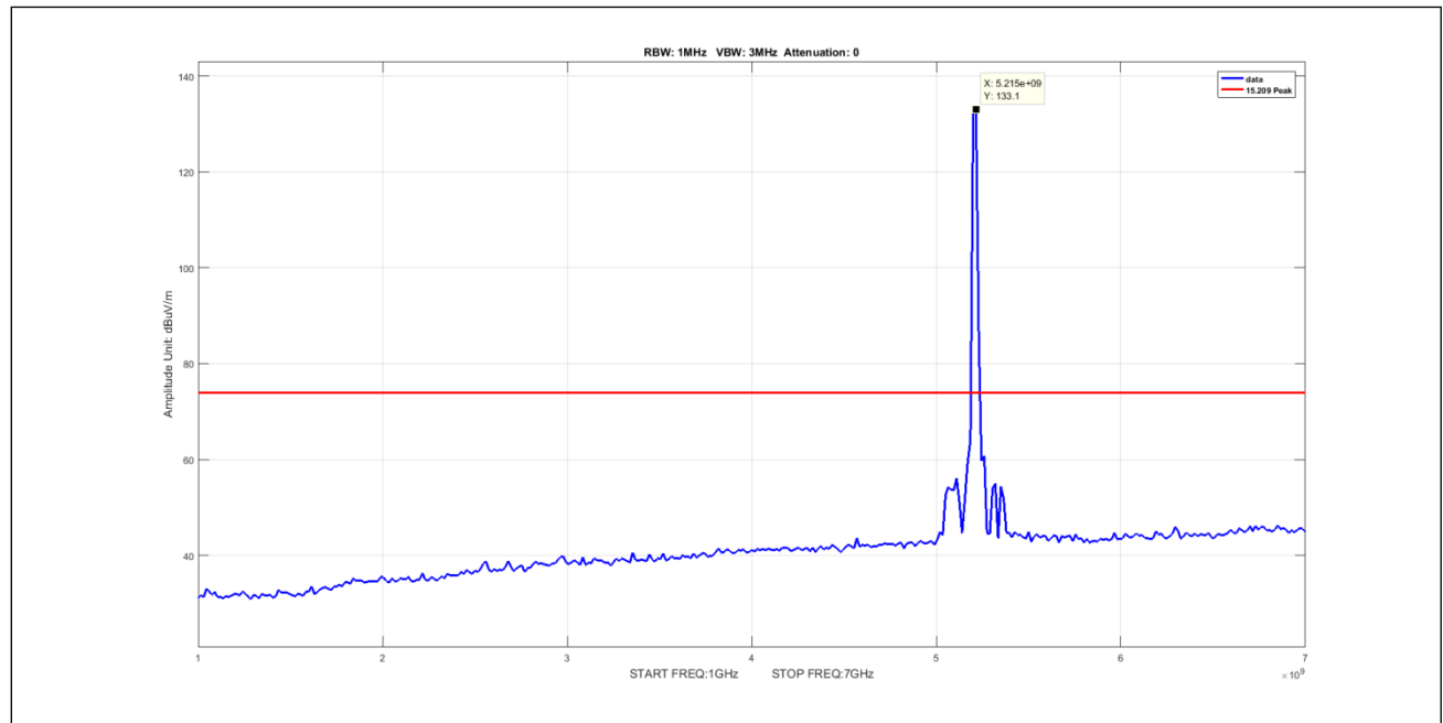
Plot 539. Undesirable Emissions, 5Omni Peak 1-7GHz 10M 5210 pow17
