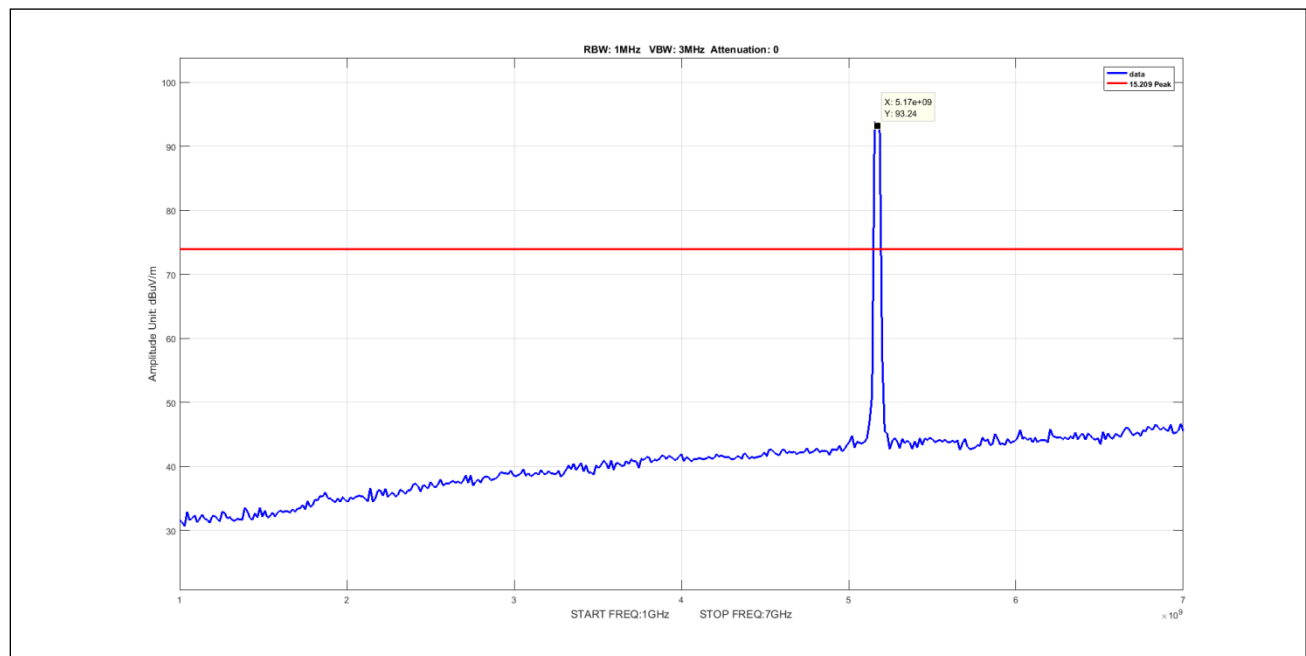
Plot 544. Undesirable Emissions, 5Omni Peak 1-7GHz 40M 5170 pow3
