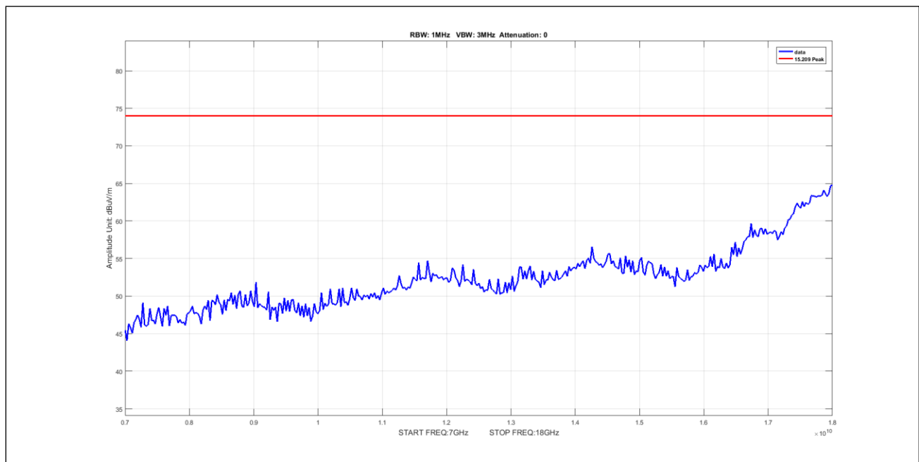
Plot 554. Undesirable Emissions, 5Omni Peak 7-18GHz 20M 5210 pow19
