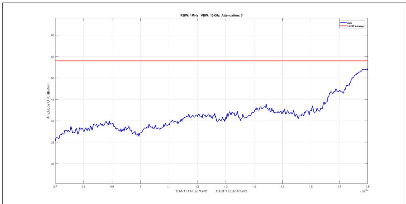
Plot 530. Undesirable Emissions, 50mni Avg 7-18GHz 20M 5210 pow19
