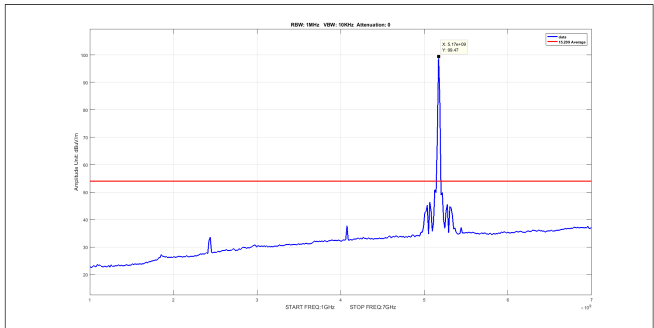
Plot 562. Undesirable Emissions, 8Omni Avg 1-7GHz 10M 5170 pow15
