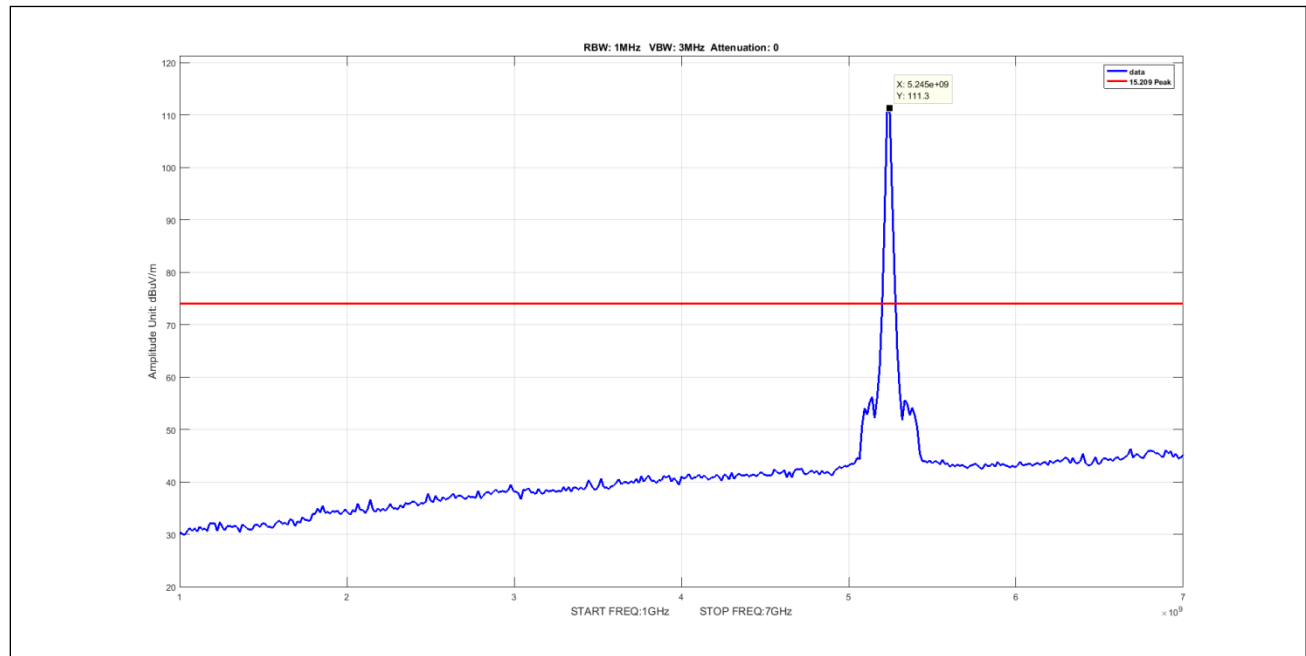
Plot 543. Undesirable Emissions, 5Omni Peak 1-7GHz 20M 5230 pow20
