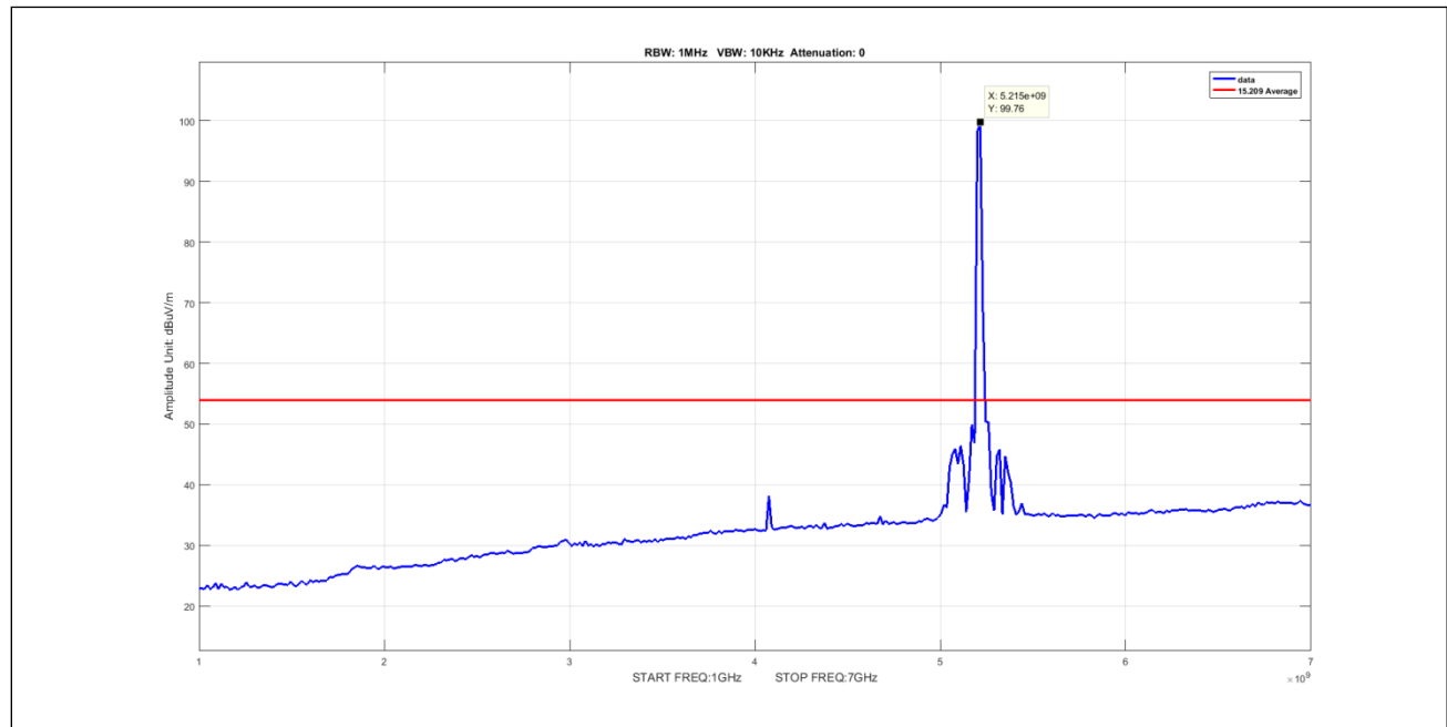
Plot 563. Undesirable Emissions, 8Omni Avg 1-7GHz 10M 5210 pow15
