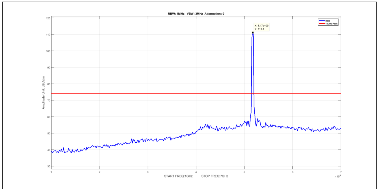
Plot 491. Undesirable Emissions, 3Para Peak 1-7GHz 20M 5170 pow-1
