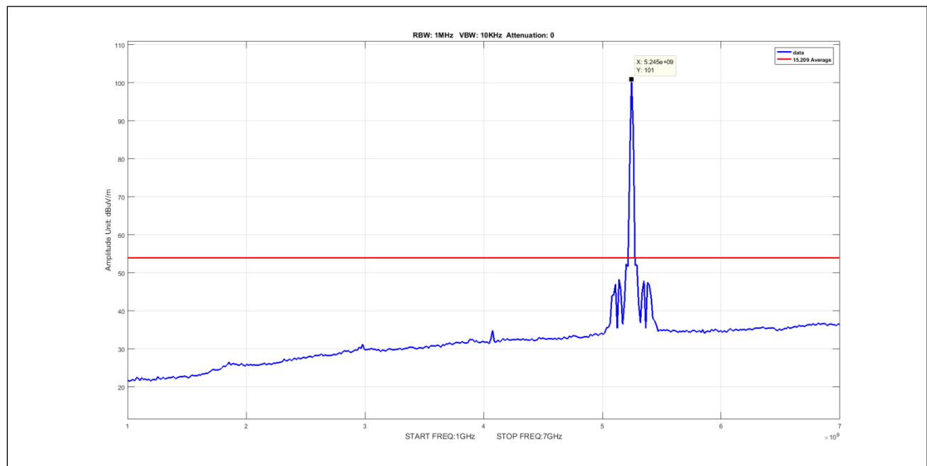
Plot 514. Undesirable Emissions, 5Omni Avg 1-7GHz 10M 5245 pow17
