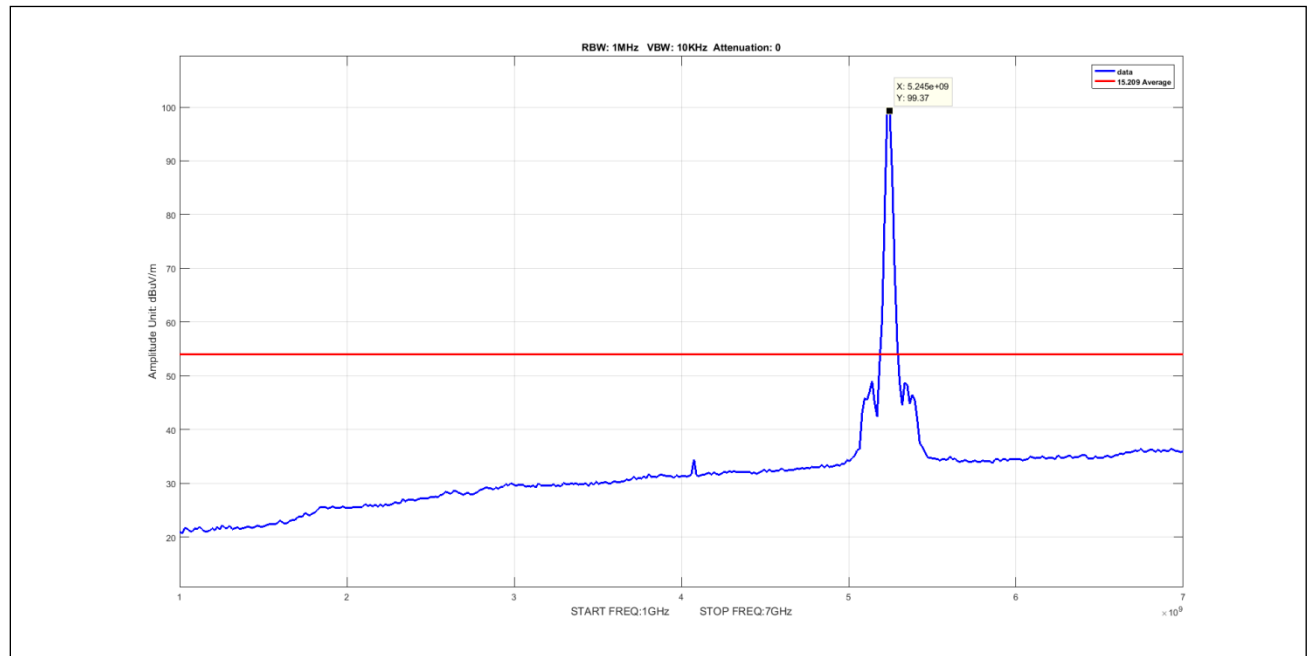
Plot 517. Undesirable Emissions, 50mni Avg 1-7GHz 20M 5240 pow20
