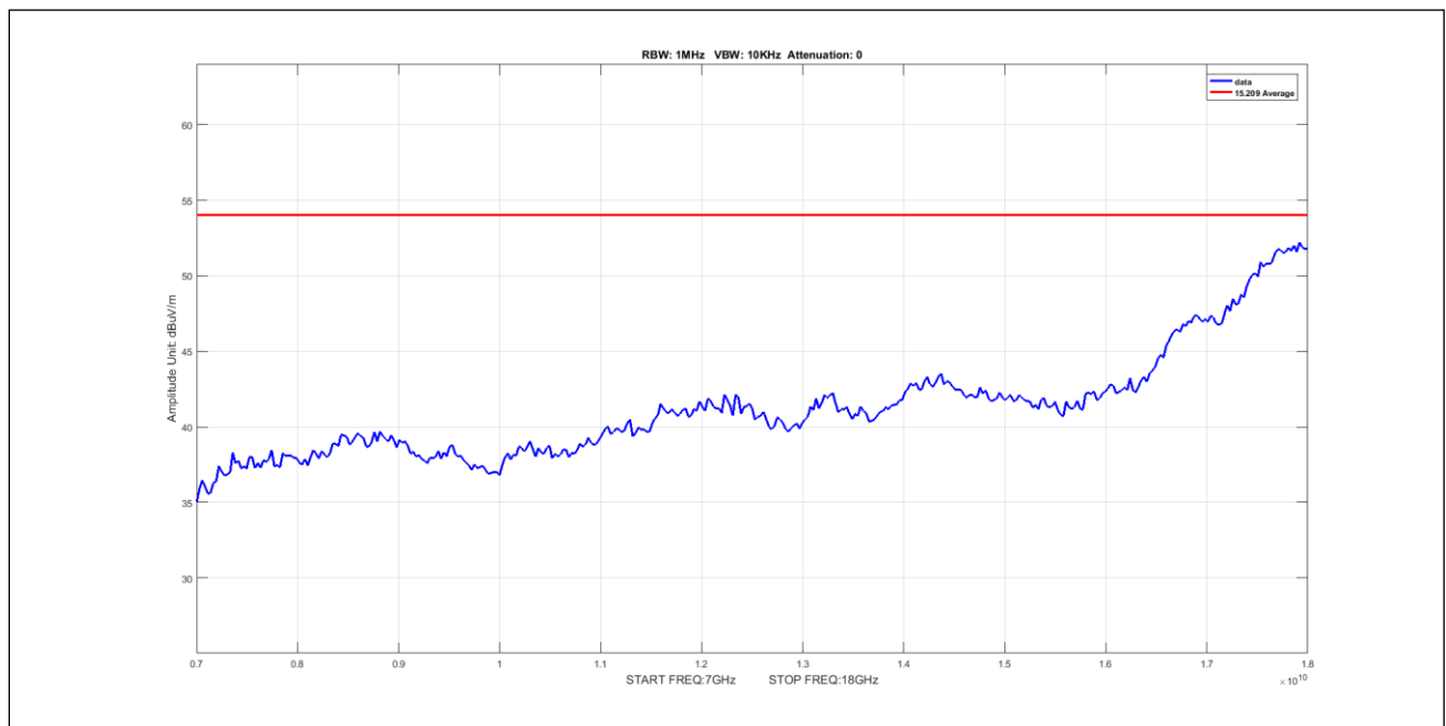
Plot 532. Undesirable Emissions, 50mni Avg 7-18GHz 40M 5170 pow3
