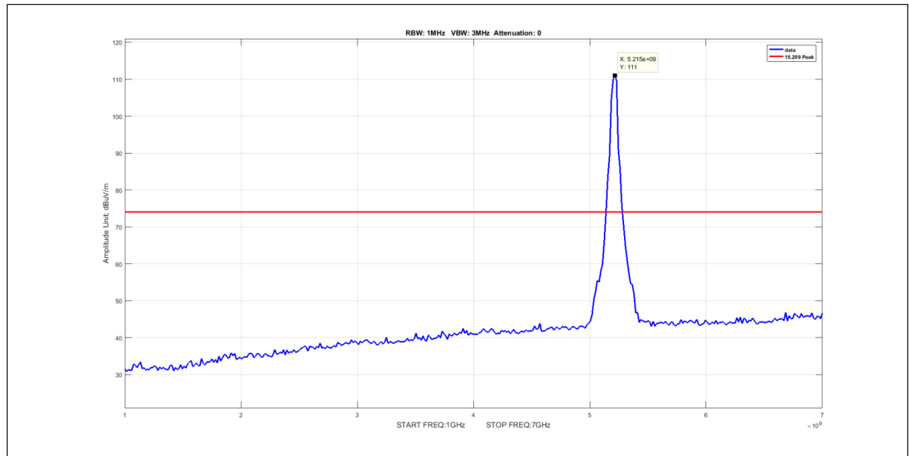
Plot 545. Undesirable Emissions, 5Omni Peak 1-7GHz 40M 5210 pow21
