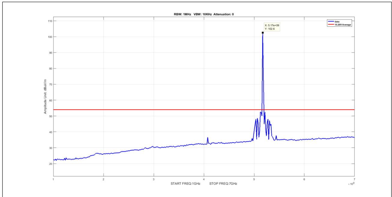
Plot 509. Undesirable Emissions, 50mni Avg 1-7GHz 5M 5170 pow14
