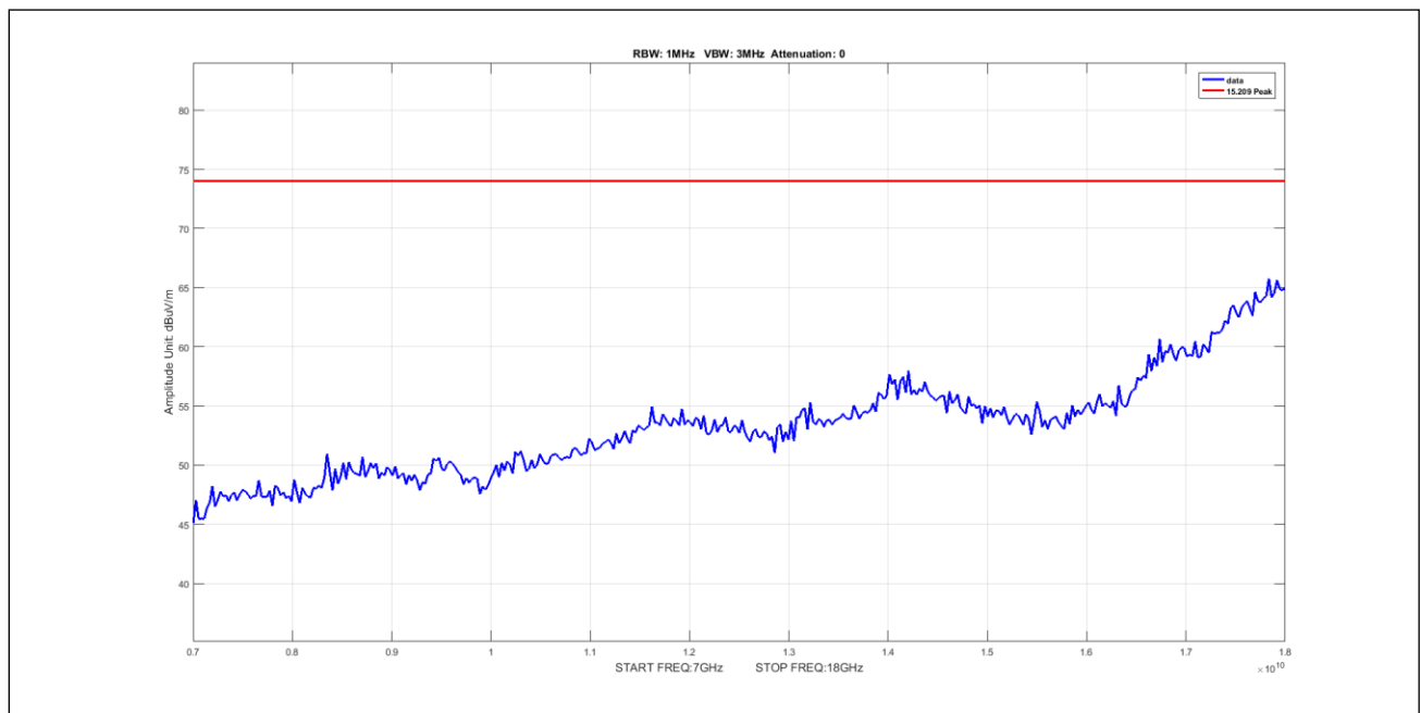
Plot 502. Undesirable Emissions, 3Para Peak 7-18GHz 10M 5240.5 pow3
