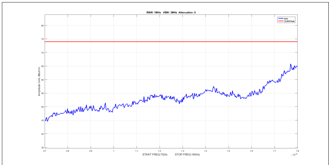
Plot 498. Undesirable Emissions, 3Para Peak 7-18GHz 5M 5210 pow0
