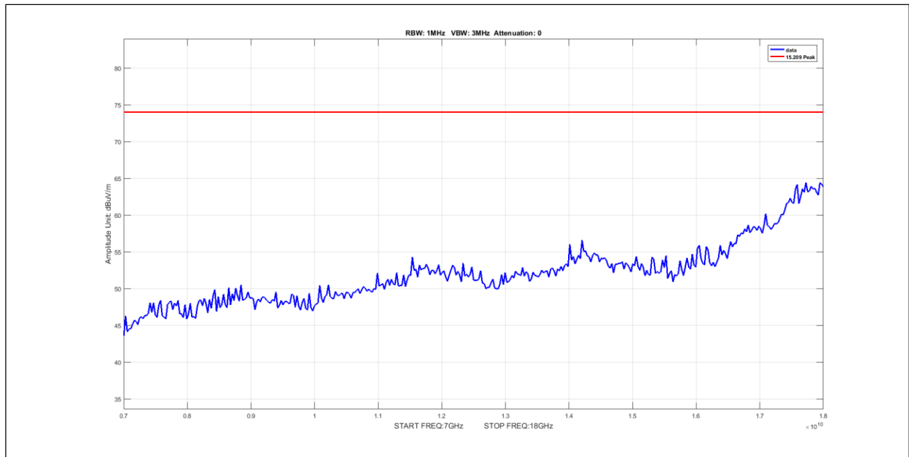
Plot 553. Undesirable Emissions, 5Omni Peak 7-18GHz 20M 5170 pow10
