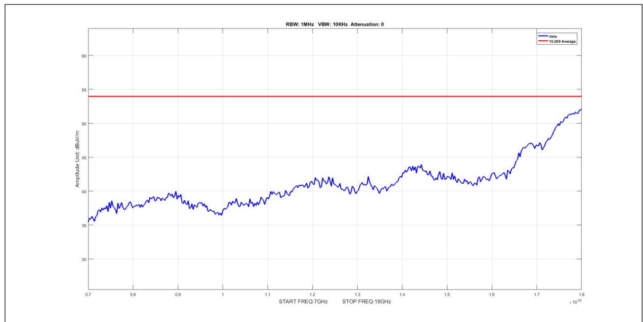
Plot 572. Undesirable Emissions, 80mni Avg 7-18GHz 5M 5170 pow12
