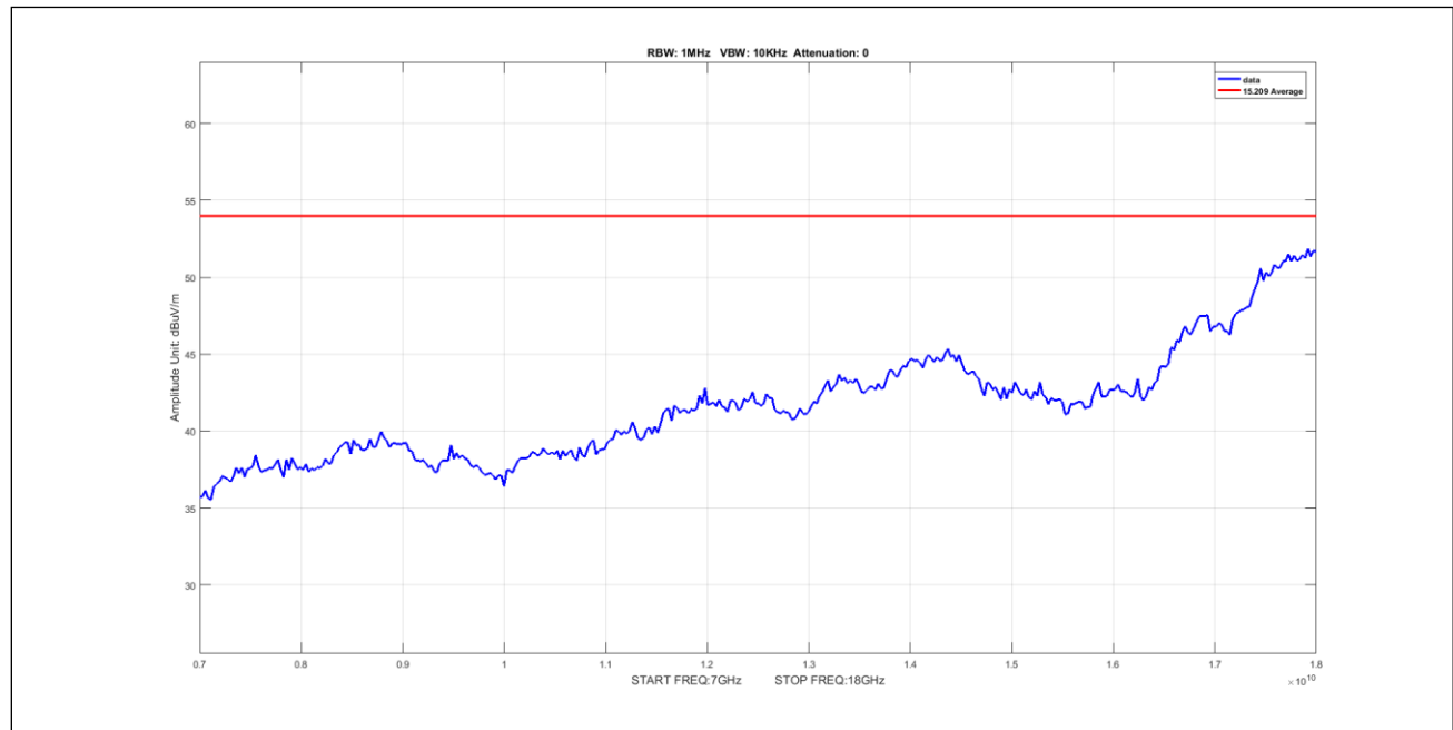
Plot 633. Undesirable Emissions, 90Sector Avg 7-18GHz 40M 5230 pow16
