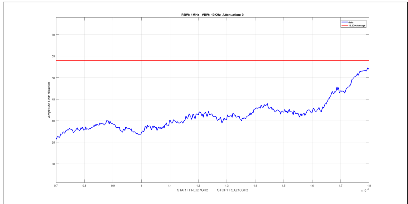
Plot 575. Undesirable Emissions, 8Omni Avg 7-18GHz 10M 5170 pow15
