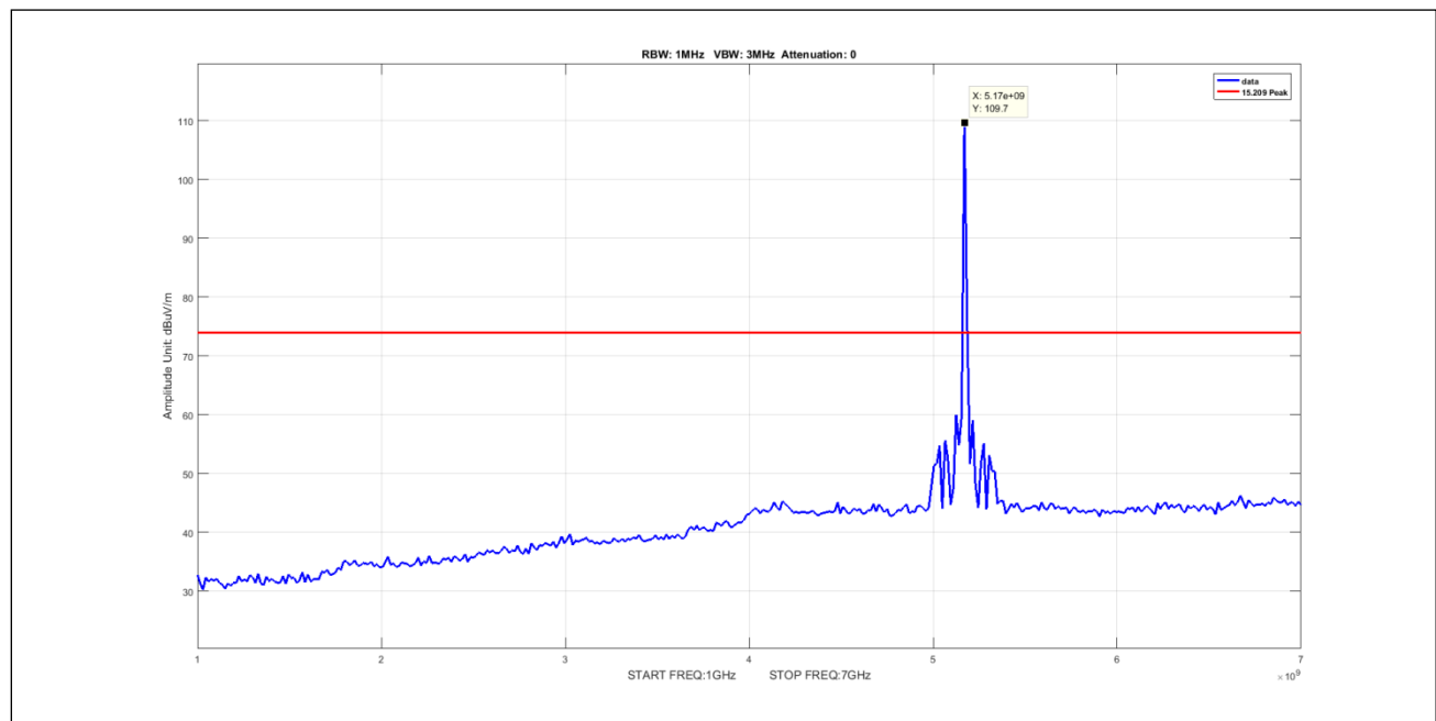
Plot 634. Undesirable Emissions, 90Sector Peak 1-7GHz 5M 5170 pow7
