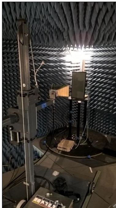
Photograph 12. Undesirable Emissions, 90 Sector above 1 GHz, Test Setup
