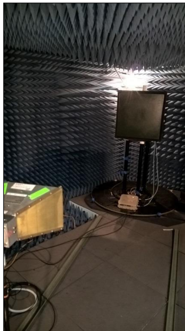
Photograph 4. Undesirable Emissions, 2' Panel above 1 GHz, Test Setup
