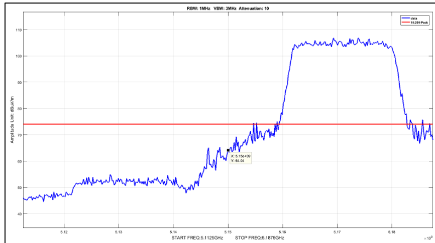
Plot 749. Radiated Band Edge, 5 Omni, Peak, 20M, 5170, pow10
