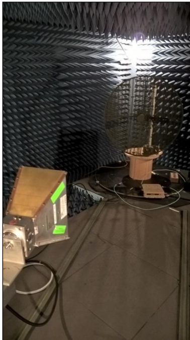
Photograph 6. Undesirable Emissions, Para above 1 GHz, Test Setup
