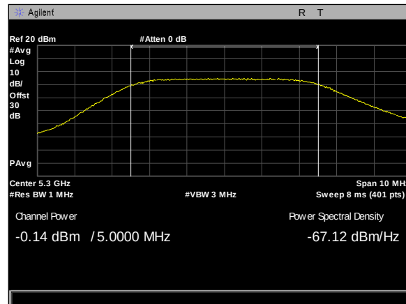
Plot 284. Maximum Conducted Output Power, 90Sector, 5M, 5300M, rf2
