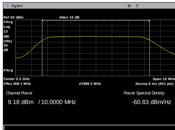
Plot 247. Maximum Conducted Output Power, 80Mni, 10M, 5300M, rf1
