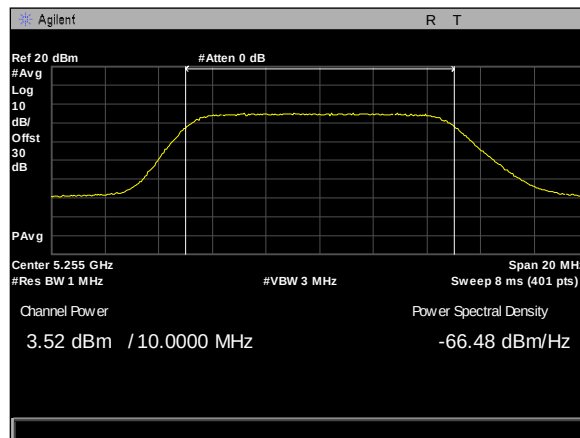
Plot 294. Maximum Conducted Output Power, 90Sector, 10M, 5255M, rf1
