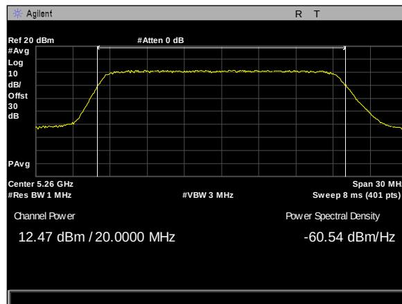
Plot 258. Maximum Conducted Output Power, 80mni, 20M, 5260M, rf2
