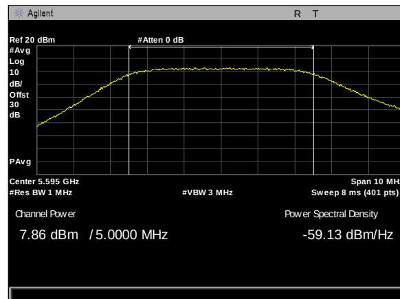
Plot 241. Maximum Conducted Output Power, 8Omni, 5M, 5595M, rf1
