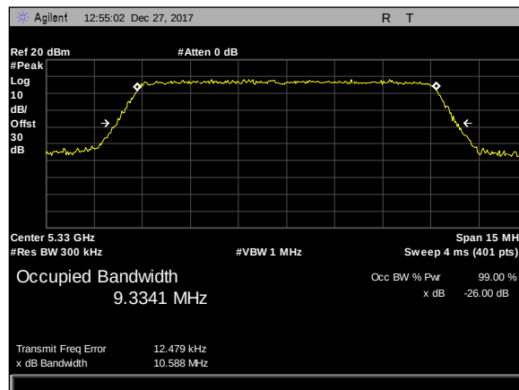
Plot 62. 26 dB Occupied Bandwidth, 5Omni, 10M, 5330M, rf2
