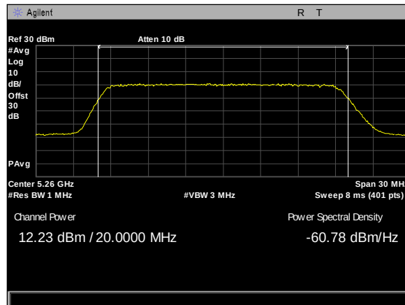
Plot 257. Maximum Conducted Output Power, 80mni, 20M, 5260M, rf1
