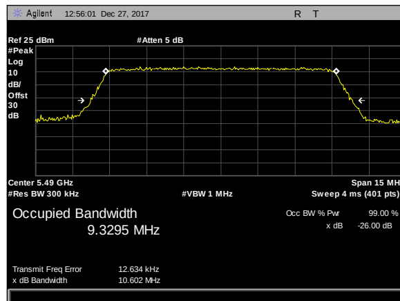
Plot 63. 26 dB Occupied Bandwidth, 5Omni, 10M, 5490M, rf2
