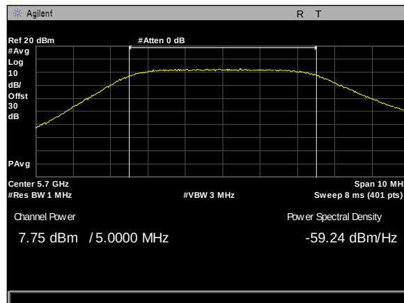
Plot 244. Maximum Conducted Output Power, 8Omni, 5M, 5700M, rf2
