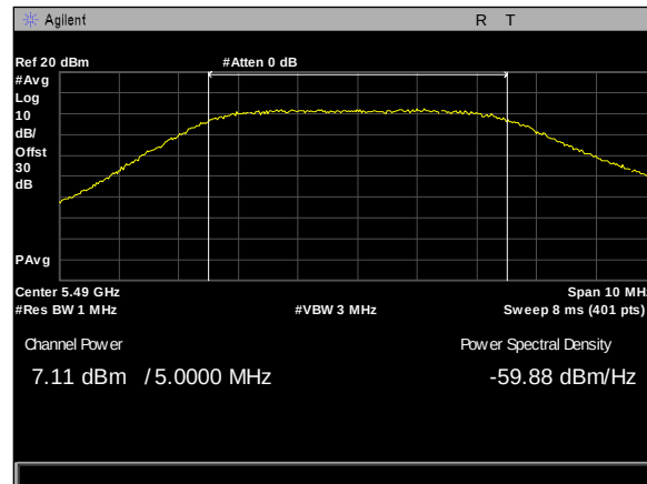
Plot 239. Maximum Conducted Output Power, 8Omni, 5M, 5490M, rf1
