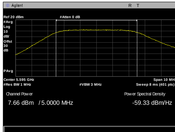
Plot 242. Maximum Conducted Output Power, 8Omni, 5M, 5595M, rf2
