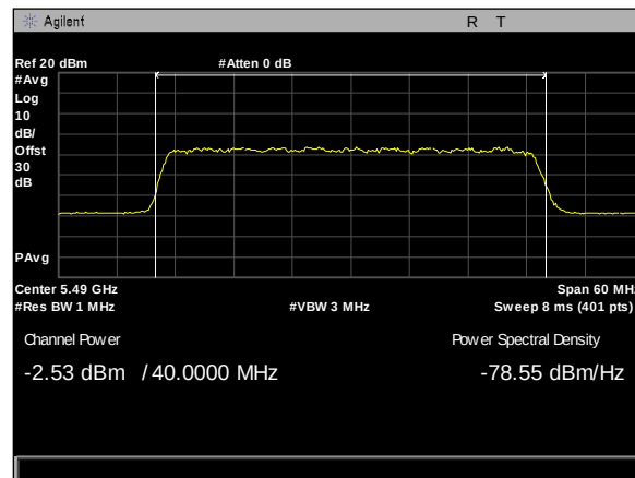
Plot 324. Maximum Conducted Output Power, 90Sector, 40M, 5490M, rf1
