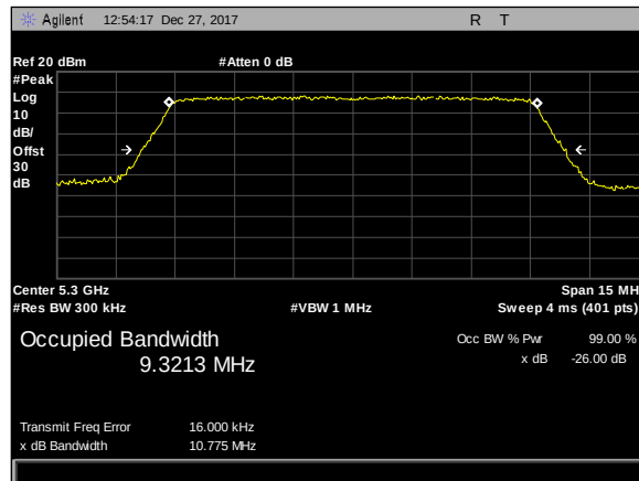
Plot 61. 26 dB Occupied Bandwidth, 5Omni, 10M, 5300M, rf2
