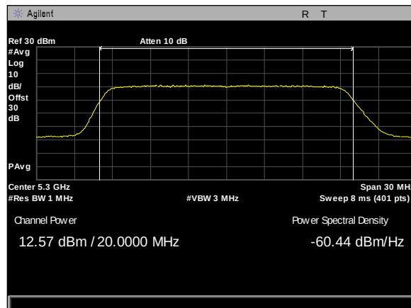
Plot 259. Maximum Conducted Output Power, 80mni, 20M, 5300M, rf1
