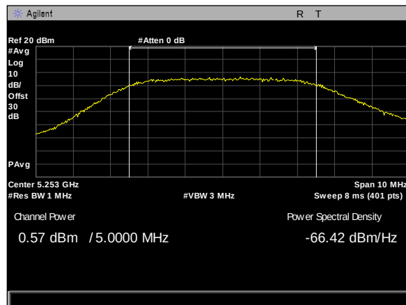
Plot 282. Maximum Conducted Output Power, 90Sector, 5M, 5252.5M, rf2
