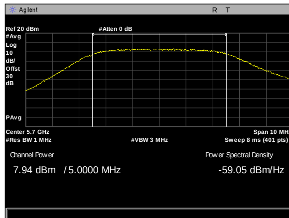
Plot 243. Maximum Conducted Output Power, 8Omni, 5M, 5700M, rf1
