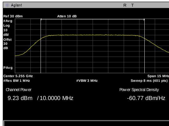
Plot 245. Maximum Conducted Output Power, 80Mni, 10M, 5255M, rf1
