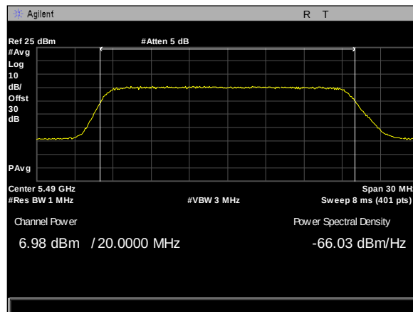
Plot 312. Maximum Conducted Output Power, 90Sector, 20M, 5490M, rf1
