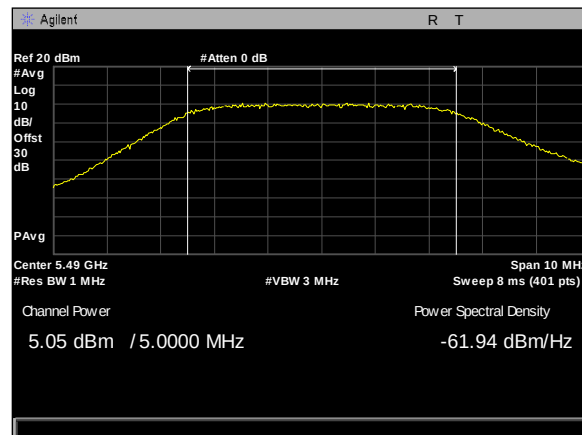
Plot 240. Maximum Conducted Output Power, 8Omni, 5M, 5490M, rf2
