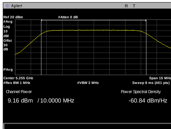
Plot 246. Maximum Conducted Output Power, 80Mni, 10M, 5255M, rf2
