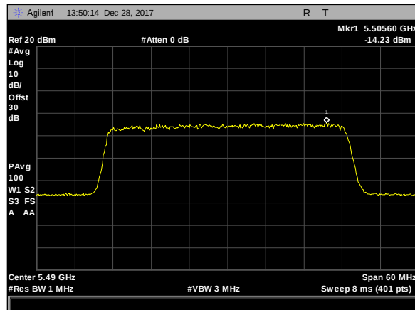
Plot 526. Power Spectral Density, 8Omni, 40M, 5490M, rf1
