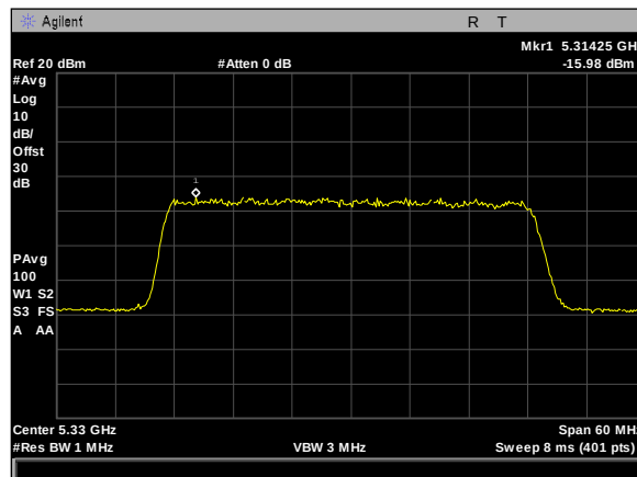
Plot 524. Power Spectral Density, 8Omni, 40M, 5330M, rf1
