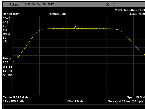
Plot 457. Power Spectral Density, 5Omni, 10M, 5595M, rf2
