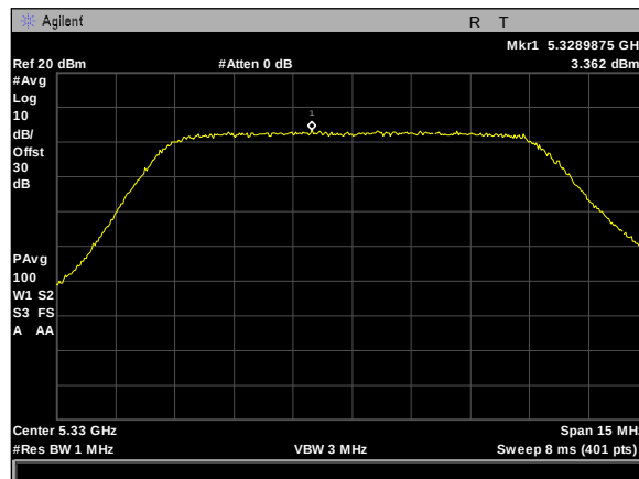
Plot 453. Power Spectral Density, 5Omni, 10M, 5330M, rf2
