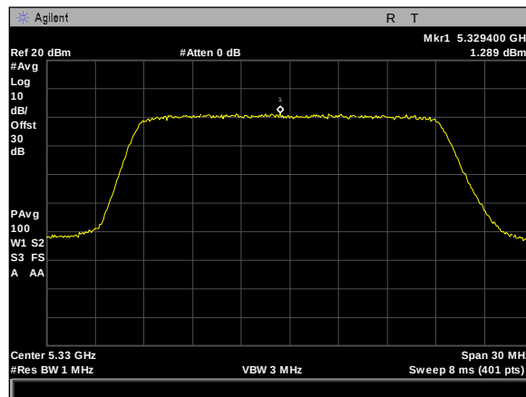
Plot 464. Power Spectral Density, 5Omni, 20M, 5330M, rf1
