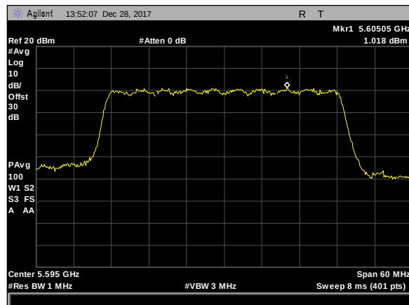
Plot 528. Power Spectral Density, 8Omni, 40M, 5595M, rf1
