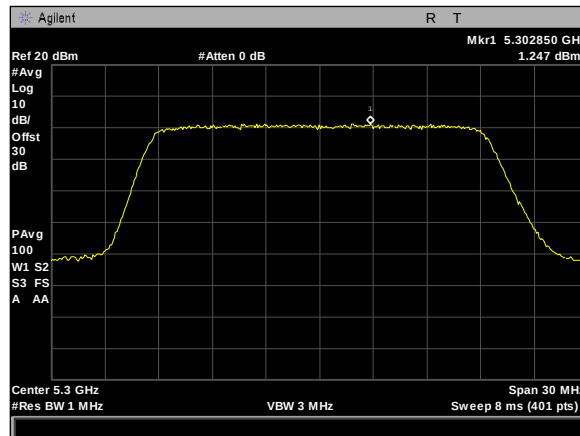
Plot 511. Power Spectral Density, 80Omni, 20M, 5300M, rf2
