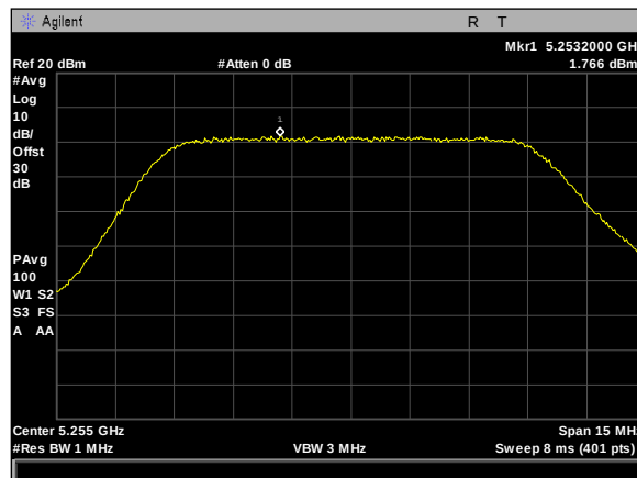
Plot 497. Power Spectral Density, 80MHz, 10M, 5253M, rf2
