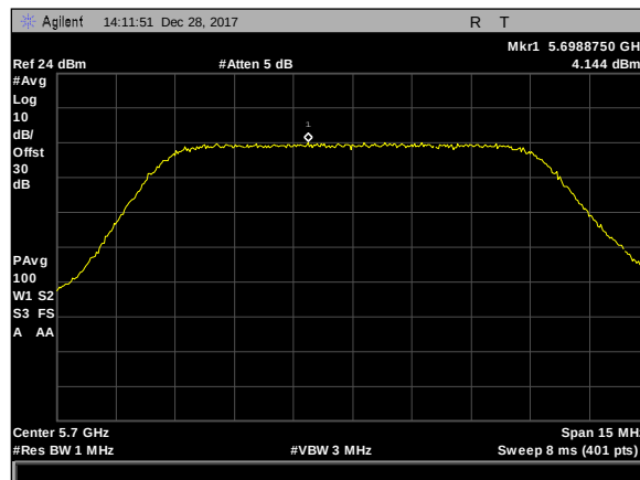
Plot 458. Power Spectral Density, 5Omni, 10M, 5700M, rf1
