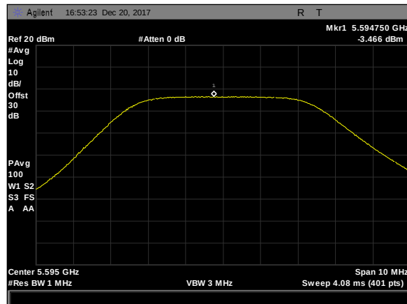
Plot 541. Power Spectral Density, 90Sector, 5M, 5595M, rf1
