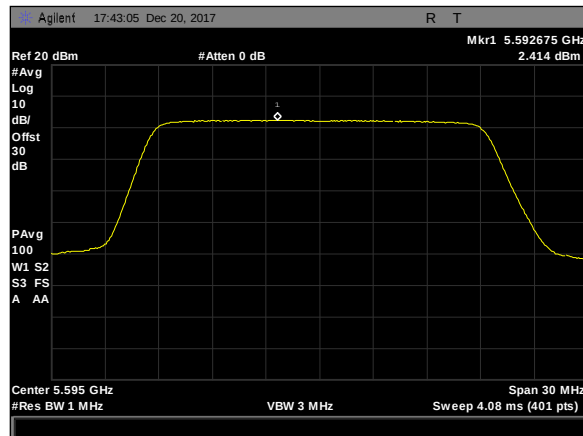
Plot 517. Power Spectral Density, 8Omni, 20M, 5595M, rf2
