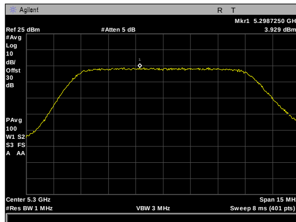
Plot 450. Power Spectral Density, 5Omni, 10M, 5300M, , rf1
