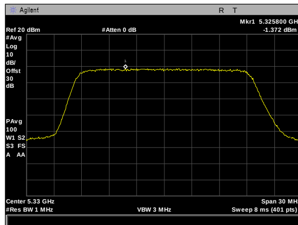
Plot 512. Power Spectral Density, 80Omni, 20M, 5330M, rf1
