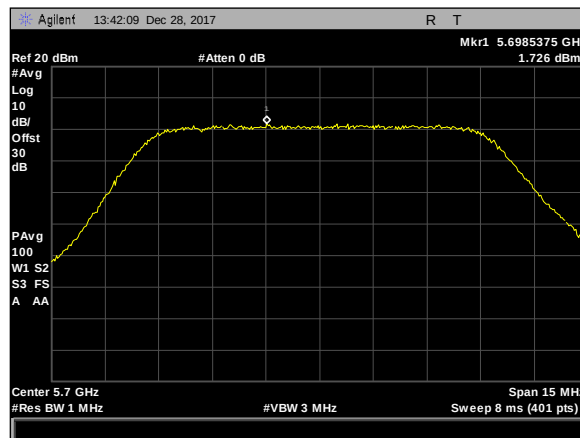
Plot 506. Power Spectral Density, 80Omni, 10M, 5700M, rf1
