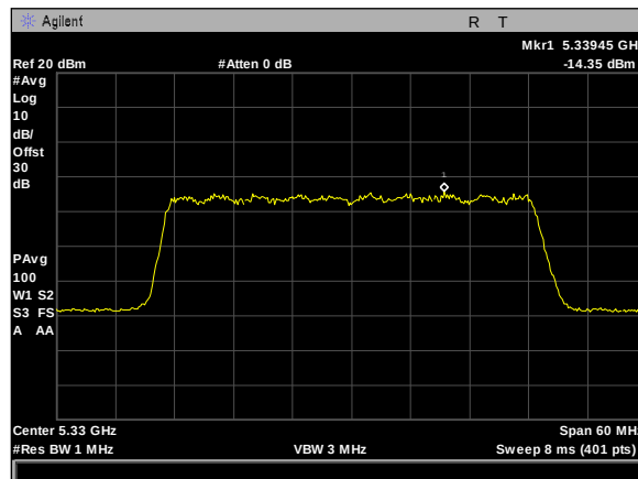
Plot 525. Power Spectral Density, 8Omni, 40M, 5330M, rf2
