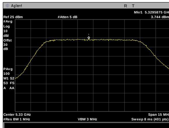
Plot 452. Power Spectral Density, 5Omni, 10M, 5330M, rf1
