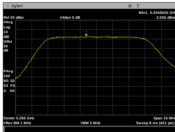
Plot 449. Power Spectral Density, 5Omni, 10M, 5255M, rf2
