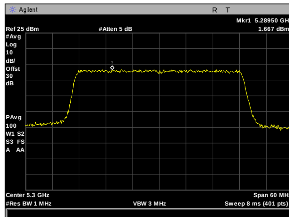
Plot 522. Power Spectral Density, 8Omni, 40M, 5300M, rf1
