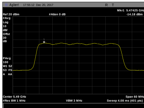
Plot 527. Power Spectral Density, 8Omni, 40M, 5490M, rf2
