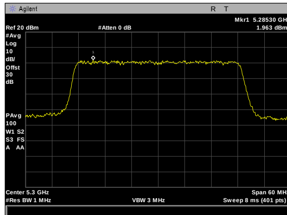
Plot 523. Power Spectral Density, 8Omni, 40M, 5300M, rf2
