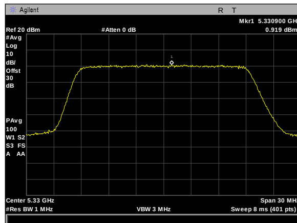
Plot 465. Power Spectral Density, 5Omni, 20M, 5330M, rf2
