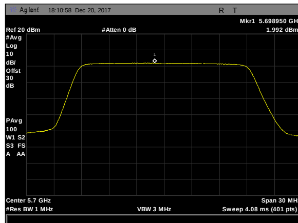
Plot 471. Power Spectral Density, 5Omni, 20M, 5700M, rf2
