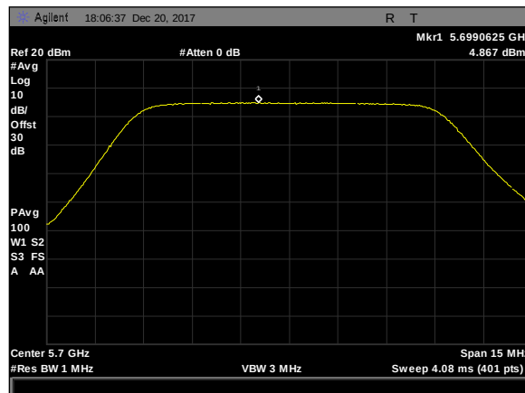
Plot 459. Power Spectral Density, 5Omni, 10M, 5700M, rf2
