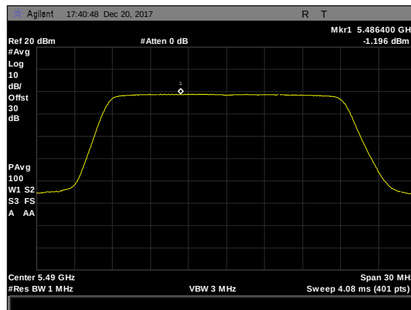
Plot 515. Power Spectral Density, 80MHz, 20M, 5490M, rf2
