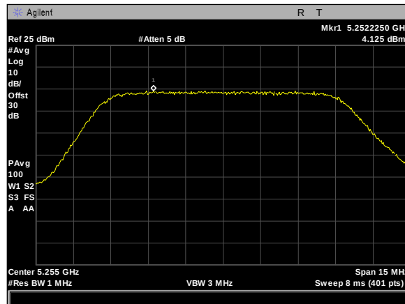
Plot 448. Power Spectral Density, 5Omni, 10M, 5255M, rf1
