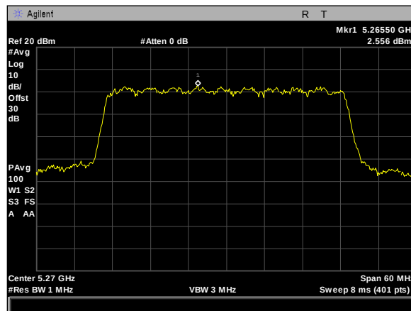
Plot 521. Power Spectral Density, 8Omni, 40M, 5270M, rf2
