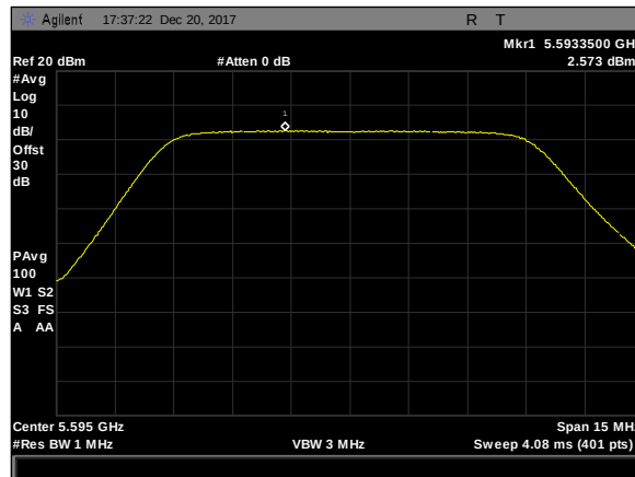
Plot 505. Power Spectral Density, 80Omni, 10M, 5595M, rf2
