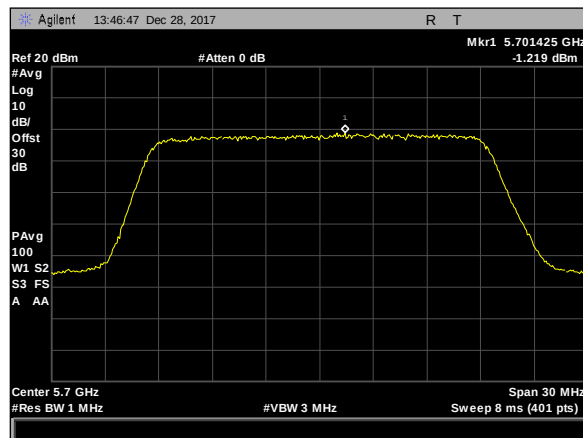
Plot 518. Power Spectral Density, 8Omni, 20M, 5700M, rf1
