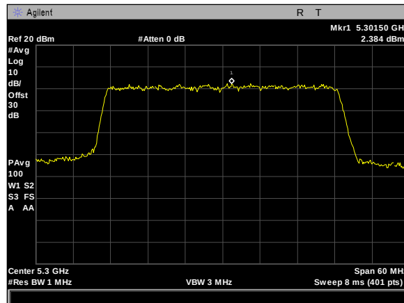
Plot 475. Power Spectral Density, 5Omni, 40M, 5300M, rf2
