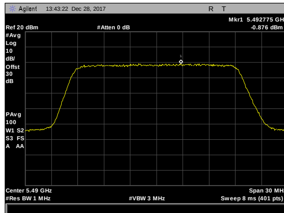
Plot 514. Power Spectral Density, 80MHz, 20M, 5490M, rf1
