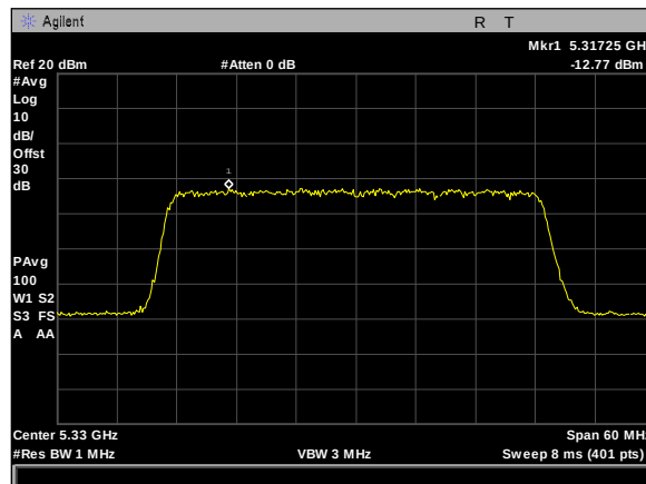
Plot 477. Power Spectral Density, 5Omni, 40M, 5330M, rf2
