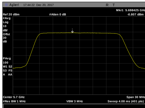
Plot 519. Power Spectral Density, 8Omni, 20M, 5700M, rf2
