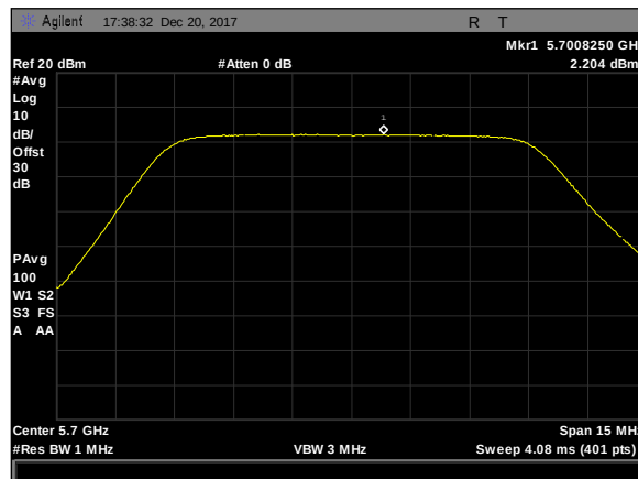
Plot 507. Power Spectral Density, 80Omni, 10M, 5700M, rf2
