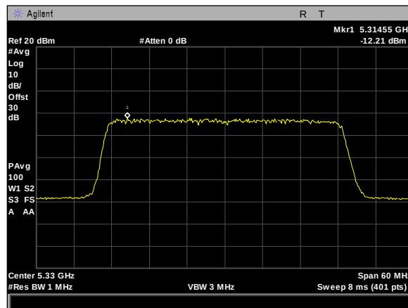
Plot 476. Power Spectral Density, 5Omni, 40M, 5330M, rf1
