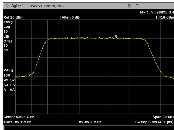
Plot 516. Power Spectral Density, 80MHz, 20M, 5595M, rf1
