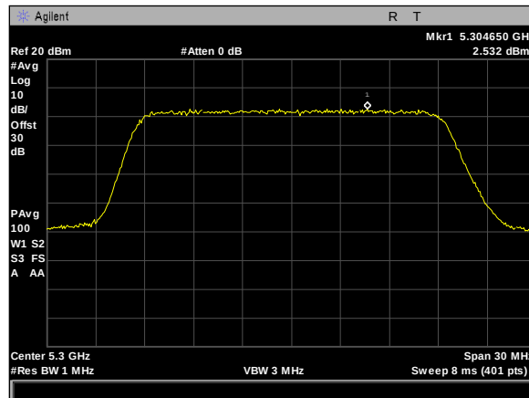
Plot 463. Power Spectral Density, 5Omni, 20M, 5300M, rf2
