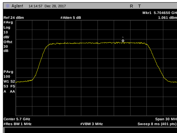
Plot 470. Power Spectral Density, 5Omni, 20M, 5700M, rf1
