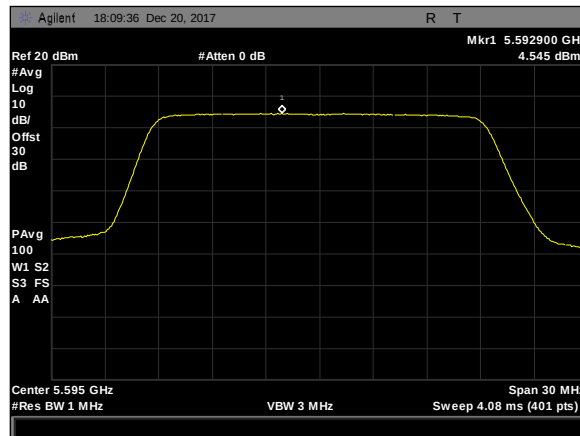
Plot 469. Power Spectral Density, 5Omni, 20M, 5595M, rf2
