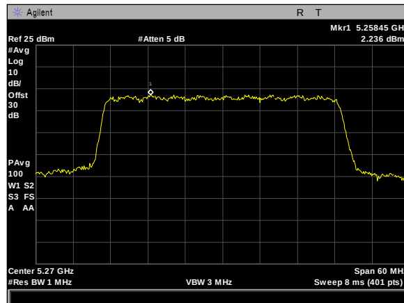
Plot 520. Power Spectral Density, 8Omni, 40M, 5270M, rf1
