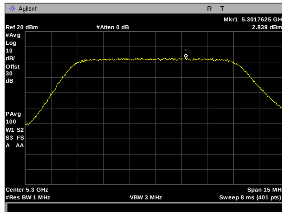
Plot 451. Power Spectral Density, 5Omni, 10M, 5300M, rf2
