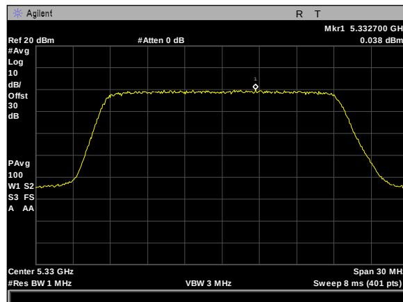
Plot 513. Power Spectral Density, 80Omni, 20M, 5330M, rf2
