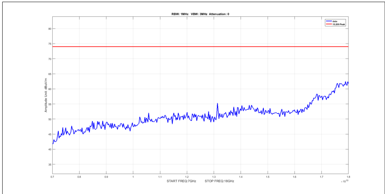
Plot 916. Undesirable Emissions, 50mni, Peak, 7-18GHz, 10M, 5255, pow11
