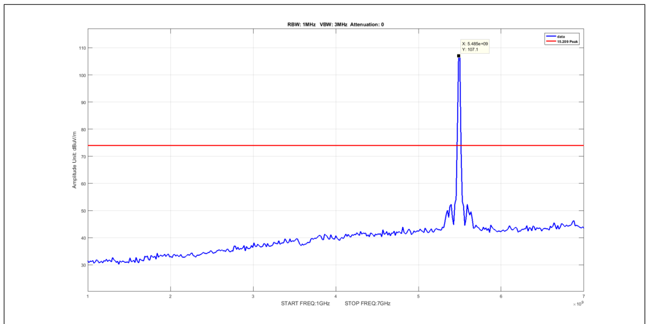
Plot 901. Undesirable Emissions, 50mni, Peak, 1-7GHz, 20M, 5490, pow11
