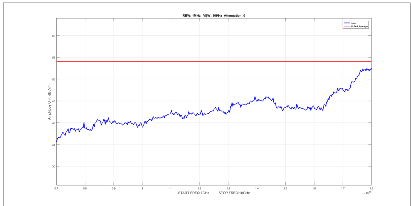
Plot 879. Undesirable Emissions, 5Omni, Average, 7-18GHz, 20M, 5700, pow11
