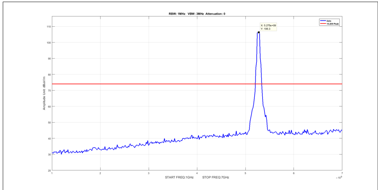
Plot 904. Undesirable Emissions, 50mni, Peak, 1-7GHz, 40M, 5270, pow19
