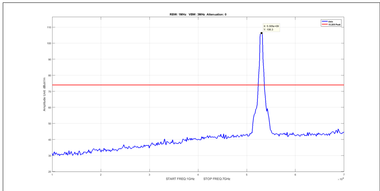
Plot 905. Undesirable Emissions, 50mni, Peak, 1-7GHz, 40M, 5300, pow19
