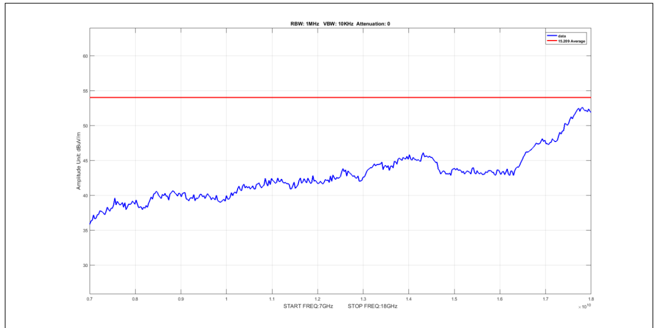
Plot 878. Undesirable Emissions, 5Omni, Average, 7-18GHz, 20M, 5595, pow14
