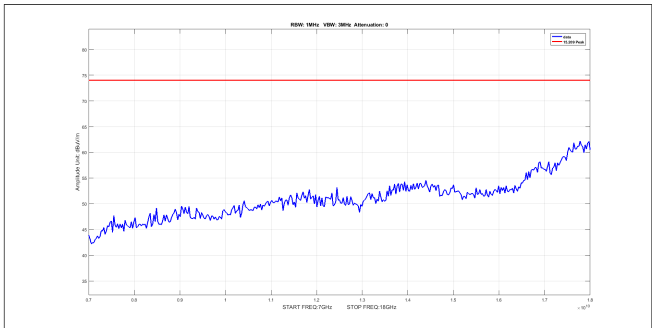
Plot 917. Undesirable Emissions, 50mni, Peak, 7-18GHz, 10M, 5300, pow11
