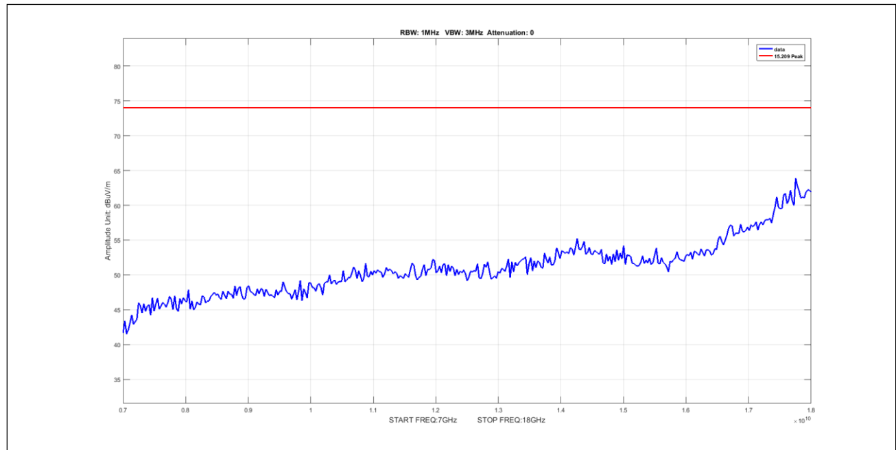
Plot 910. Undesirable Emissions, 5Omni, Peak, 7-18GHz, 5M, 5252.5, pow8
