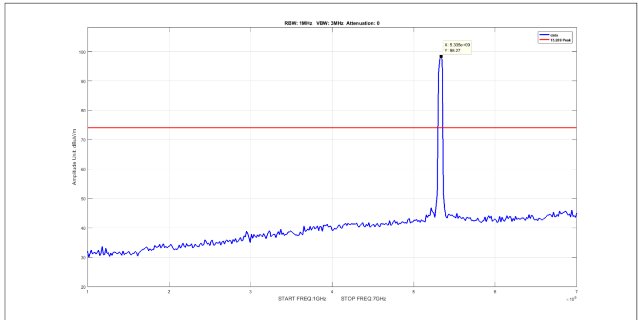
Plot 906. Undesirable Emissions, 5Omni, Peak, 1-7GHz, 40M, 5330, pow4
