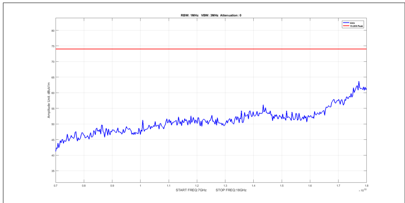
Plot 911. Undesirable Emissions, 5Omni, Peak, 7-18GHz, 5M, 5300, pow8
