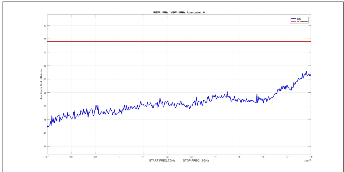
Plot 924. Undesirable Emissions, 5Omni, Peak, 7-18GHz, 20M, 5330, pow12
