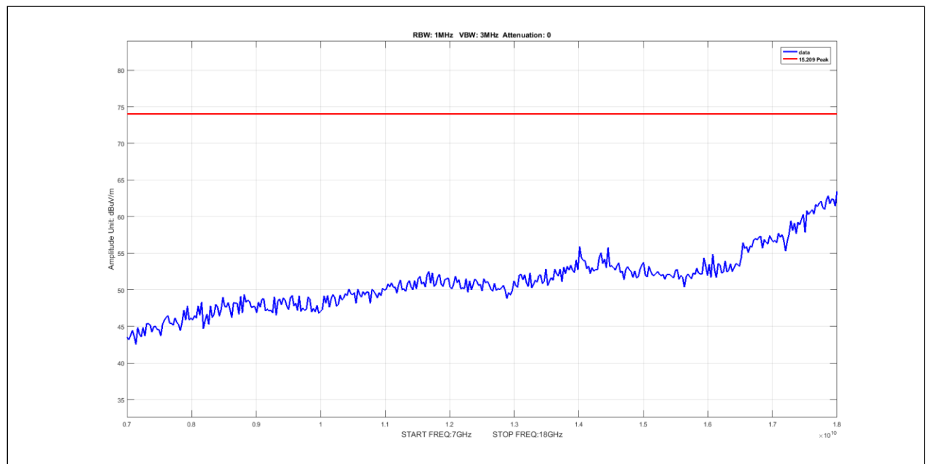
Plot 925. Undesirable Emissions, 5Omni, Peak, 7-18GHz, 20M, 5490, pow11
