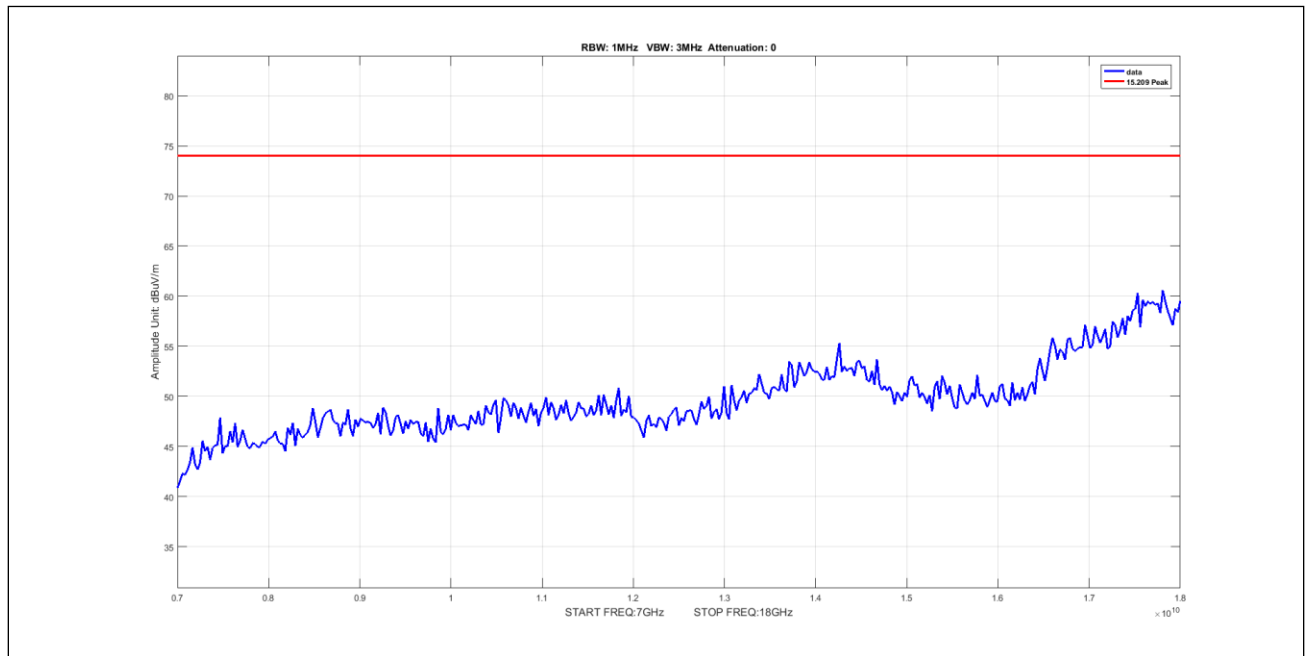
Plot 1006. Undesirable Emissions, 8Omni, Peak, 7-18GHz, 5M, 5252.5, pow6
