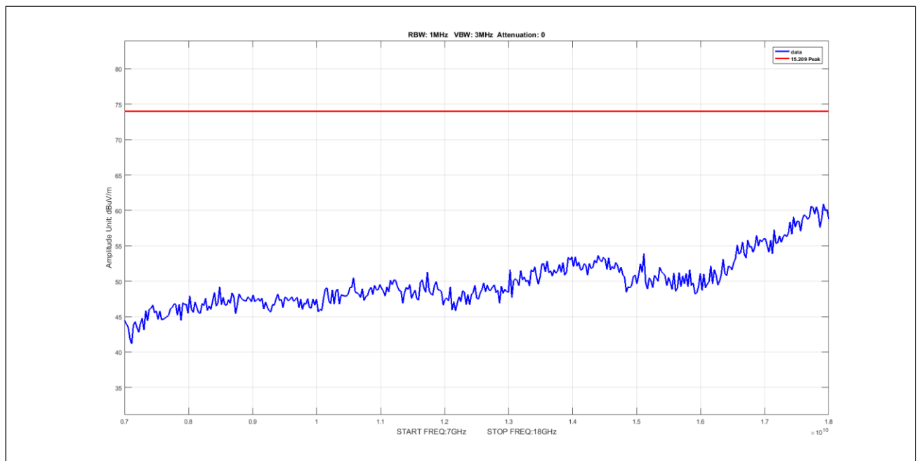
Plot 1007. Undesirable Emissions, 8Omni, Peak, 7-18GHz, 5M, 5300, pow6
