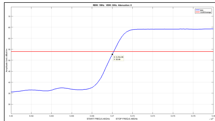
Plot 1243. Radiated Band Edge, 90 Sector, Average, 40M, 5490, pow0
