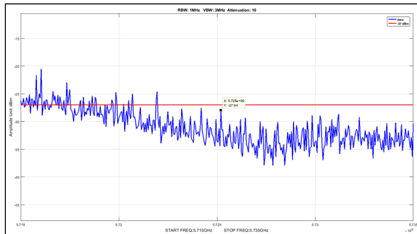
Plot 1214. Radiated Band Edge, 8 Omni, -27 dBm, 20M, 5700, pow8
