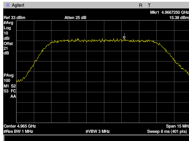
Plot 91. Power Spectral Density, 10MHz, 4965MHz, 8Omni, Port 2
