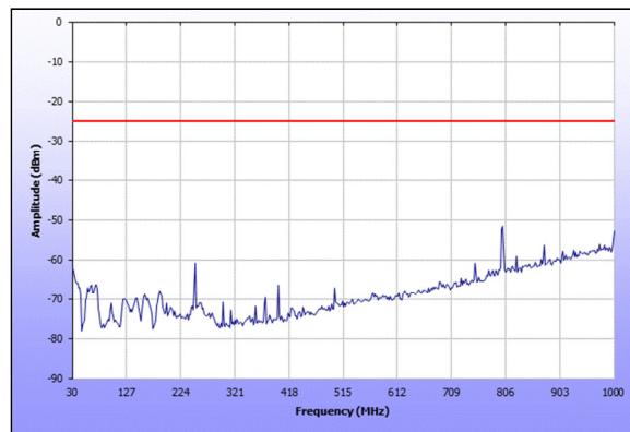
Plot239. Radiated Spurious Emissions, 20M, Low Channel, 30-1000MHz
