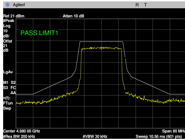
Plot 169. Emissions Mask, 20MHz, 4980MHz, 80Omni, Port 2
