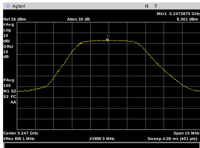
Plot 162. Power Spectral Density, 5M, 5247.5, 2Panel, Port 2
