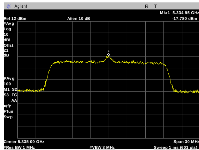
Plot 388. Power Spectral Density, 3 Para, 20MHz, 5335MHz, Port 1
