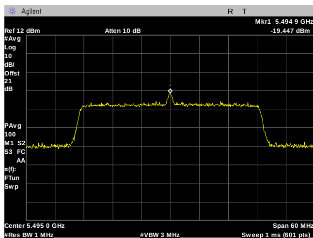
Plot 403. Power Spectral Density, 3 Para, 40MHz, 5495MHz, Port 2
