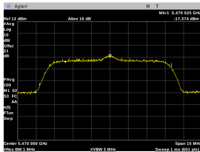
Plot 379. Power Spectral Density, 3 Para, 10MHz, 5470MHz, Port 2
