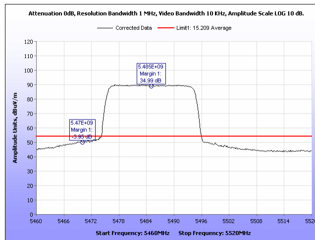
Plot 691. Radiated Band Edge, Average 90 Sector, 20MHz, 5485MHz, Port 1
