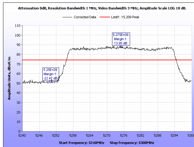
Plot 548. Radiated Band Edge, Peak 8 Omni, 40M, 5275, Port 2
