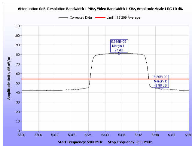
Plot 520. Radiated Band Edge, Average 8 Omni, 20M, 5335, Port 2
