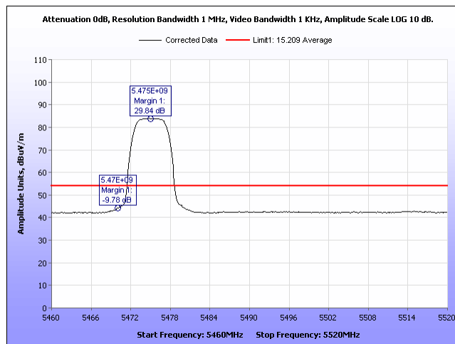
Plot 526. Radiated Band Edge, Average 8 Omni, 5M, 5475, Port 2
