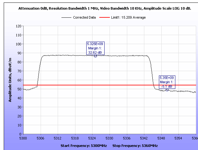
Plot 682. Radiated Band Edge, Average 90 Sector, 40MHz, 5325MHz, Port 2
