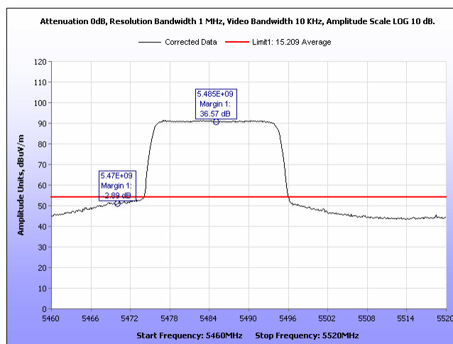
Plot 849. Radiated Band Edge, Average 2 Panel, 20MHz, 5485MHz, Port 2
