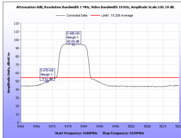
Plot 844. Radiated Band Edge, Average 2 Panel, 10MHz, 5480MHz, Port 1
