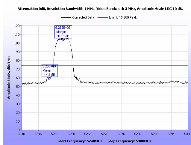
Plot 856. Radiated Band Edge, Peak 2 Panel, 5MHz, 5255MHz, Port 1
