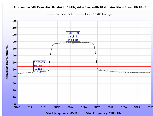
Plot 676. Radiated Band Edge, Average 90 Sector, 20MHz, 5265MHz, Port 2
