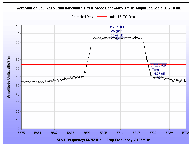
Plot 875. Radiated Band Edge, Peak 2 Panel, 20MHz, 5710MHz, Port 2
