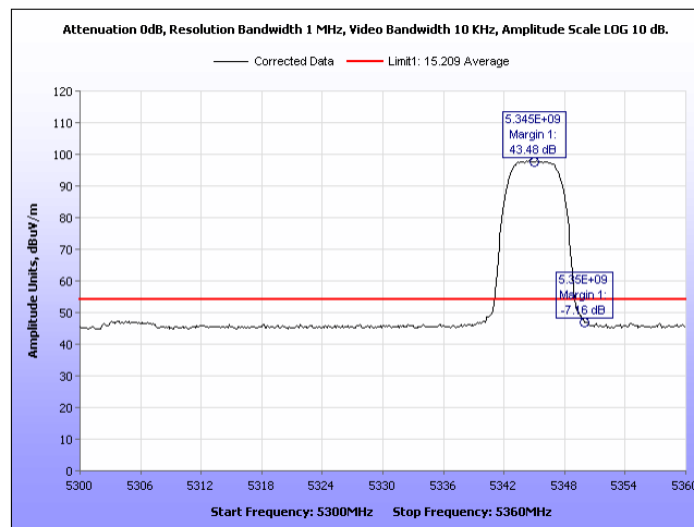
Plot 670. Radiated Band Edge, Average 90 Sector, 5MHz, 5345MHz, Port 2
