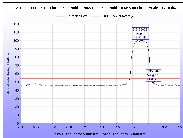
Plot 827. Radiated Band Edge, Average 2 Panel, 5MHz, 5345MHz, Port 2
