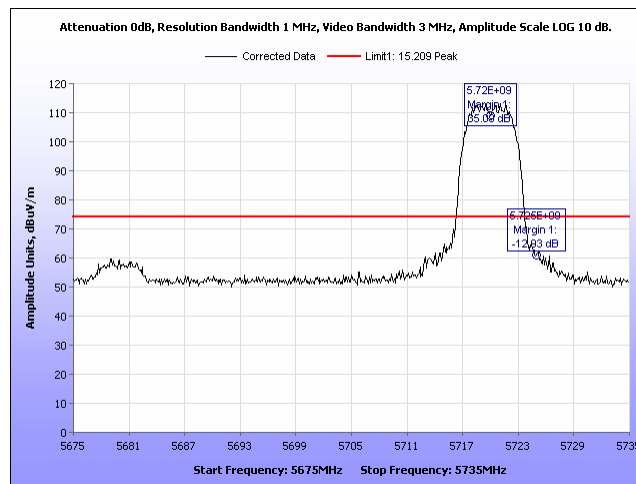
Plot 866. Radiated Band Edge, Peak 2 Panel, 5MHz, 5720MHz, Port 1
