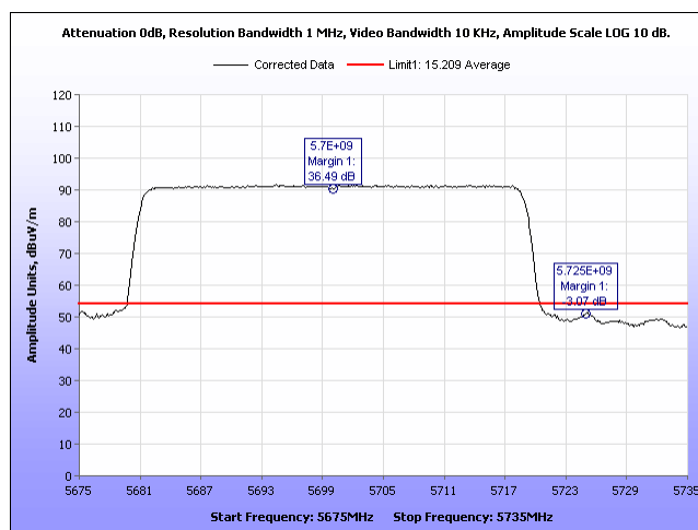
Plot 698. Radiated Band Edge, Average 90 Sector, 40MHz, 5700MHz, Port 2
