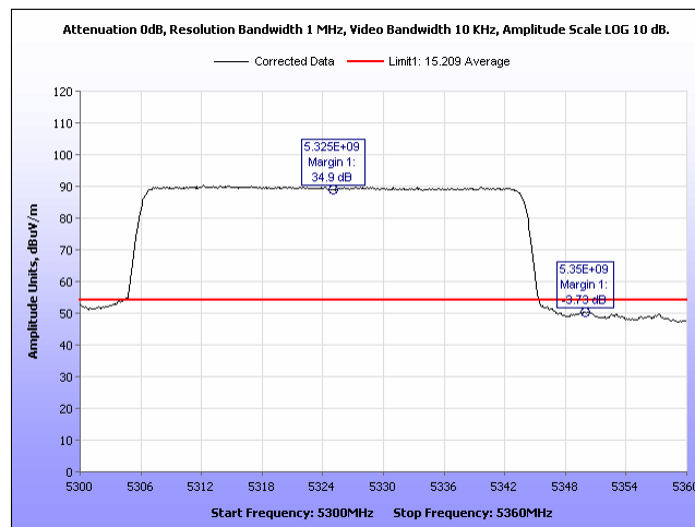
Plot 838. Radiated Band Edge, Average 2 Panel, 40MHz, 5325MHz, Port 1
