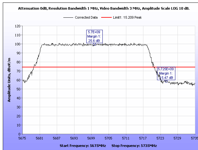
Plot 721. Radiated Band Edge, Peak 90 Sector, 40MHz, 5700MHz, Port 1
