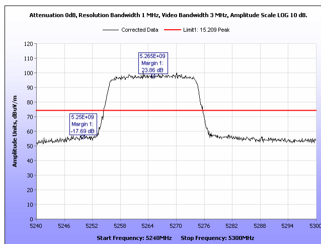
Plot 704. Radiated Band Edge, Peak 90 Sector, 20MHz, 5265MHz, Port 2
