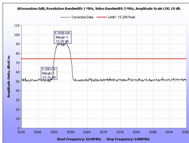
Plot 541. Radiated Band Edge, Peak 8 Omni, 5M, 5255, Port 1
