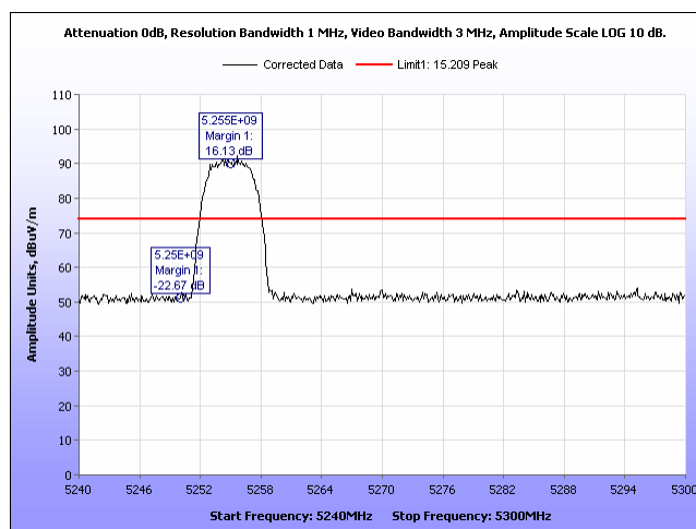
Plot 542. Radiated Band Edge, Peak 8 Omni, 5M, 5255, Port 2
