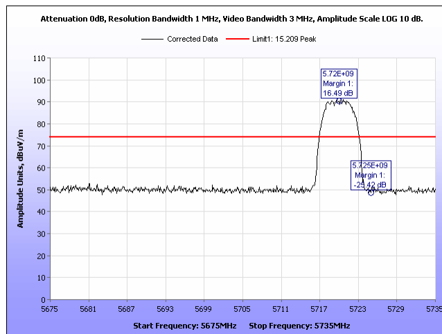
Plot 552. Radiated Band Edge, Peak 8 Omni, 5M, 5720, Port 2
