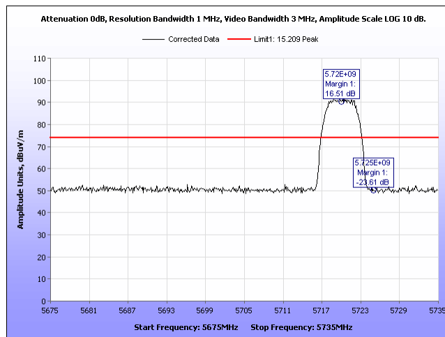
Plot 551. Radiated Band Edge, Peak 8 Omni, 5M, 5720, Port 1
