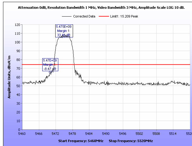
Plot 865. Radiated Band Edge, Peak 2 Panel, 5MHz, 5475MHz, Port 2
