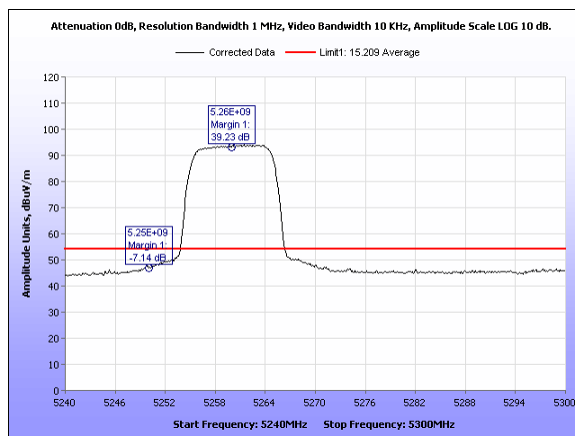
Plot 829. Radiated Band Edge, Average 2 Panel, 10MHz, 5260MHz, Port 2
