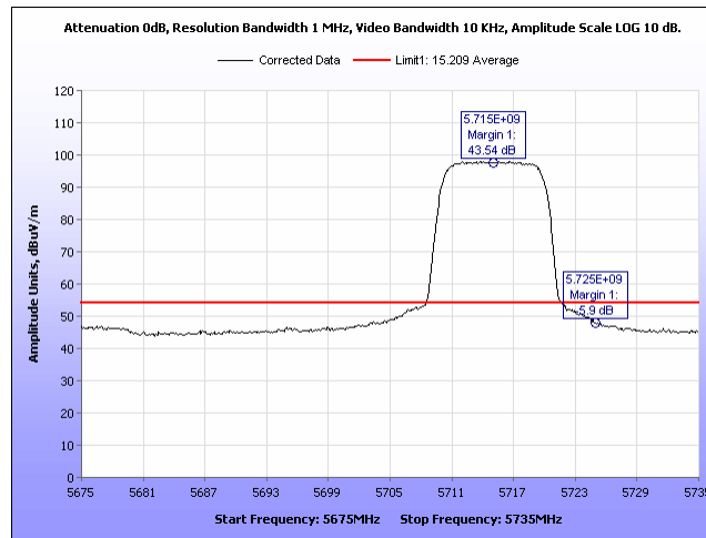
Plot 690. Radiated Band Edge, Average 90 Sector, 10MHz, 5715MHz, Port 2
