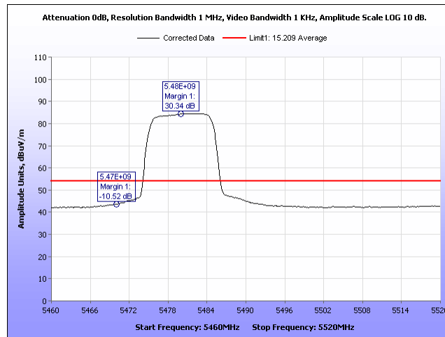
Plot 530. Radiated Band Edge, Average 8 Omni, 10M, 5480, Port 2
