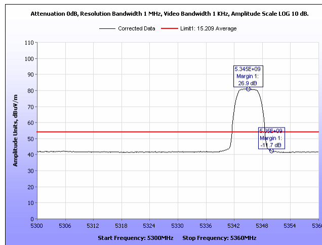
Plot 512. Radiated Band Edge, Average 8 Omni, 5M, 5345, Port 2
