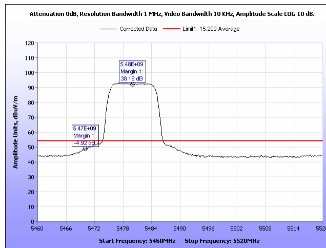
Plot 688. Radiated Band Edge, Average 90 Sector, 10MHz, 5480MHz, Port 2
