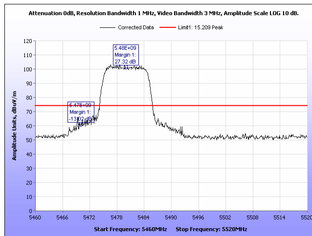
Plot 712. Radiated Band Edge, Peak 90 Sector, 10MHz, 5480MHz, Port 2
