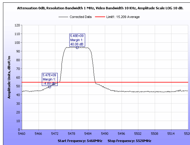
Plot 845. Radiated Band Edge, Average 2 Panel, 10MHz, 5480MHz, Port 2
