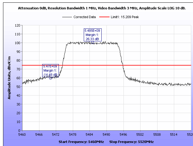
Plot 872. Radiated Band Edge, Peak 2 Panel, 20MHz, 5485MHz, Port 1
