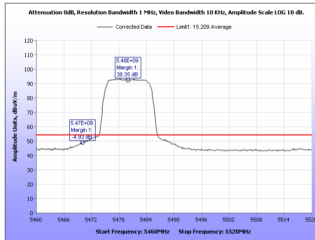
Plot 687. Radiated Band Edge, Average 90 Sector, 10MHz, 5480MHz, Port 1
