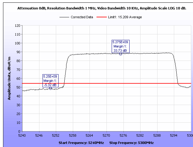
Plot 836. Radiated Band Edge, Average 2 Panel, 40MHz, 5275MHz, Port 1
