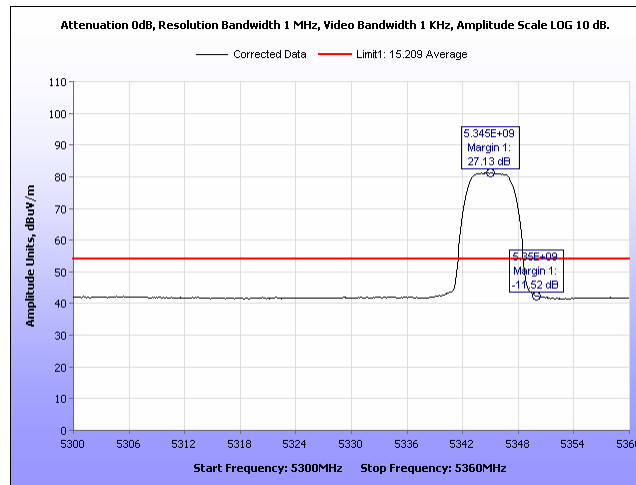
Plot 511. Radiated Band Edge, Average 8 Omni, 5M, 5345, Port 1
