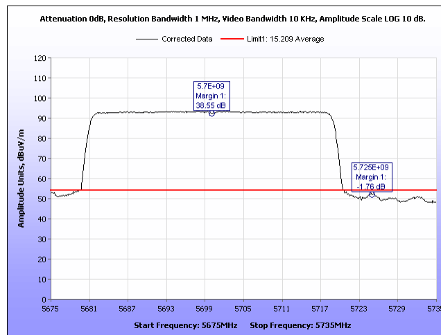
Plot 854. Radiated Band Edge, Average 2 Panel, 40MHz, 5700MHz, Port 1
