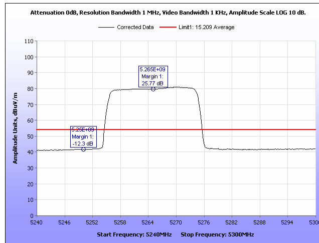
Plot 517. Radiated Band Edge, Average 8 Omni, 20M, 5265, Port 1
