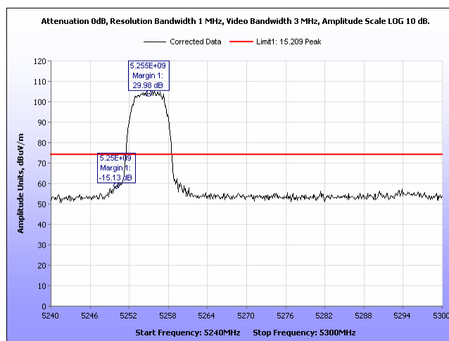
Plot 857. Radiated Band Edge, Peak 2 Panel, 5MHz, 5255MHz, Port 2
