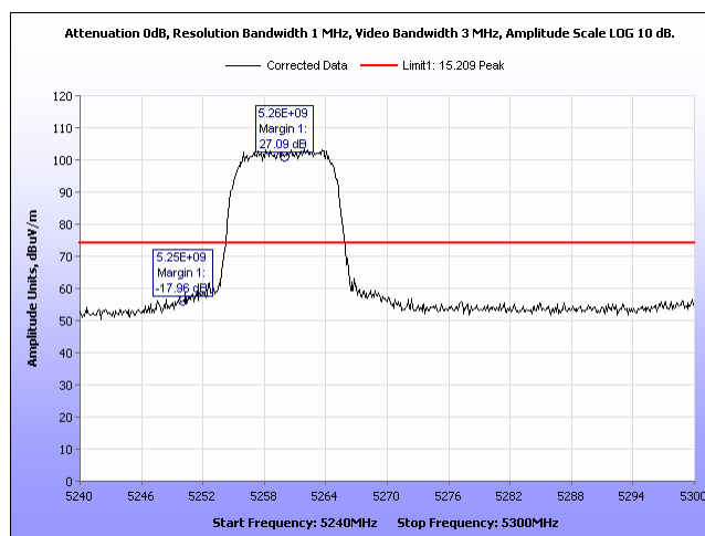
Plot 858. Radiated Band Edge, Peak 2 Panel, 10MHz, 5260MHz, Port 1
