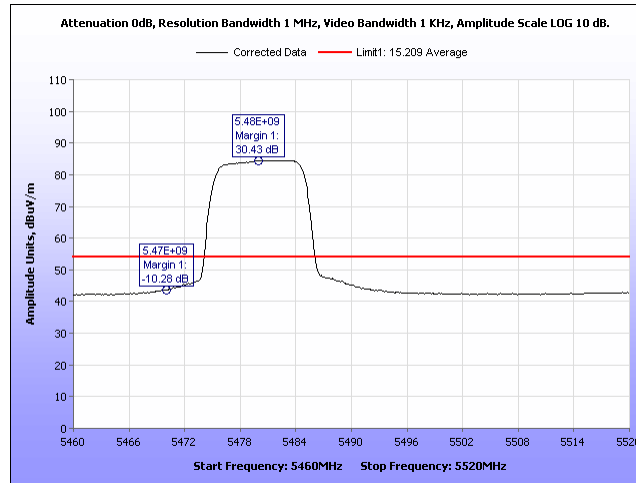
Plot 529. Radiated Band Edge, Average 8 Omni, 10M, 5480, Port 1
