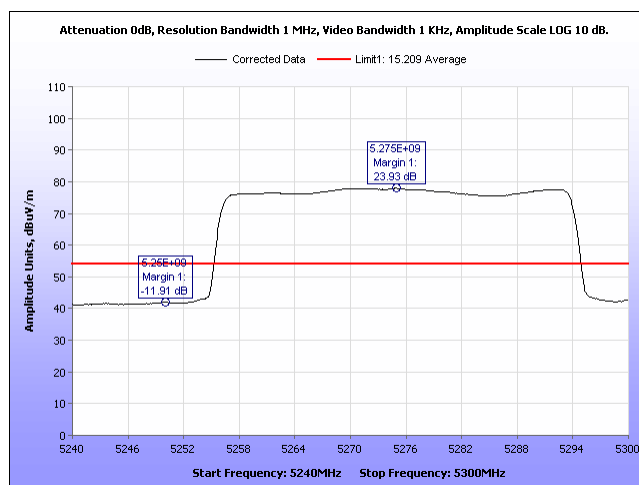
Plot 521. Radiated Band Edge, Average 8 Omni, 40M, 5275, Port 1
