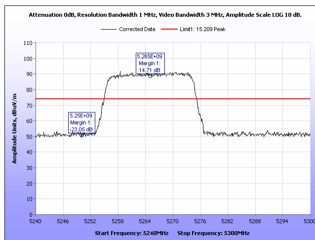
Plot 545. Radiated Band Edge, Peak 8 Omni, 20M, 5265, Port 1
