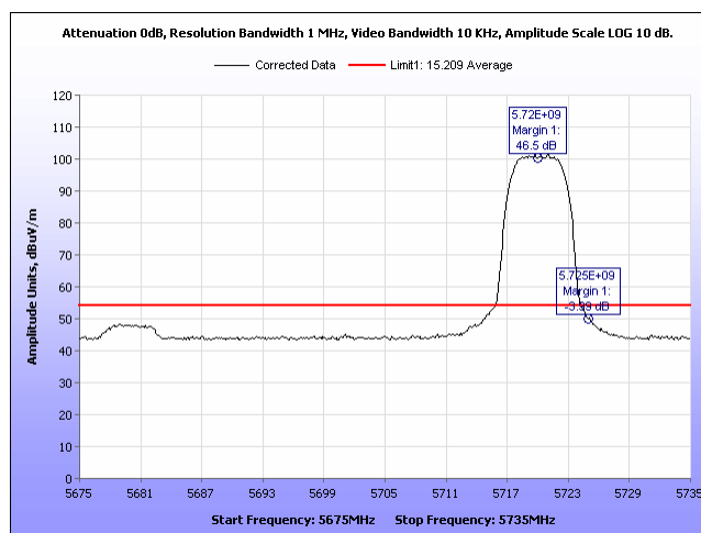
Plot 686 Radiated Band Edge, Average 90 Sector, 5MHz, 5720MHz, Port 2
