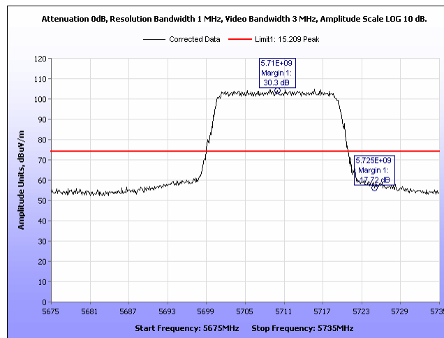
Plot 718. Radiated Band Edge, Peak 90 Sector, 20MHz, 5710MHz, Port 2
