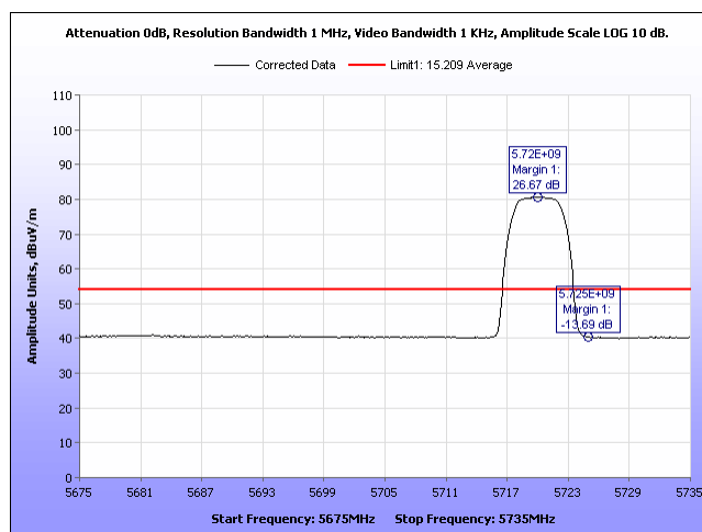
Plot 527. Radiated Band Edge, Average 8 Omni, 5M, 5720, Port 1
