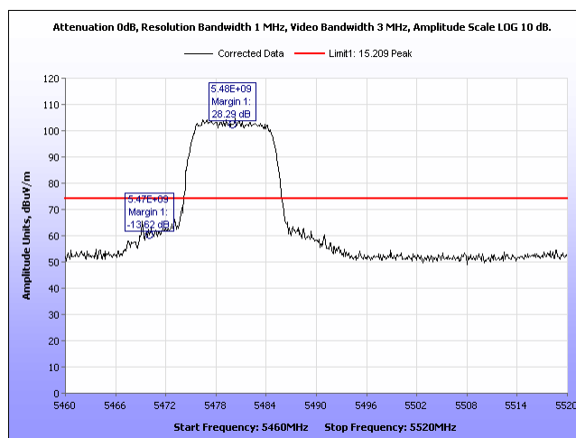
Plot 869. Radiated Band Edge, Peak 2 Panel, 10MHz, 5480MHz, Port 2
