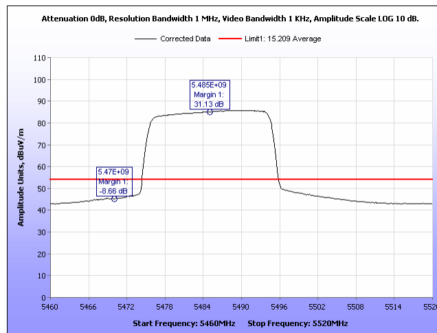
Plot 533. Radiated Band Edge, Average 8 Omni, 20M, 5485, Port 1
