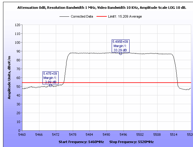
Plot 853. Radiated Band Edge, Average 2 Panel, 40MHz, 5495MHz, Port 2
