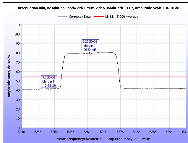
Plot 518. Radiated Band Edge, Average 8 Omni, 20M, 5265, Port 2
