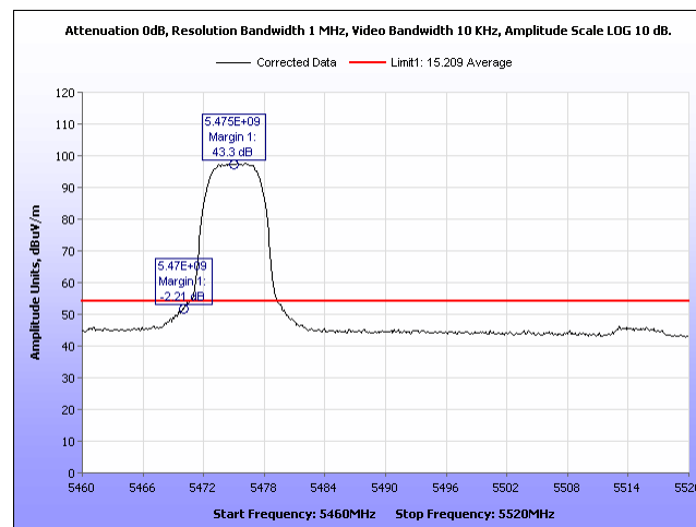
Plot 988. Radiated Band Edge, Average 3 Para, 5MHz, 5475MHz, Port 2
