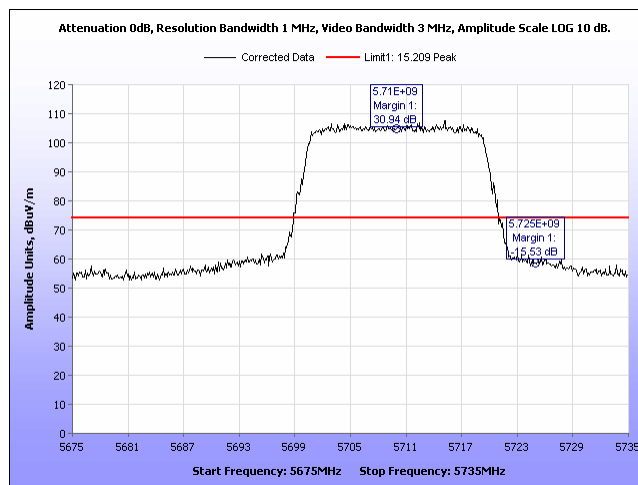
Plot 1021. Radiated Band Edge, Peak 3 Para, 20MHz, 5710MHz, Port 1
