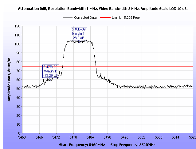
Plot 1015. Radiated Band Edge, Peak 3 Para, 10MHz, 5480MHz, Port 1
