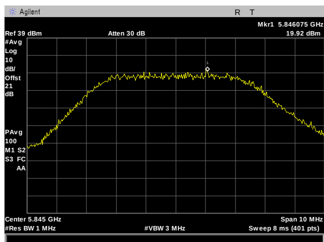
Plot 113. Power Spectral Density, 5M, 5845MHz, 8Omni, Port 2
