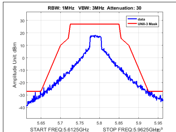
Plot 425. Undesirable Emissions, UNII-3 Emissions Mask, 20M, 5785MHz, 80mni
