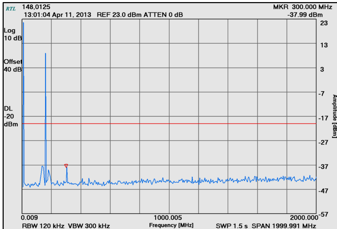
Plot 4-5: Conducted Spurious Emissions – H-CPM TDMA; 148.0125 MHz
