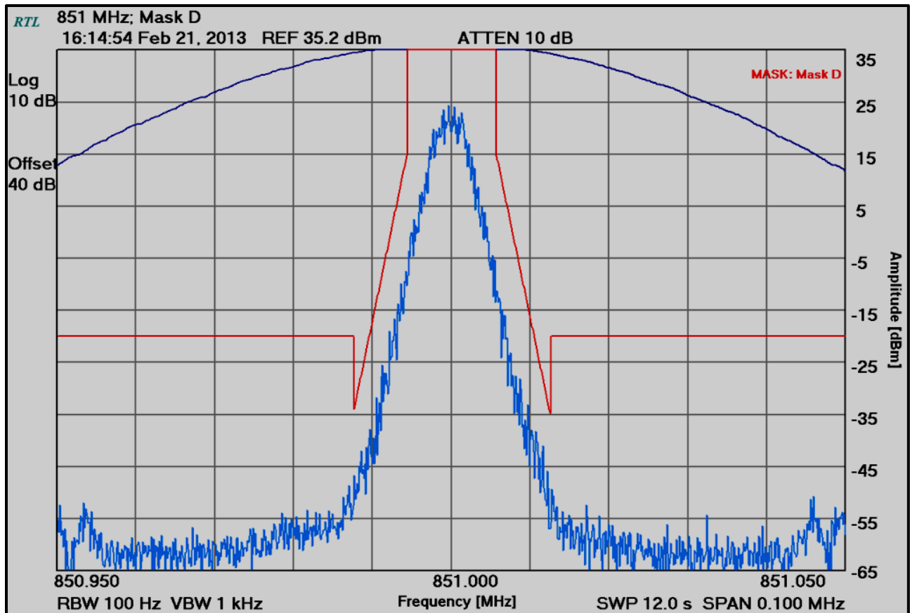
Plot 6-16: Occupied Bandwidth – H-CPM TDMA; 851.0000 MHz; Mask D
