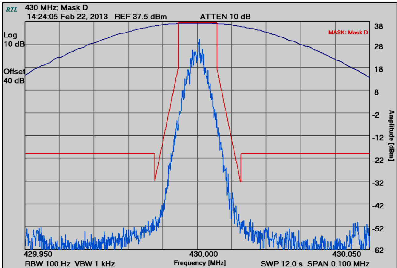
Plot 6-9: Occupied Bandwidth – H-CPM TDMA; 430.0000 MHz; Mask D
