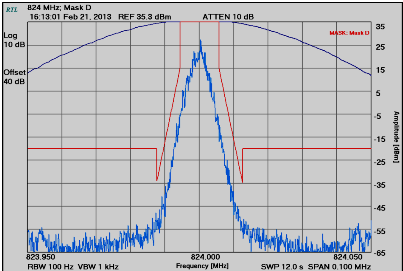
Plot 6-15: Occupied Bandwidth – H-CPM TDMA; 824.0000 MHz; Mask D
