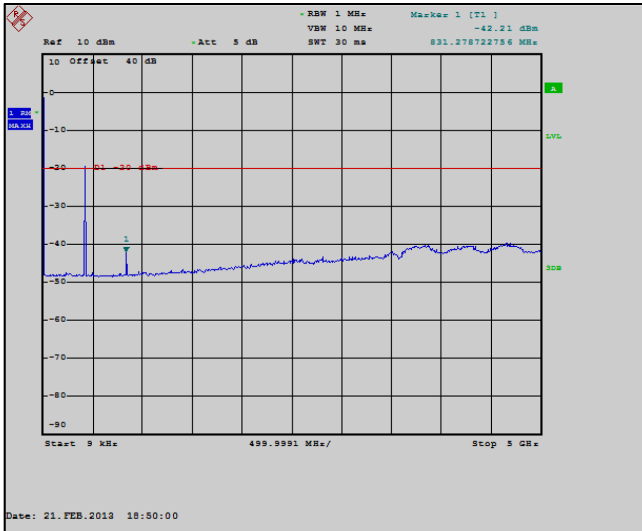
Plot 5-8: Conducted Spurious Emissions – H-CPM TDMA; 418.0000 MHz
