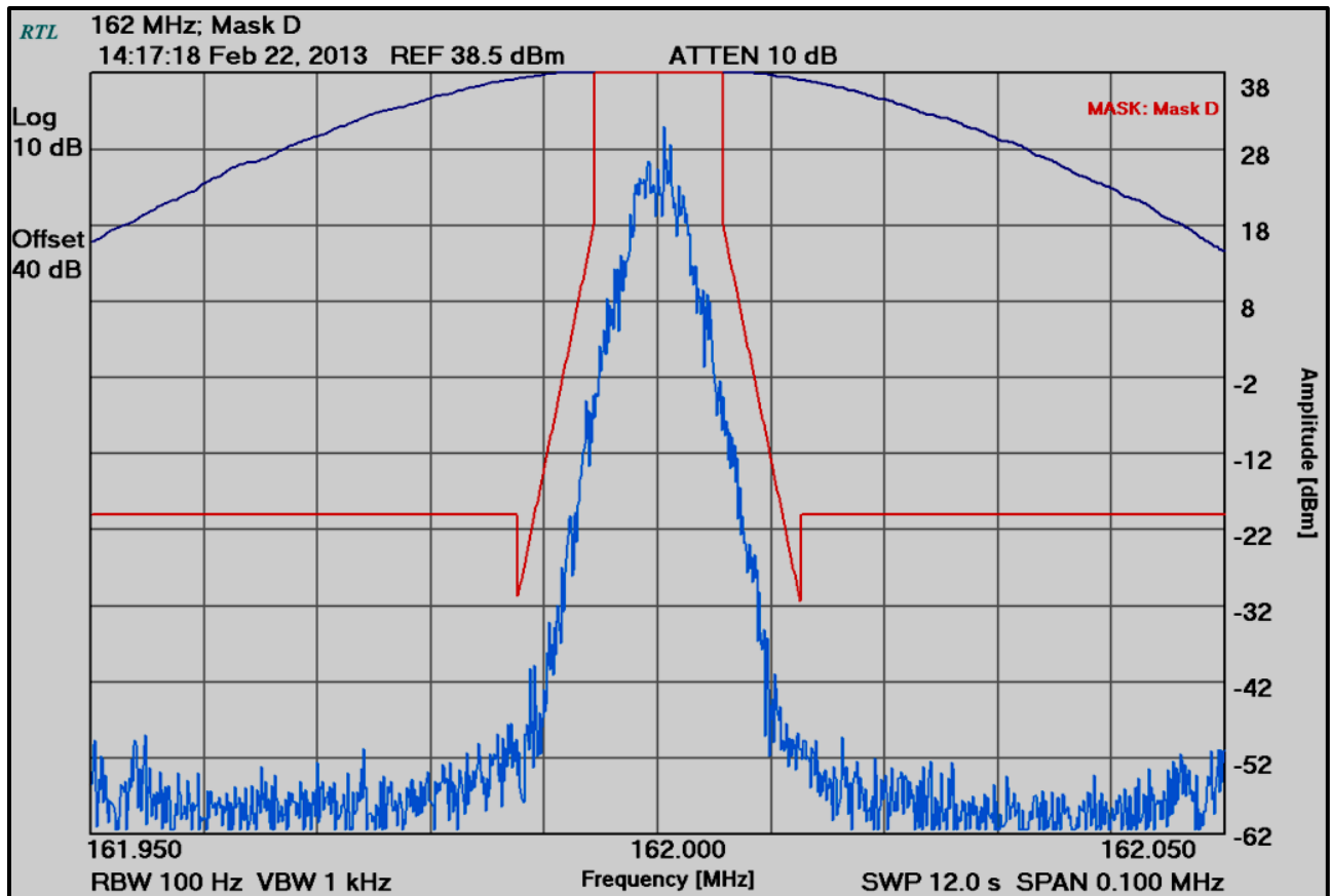
Plot 6-5: Occupied Bandwidth – H-CPM TDMA; 162.0000 MHz; Mask D
