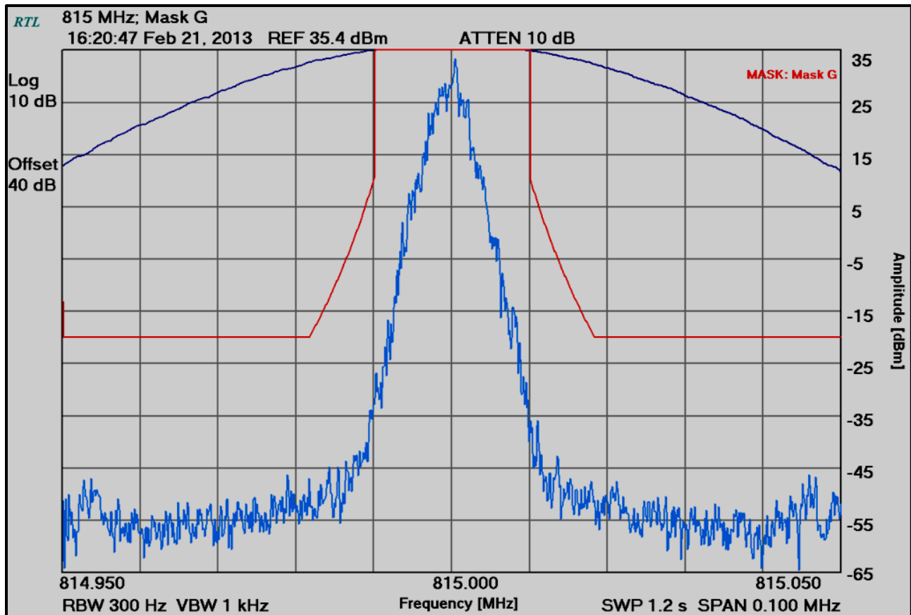
Plot 6-20: Occupied Bandwidth – H-CPM TDMA; 815.0000 MHz; Mask G
