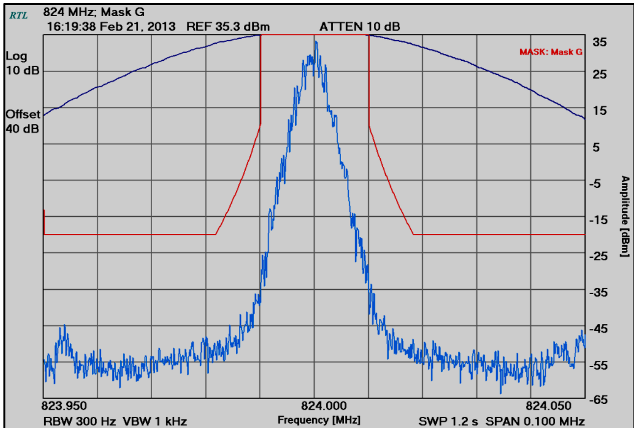
Plot 6-21: Occupied Bandwidth – H-CPM TDMA; 824.0000 MHz; Mask G
