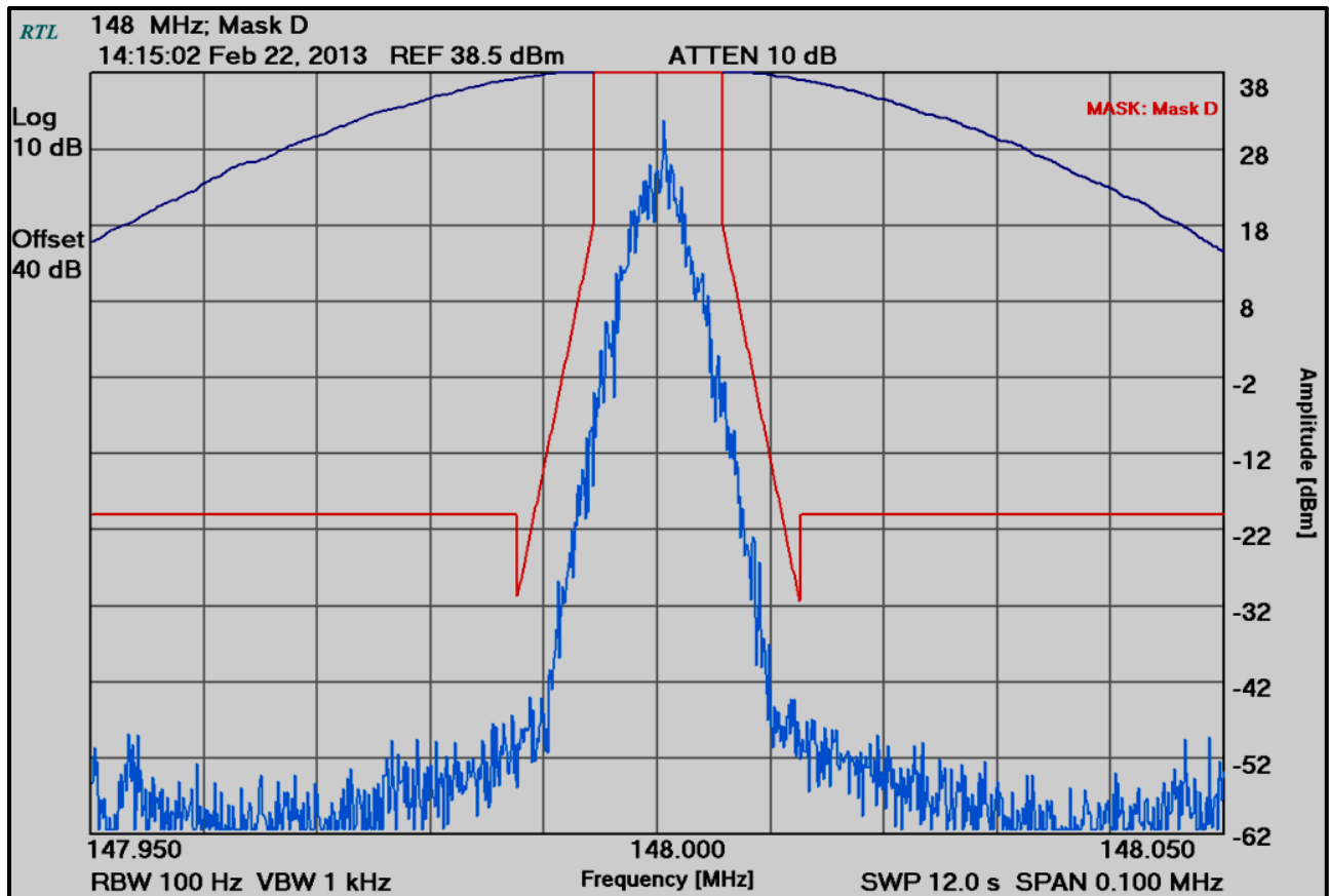
Plot 6-4: Occupied Bandwidth – H-CPM TDMA; 148.0000 MHz; Mask D
