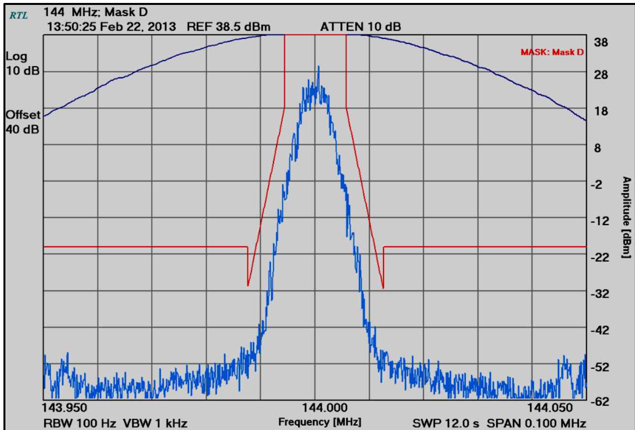
Plot 6-3: Occupied Bandwidth – H-CPM TDMA; 144.0000 MHz; Mask D
