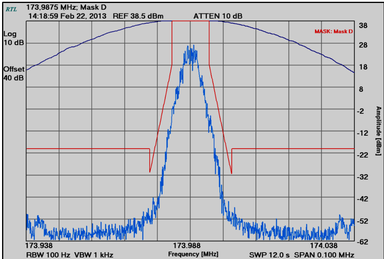
Plot 6-6: Occupied Bandwidth – H-CPM TDMA; 173.9875 MHz; Mask D
