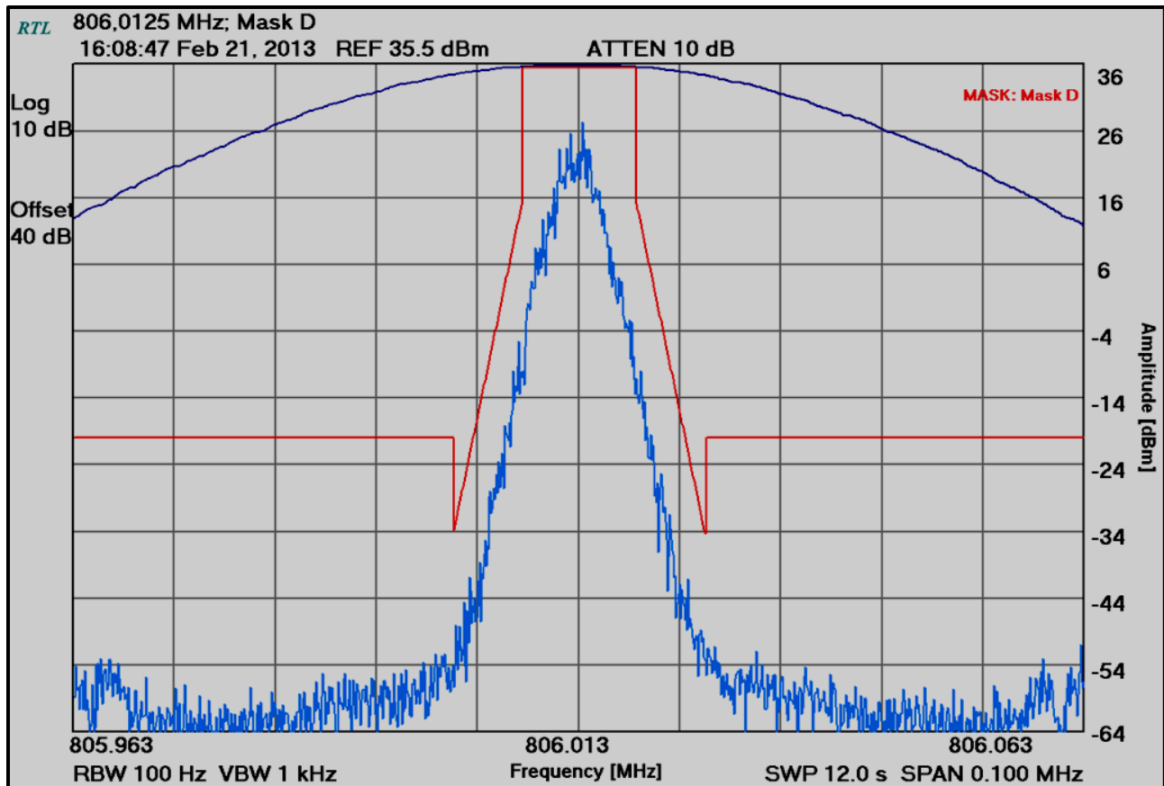
Plot 6-13: Occupied Bandwidth – H-CPM TDMA; 806.0125 MHz; Mask D
