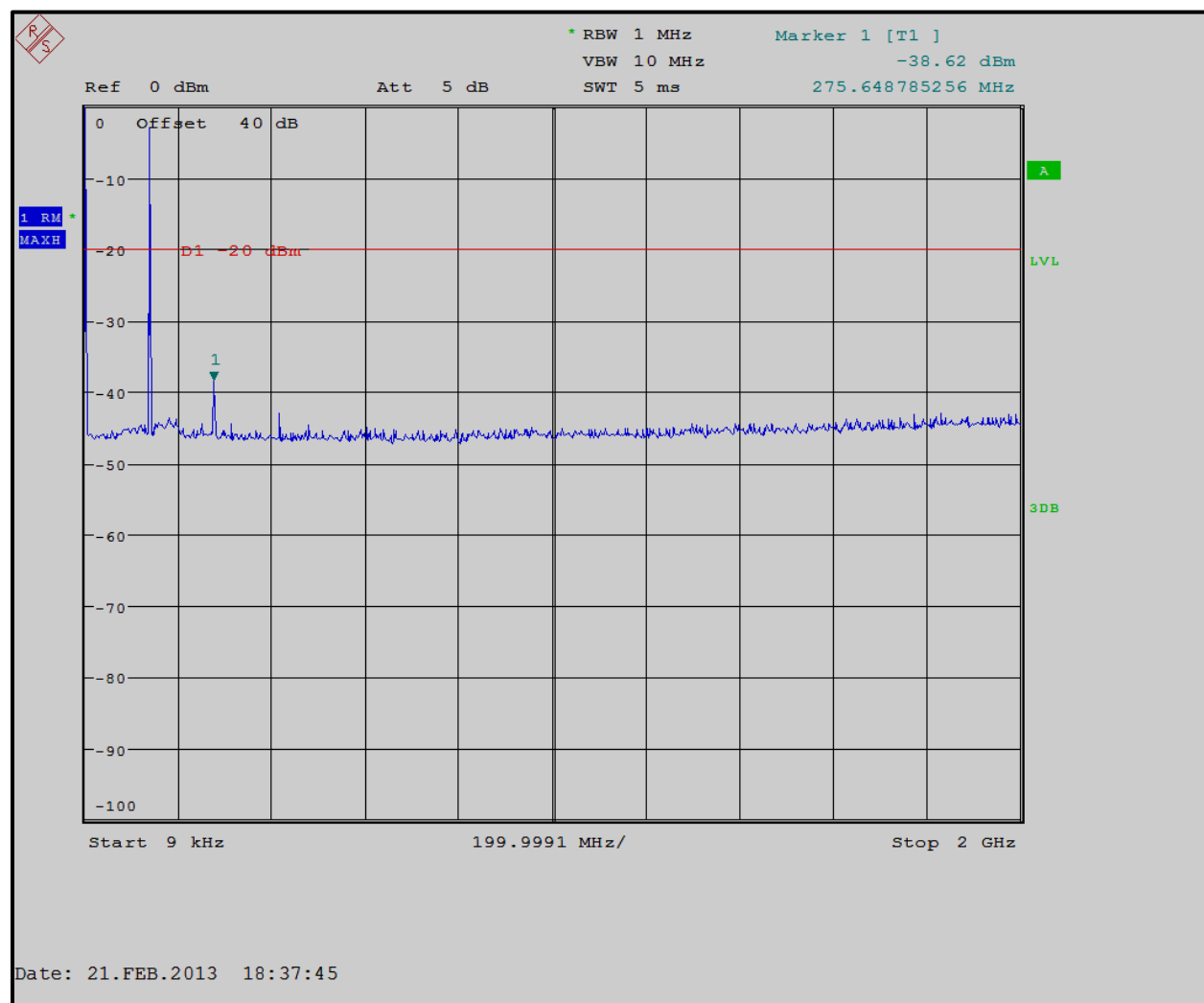
Plot 5-1: Conducted Spurious Emissions – H-CPM TDMA; 138.0000 MHz
