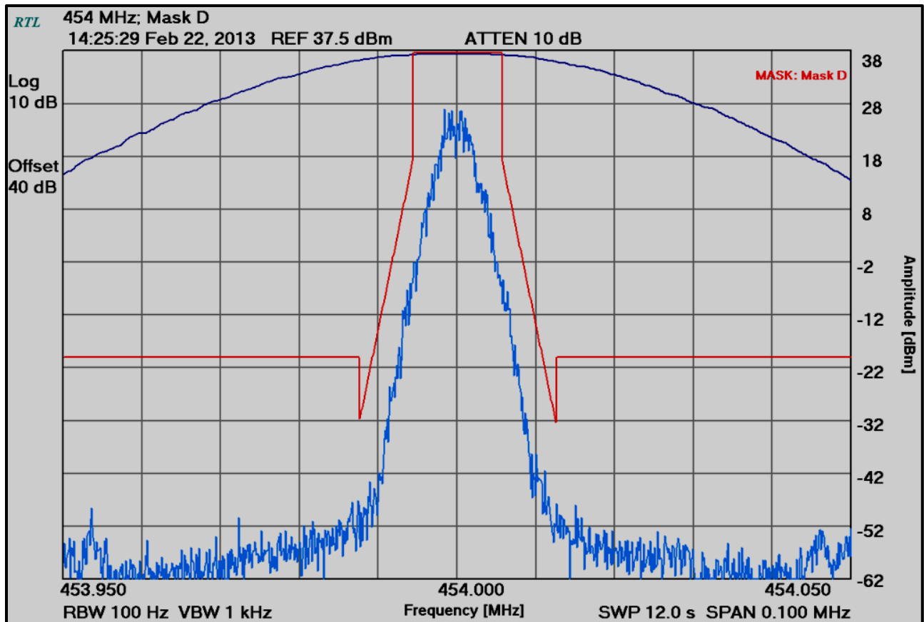
Plot 6-11: Occupied Bandwidth – H-CPM TDMA; 454.0000 MHz; Mask D
