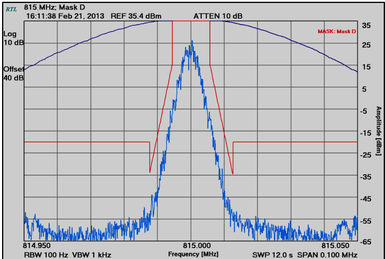
Plot 6-14: Occupied Bandwidth – H-CPM TDMA; 815.0000 MHz; Mask D
