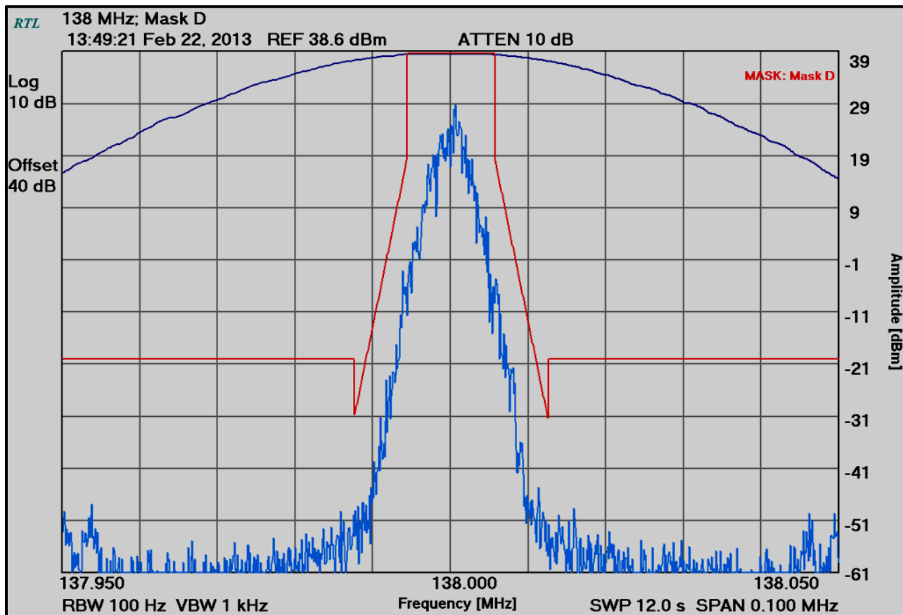
Plot 6-1: Occupied Bandwidth – H-CPM TDMA; 138.0000 MHz; Mask D
