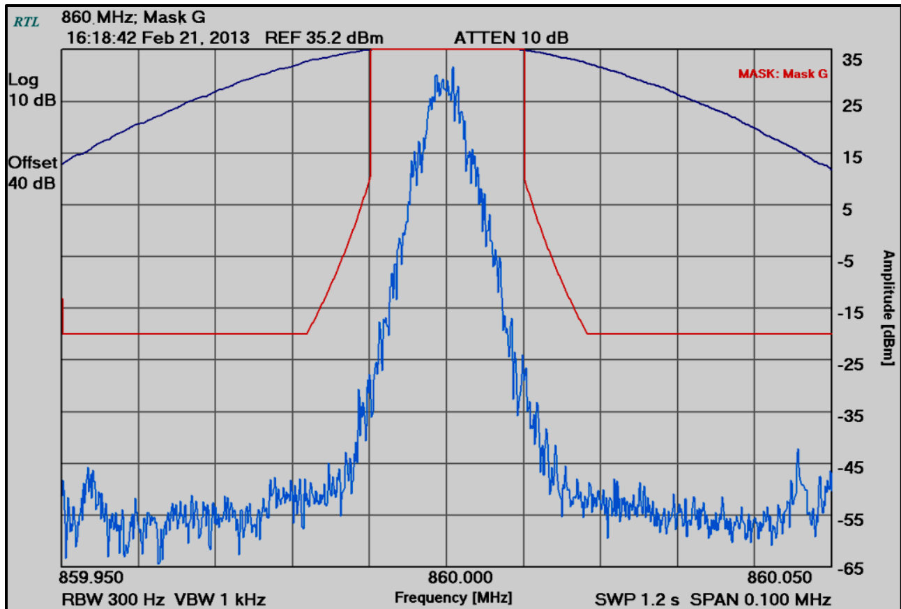
Plot 6-23: Occupied Bandwidth – H-CPM TDMA; 860.0000 MHz; Mask G
