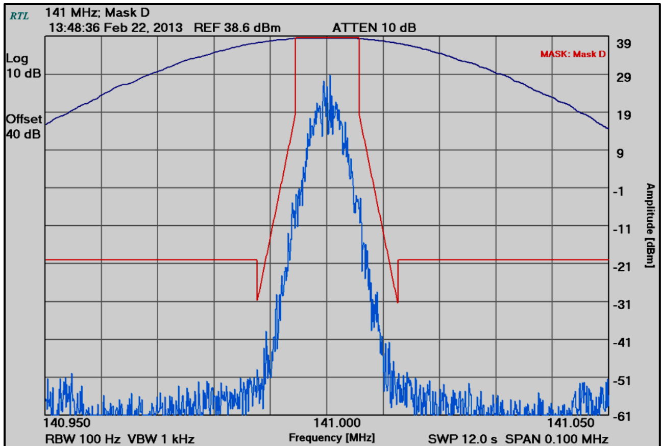
Plot 6-2: Occupied Bandwidth – H-CPM TDMA; 141.0000 MHz; Mask D
