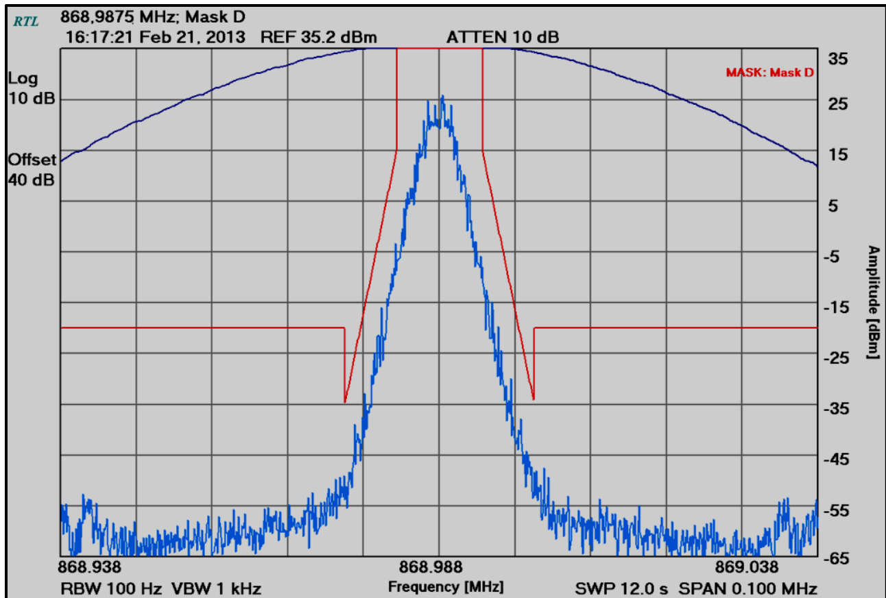
Plot 6-18: Occupied Bandwidth – H-CPM TDMA; 868.9875 MHz; Mask D
