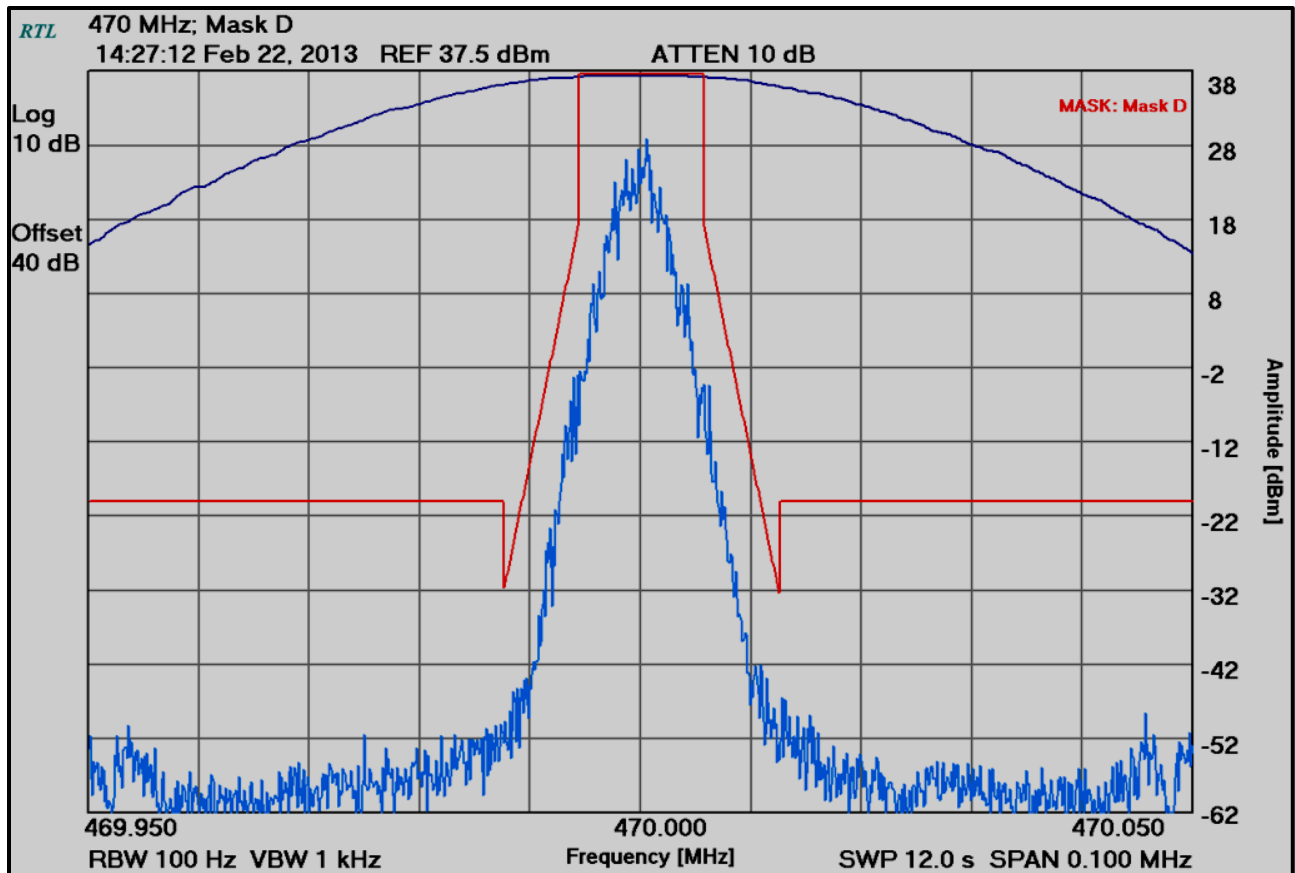
Plot 6-12: Occupied Bandwidth – H-CPM TDMA; 470.0000 MHz; Mask D
