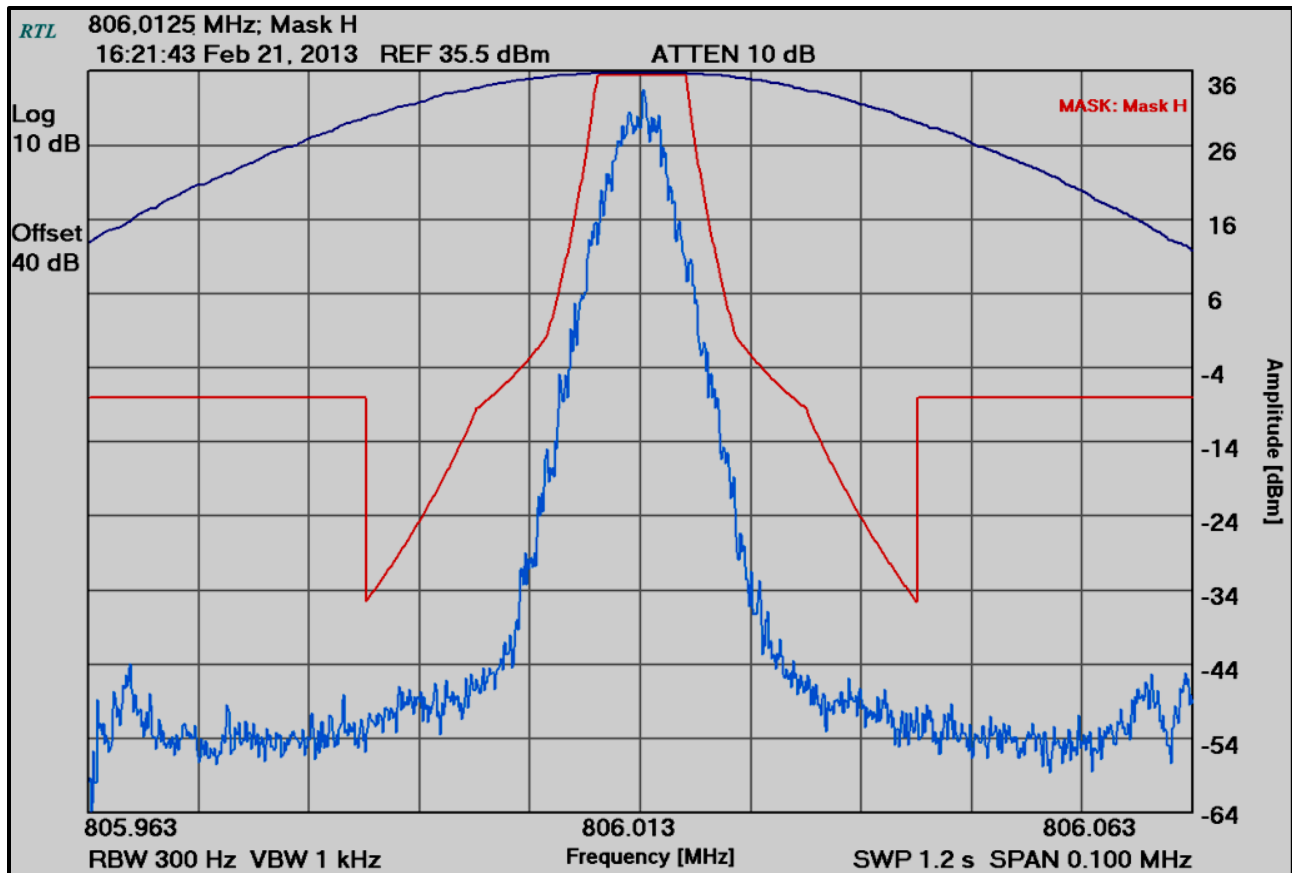
Plot 6-19: Occupied Bandwidth – H-CPM TDMA; 806.0125 MHz; Mask H
