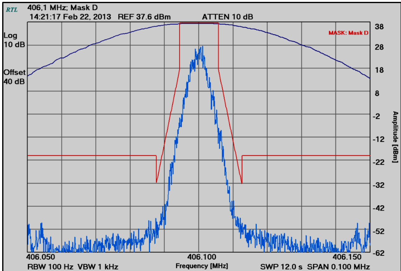
Plot 6-7: Occupied Bandwidth – H-CPM TDMA; 406.1000 MHz; Mask D
