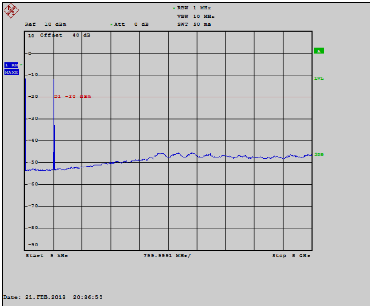
Plot 5-18: Conducted Spurious Emissions – H-CPM TDMA; 805.9875 MHz
