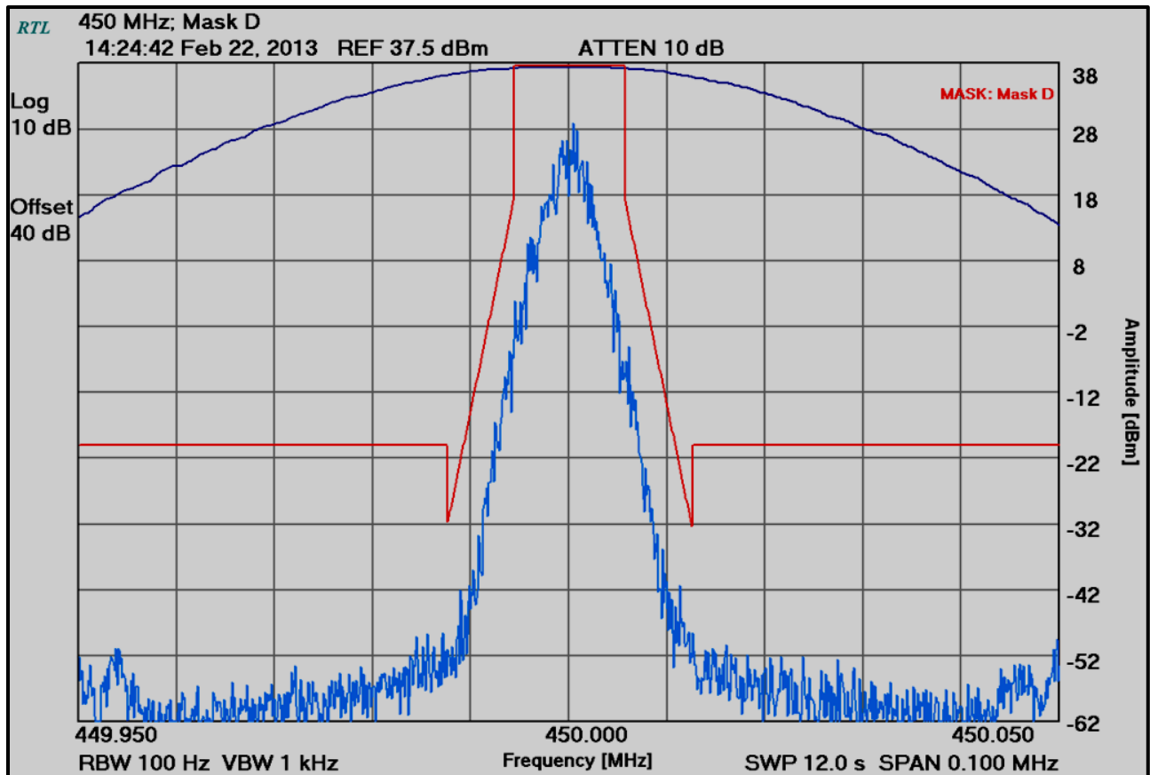
Plot 6-10: Occupied Bandwidth – H-CPM TDMA; 450.0000 MHz; Mask D
