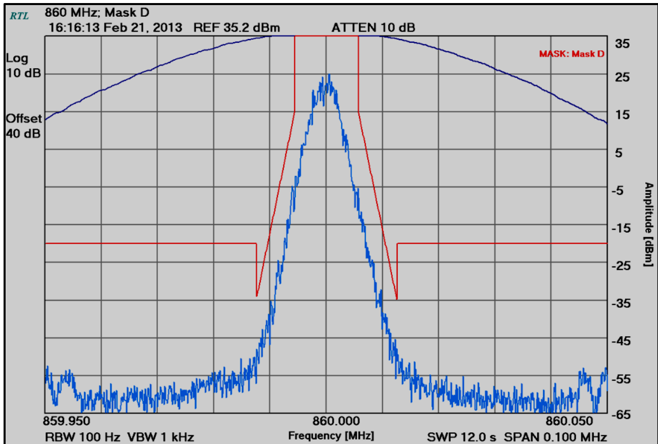
Plot 6-17: Occupied Bandwidth – H-CPM TDMA; 860.0000 MHz; Mask D
