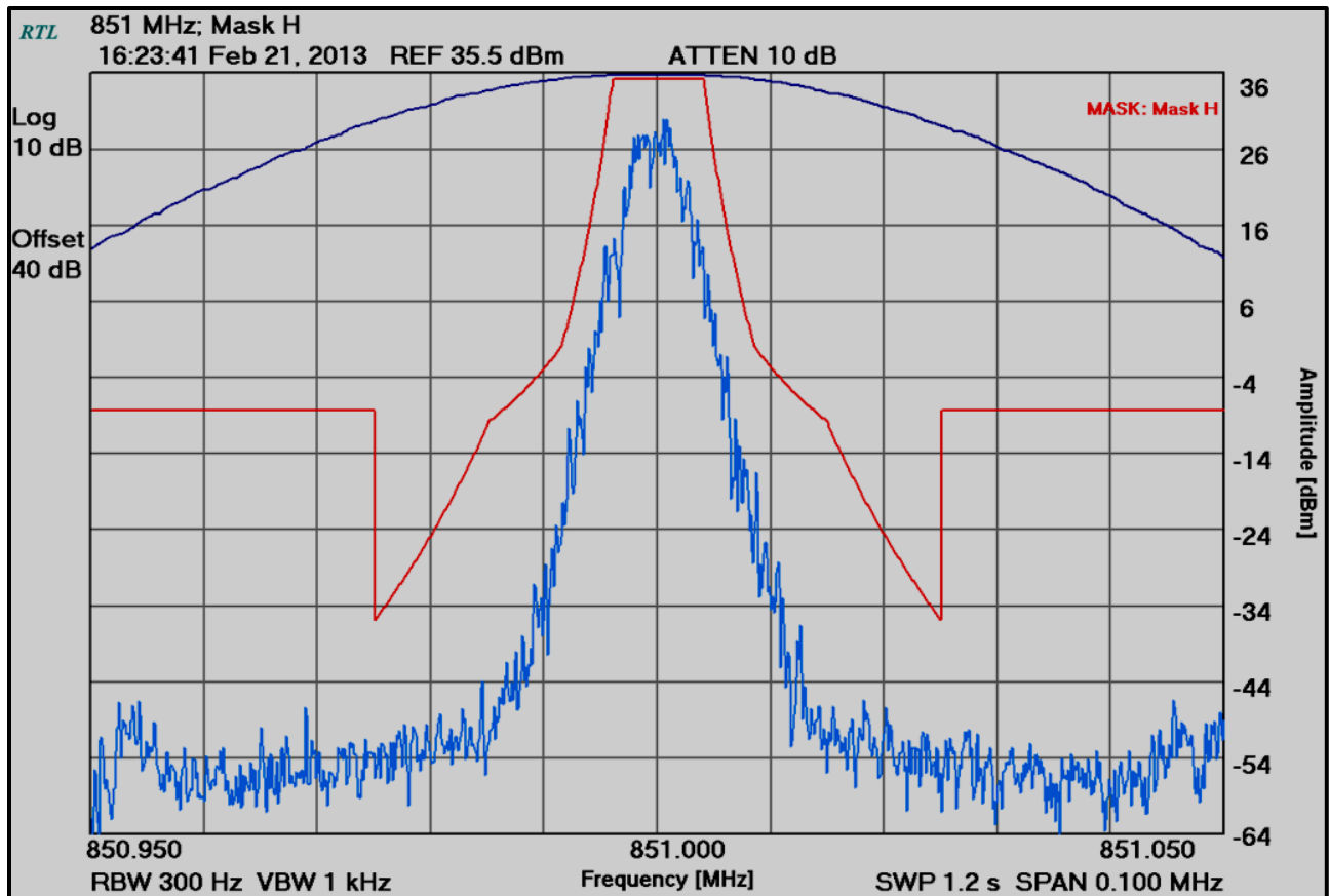
Plot 6-22: Occupied Bandwidth – H-CPM TDMA; 851.0000 MHz; Mask H
