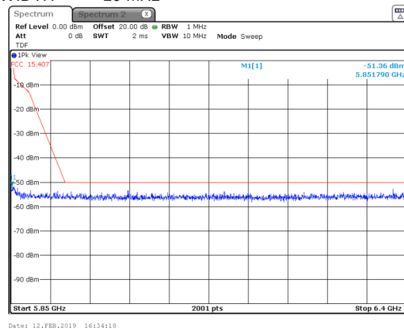
Plot 7.10.4 Conducted spurious emission measurements in the range 5.85 – 6.4 GHz CARRIER FREQUENCY 5730 MHz CHANNEL BANDWIDTH 10 MHz
