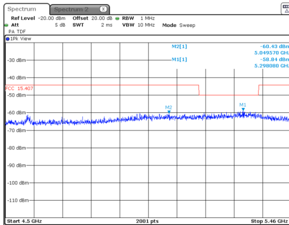
Plot 7.10.2 Conducted spurious emission measurements in the range 4.5 – 5.46 GHz
