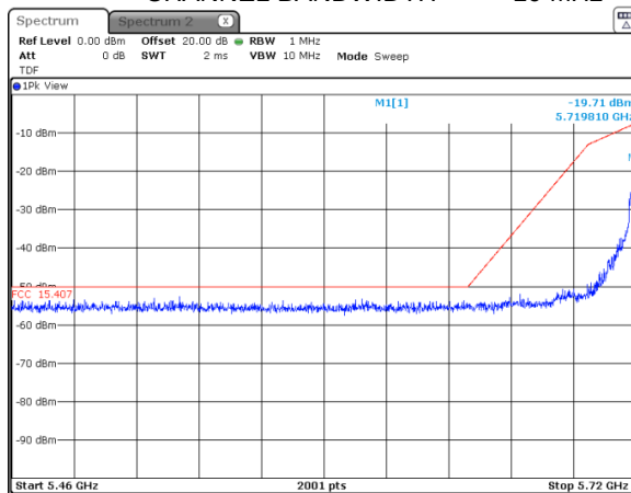
Plot 7.10.3 Conducted spurious emission measurements in the range 5.46 – 5.725 GHz
