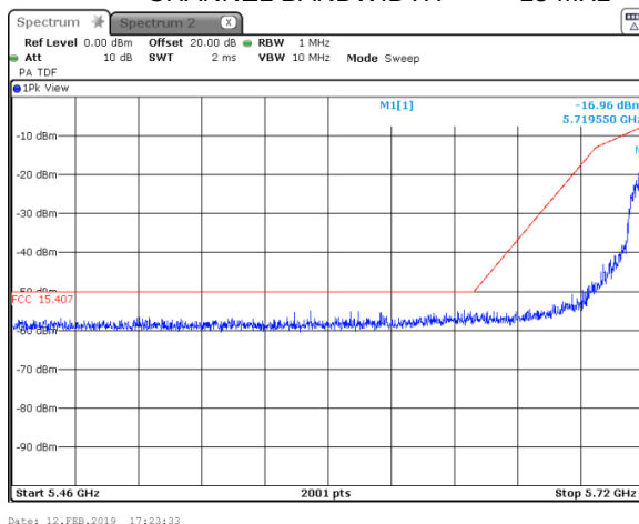
Plot 7.10.12 Conducted spurious emission measurements in the range 5.46 – 5.725 GHz
