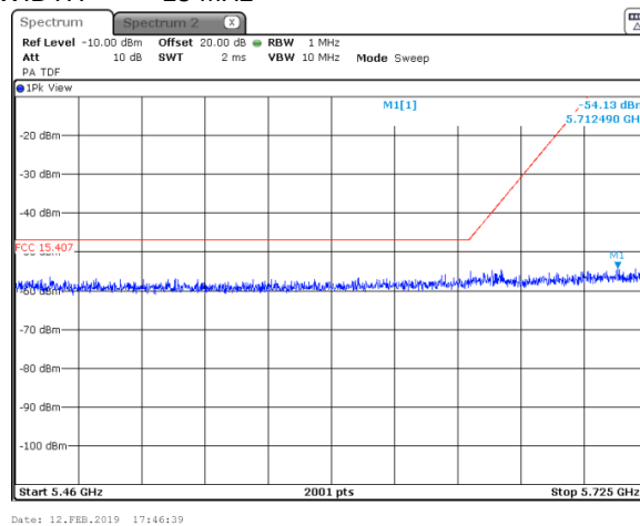
Plot 7.9.18 Conducted spurious emission measurements in the range 5.46 – 5.725 GHz
