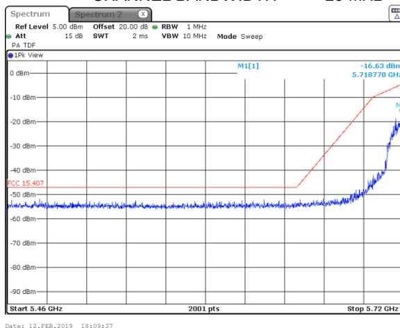
Plot 7.9.21 Conducted spurious emission measurements in the range 5.46 – 5.725 GHz
