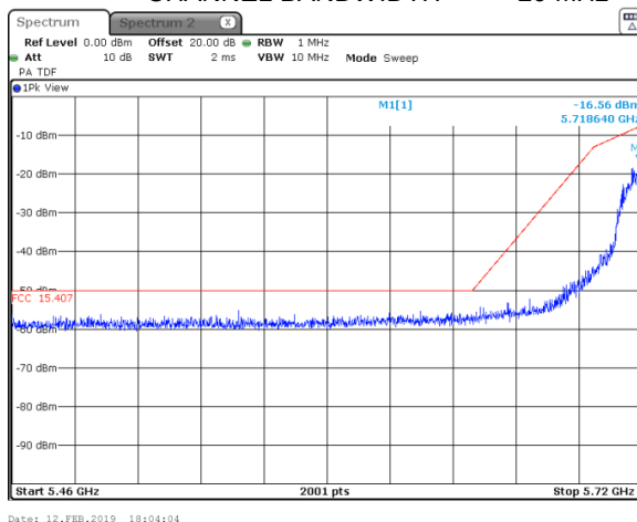
Plot 7.10.21 Conducted spurious emission measurements in the range 5.46 – 5.725 GHz
