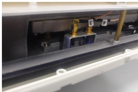
Photograph 7.16.1 Antenna assembly
