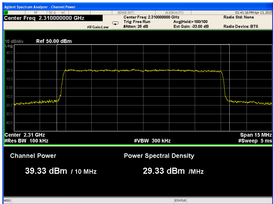
Figure 59. — 64QAM 2310.0 MHz, BW 10MHz Port I 1
