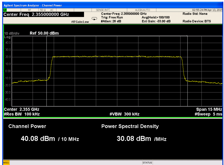
Figure 16. — QPSK - 2355.0 MHz, BW 10MHz Port 2
