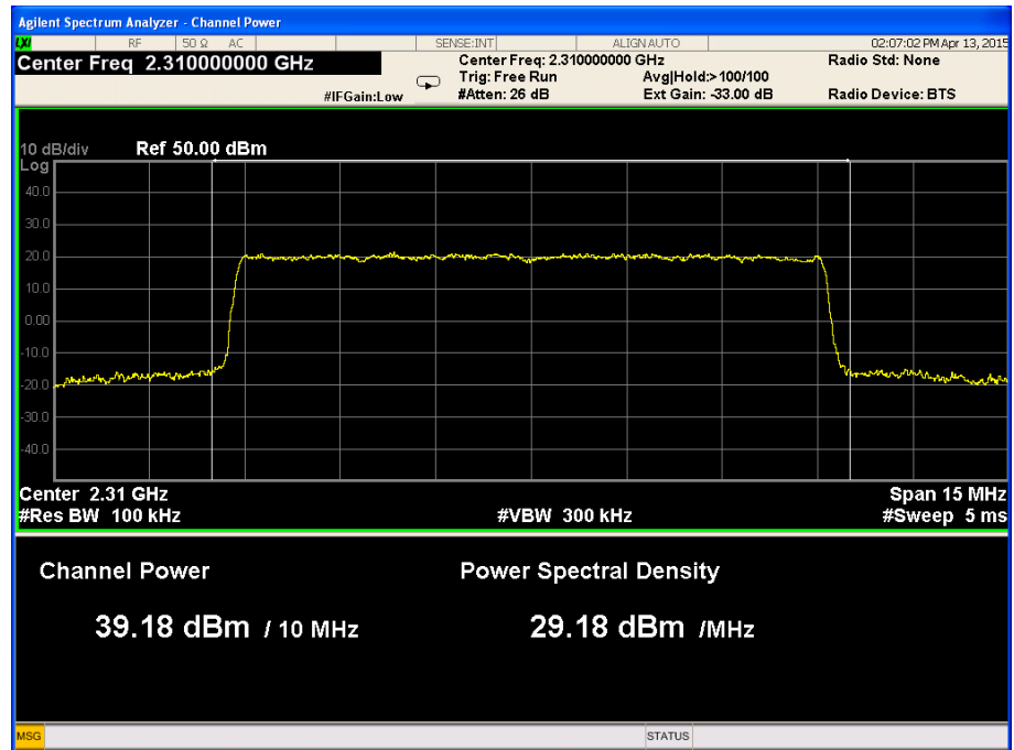
Figure 61. — 64QAM 2310.0 MHz, BW 10MHz Port 3
