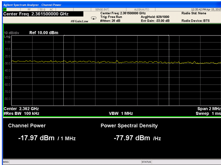
Figure 81. — 2361.0 MHz-2362.0 MHz
