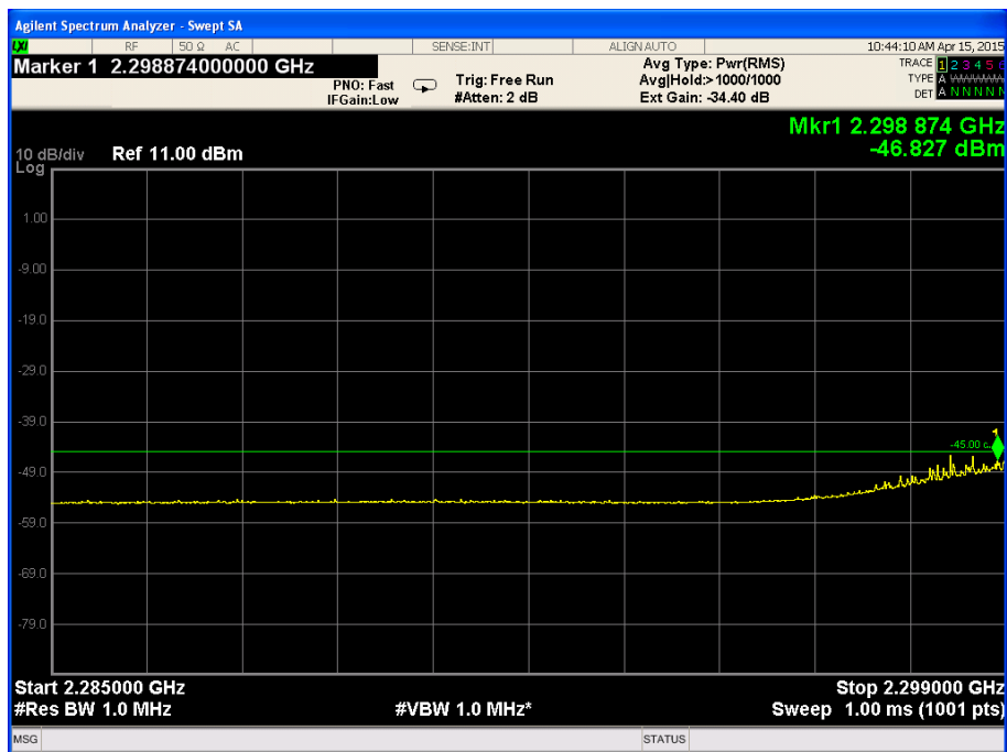
Figure 55. — 2285.0 MHz-2299.0 MHz
