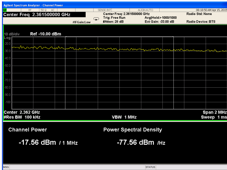
Figure 26. — 2361.0MHz-2362.0 MHz
