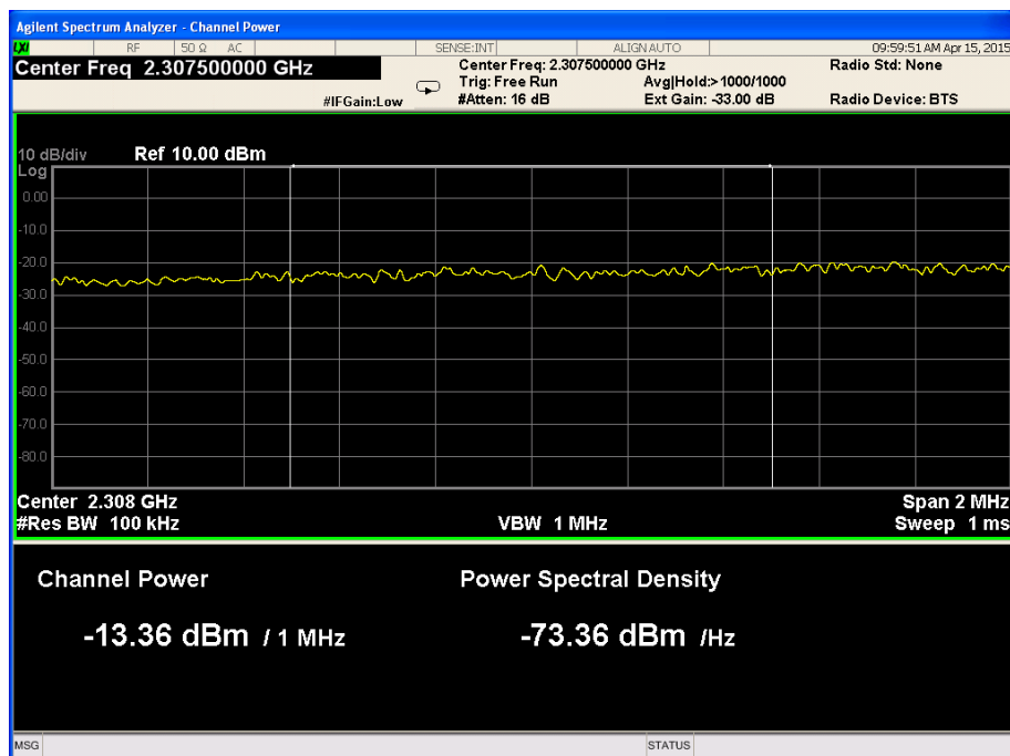
Figure 48. — 2307.0 MHz-2308.0 MHz
