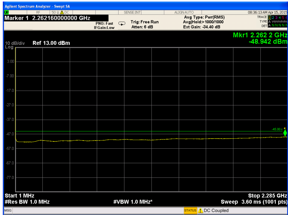
Figure 30. — 1.0 MHz-2285.0 MHz
