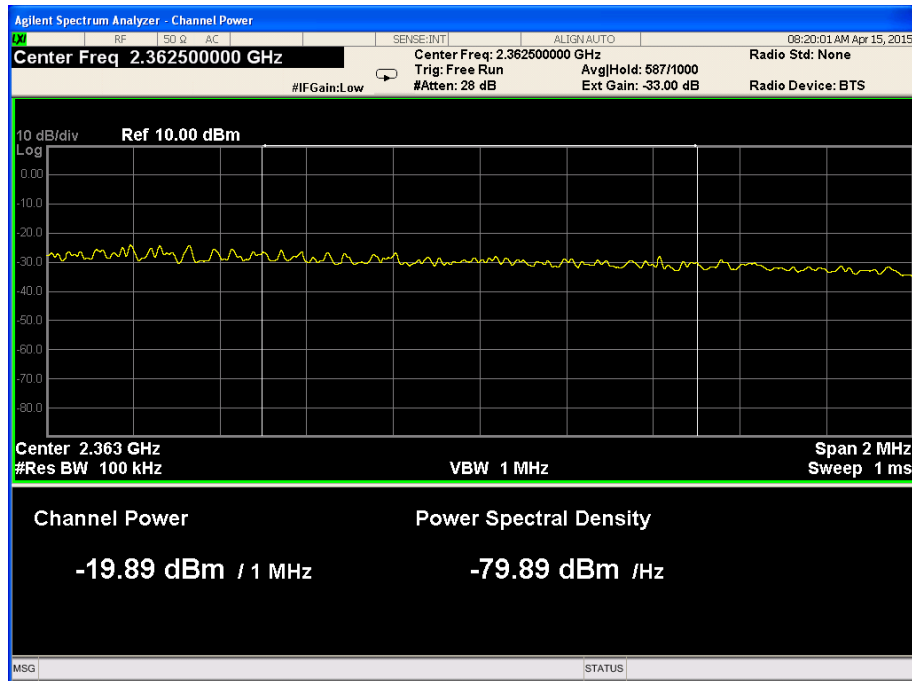
Figure 27. — 2362.0MHz-2363.0 MHz
