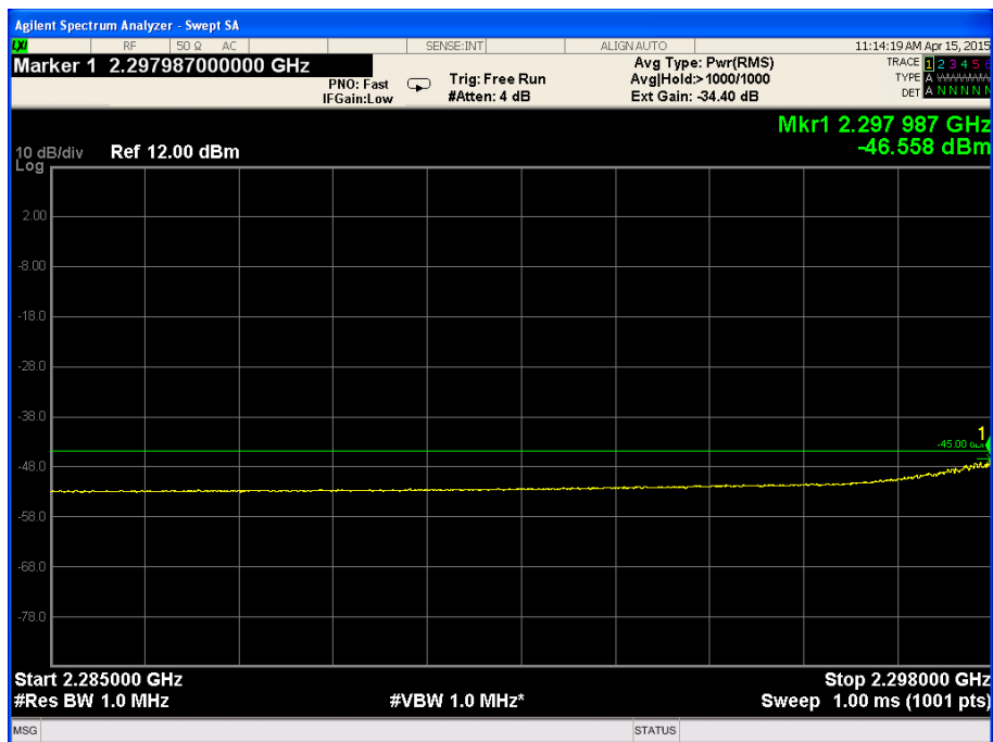
Figure 66. — 2285.0 MHz-2298.0 MHz
