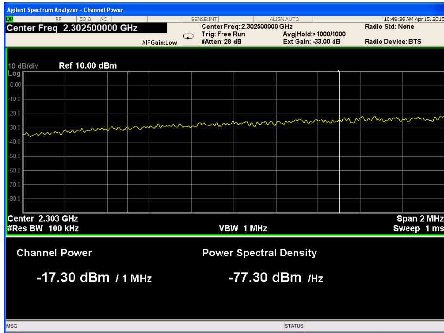
Figure 58. — 2302.0 MHz-2303.0 MHz
