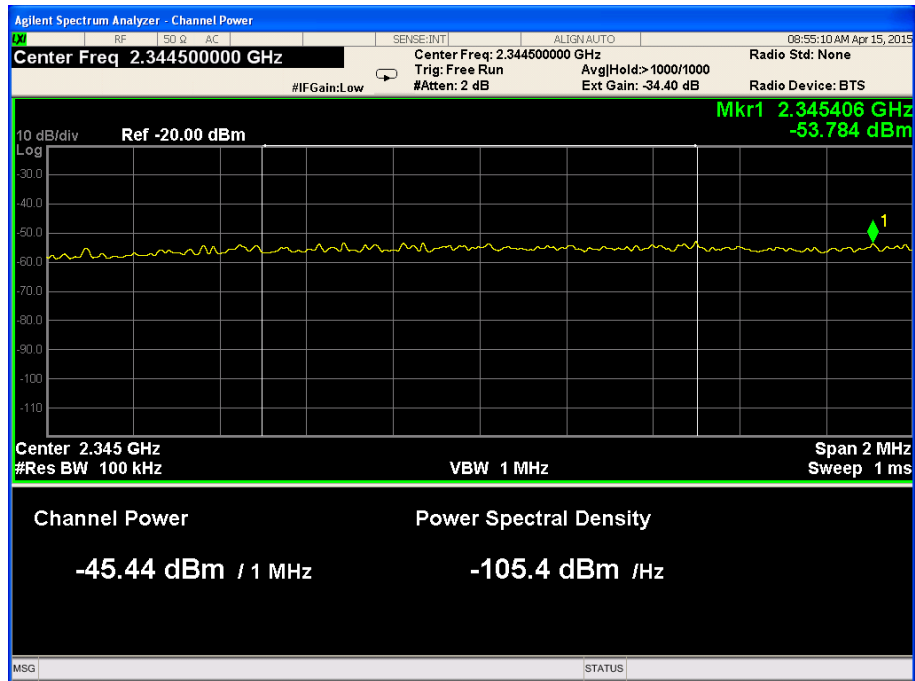
Figure 32. — 2344.0 MHz-2345.0 MHz
