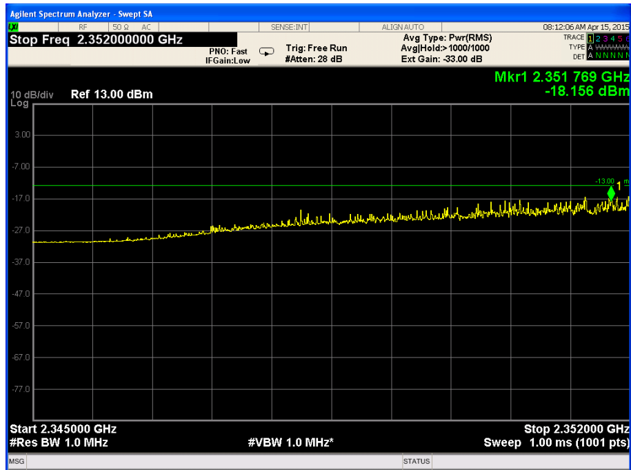
Figure 23. — 2345.0 MHz-2352.0 MHz
