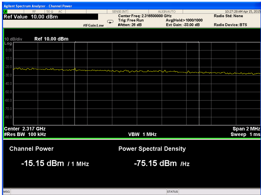
Figure 50. — 2316.0 MHz-2317.0 MHz
