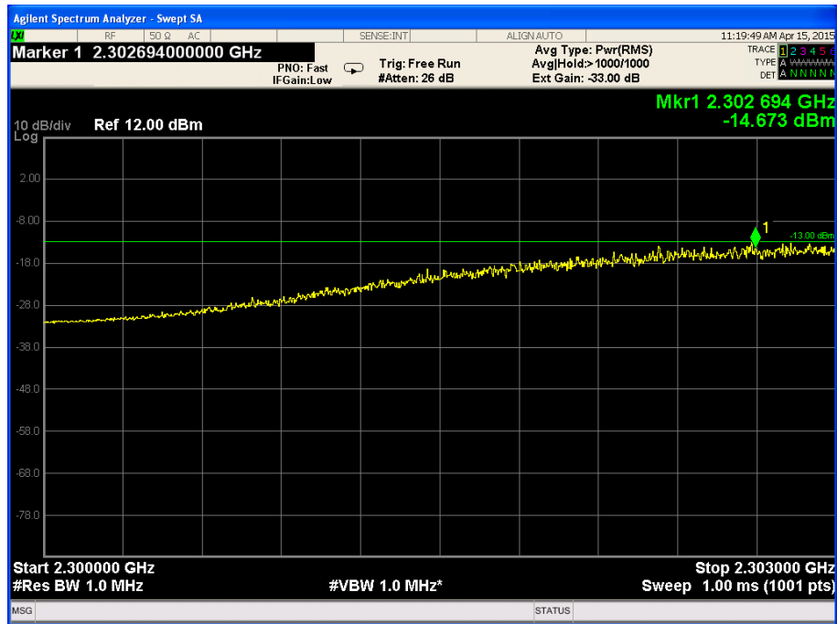
Figure 69. — 2300.0 MHz-2303.0 MHz
