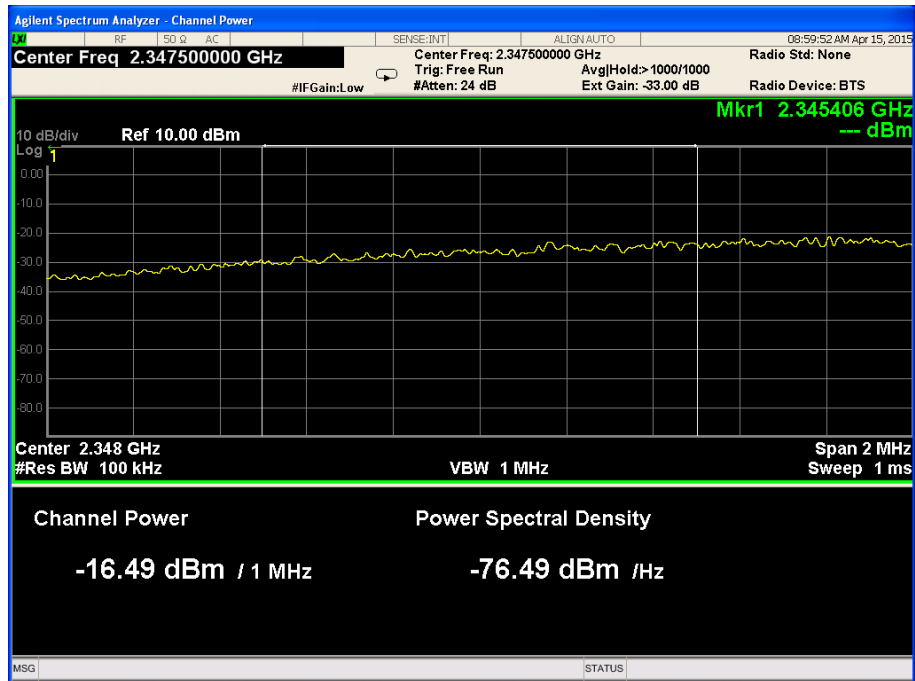
Figure 34. — 2347.0 MHz-2348.0 MHz
