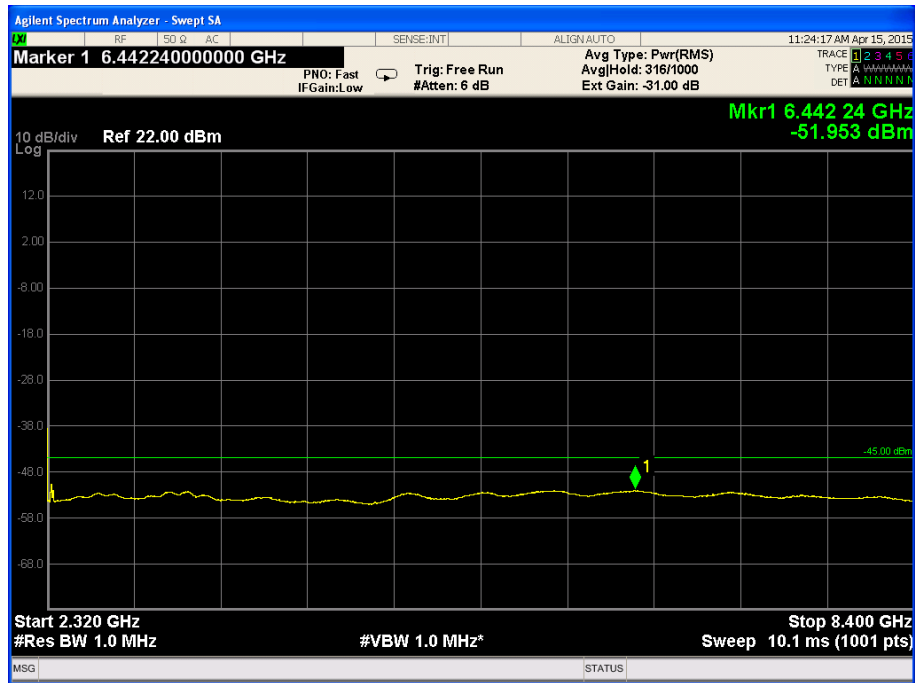
Figure 73. — 2320.0 MHz-8400.0 MHz
