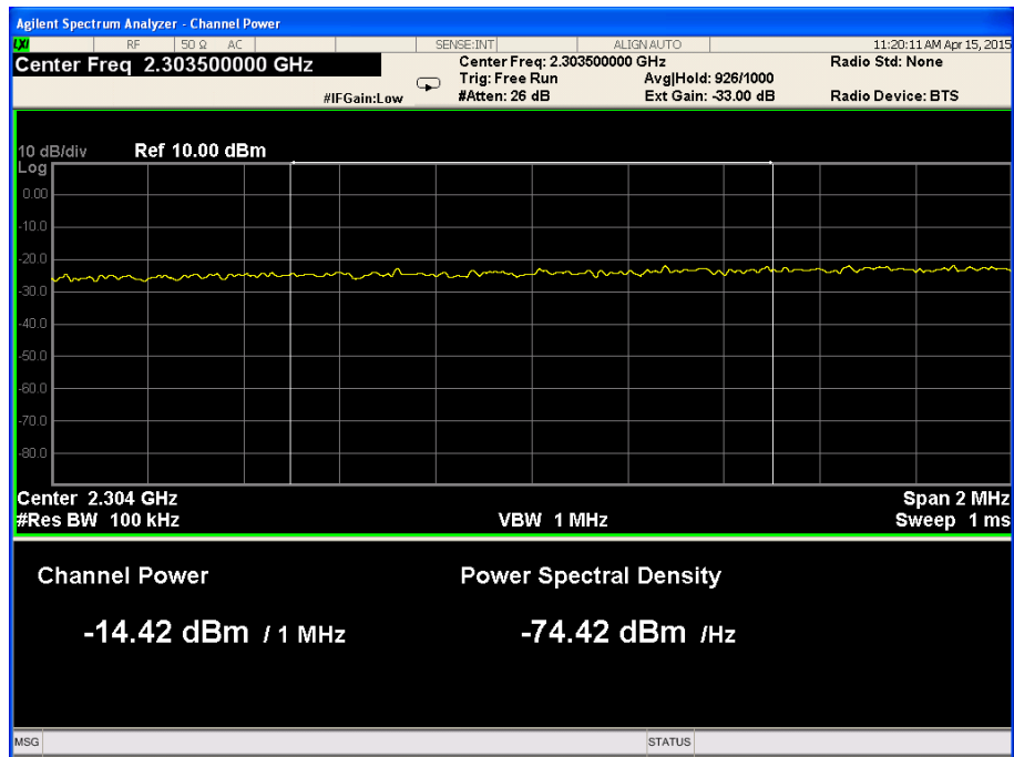
Figure 70. — 2303.0 MHz-2304.0 MHz
