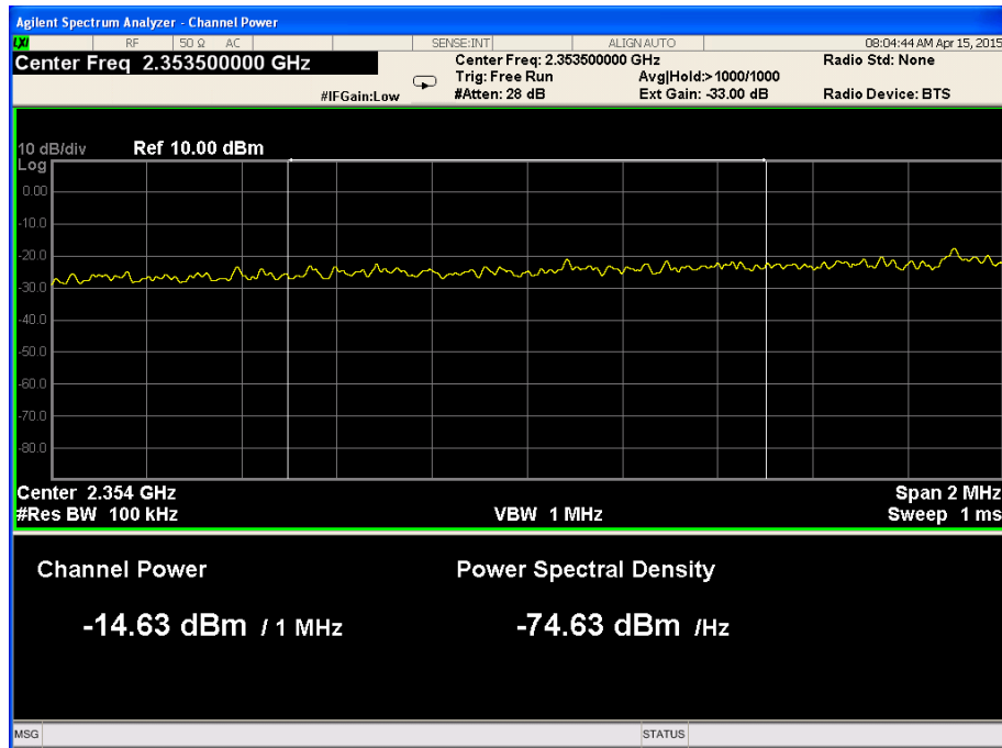
Figure 25. — 2353.0 MHz-2354.0 MHz
