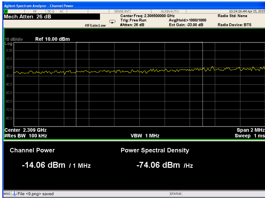
Figure 49. — 2308.0 MHz-2309.0 MHz
