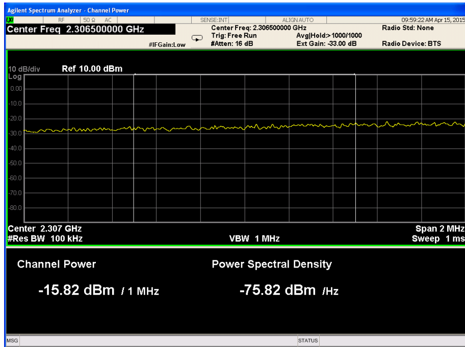
Figure 47. — 2306.0 MHz-2307.0 MHz
