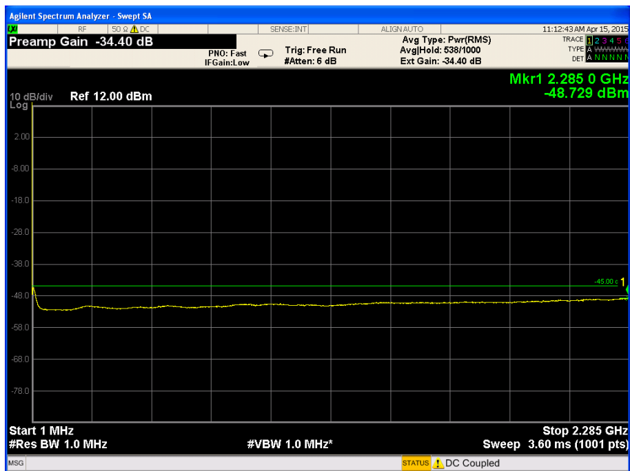
Figure 65. — 1.0 MHz-2285.0 MHz
