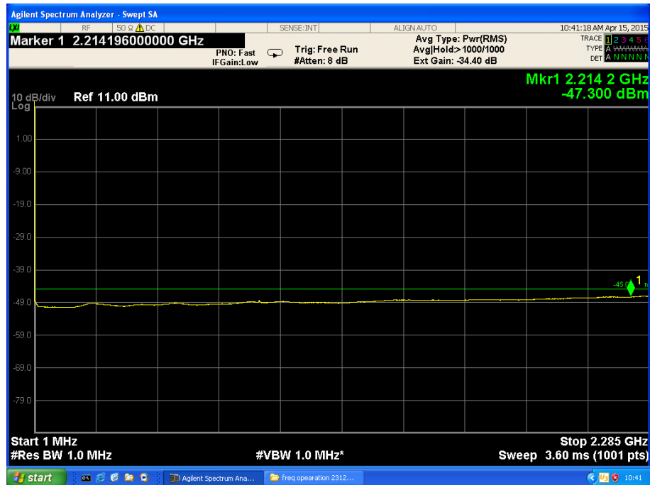
Figure 54. — 1.0 MHz-2285.0 MHz
