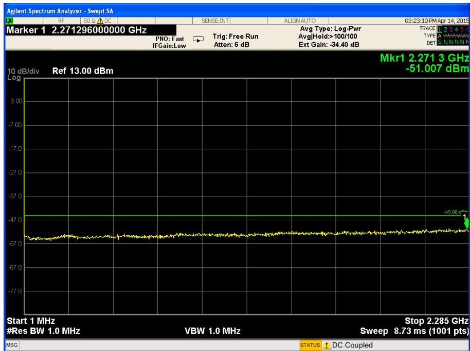
Figure 21. — 1.0 MHz-2285.0 MHz
