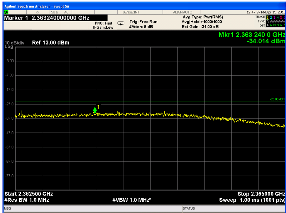
Figure 83. — 2362.5 MHz-2365.0 MHz
