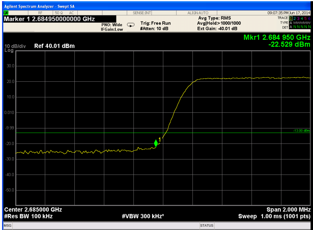
Figure 207.— 2687.50 MHz 64QAM
