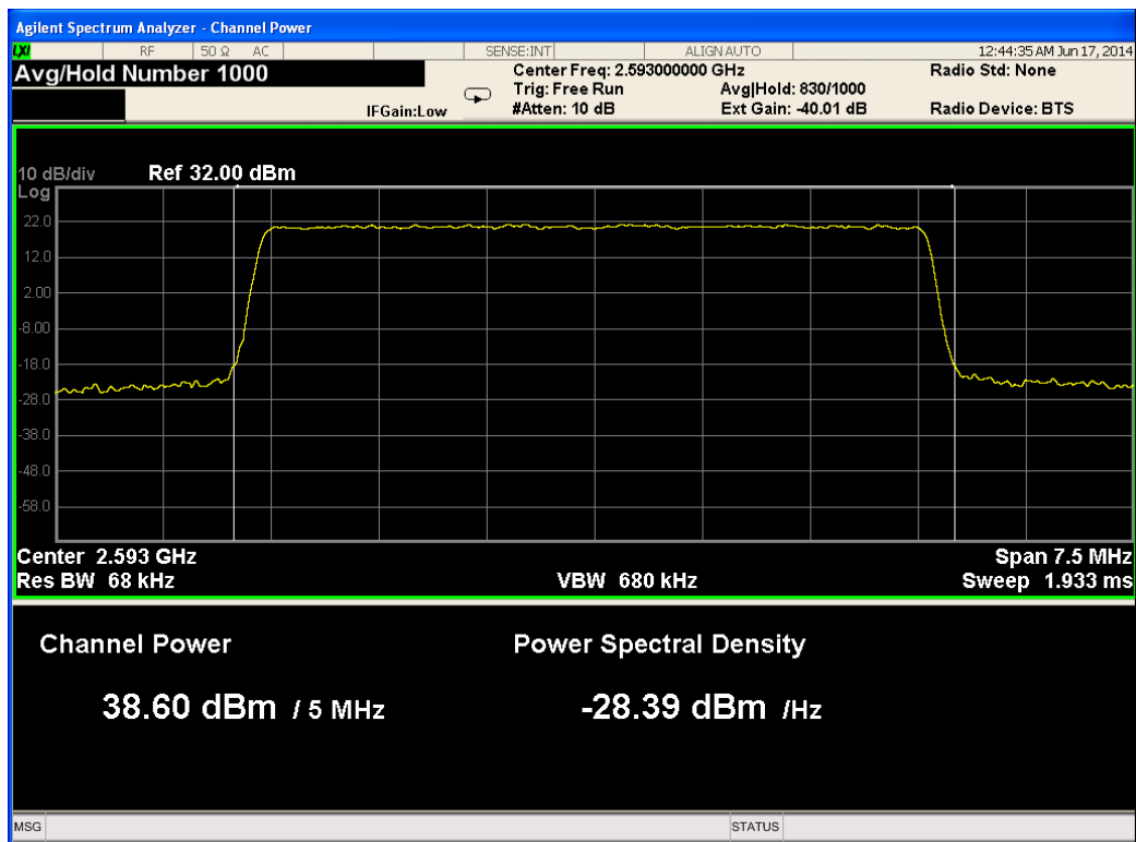
Figure 98.— 2593.00 MHz QPSK Port 4
