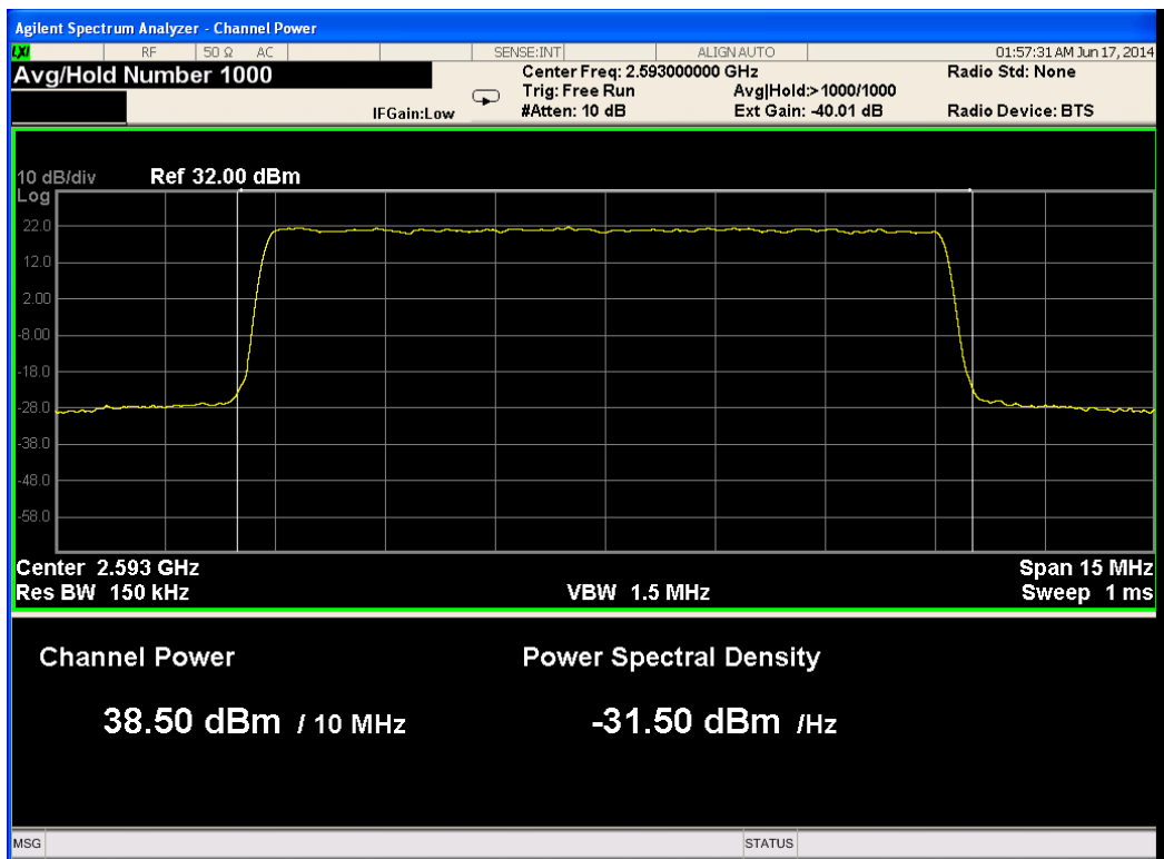
Figure 62.— 2593.00 MHz QPSK Port 4
