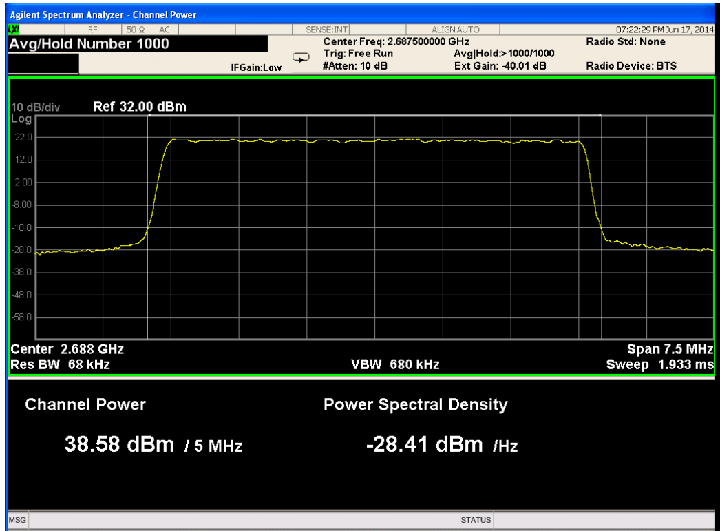
Figure 113.— 2687.50 MHz 16QAM Port 3
