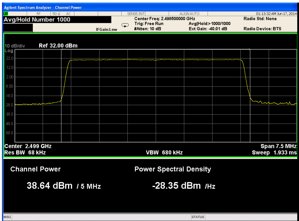
Figure 10.— 2498.50 MHz QPSK Port 2
