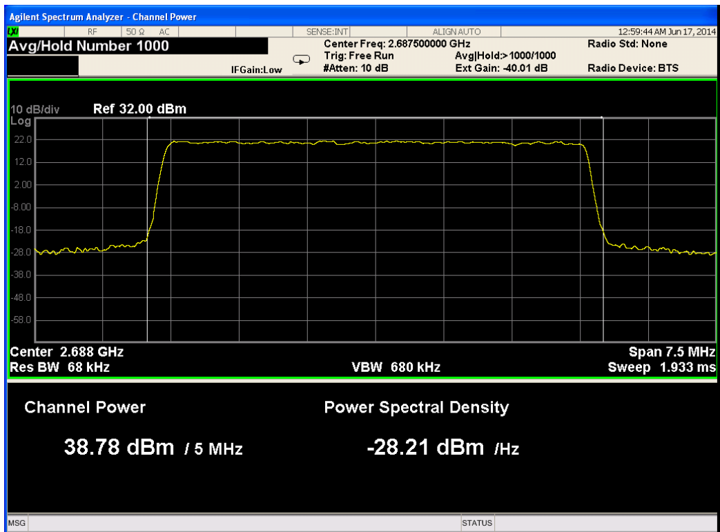
Figure 112.— 2687.50 MHz 16QAM Port 2
