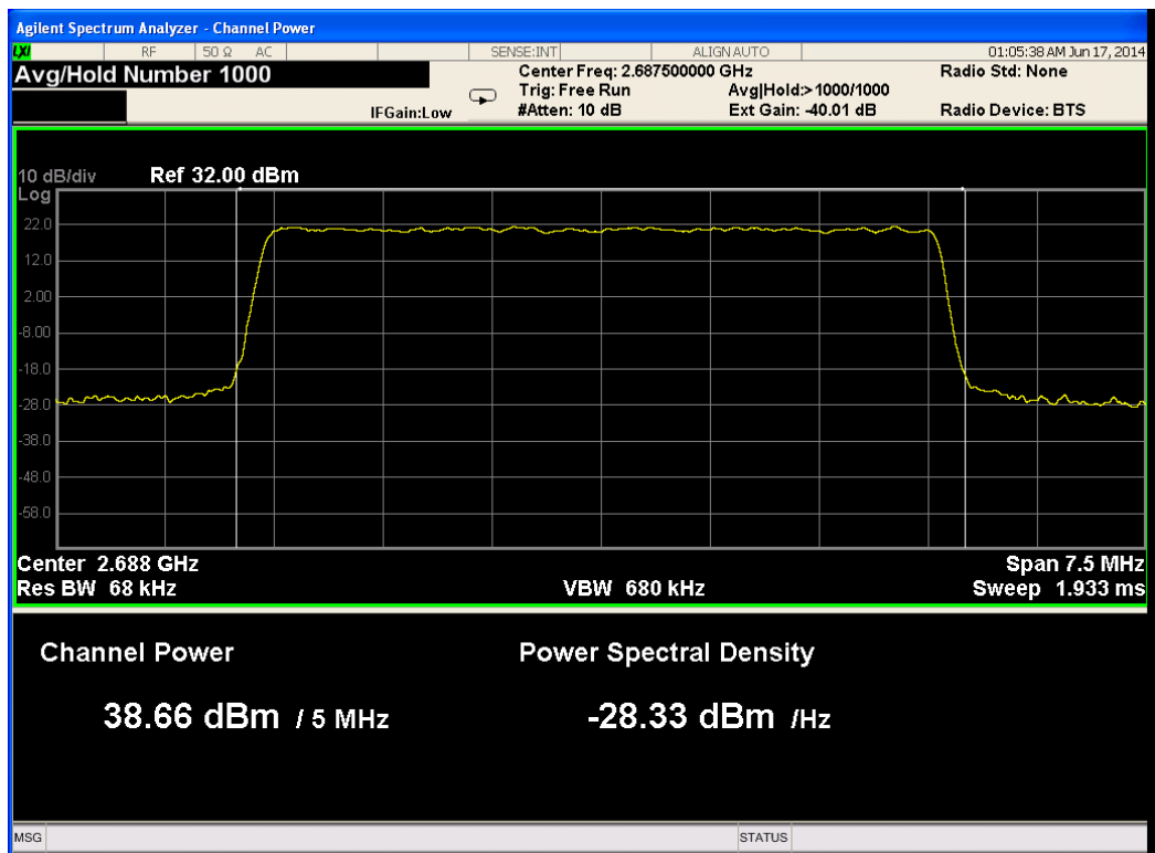
Figure 114.— 2687.50 MHz 16QAM Port 4
