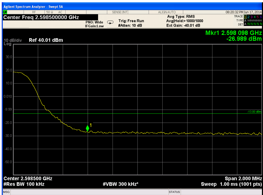
Figure 216.— 2593.00 MHz QPSK
