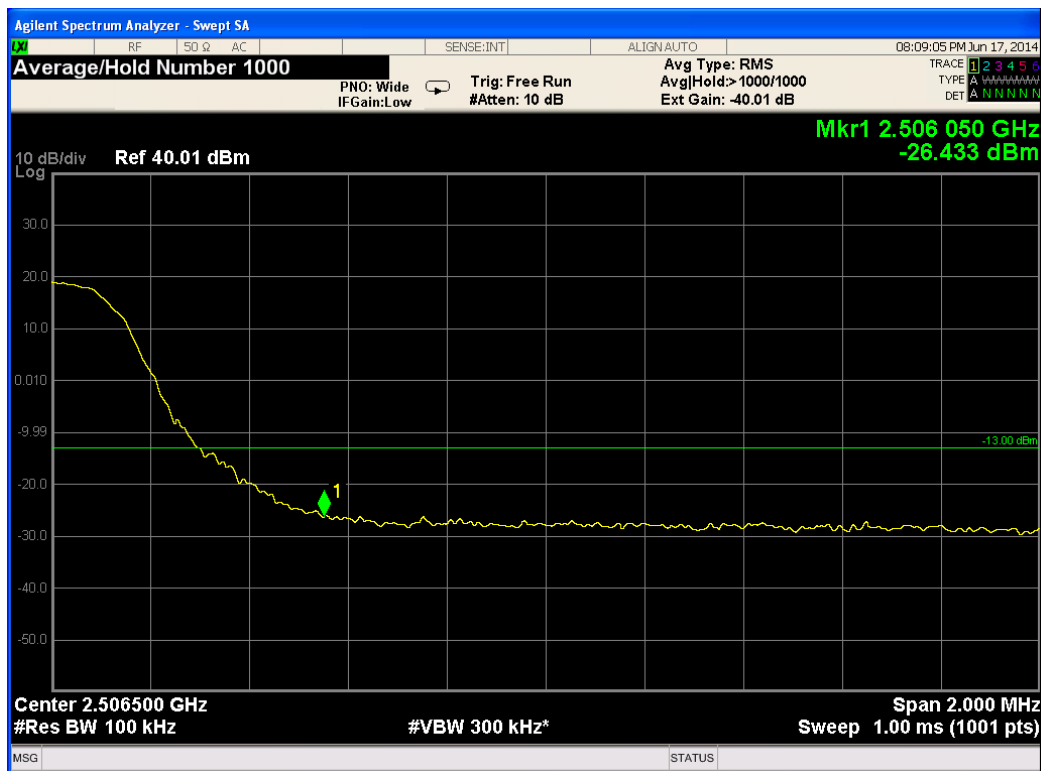
Figure 212.— 2501.00 MHz 16QAm
