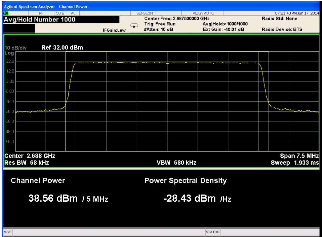
Figure 35.— 2687.50 MHz QPSK Port 3
