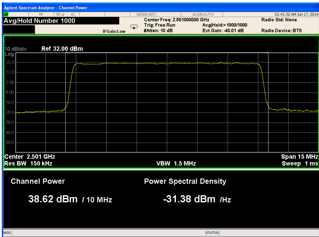
Figure 54.— 2501.00 MHz 16QAM Port 4
