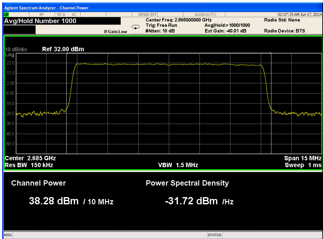
Figure 152.— 2685.00 MHz 64QAM Port 2
