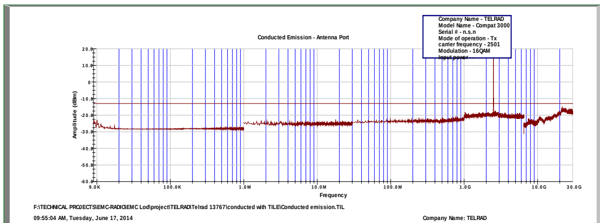
Figure 183.— 2501.00 MHz 16QAM
