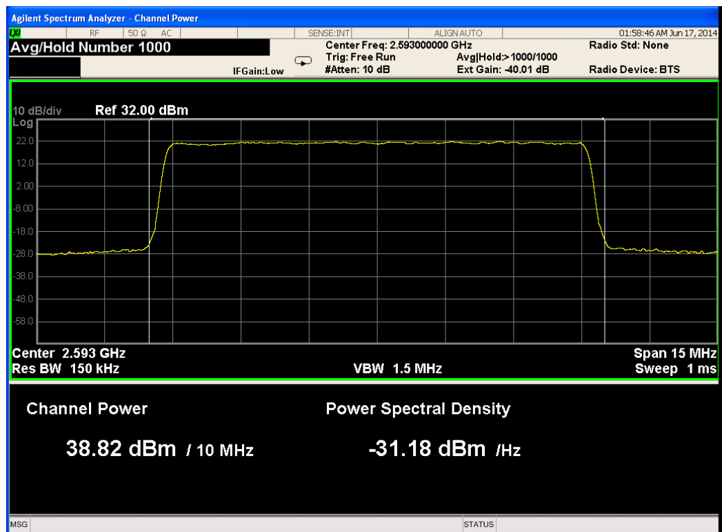
Figure 138.— 2593.00 MHz 16QAM Port 4
