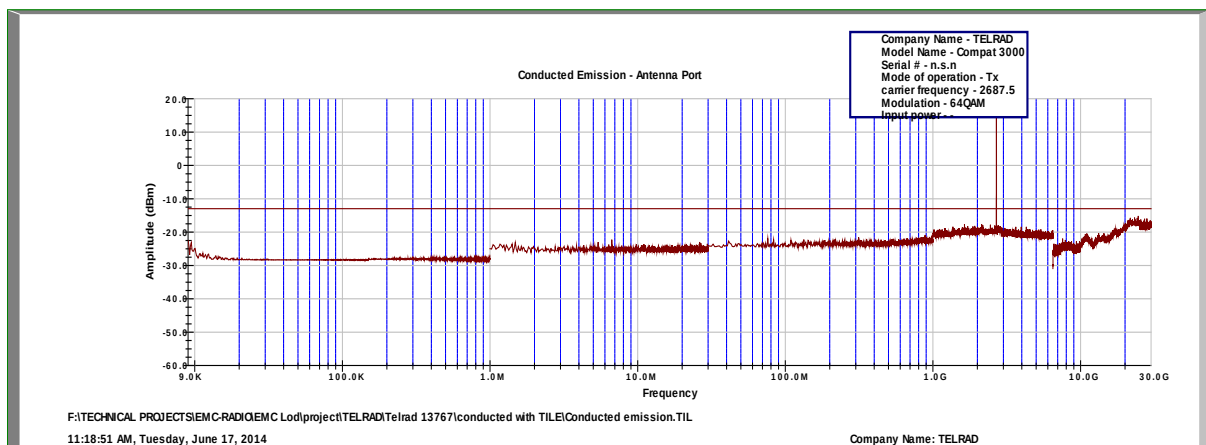
Figure 181.— 2687.50 MHz 64QAM
