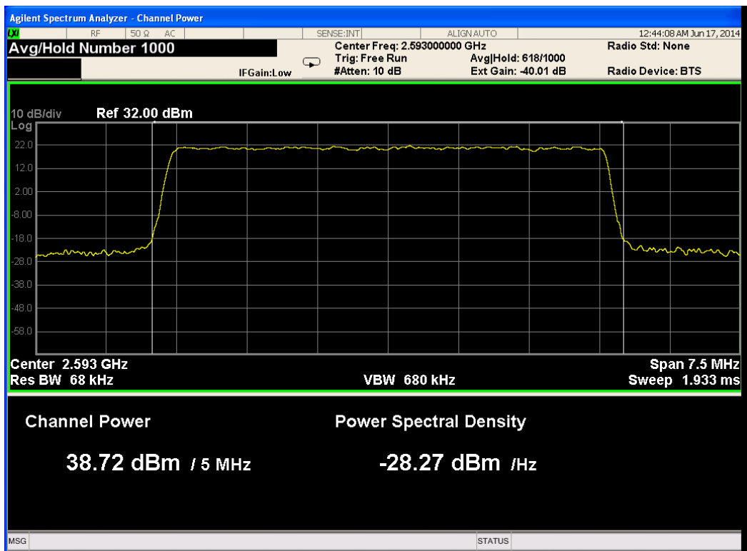
Figure 28.— 2593.00 MHz 16QAM Port 4
