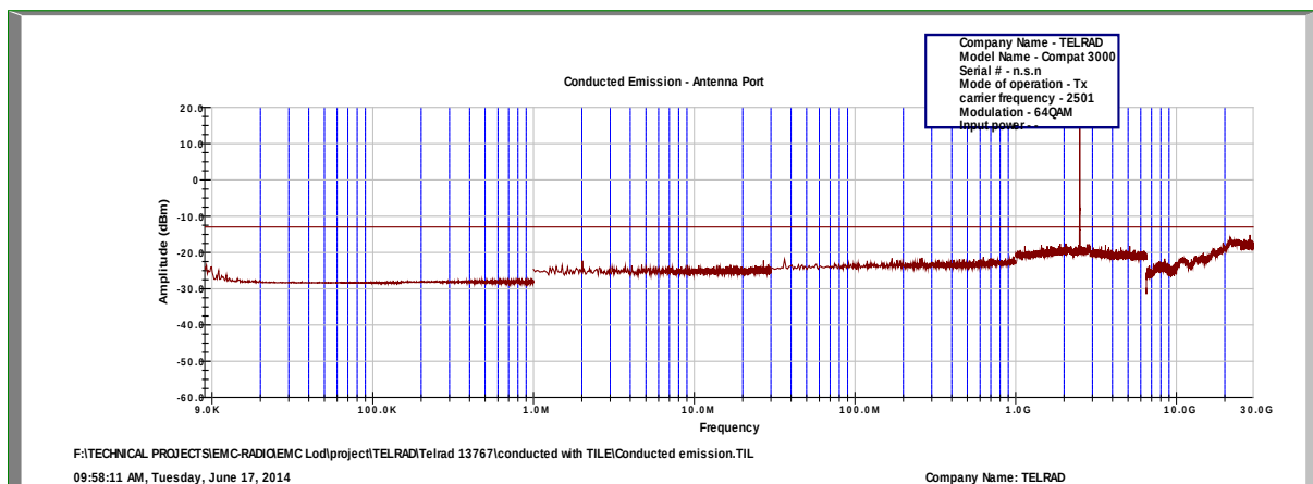
Figure 184.— 2501.00 MHz 64QAM
