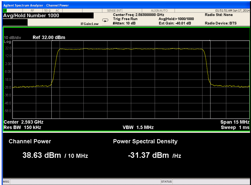
Figure 136.— 2593.00 MHz 16QAM Port 2
