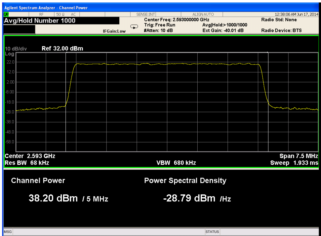
Figure 26.— 2593.00 MHz 16QAM Port 2
