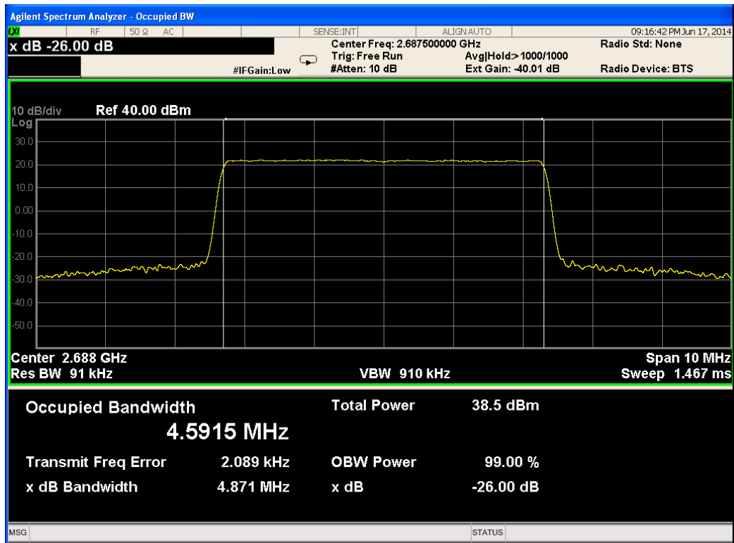
Figure 161.— 2687.50 MHz QPSK
