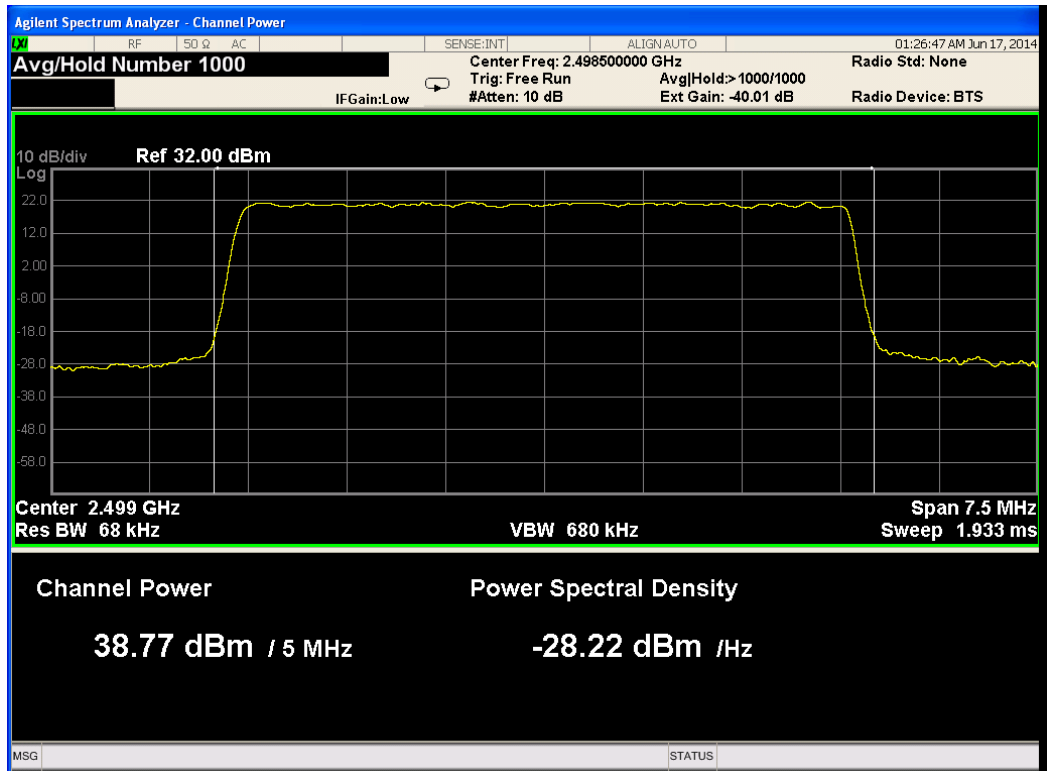
Figure 89.— 2498.50 MHz 16QAM Port3
