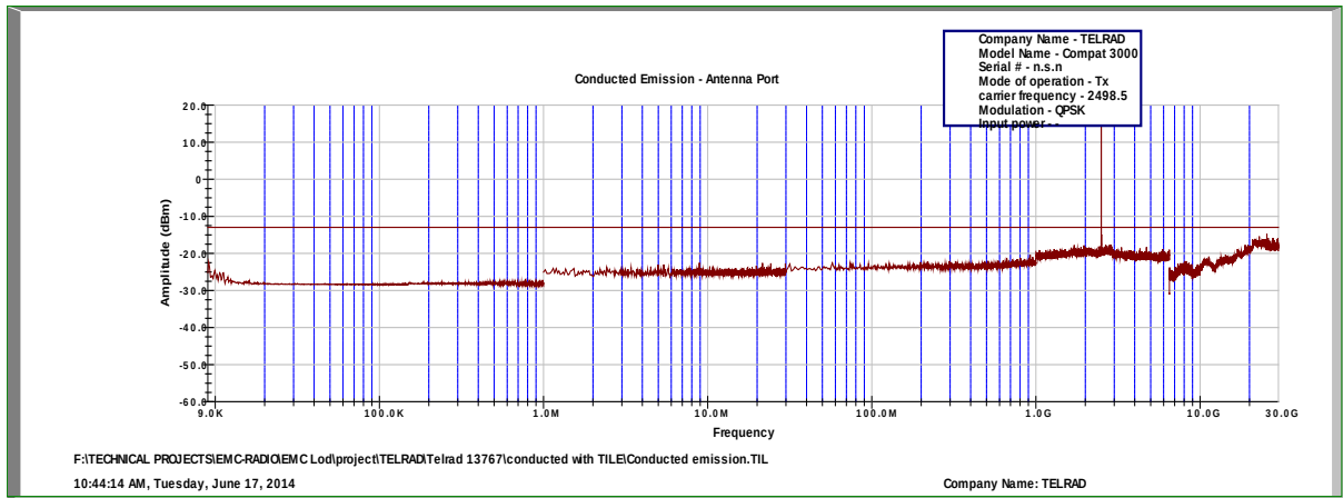
Figure 173.— 2498.50 MHz QPSK
