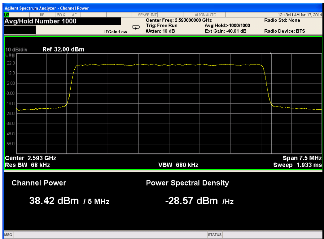
Figure 32.— 2593.00 MHz 64QAM Port 4
