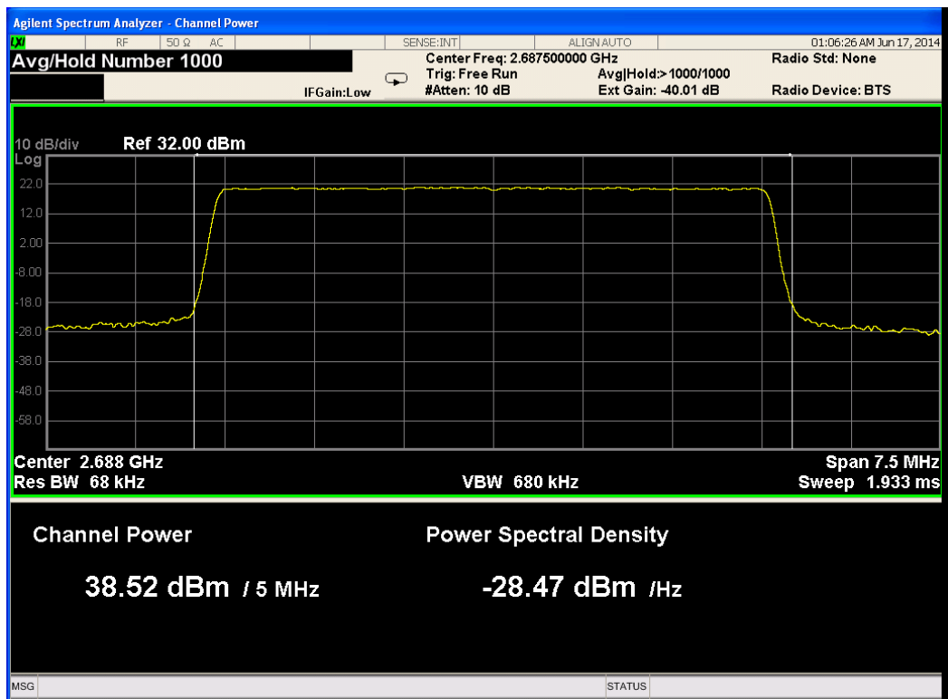
Figure 36.— 2687.50 MHz QPSK Port 4
