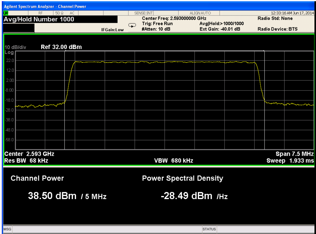
Figure 99.— 2593.00 MHz 16QAM Port 1
