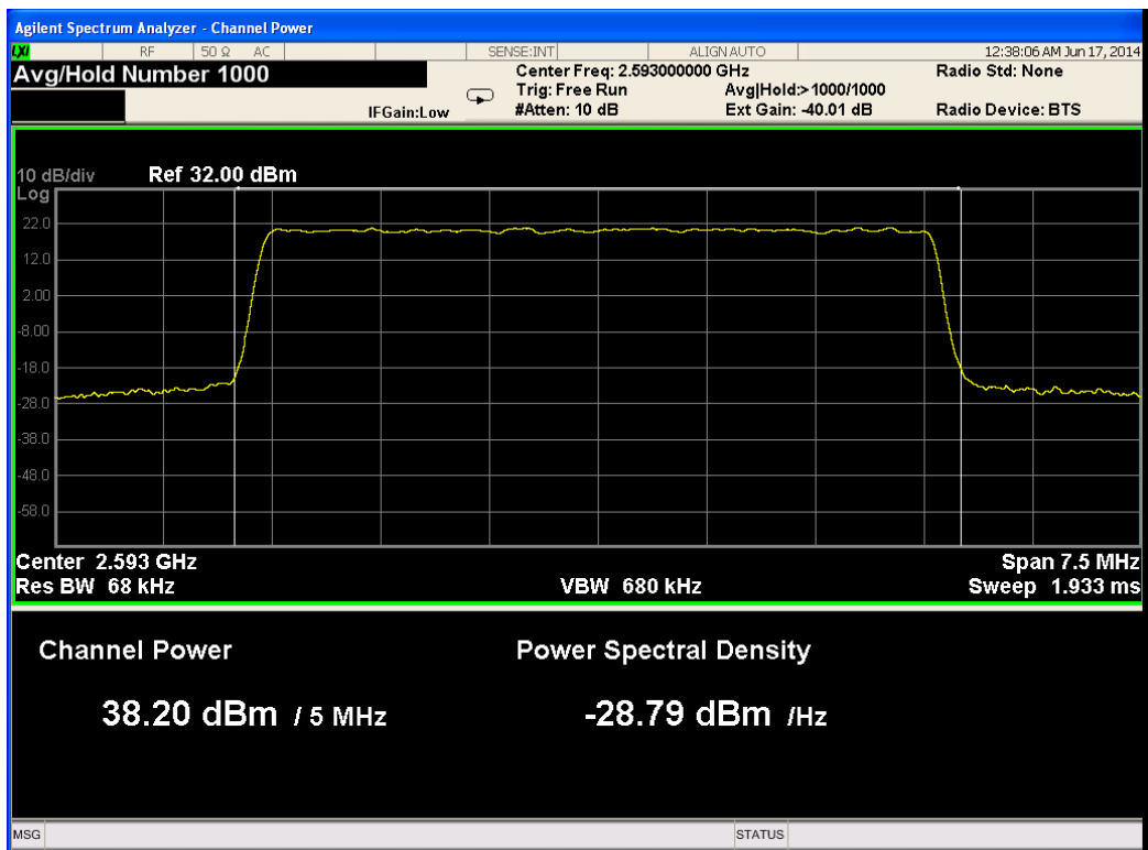
Figure 100.— 2593.00 MHz 16QAM Port 2
