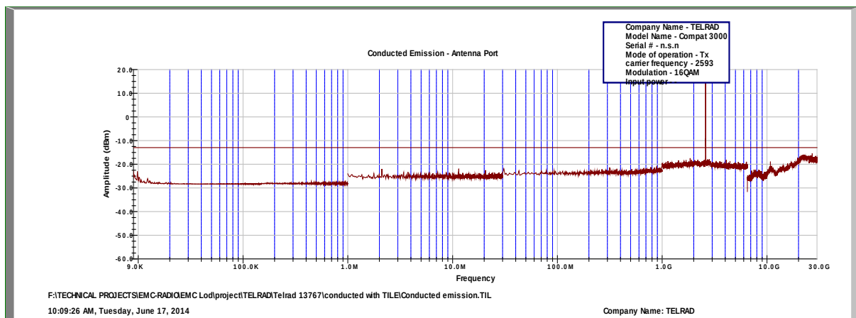
Figure 186.— 2593.00 MHz 16QAM
