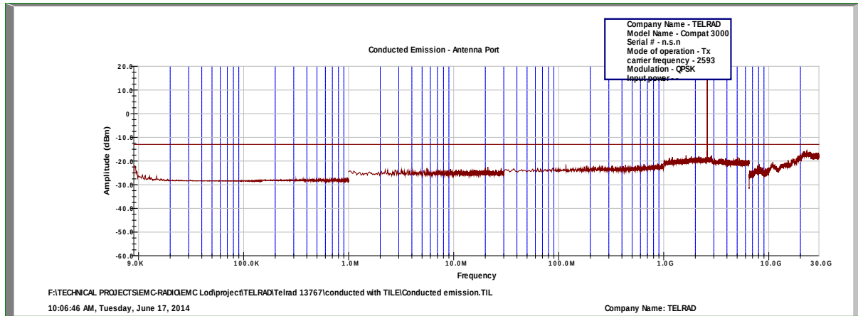
Figure 185.— 2593.00 MHz QPSK
