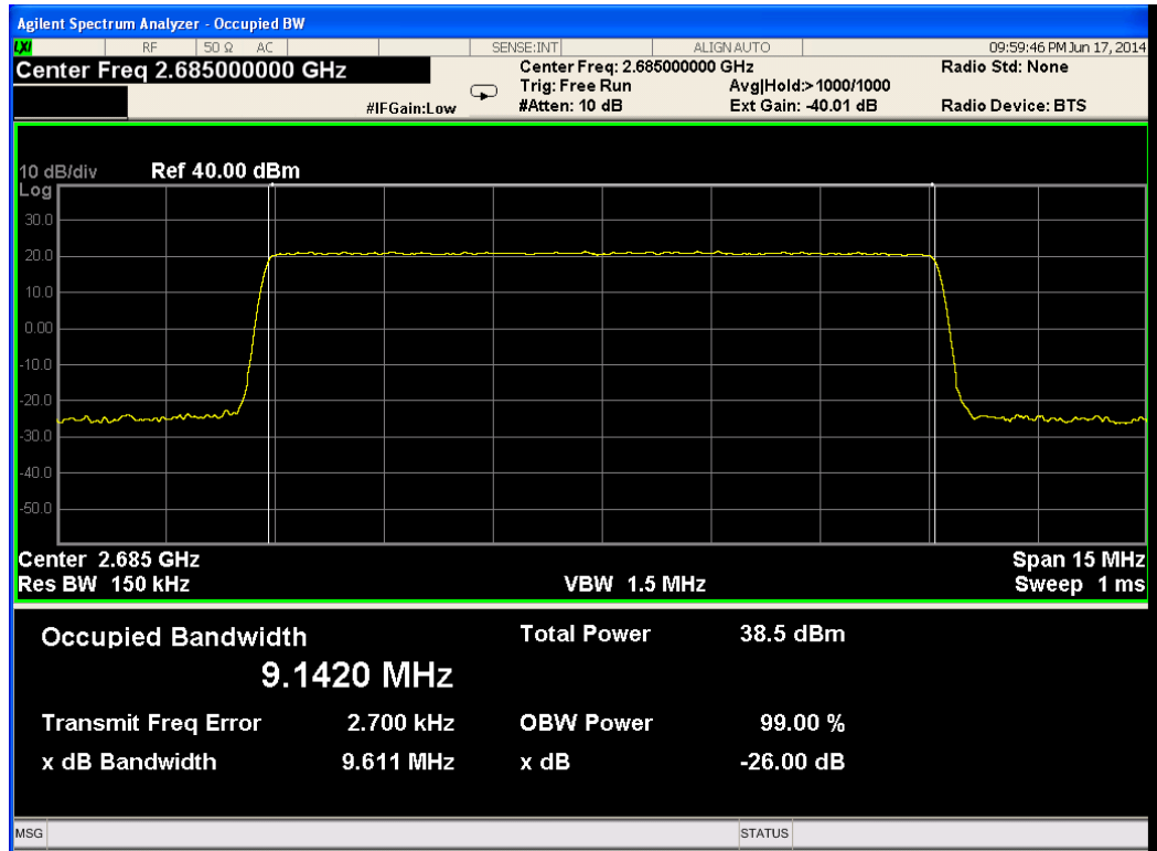
Figure 170.— 2685.00 MHz QPSK
