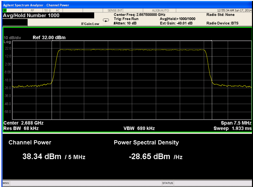
Figure 33.— 2687.50 MHz QPSK Port 1
