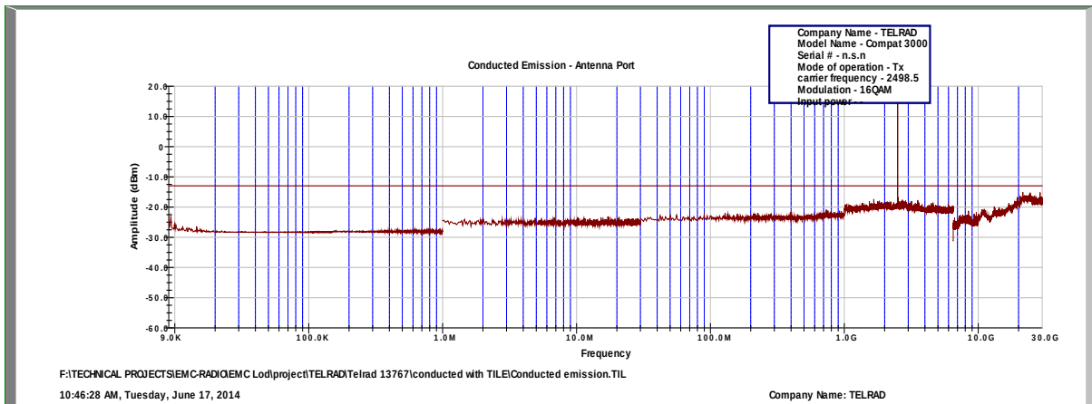
Figure 174.— 2498.50 MHz 16QAM
