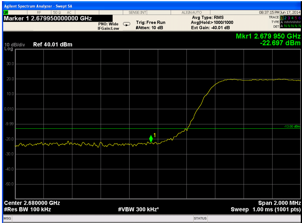
Figure 225.— 2685.00 MHz 64QAM
