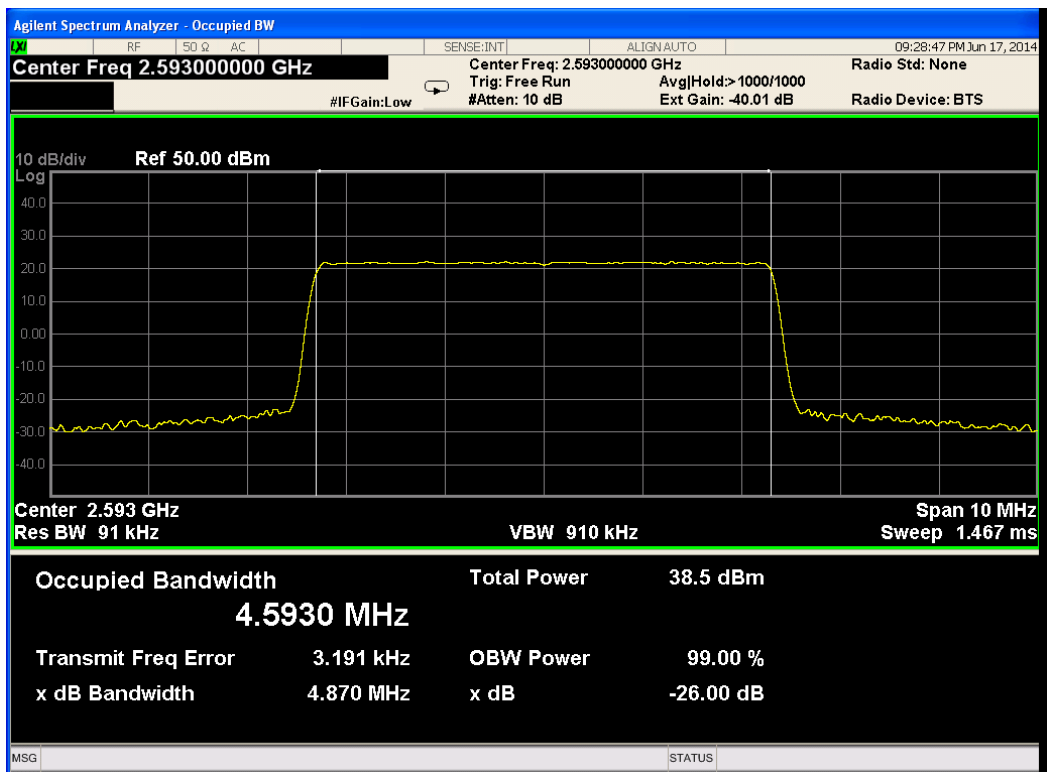
Figure 158.— 2593.00 MHz QPSK
