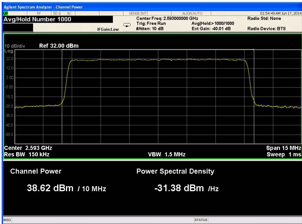
Figure 137.— 2593.00 MHz 16QAM Port 3
