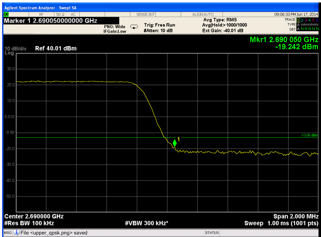
Figure 206.— 2687.50 MHz 16QAM
