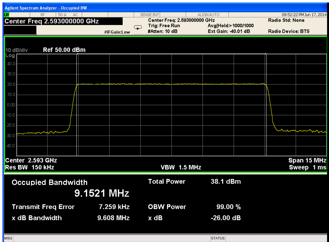
Figure 167.— 2593.00 MHz QPSK
