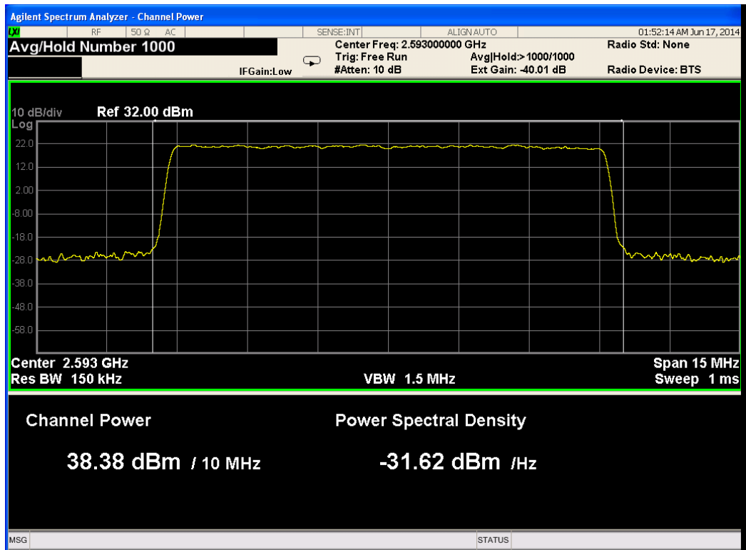
Figure 68.— 2593.00 MHz 64QAM Port 2
