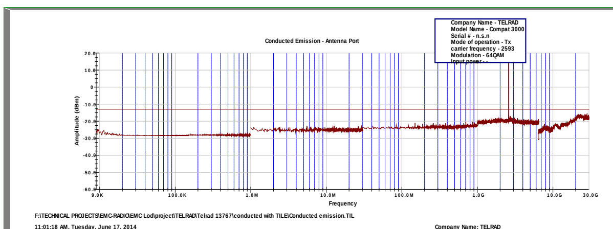
Figure 178.— 2593.00 MHz 64QAM
