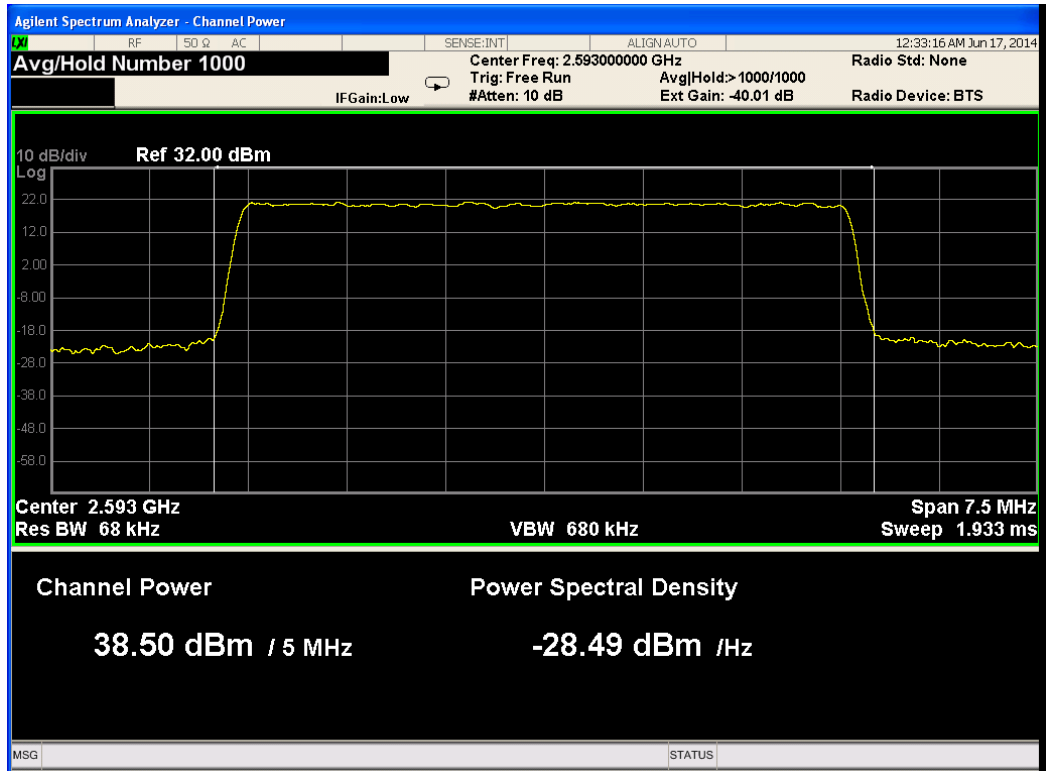
Figure 25.— 2593.00 MHz 16QAM Port 1
