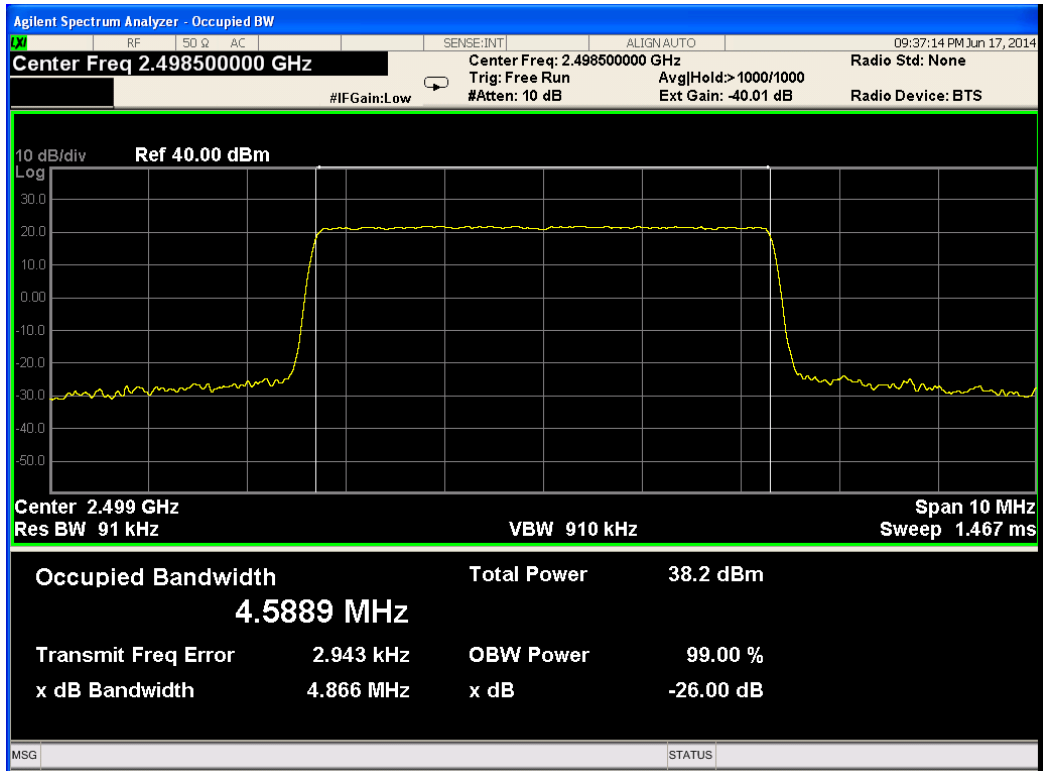
Figure 155.— 2498.50 MHz QPSK
