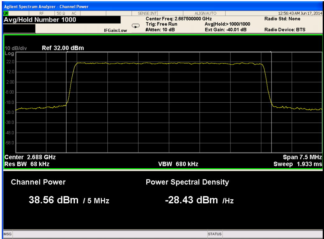
Figure 111.— 2687.50 MHz 16QAM Port 1
