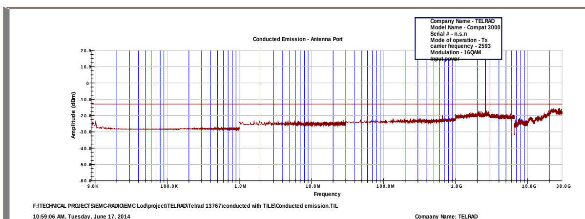
Figure 177.— 2593.00 MHz 16QAM
