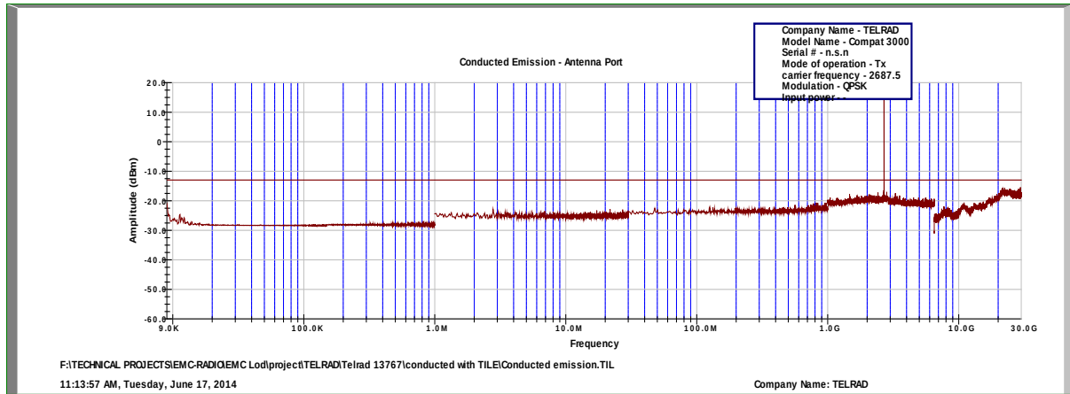
Figure 179.— 2687.50 MHz QPSK
