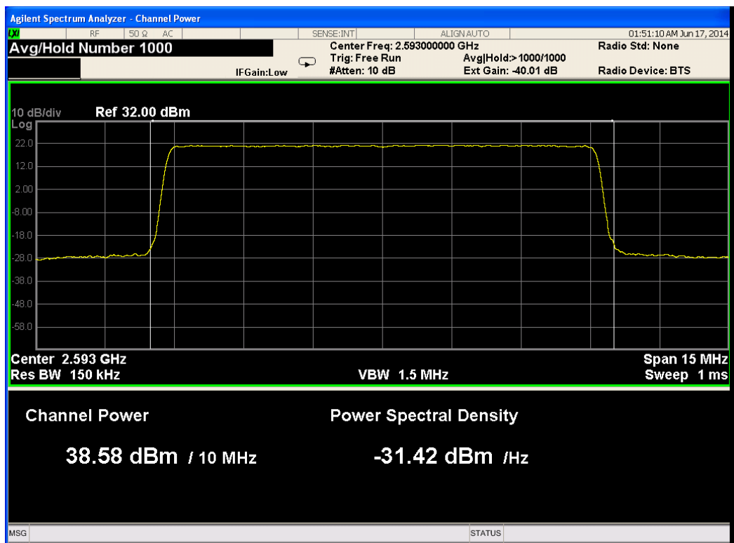
Figure 60.— 2593.00 MHz QPSK Port 2
