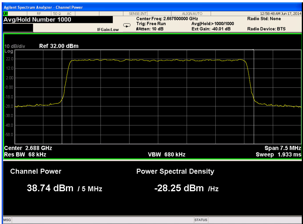
Figure 34.— 2687.50 MHz QPSK Port 2
