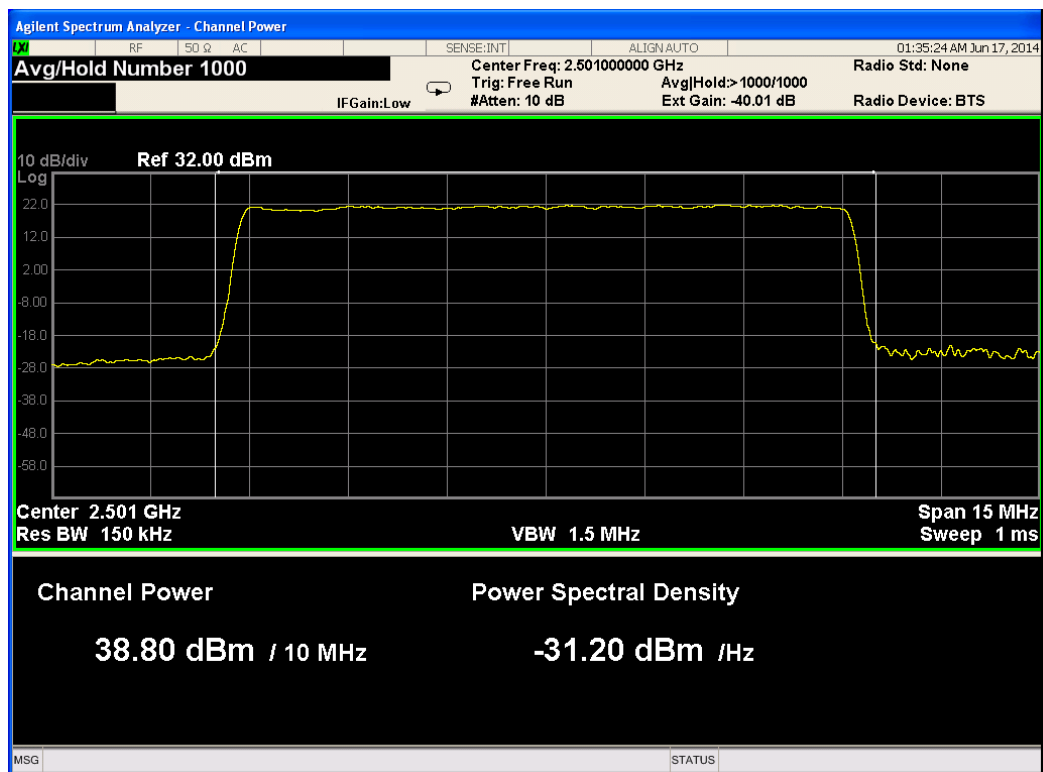
Figure 52.— 2501.00 MHz 16QAM Port 2
