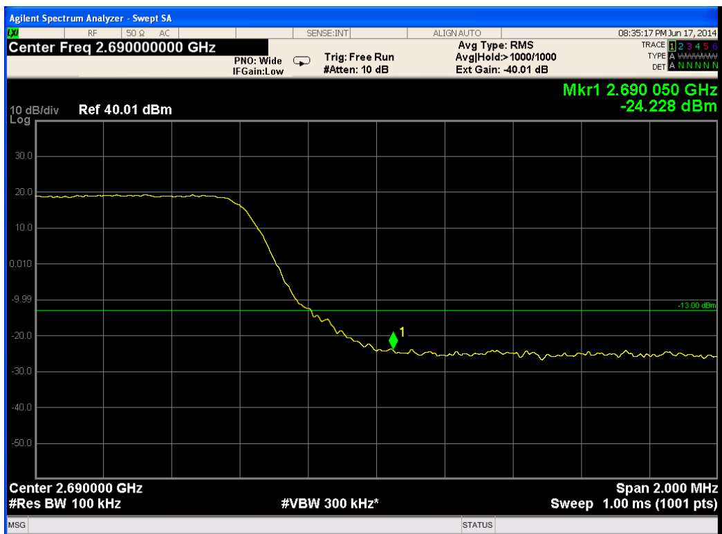
Figure 222.— 2685.00 MHz QPSK
