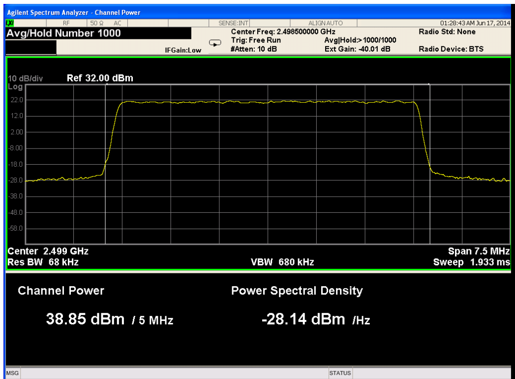
Figure 16.— 2498.5. MHz 16QAM Port4
