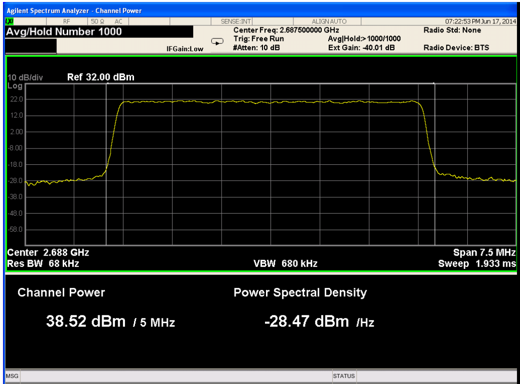
Figure 43.— 2687.50 MHz 64QAM Port 3
