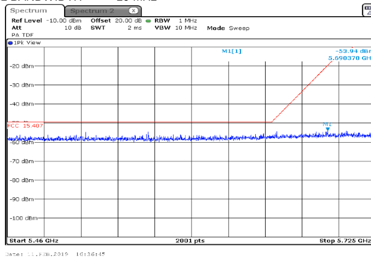
Plot 7.10.9 Conducted spurious emission measurements in the range 5.46 – 5.725 GHz
