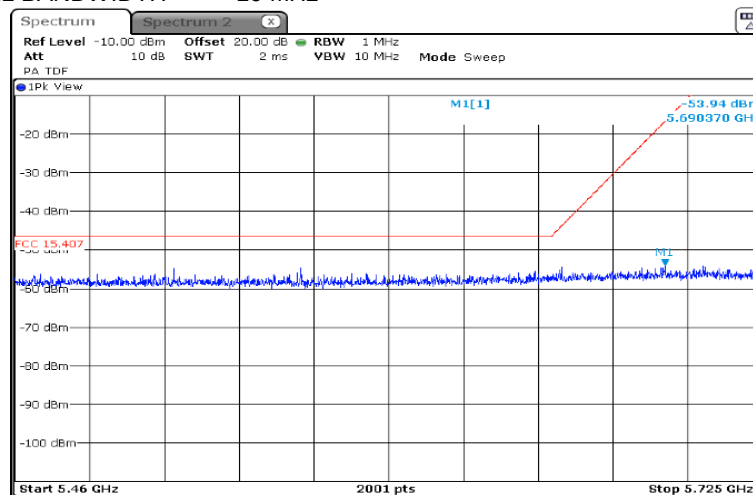
Plot 7.9.9 Conducted spurious emission measurements in the range 5.46 – 5.725 GHz
