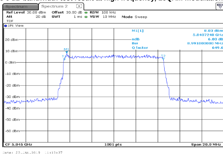
Plot 7.1.8 The 6 dB bandwidth test result at high frequency, 16QAM modulation, 10 MHz EBW
