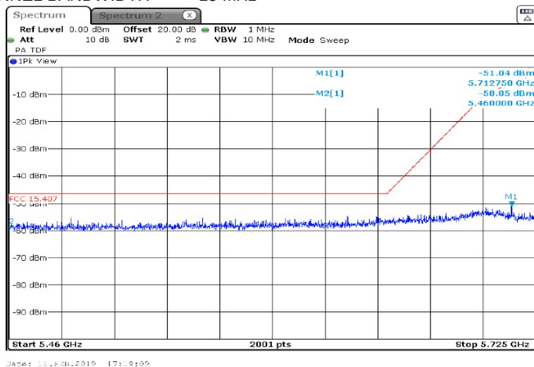
Plot 7.7.15 Conducted spurious emission measurements in the range 5.46 – 5.725 GHz
