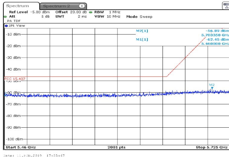
Plot 7.7.18 Conducted spurious emission measurements in the range 5.46 – 5.725 GHz
