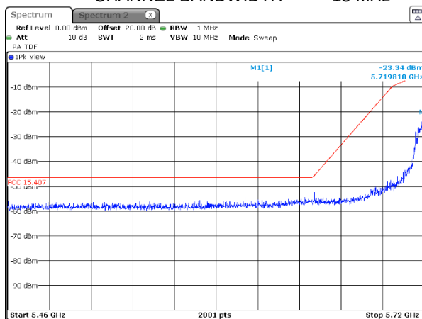
Plot 7.7.12 Conducted spurious emission measurements in the range 5.46 – 5.725 GHz CARRIER FREQUENCY 5732.5 MHz CHANNEL BANDWIDTH 15 MHz
