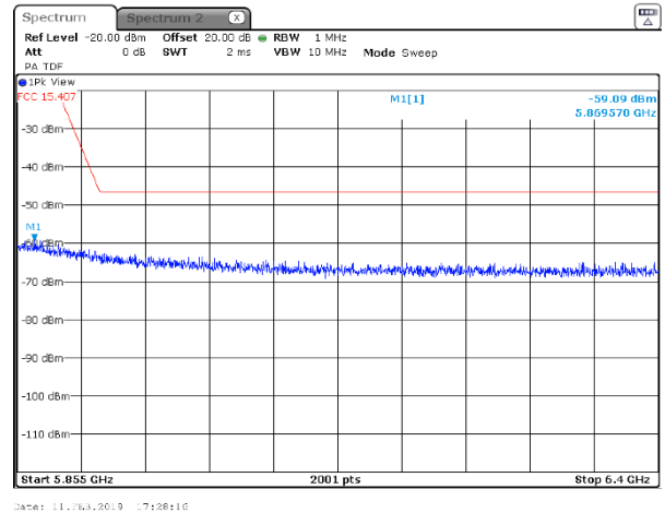
Plot 7.7.19 Conducted spurious emission measurements in the range 5.85 – 6.4 GHz CARRIER FREQUENCY 5842.5 MHz CHANNEL BANDWIDTH 15 MHz
