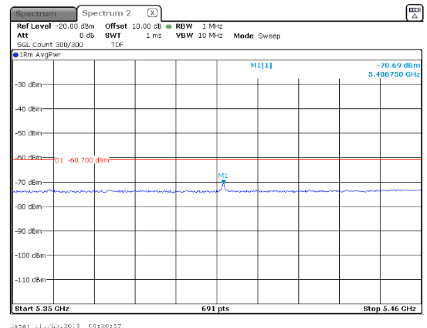
Plot 7.9.3 Conducted spurious emission measurements in the range 5.35 – 5.46 GHz CARRIER FREQUENCY 5160 MHz CHANNEL BANDWIDTH 10 MHz
