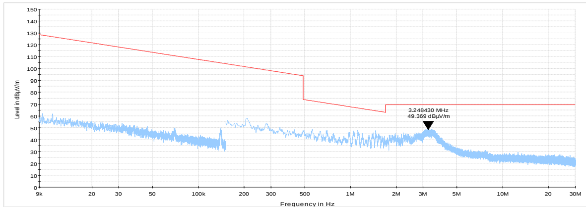
Plot 7.11.2 Radiated emission measurements from 9 kHz to 30 MHz at the mid carrier frequency
