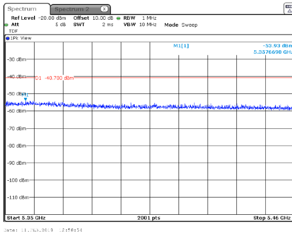
Plot 7.9.27 Conducted spurious emission measurements in the range 5.35 – 5.46 GHz
