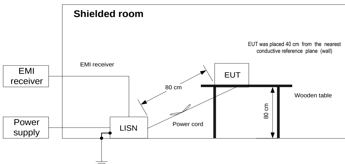
Figure 7.13.1 Setup for conducted emission measurements, table-top equipment
