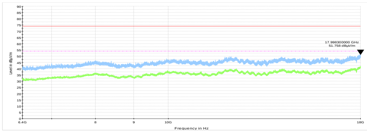
Plot 7.12.14 Radiated emission measurements from 6.4 to 18 GHz at the mid carrier frequency
