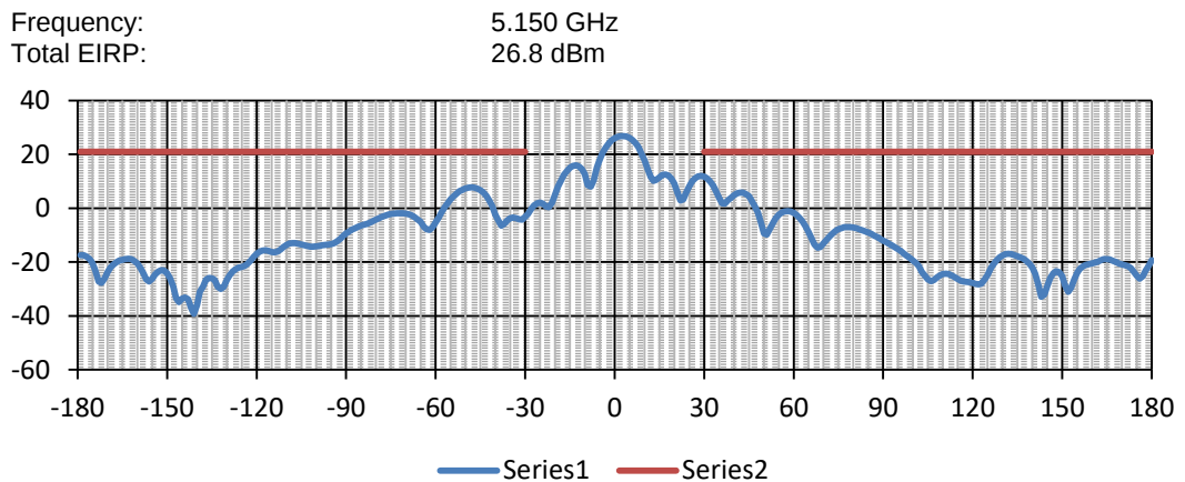
Plot 7.15.1 Antenna pattern test results, Antenna #1
