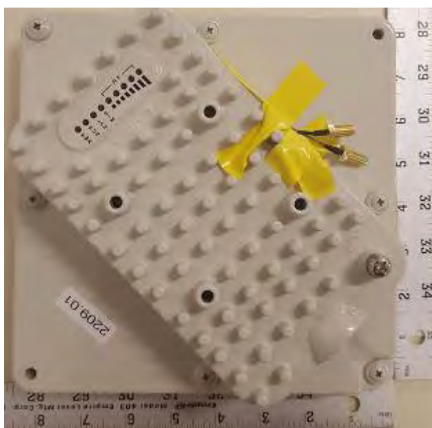
Figure B2. DUT rear view
