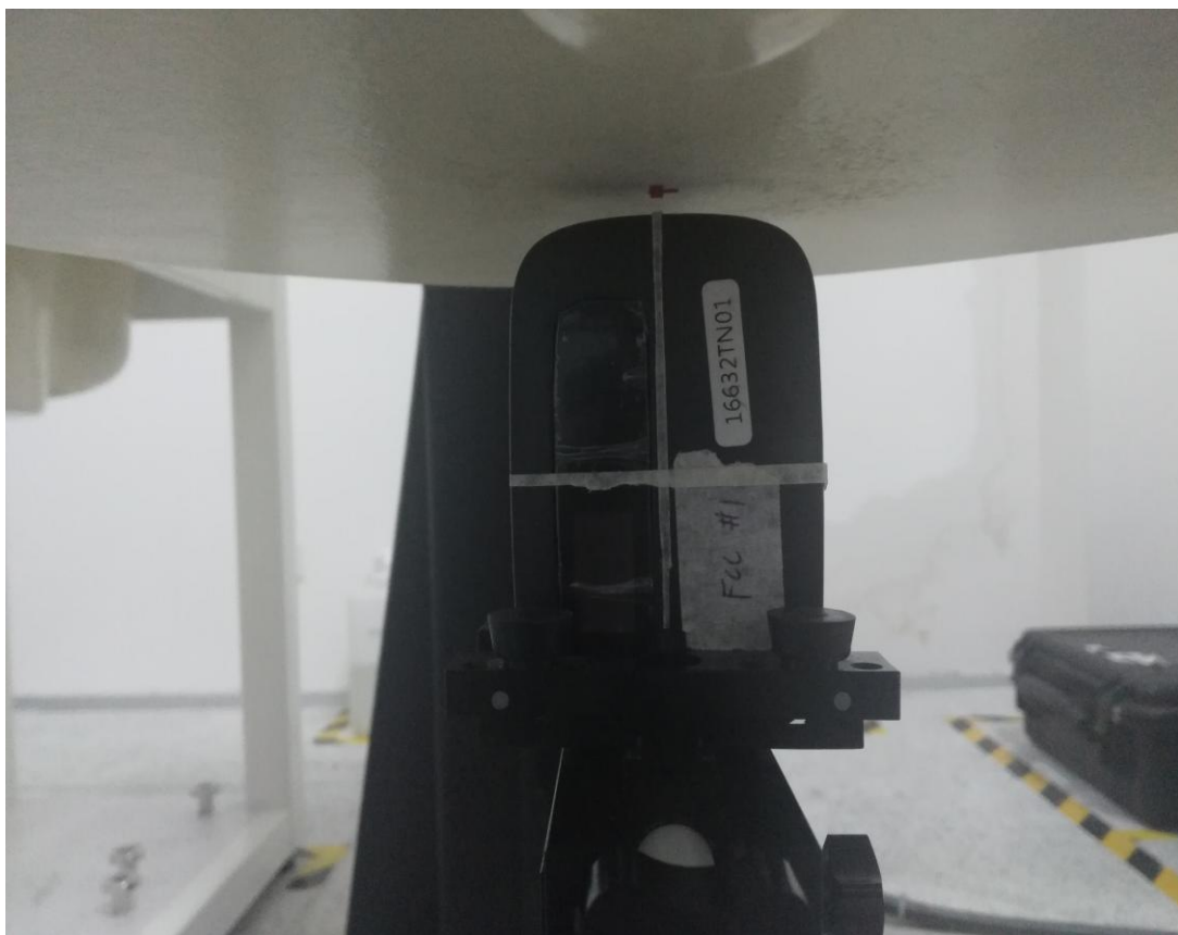
POSITION OF BODY RIGHT SIDE WITH 5mm DISTANCE
