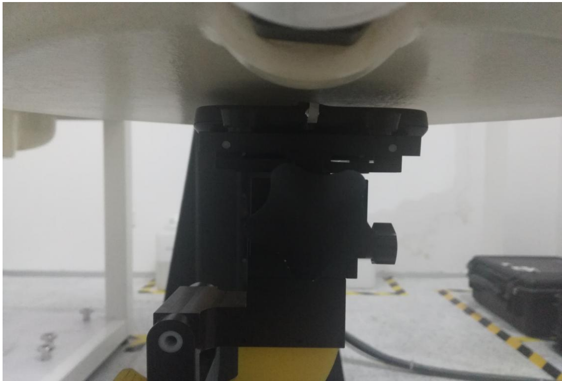
POSITION OF BODY TOWARDS PHANTOM WITH 5mm DISTANCE
