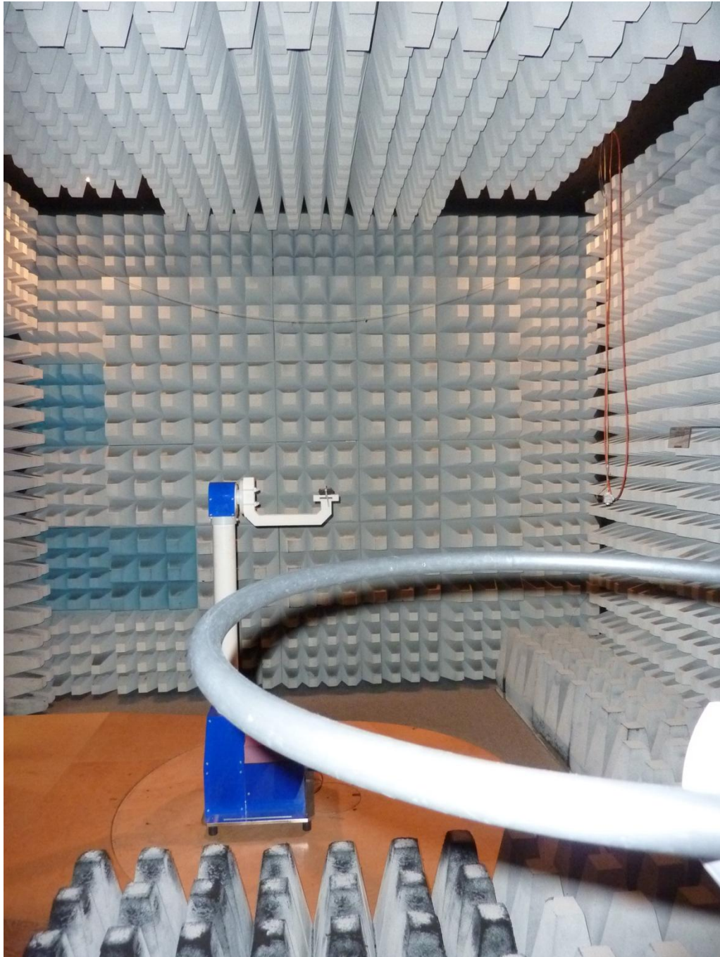
171626_e.JPG: Barryvox S, test setup fully anechoic chamber
