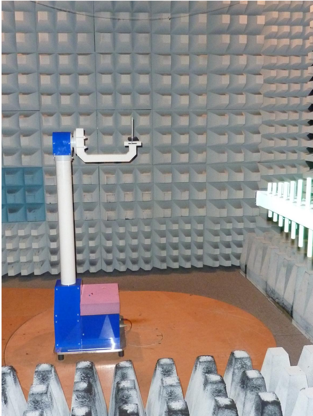
171626_d.JPG: Barryvox S, test setup fully anechoic chamber
