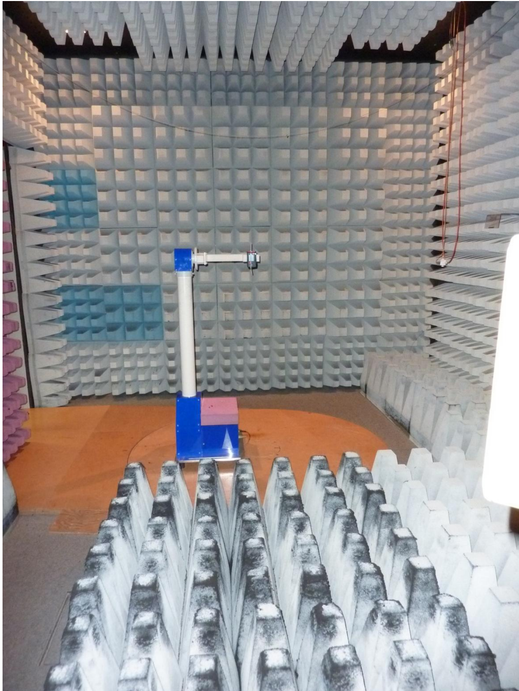
171626_g.JPG: Barryvox S, test setup fully anechoic chamber
