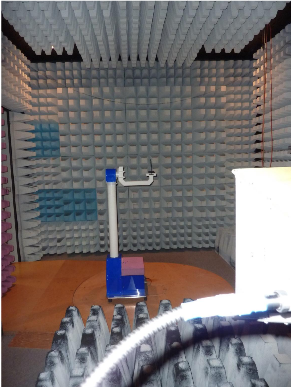
171626_s.JPG: Barryvox, test setup fully anechoic chamber
