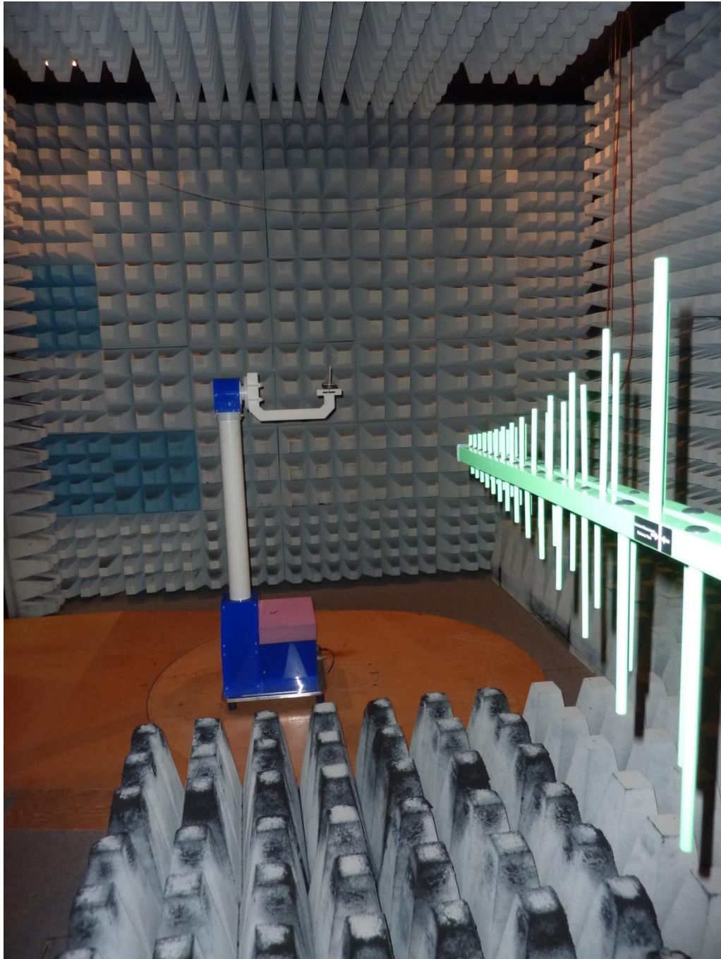
171626_q.JPG: Barryvox, test setup fully anechoic chamber
