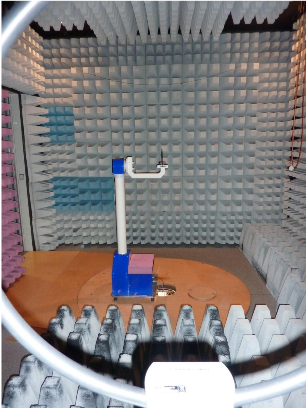
171626_r.JPG: Barryvox, test setup fully anechoic chamber
