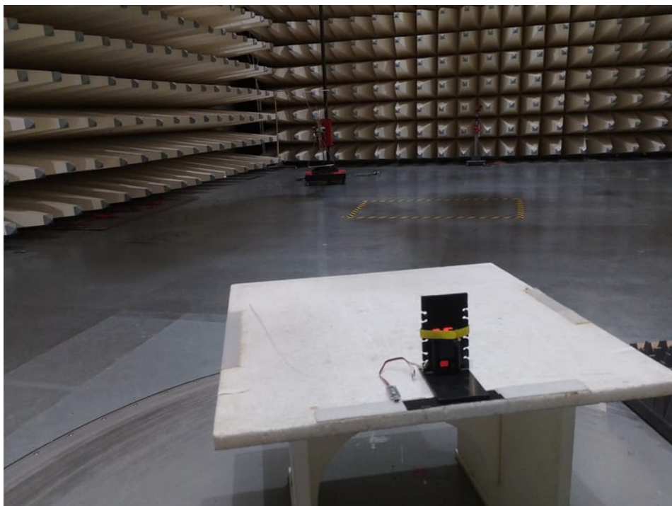
Photo 13: Barryvox S2
