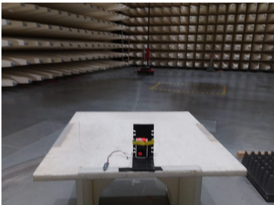
Photo 14: Barryvox 2
