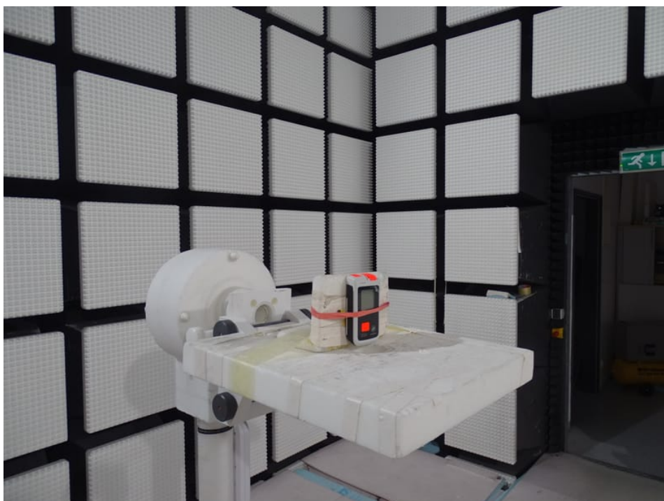
Photo 4: Barryvox 2
