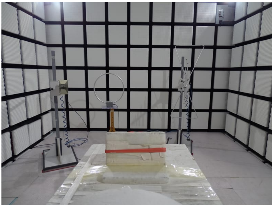
Photo 9: Barryvox S2
