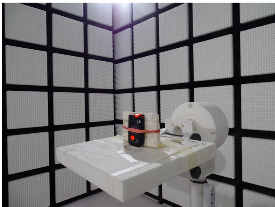
Photo 8: Barryvox S2
