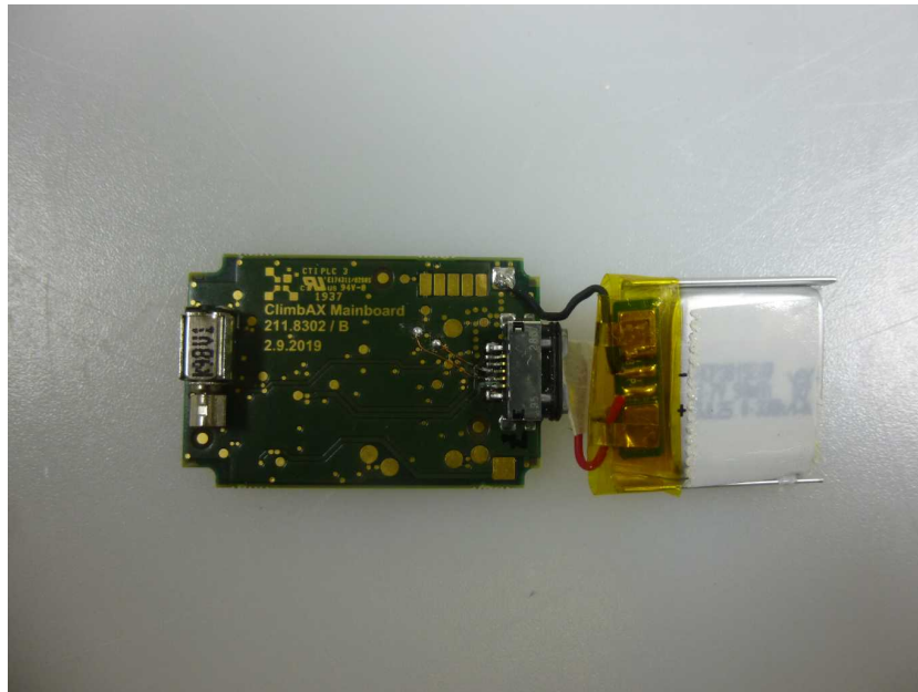
Photo 7: PCB 2, back side view
