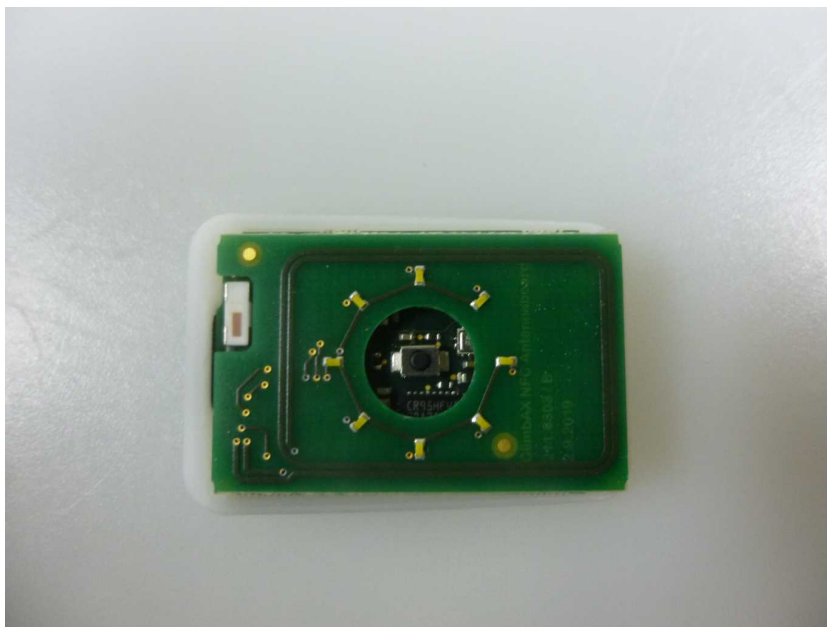
Photo 2: PCB 1, front side view
