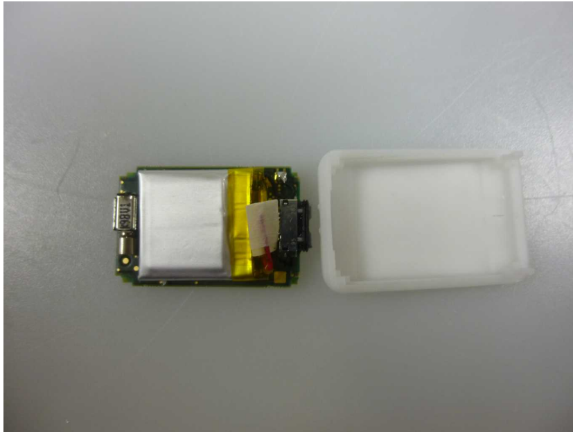
Photo 5: Back cover removed
