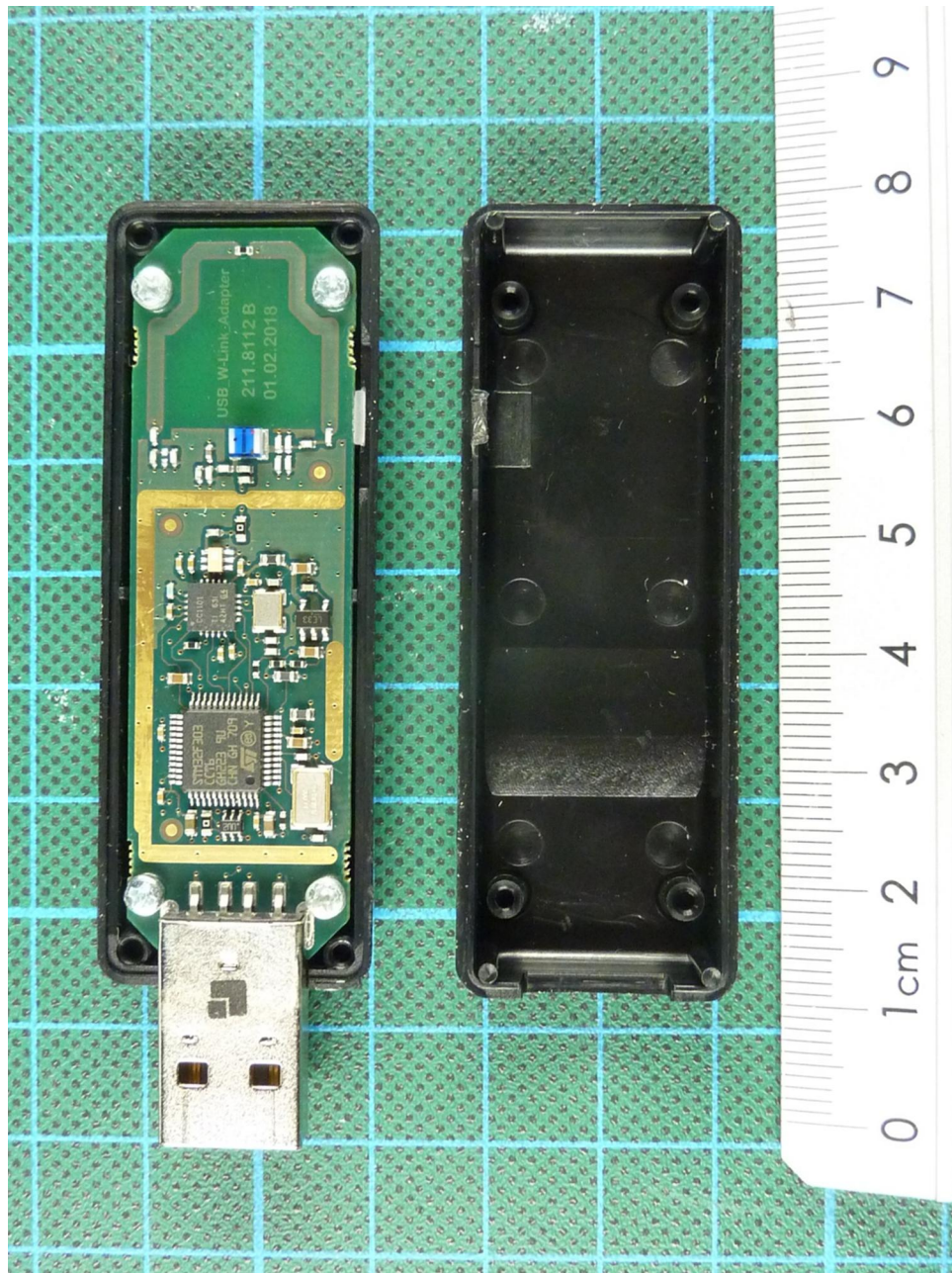
180803_e.JPG: W-LINK STICK, internal view
