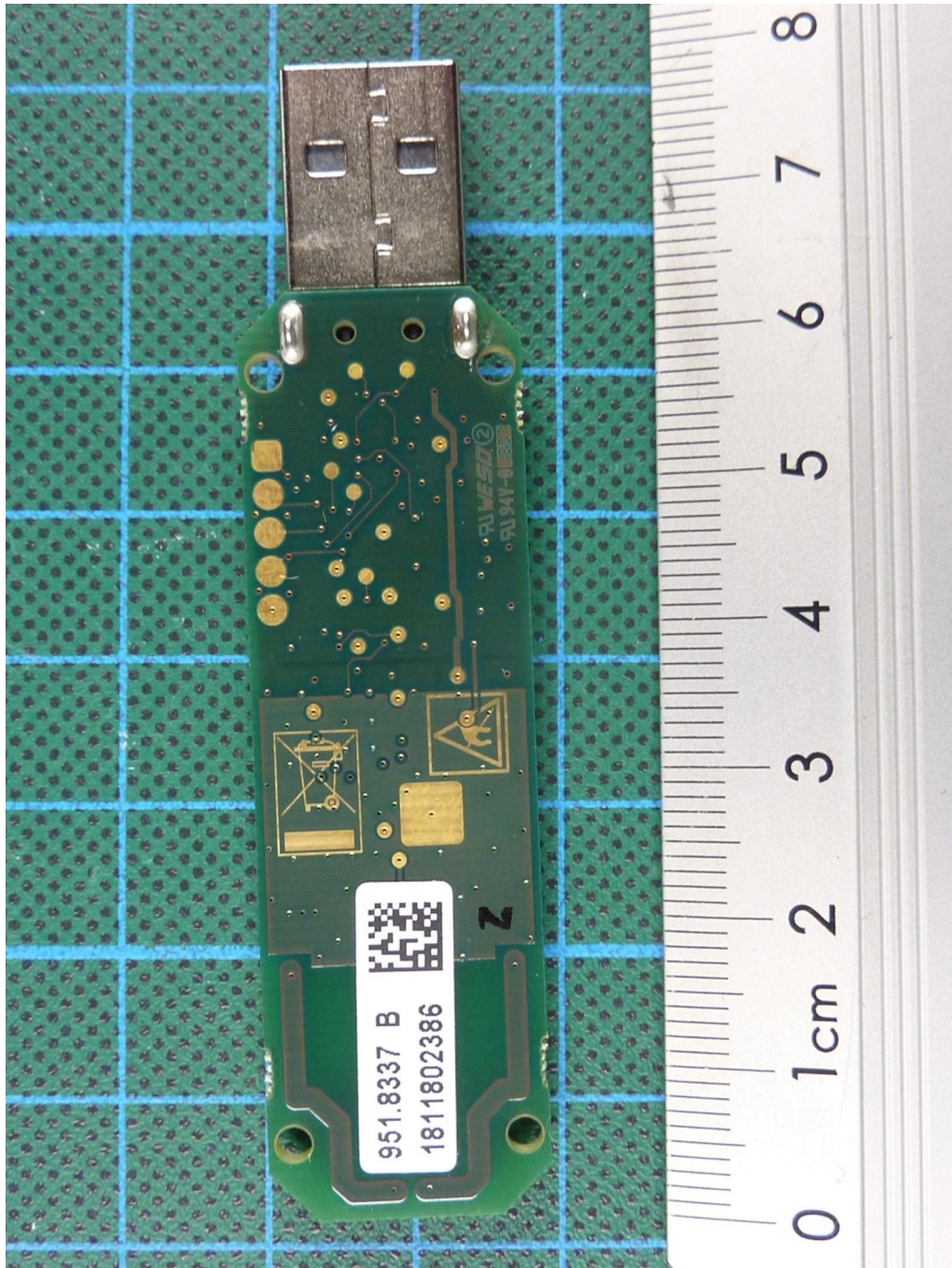
180803_g.JPG: W-LINK STICK, PCB, bottom view
