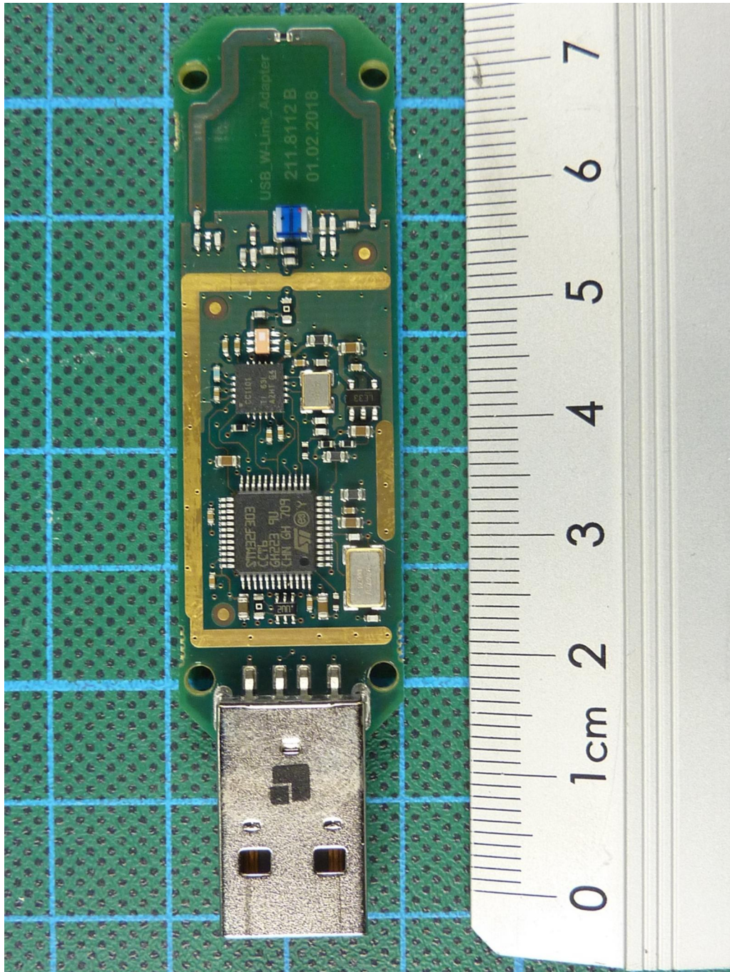
180803_f.JPG: W-LINK STICK, PCB, top view
