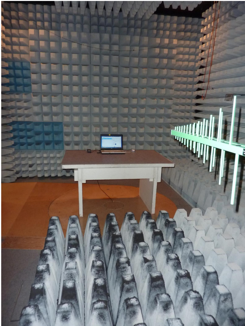
180803_14.JPG: W-LINK STICK, test setup fully anechoic chamber
