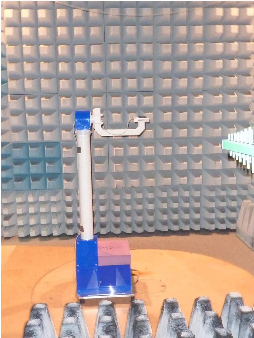
180803_4.JPG: W-LINK STICK, test setup fully anechoic chamber
