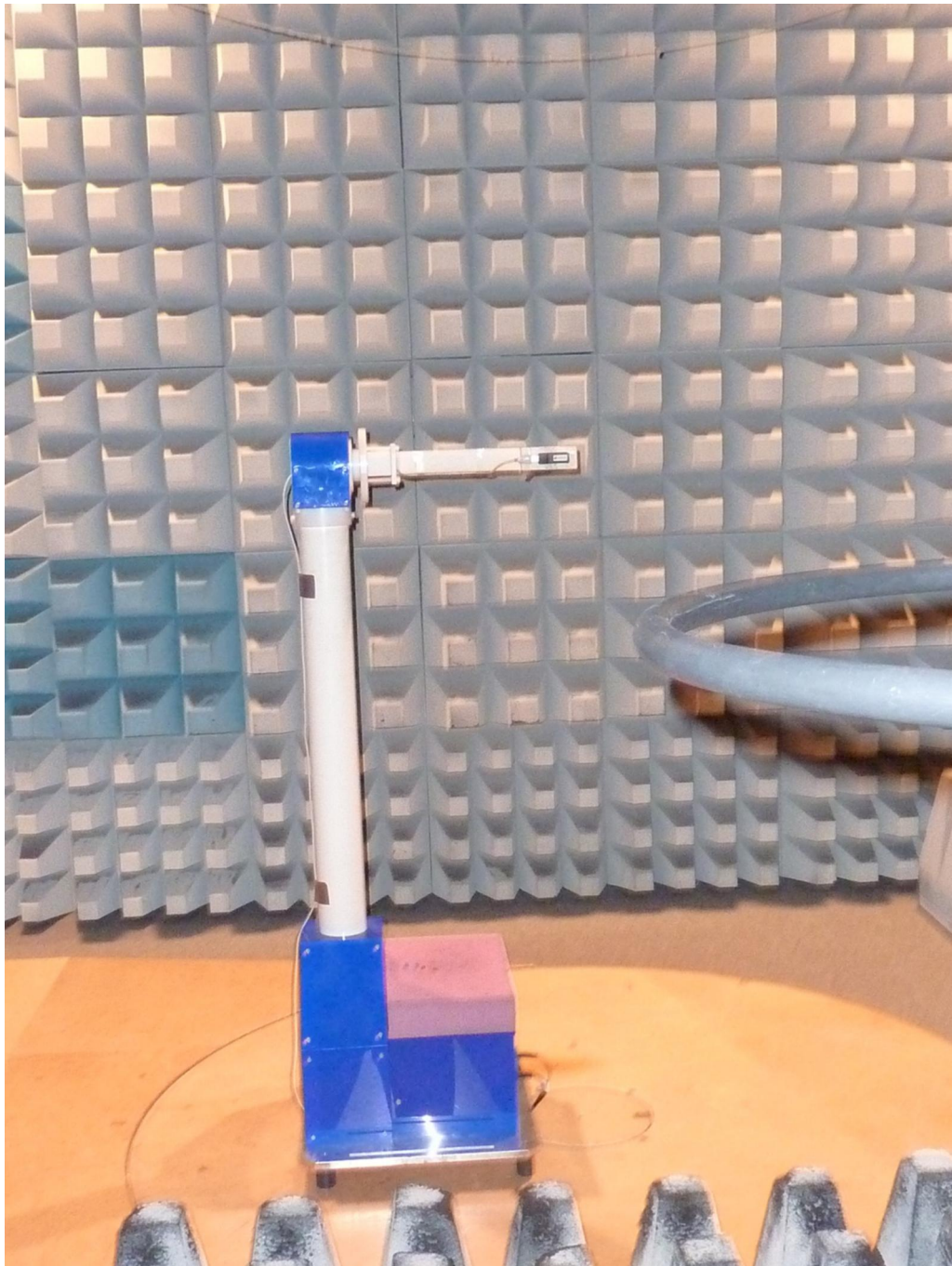
180803_3.JPG: W-LINK STICK, test setup fully anechoic chamber
