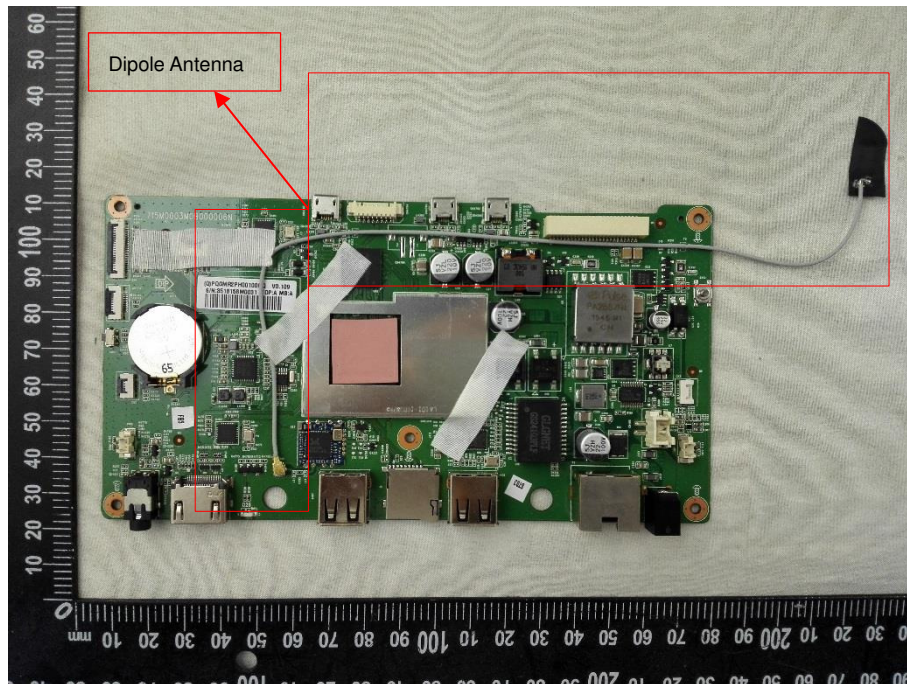
MAIN BOARD TOP VIEW 1 (10BDL3051T)
