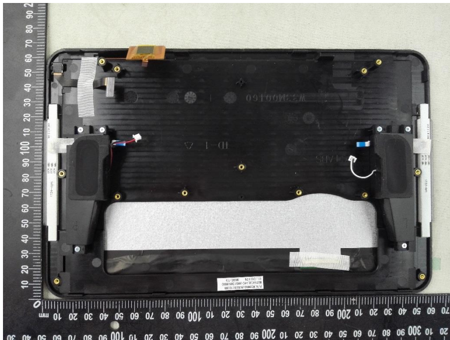
EUT UNCOVER VIEW 5 (10BDL3050Q)
