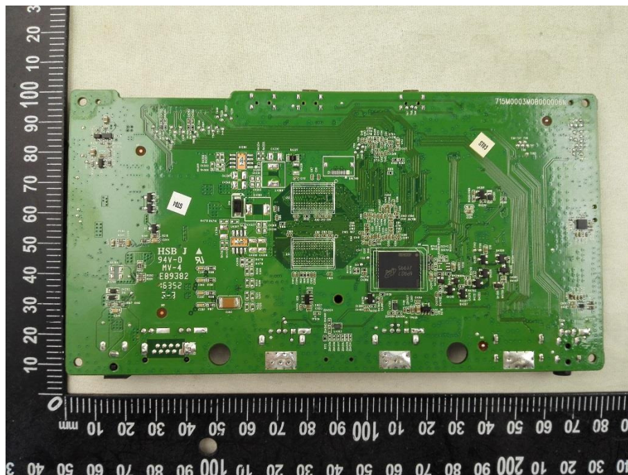
MAIN BOARD BACK VIEW 1 (10BDL3051T)
