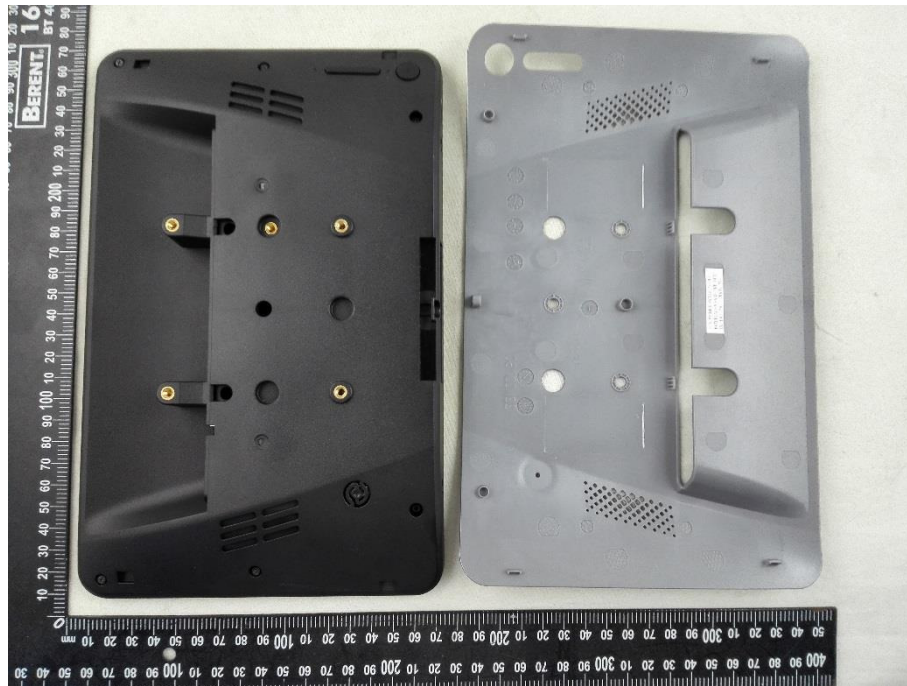
EUT UNCOVER VIEW 1 (10BDL3051T)
